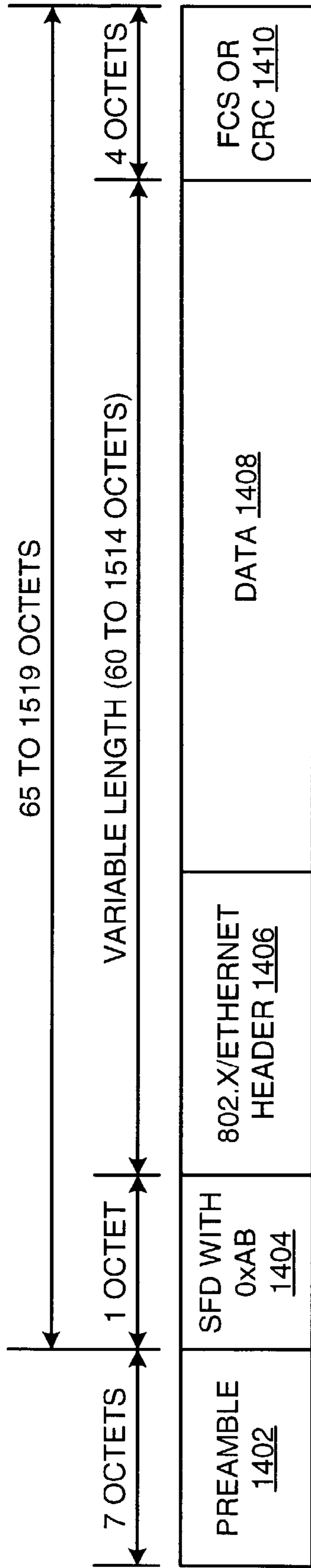
FIG. 14 - PRIOR ART
