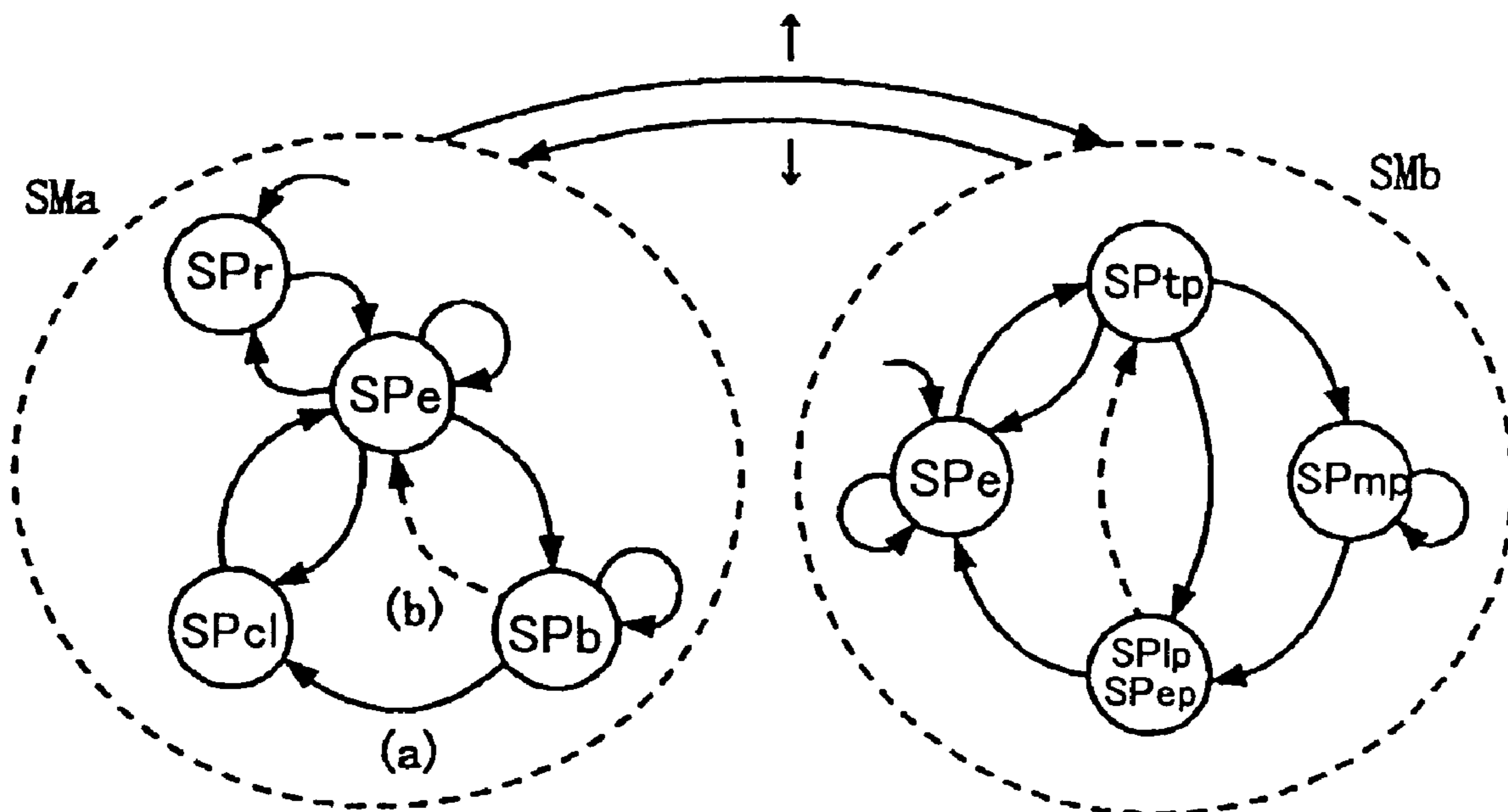
State Machine
