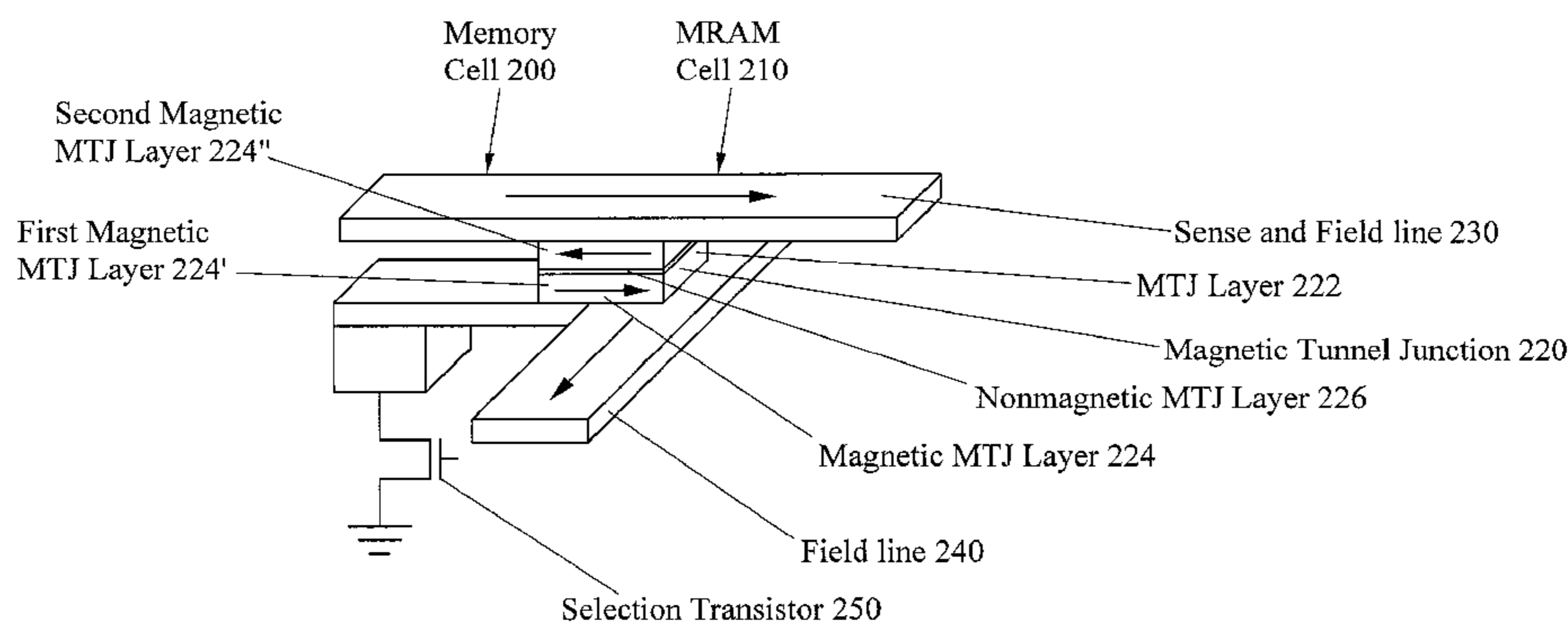
MEMORY SYSTEM 100
