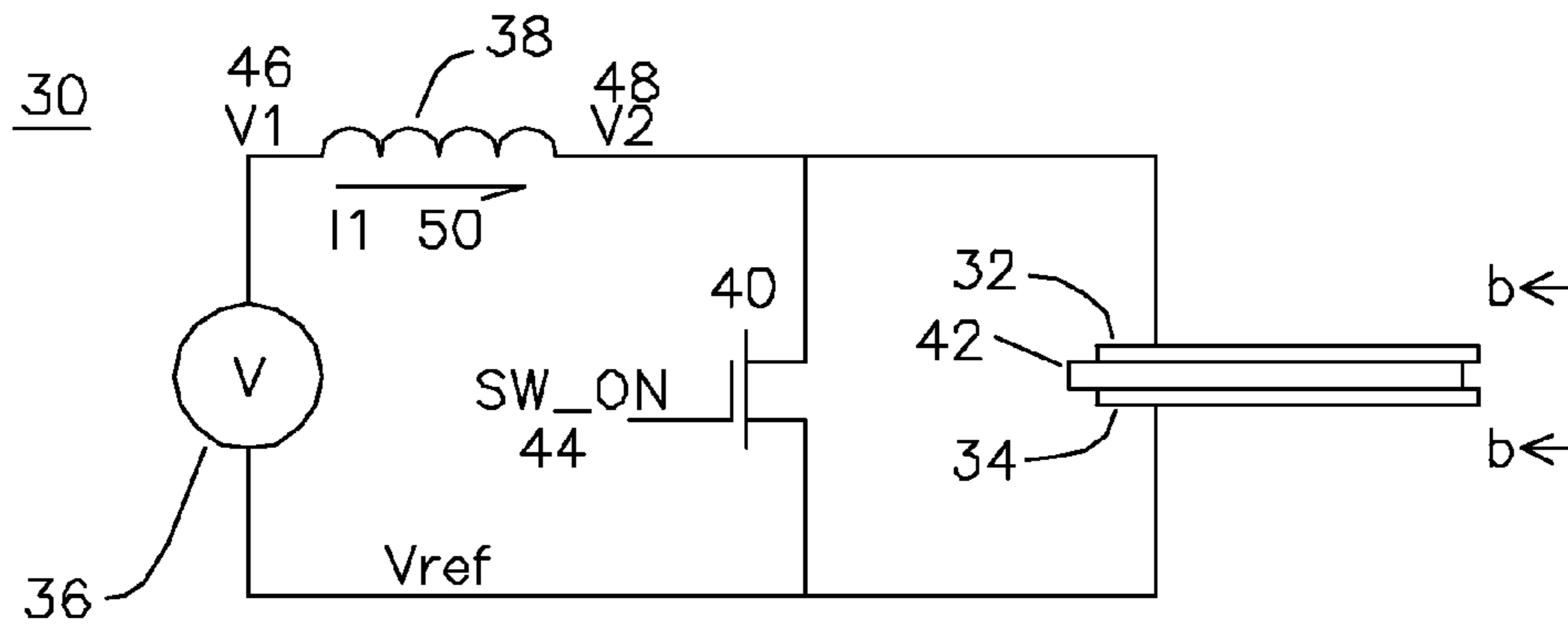
Figure 2: Low Voltage Pulsed Plasma Thruster
