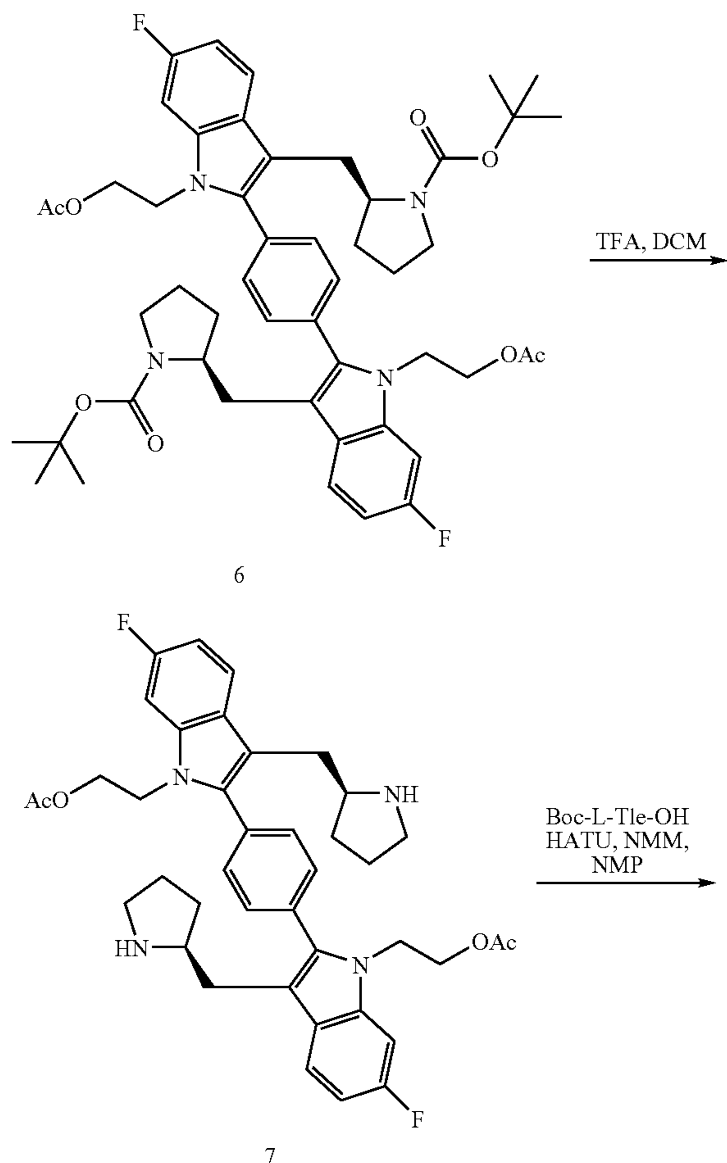
Scheme III
