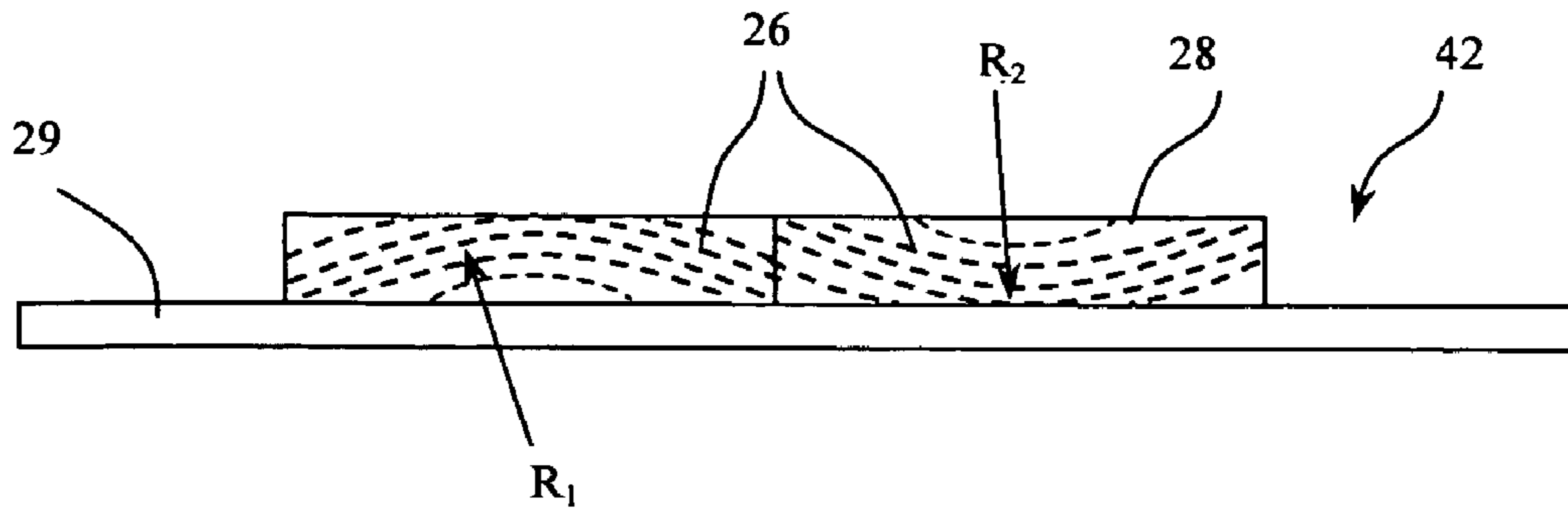
Fig. 2D (cross-section)
