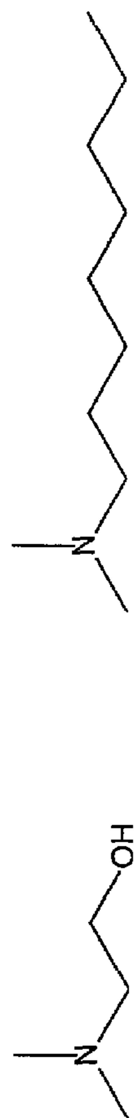
N,N - Dimethylethanolamine
