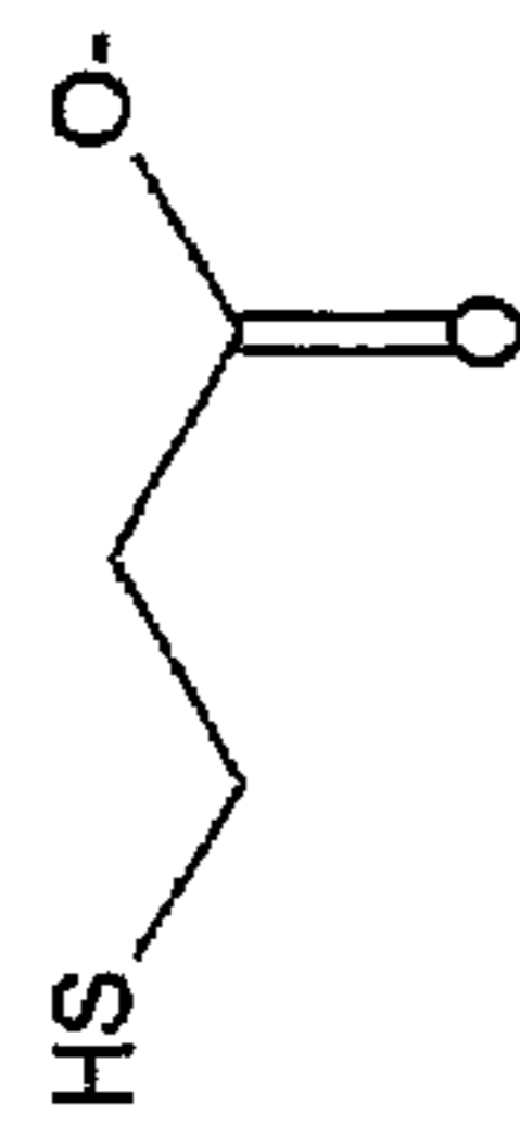
3-Mercaptopropionate
