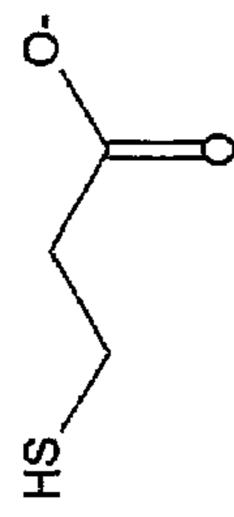
3-Mercaptopropionate
