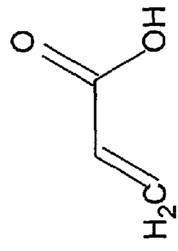
Acrylic Acid
