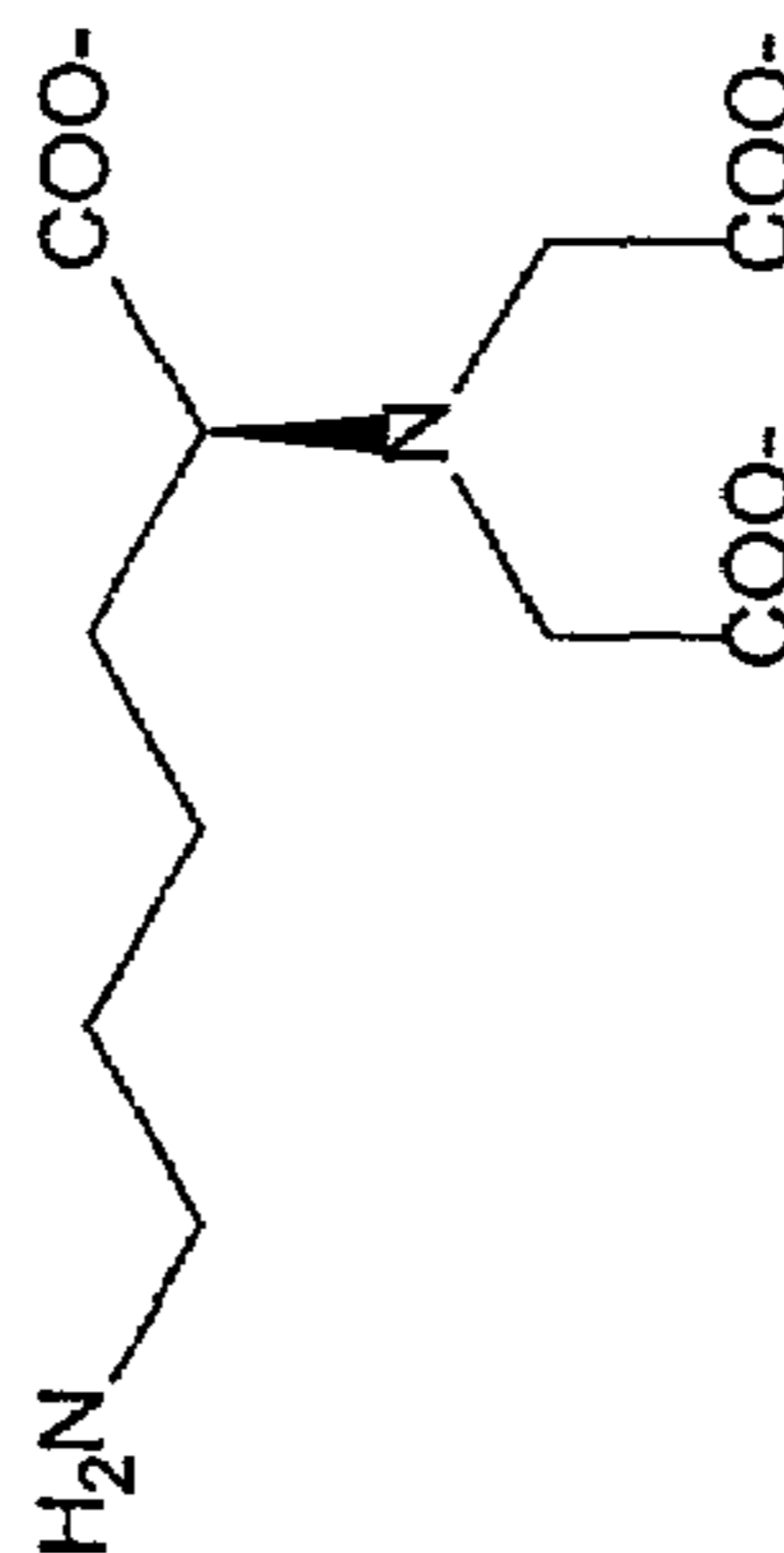
N,N - Bis(carboxymethyl)-L-Lysine
