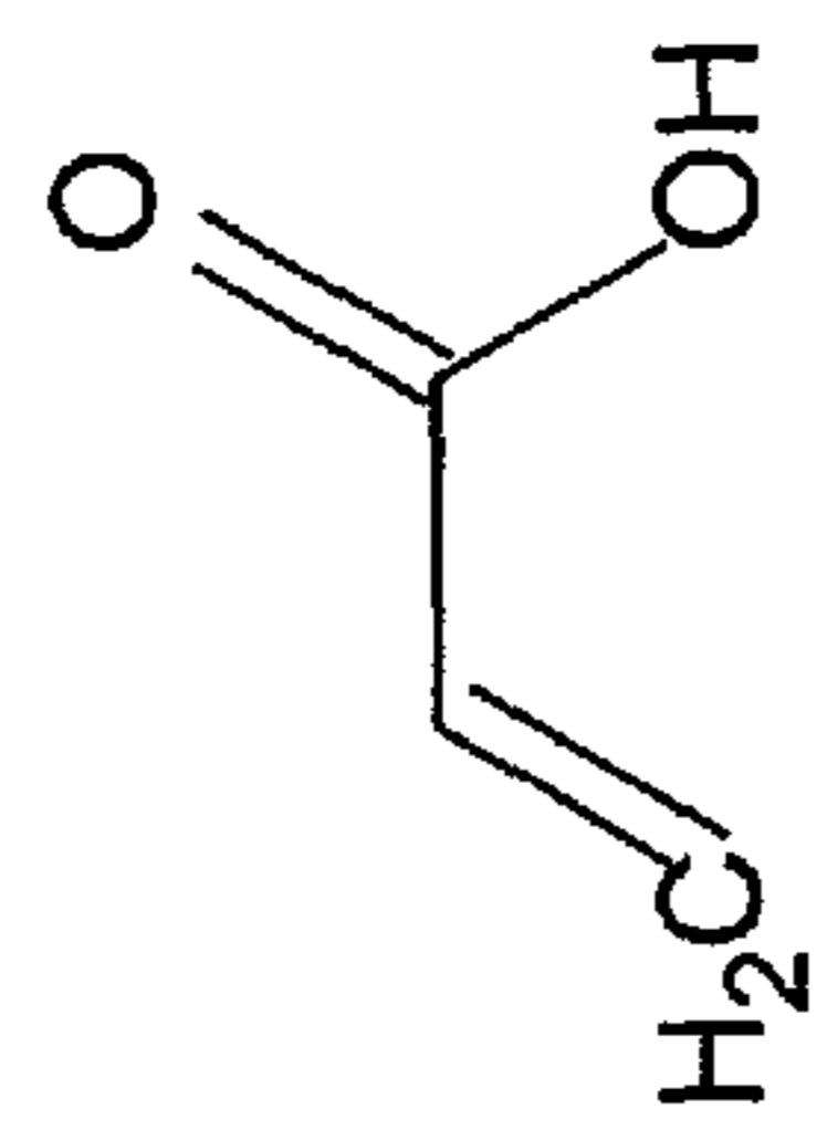
Acrylic Acid
