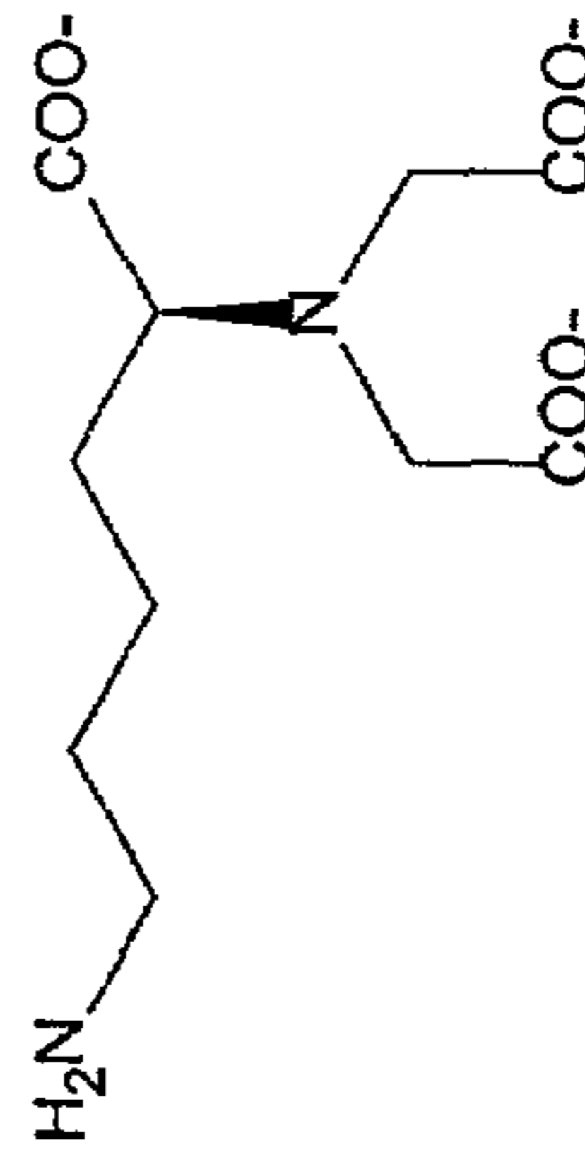
N,N - Bis(carboxymethyl)-L-Lysine
