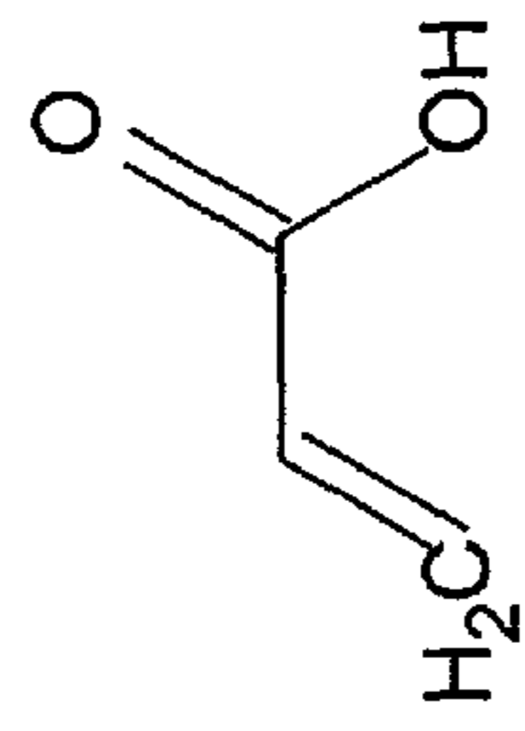
Acrylic Acid
