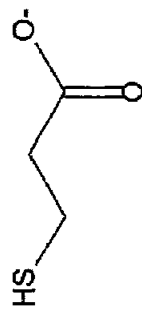
3-Mercaptopropionate
