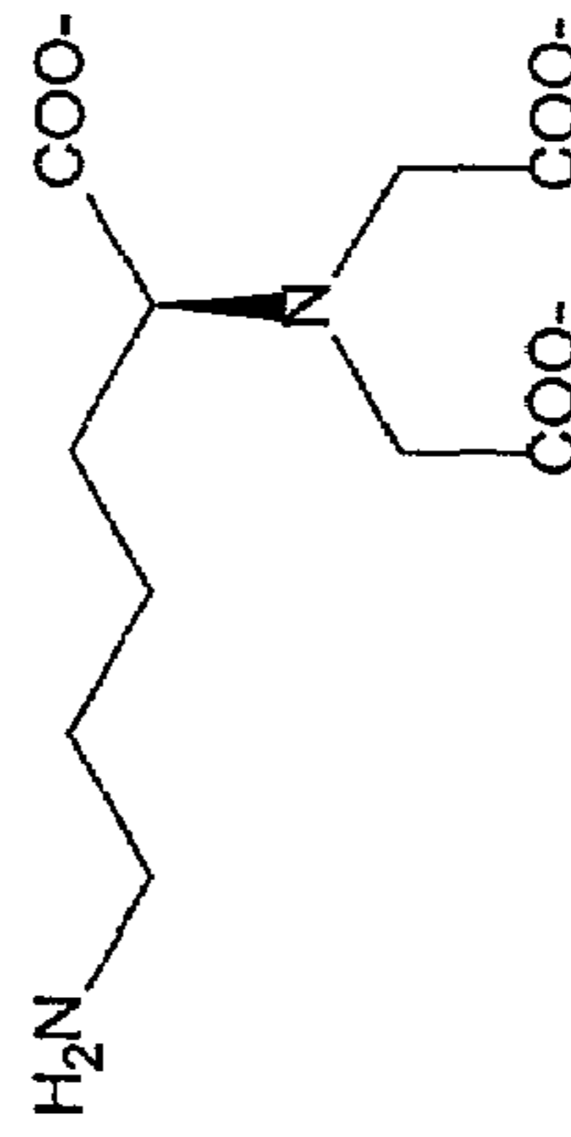
N,N - Bis(carboxymethyl)-L-Lysine
