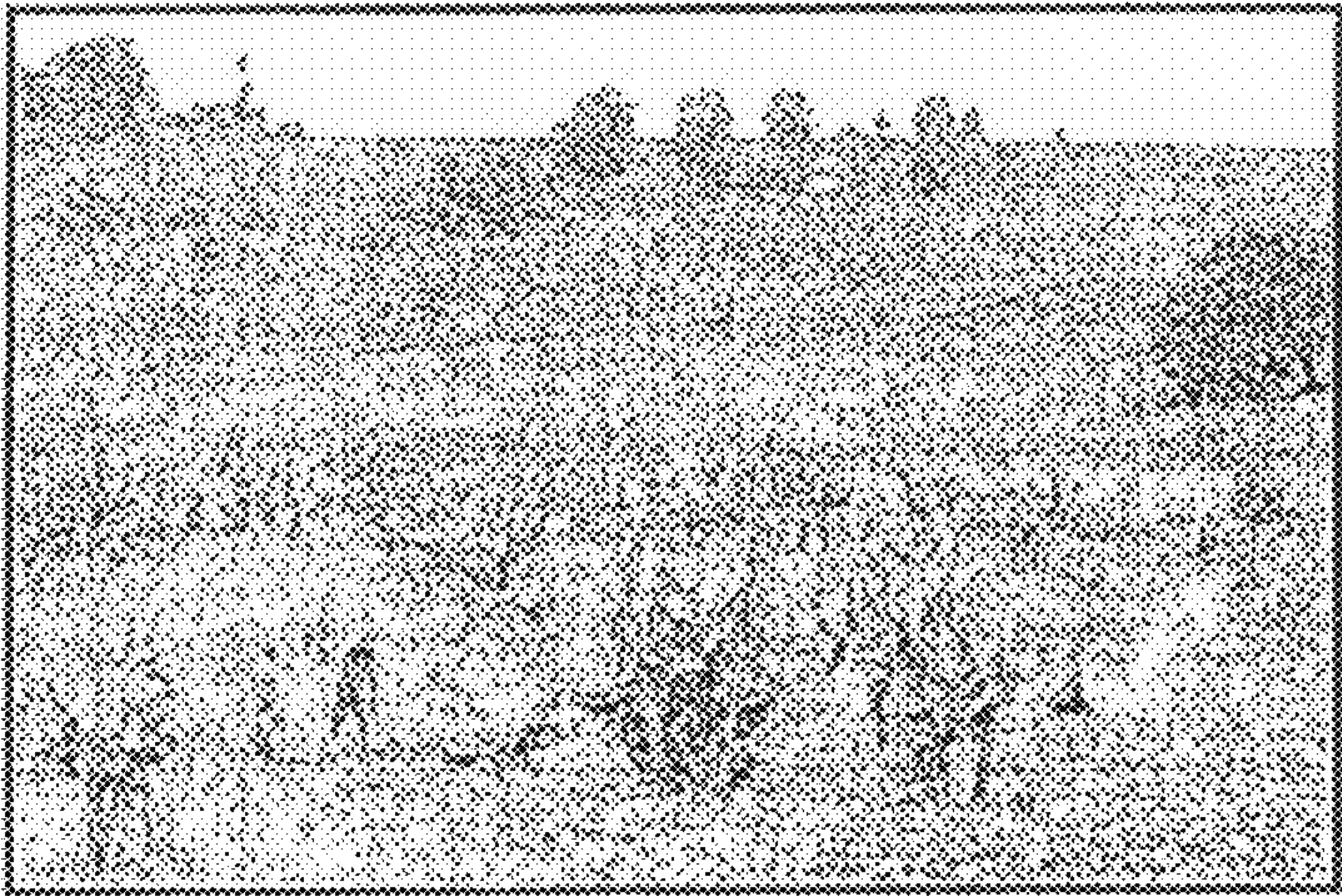
Fig 24 A distant shot of the FlipFlop in operation. The man second from left is pumping water from a stream while the man on the right directs the spray of water into crops through a nozzle.
