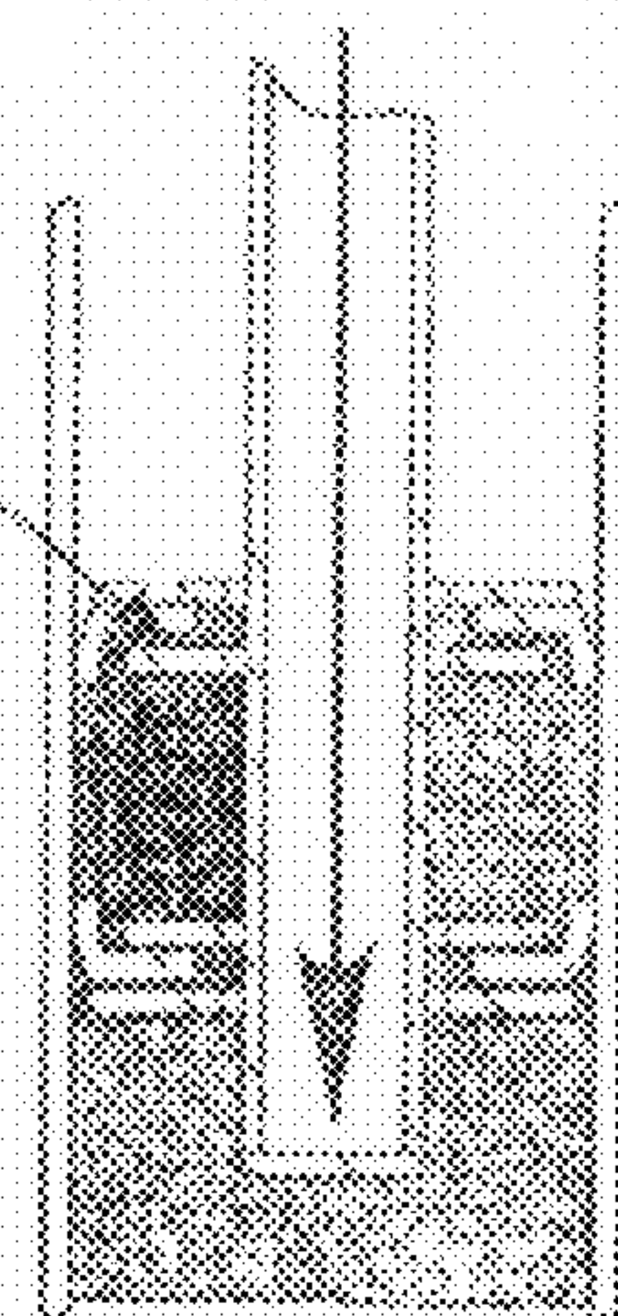
Fig 39 Leak valve closing as inter-valve space is filled with water.
