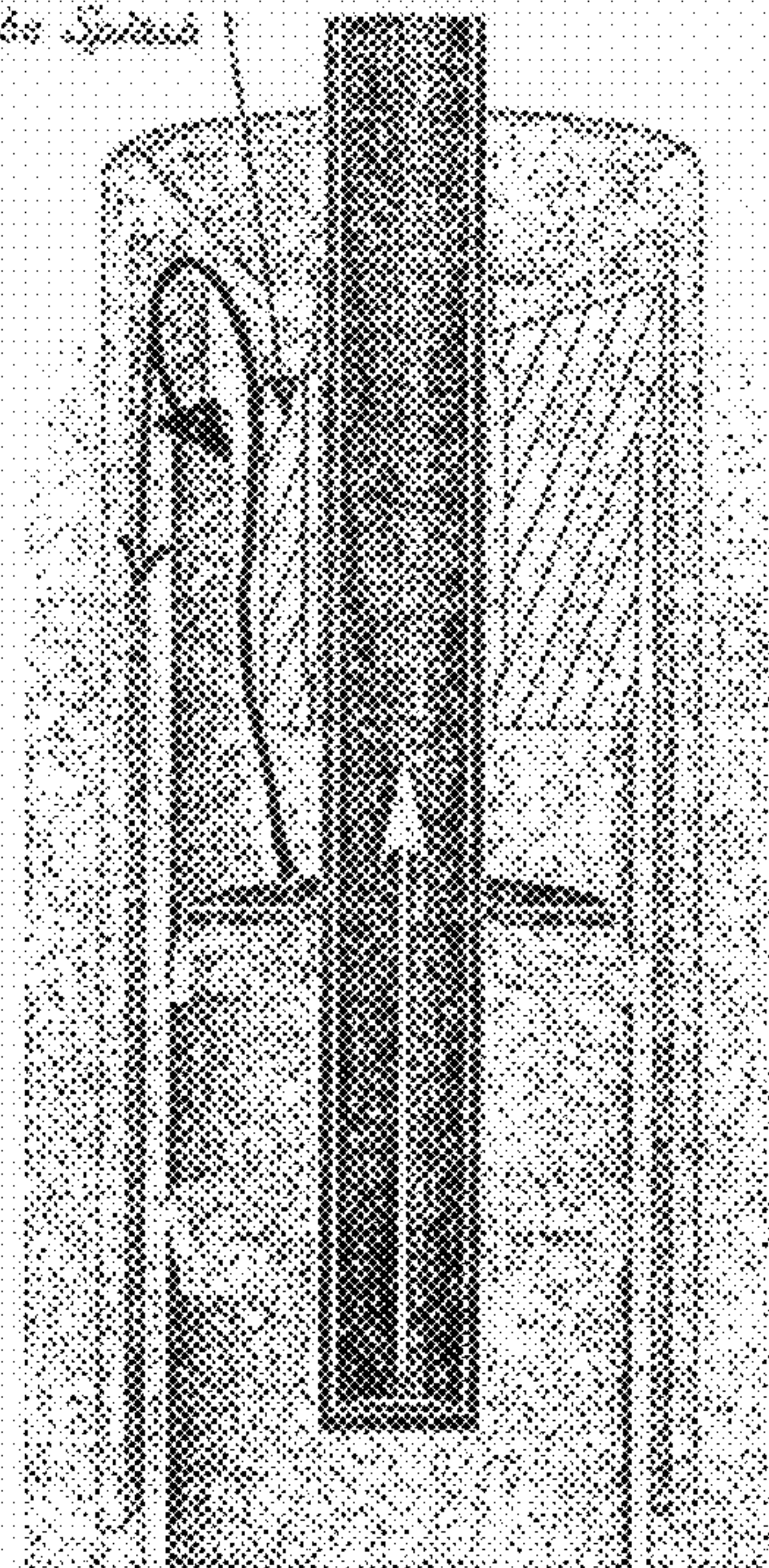
Fig. 34 Redirection of water by the Splash Cap
