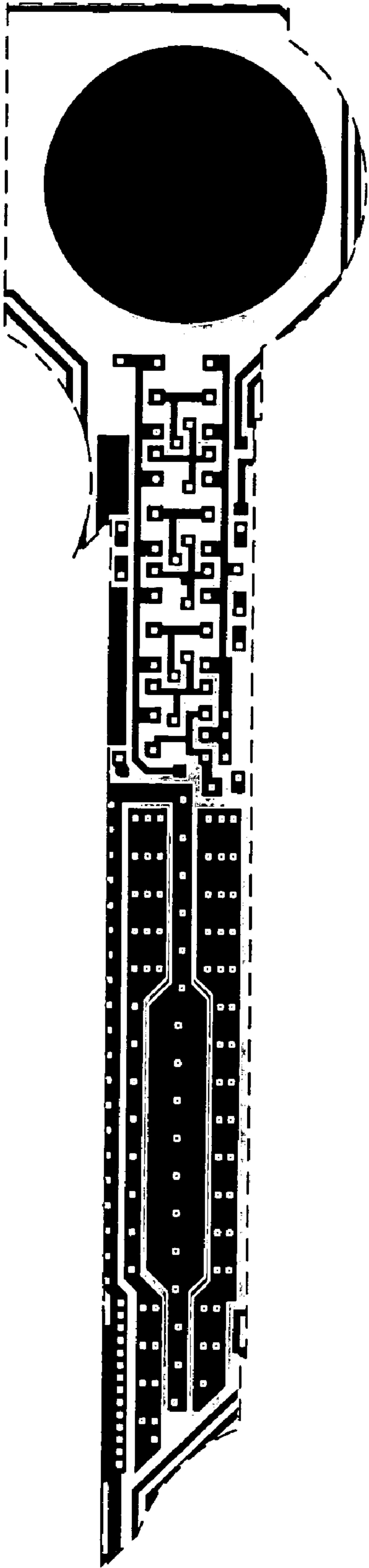
Metal 1 mask
