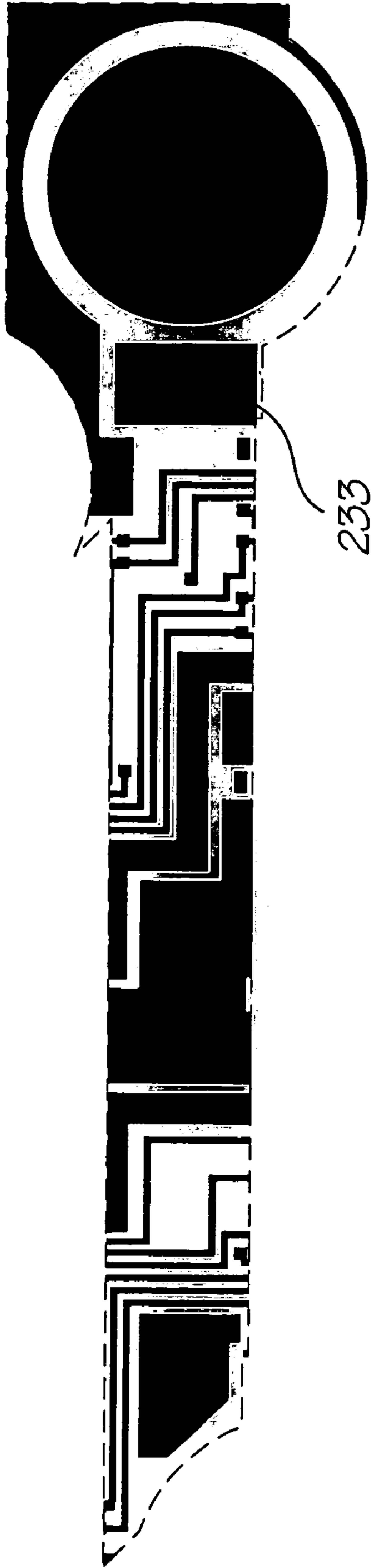
Metal 2 mask
