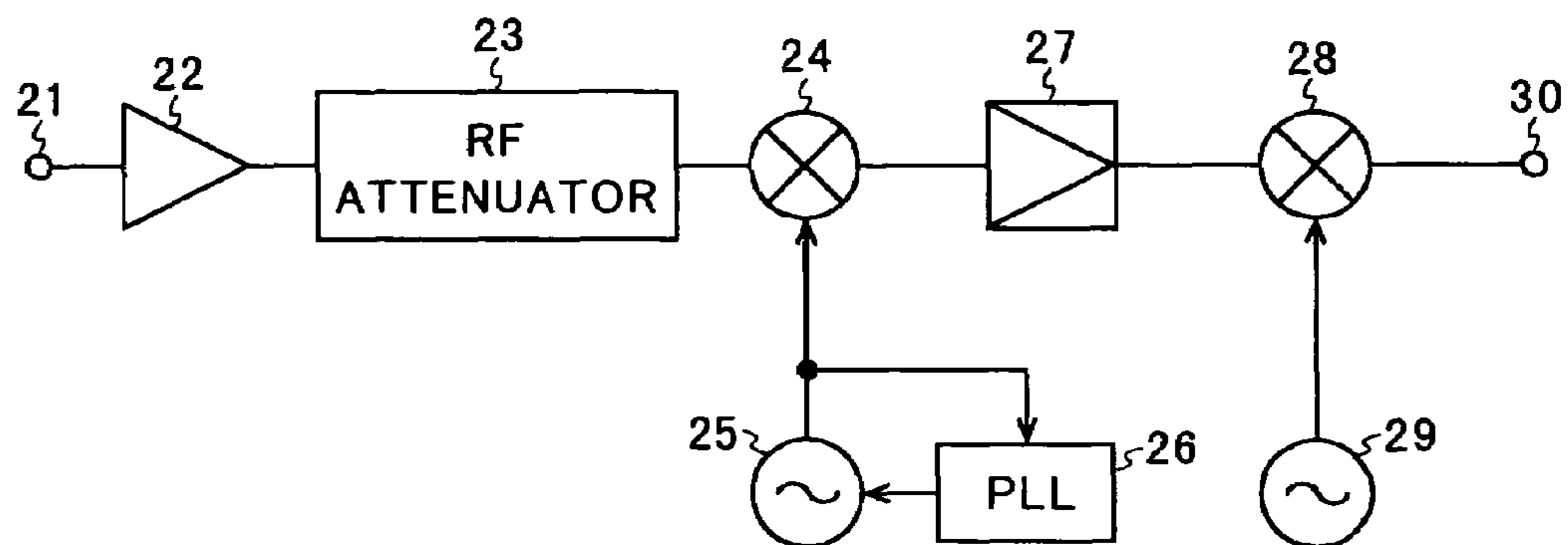
Prior Art Fig. 6
