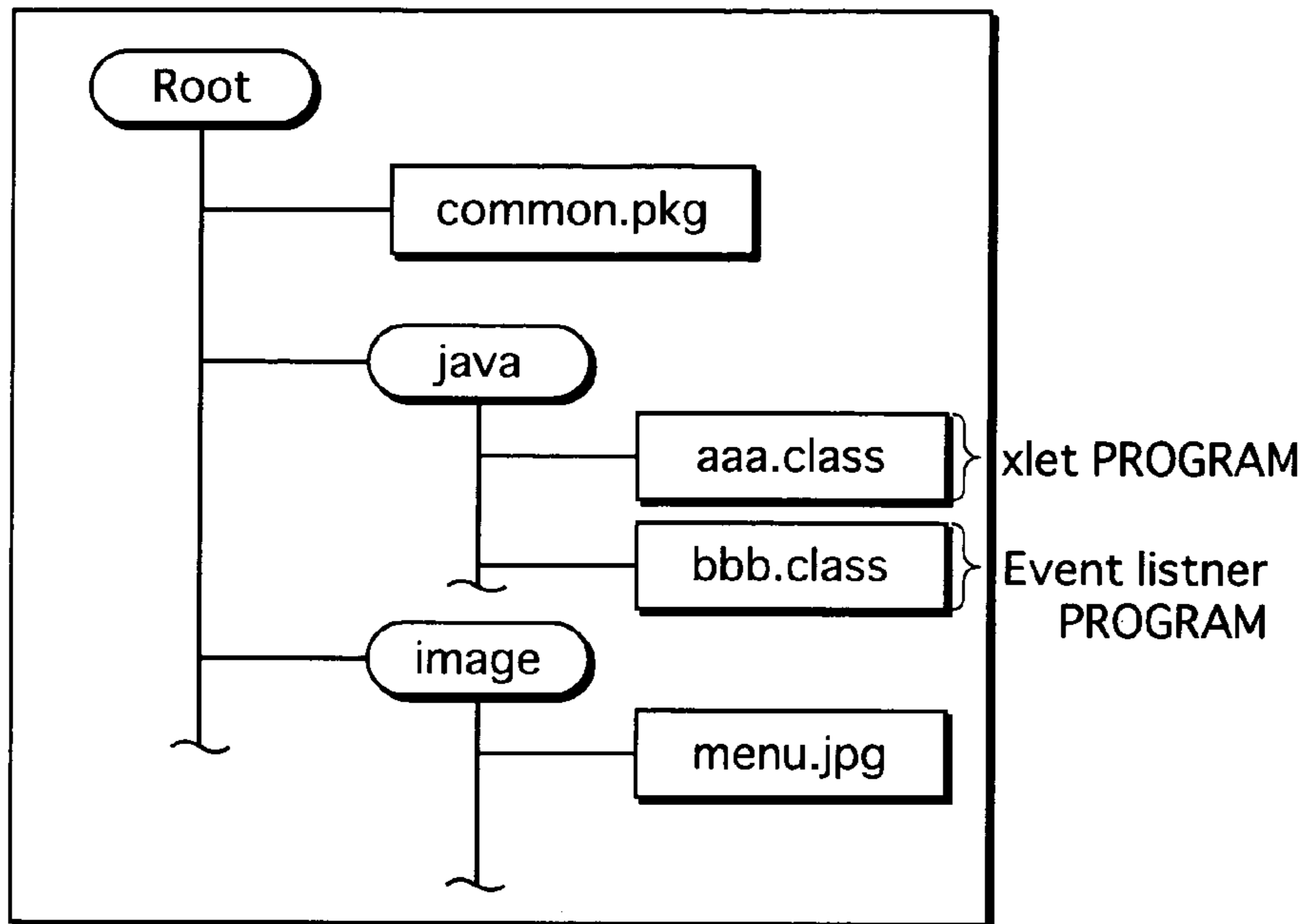
JAR FILE
