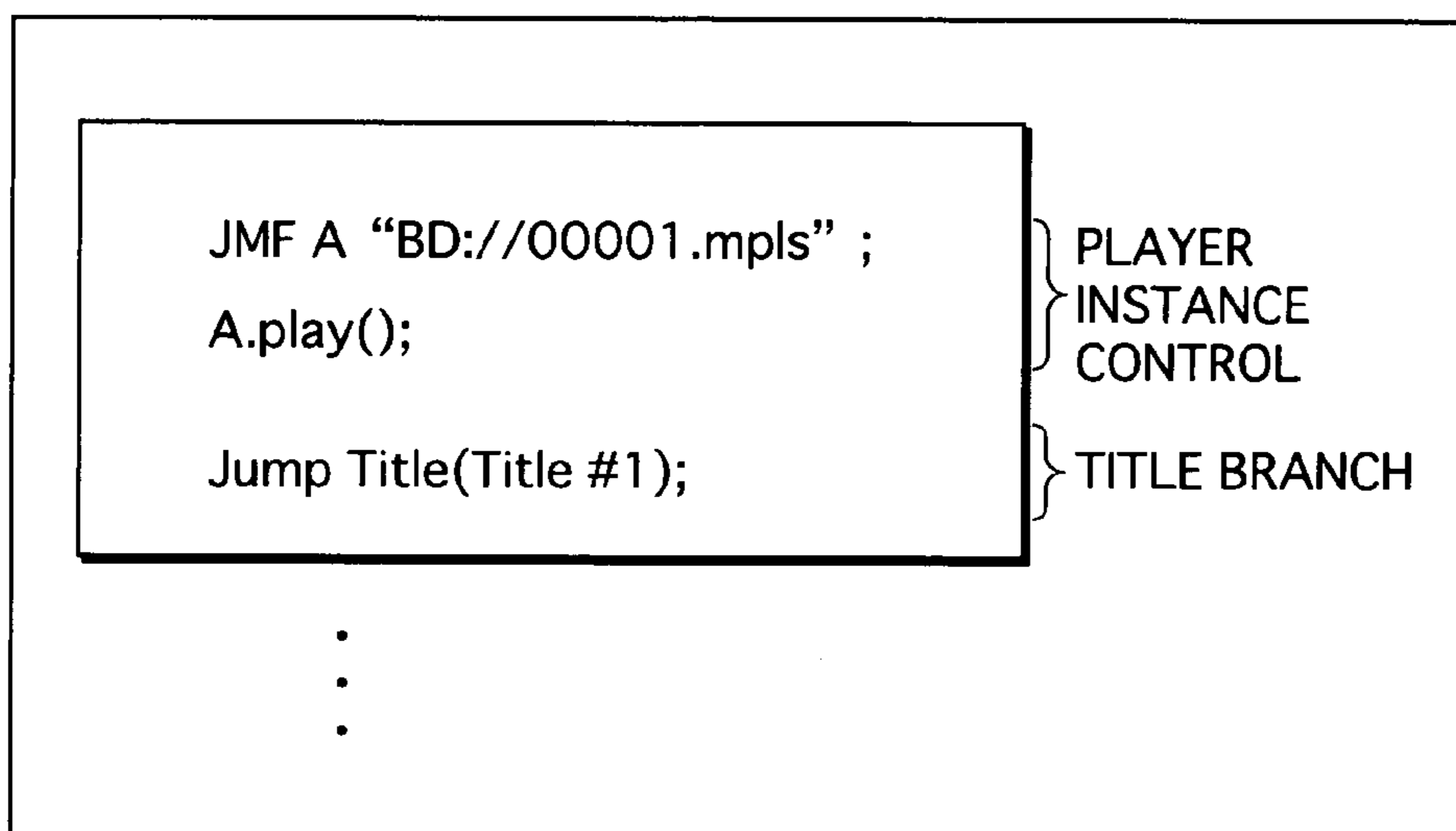
xlet PROGRAM
