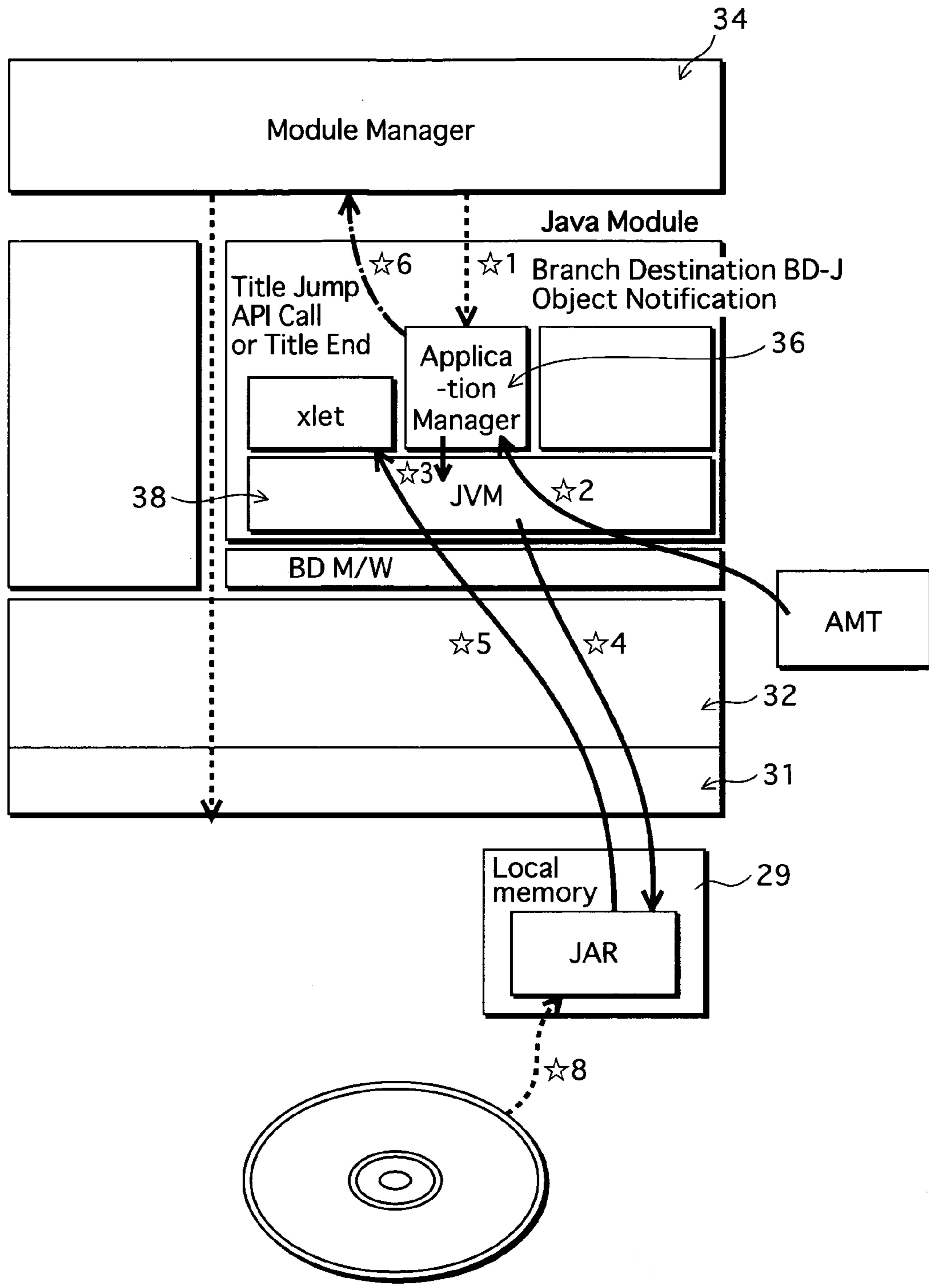
xlet LOAD AND RUN CONTROL
