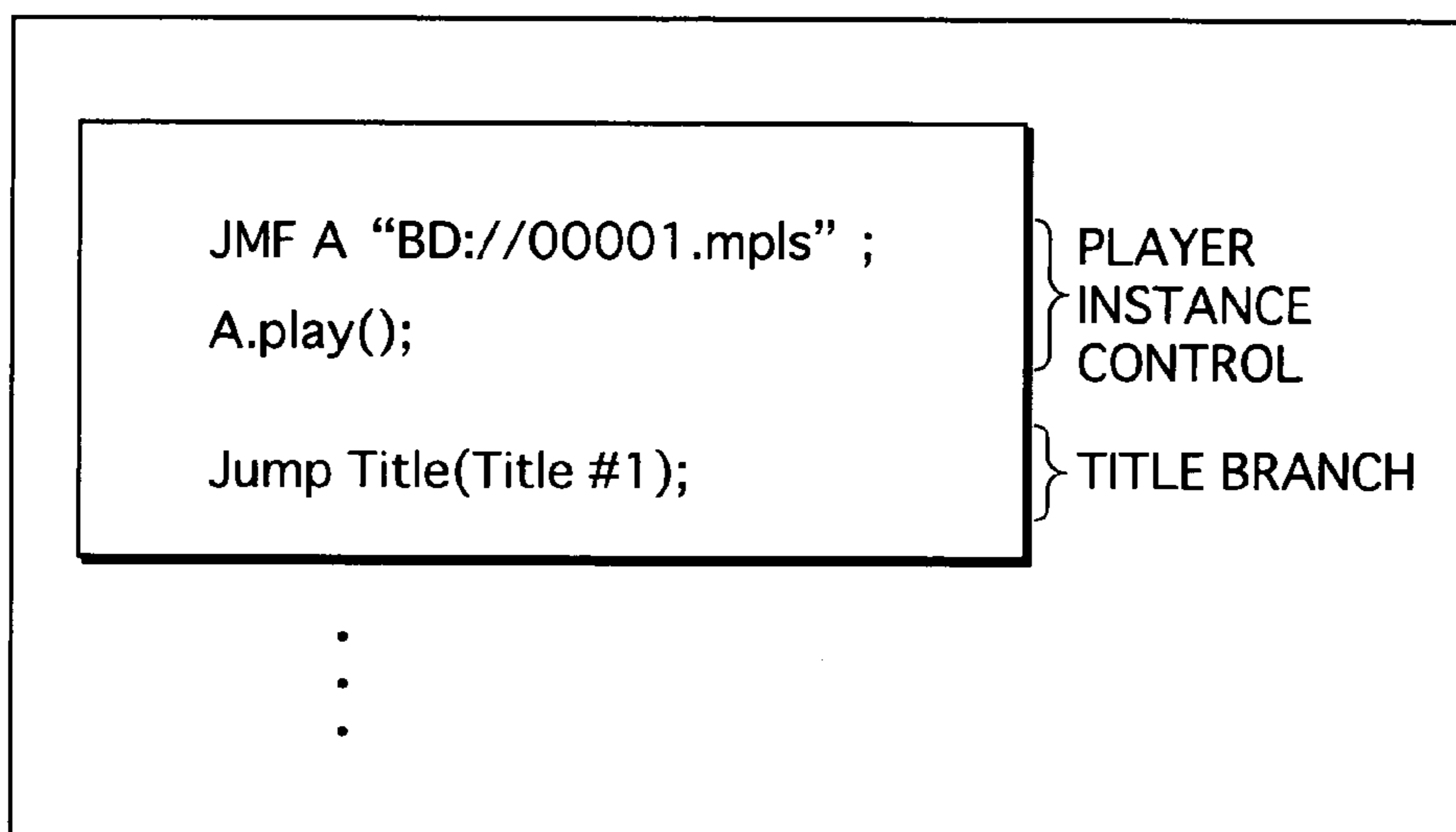
xlet PROGRAM
