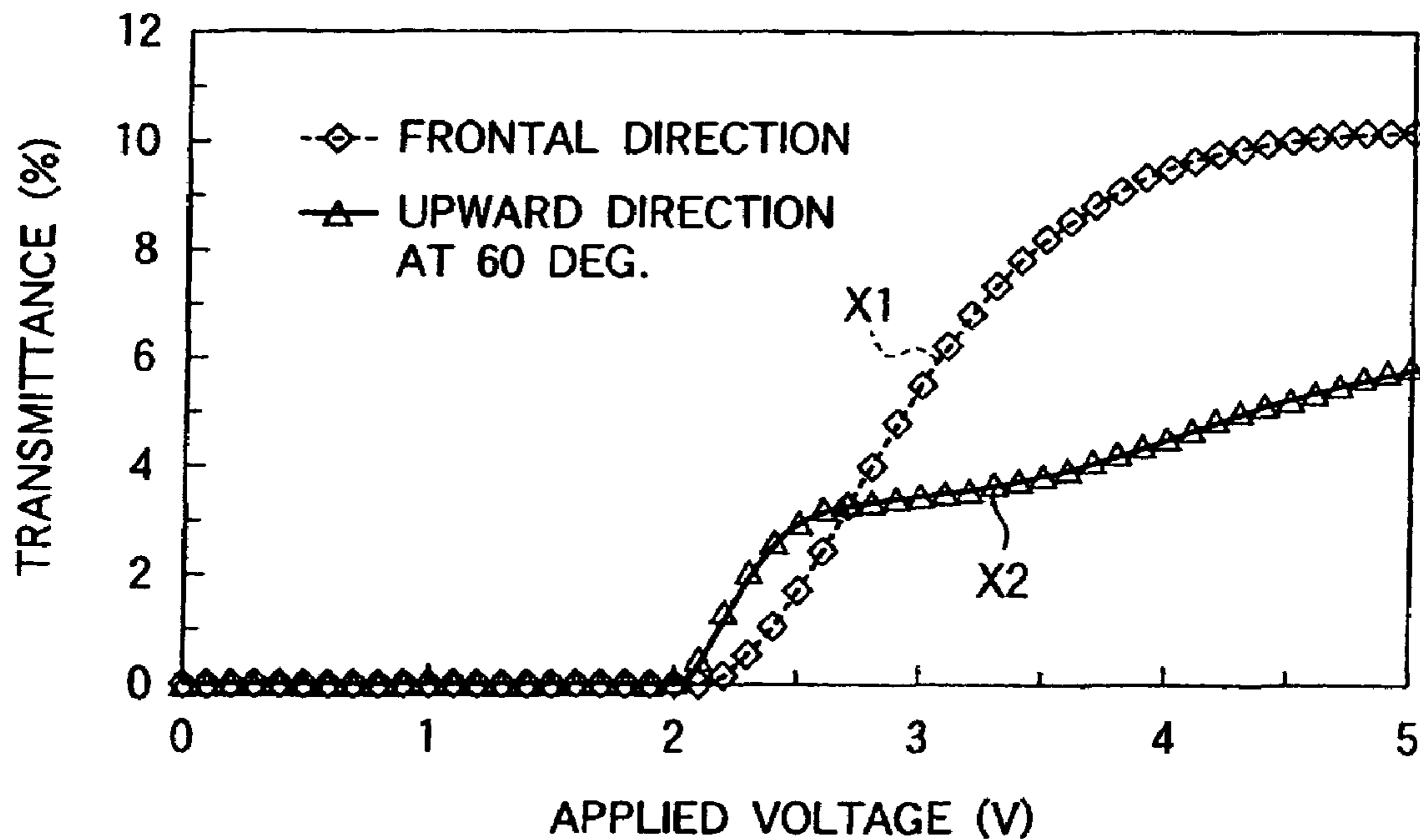
FIG.18 PRIOR ART
