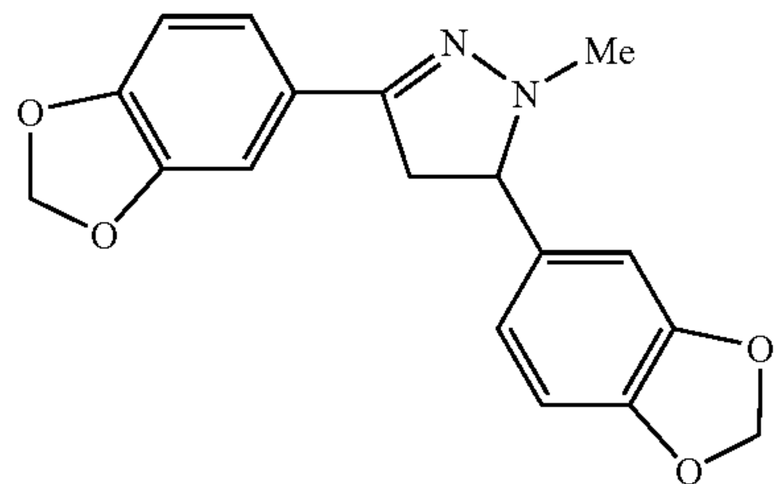
3,5-bis(3,4-methylenedioxyphenyl)-1-methyl-2-pyrazoline
