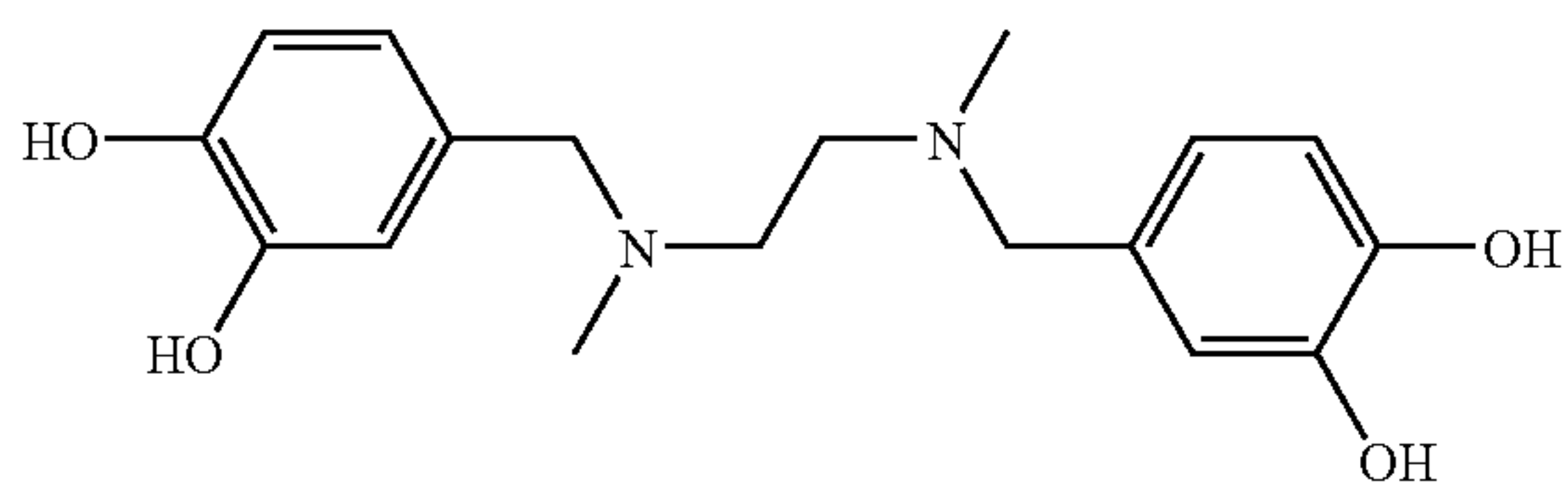
N,N'-bis(3,4-dihydroxybenzyl)-N,N'-dimethylethylenediamine
