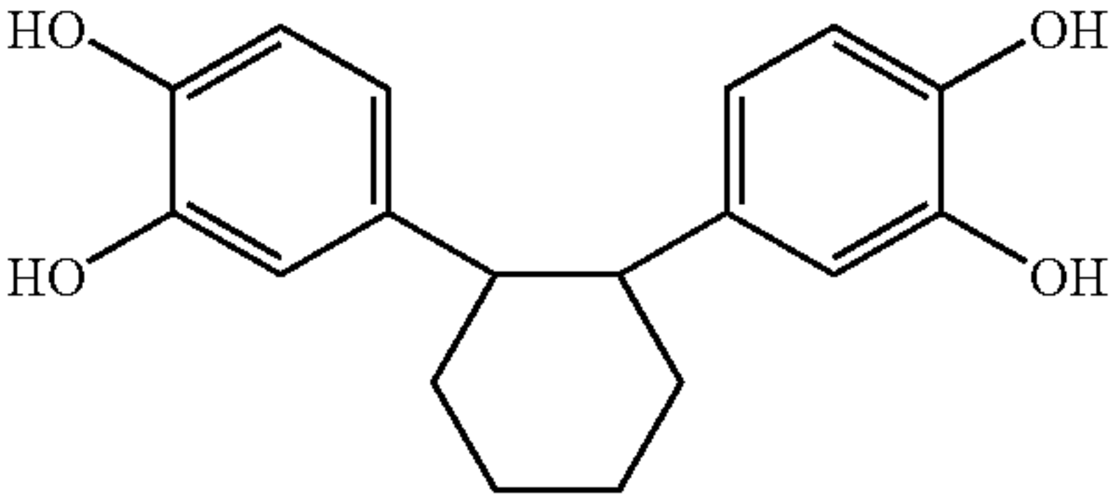
1,2-bis(3,4-dihydroxyphenyl)cyclohexane
