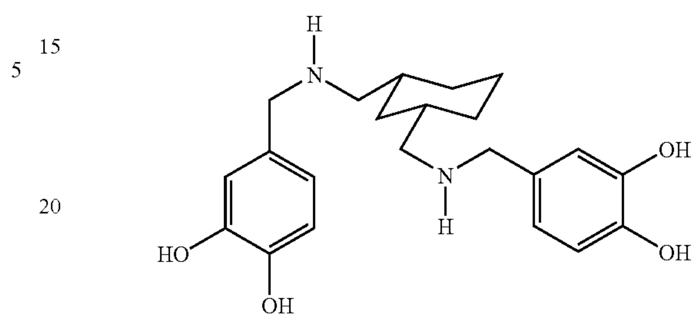
N,N'-bis(3,4-dihydroxybenzyl)-cis-1,3-bis-(aminomethyl)cyclohexane
