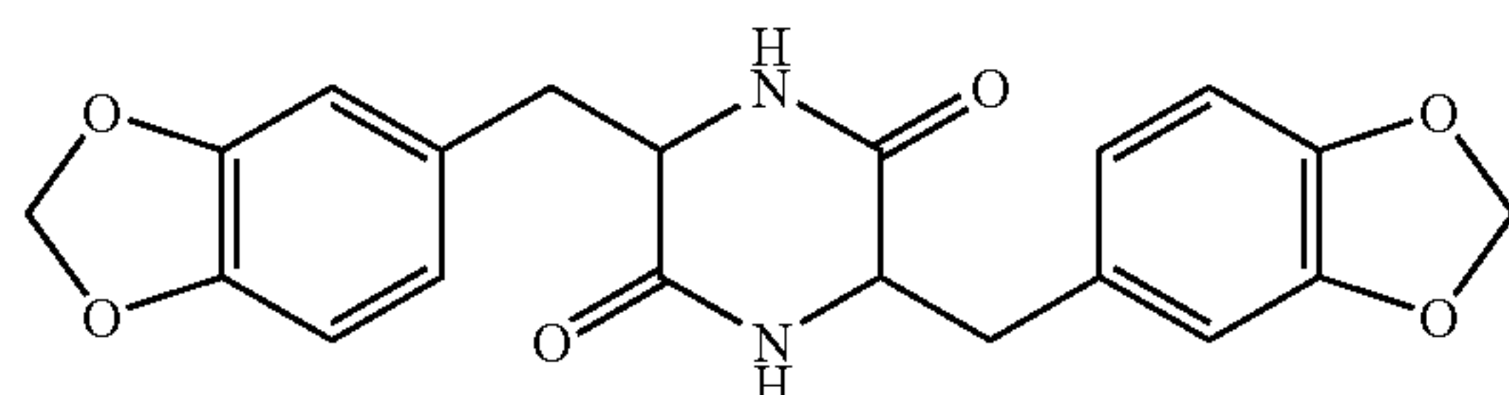
3,6-bis(3,4-methylenedioxybenzyl)-2,5-diketopiperazine
