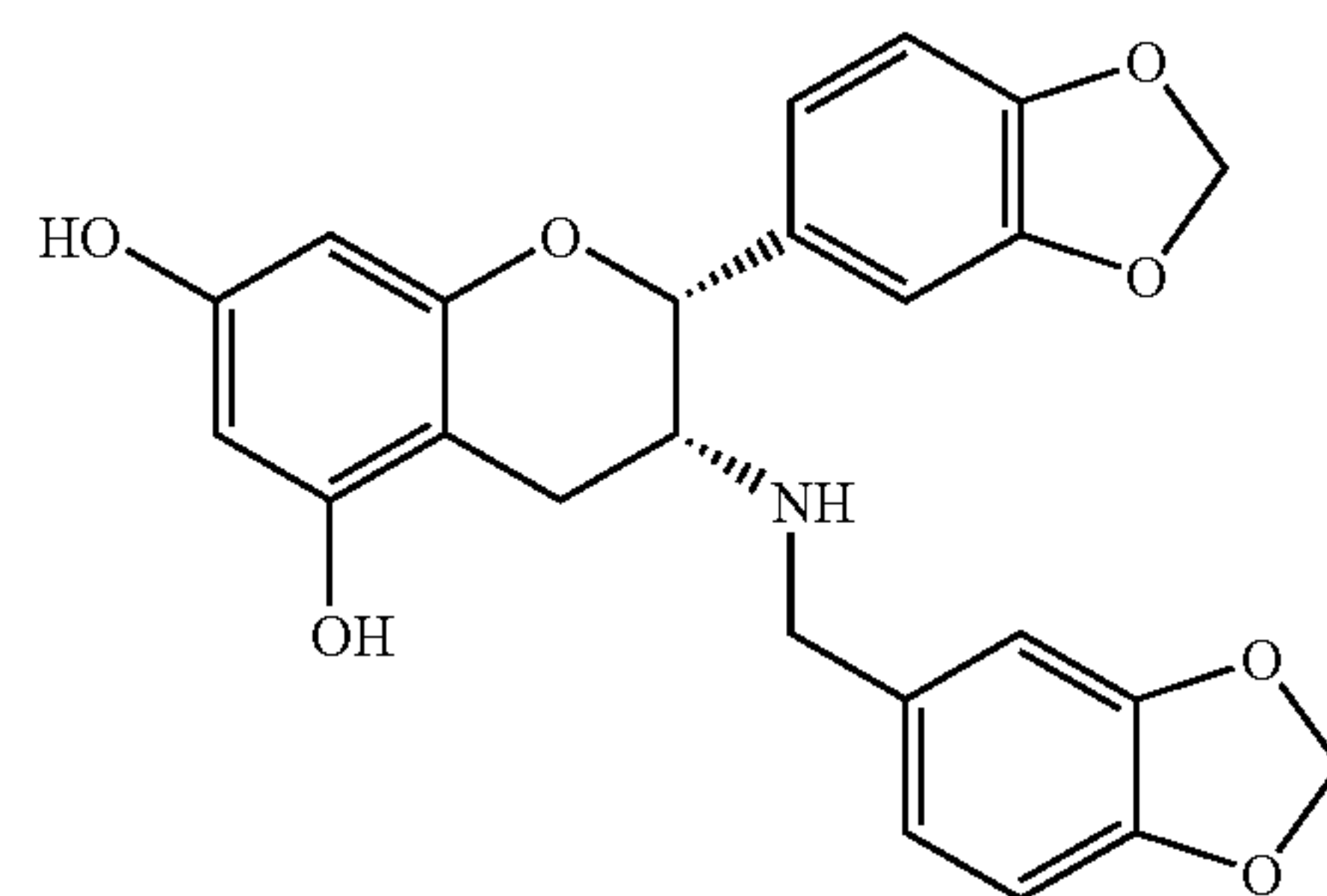
3-deoxy-3-(3,4-methylenedioxybenzyl)-aminoepicatechin
