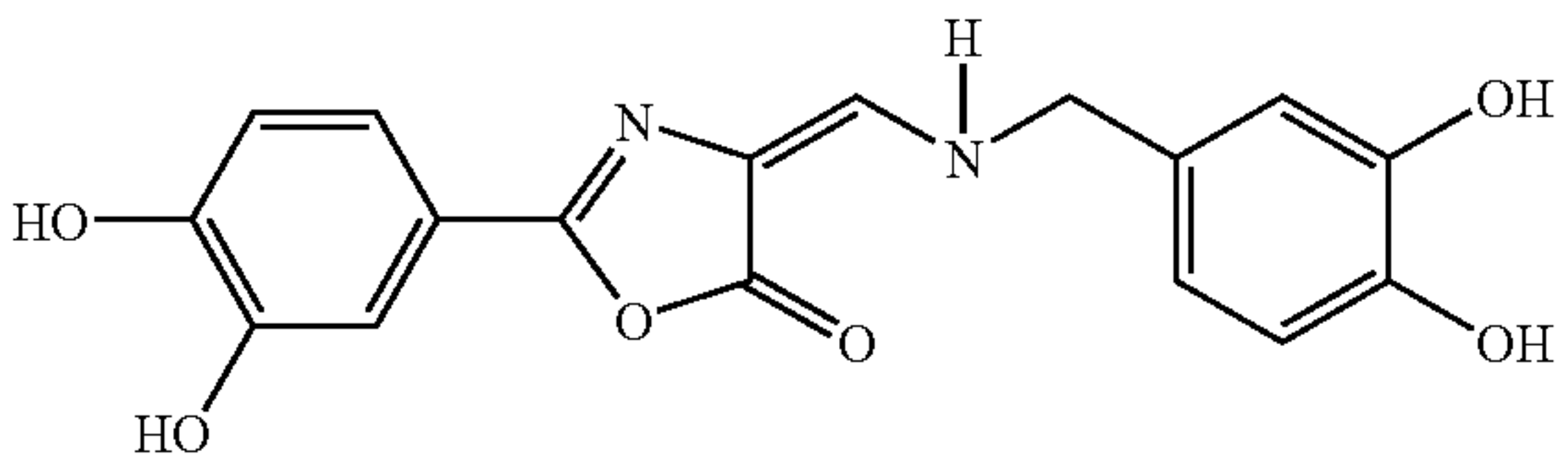
4-(3,4-dihydroxybenzylaminomethylene)-2-(3,4-dihydroxyphenyl)oxazolin-5-one
