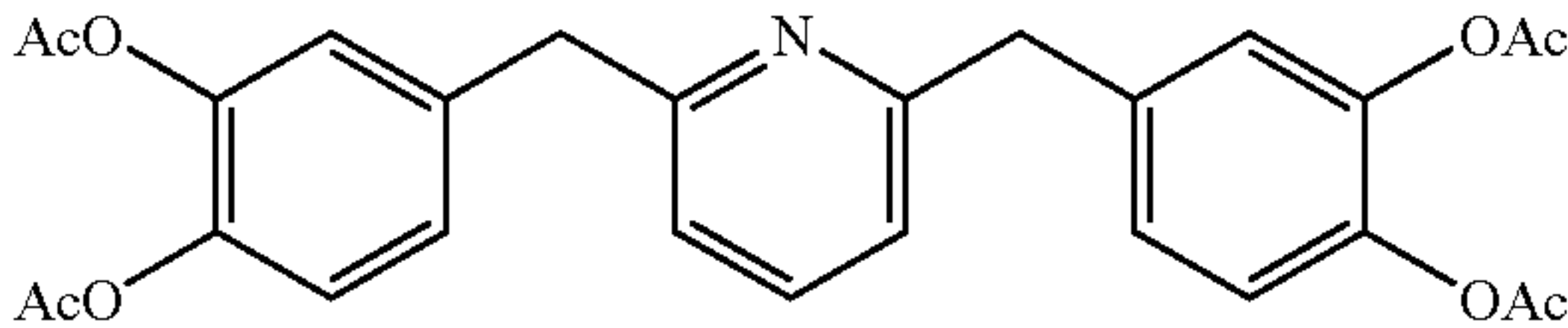
2,6-bis(3,4-diacetoxybenzyl)-pyridine
