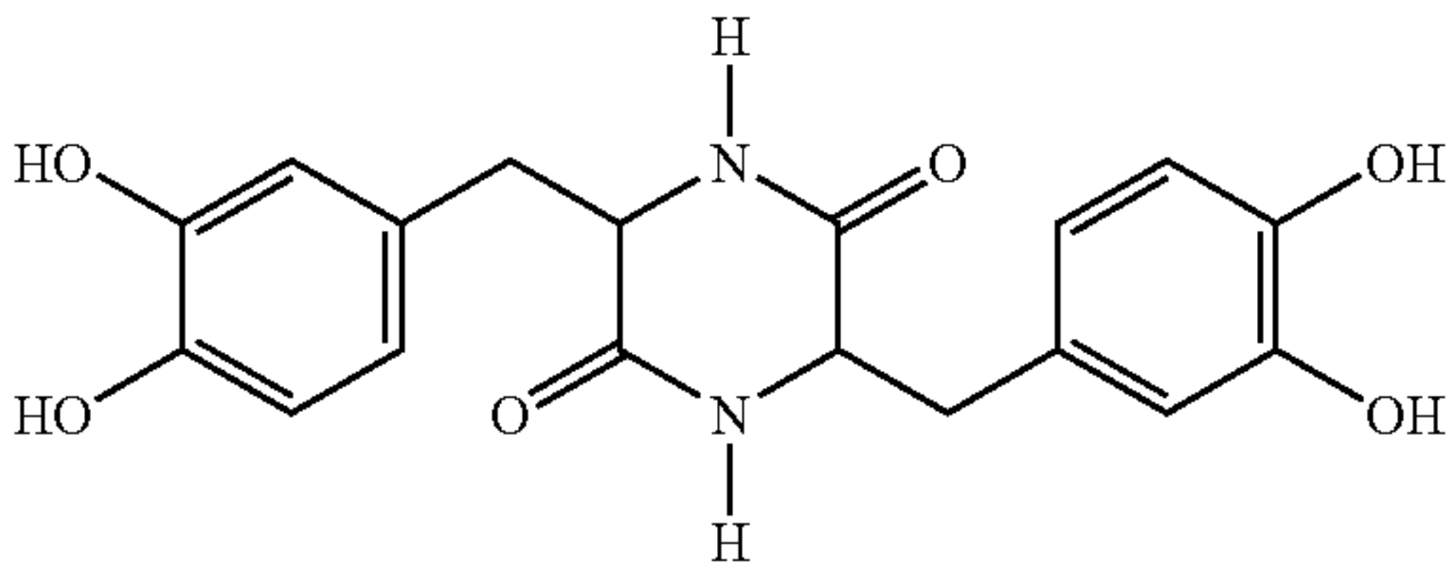
3,6-bis(3,4-dihydroxybenzyl)-2,5-diketopiperazine
