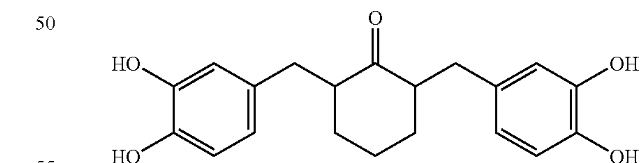
2,6-bis(3,4-dihydroxybenzyl)cyclohexanone
