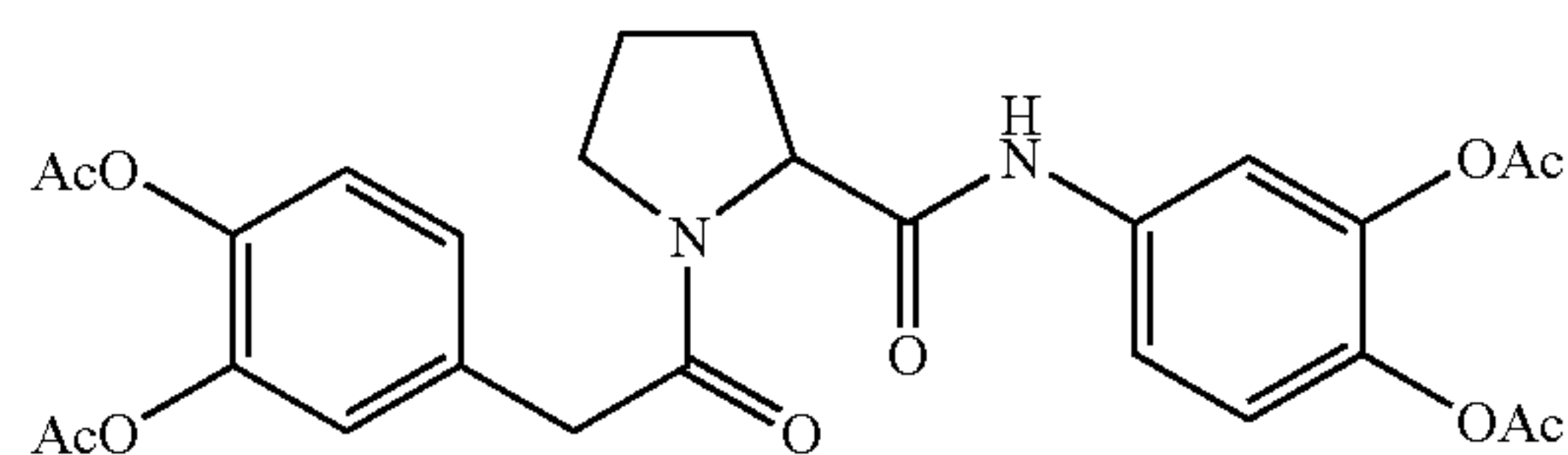
N-(3,4-diacetoxyphenylacetyl)-proline-3,4- diacetoxyanilide
