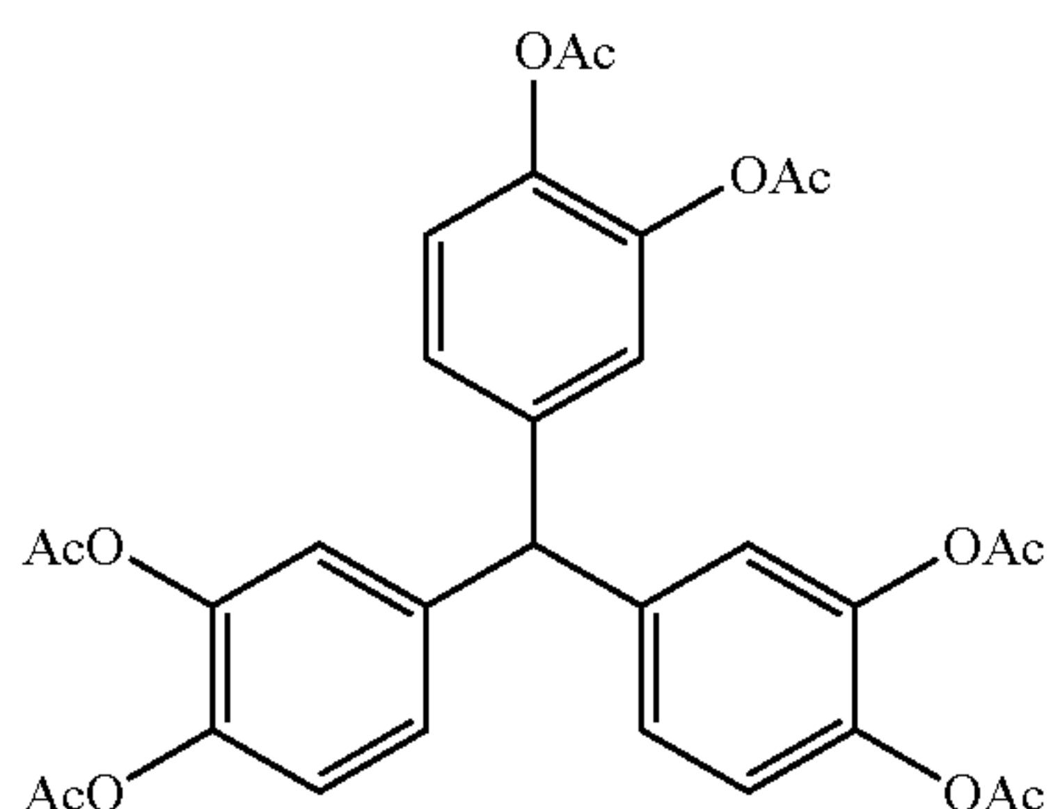
Tris-(3,4-diacetoxyphenyl)methane
