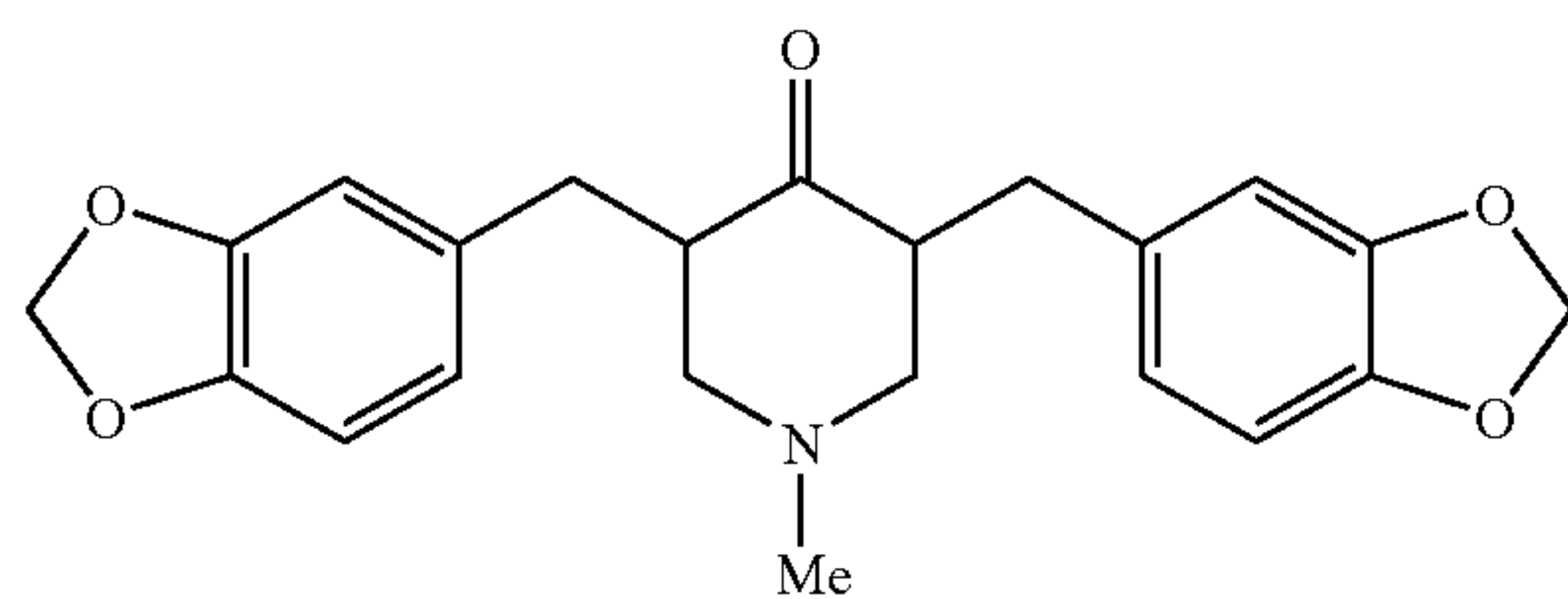
3,5-bis(3,4-methylenedioxybenzyl)-1-methyl-4-piperidinone
