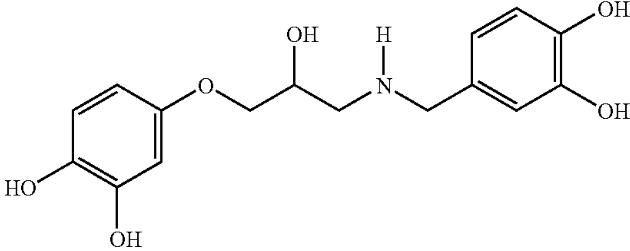
N-(3,4-dihydroxybenzyl)-3-(3,4-dihydroxyphenoxy)-2-hydroxypropylamine
