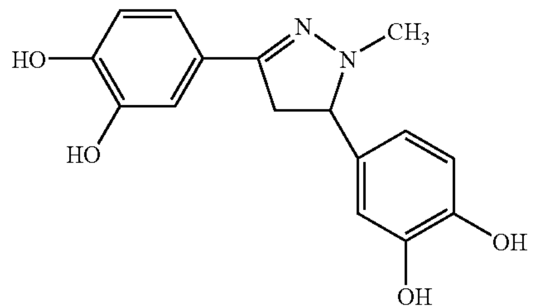
3,5-bis(3,4-dihydroxyphenyl)-1-methyl-2-pyrazoline
