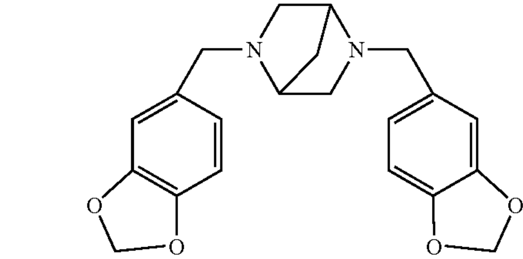
2,5-bis(3,4-methylenedioxybenzyl)-2,5-diaza[2,2,1]- bicycloheptane
