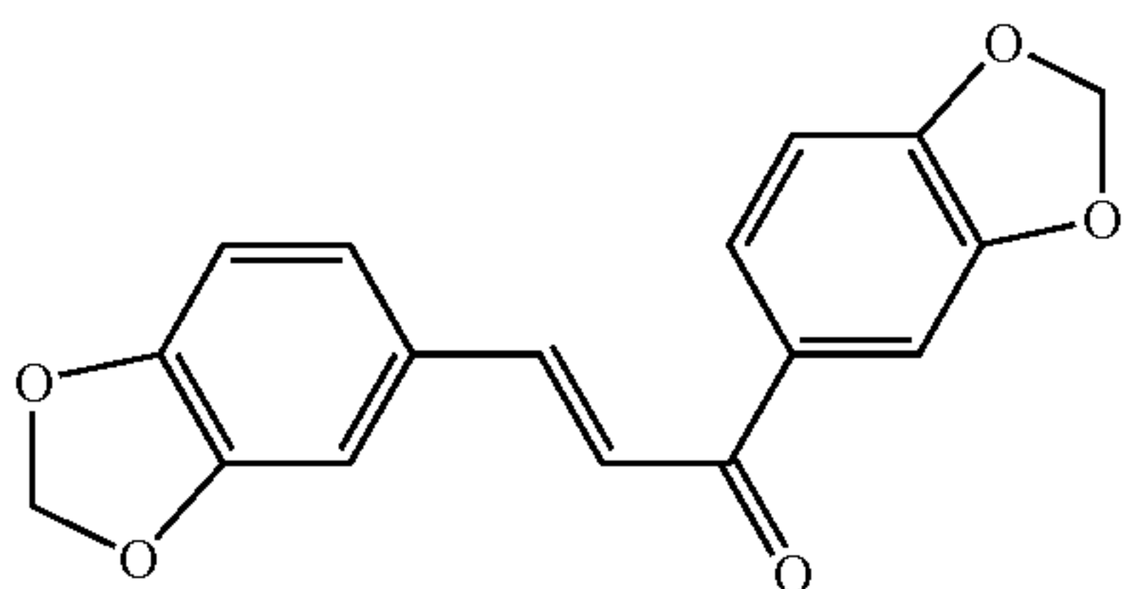
bis(3,4-methylenedioxy)chalcone
