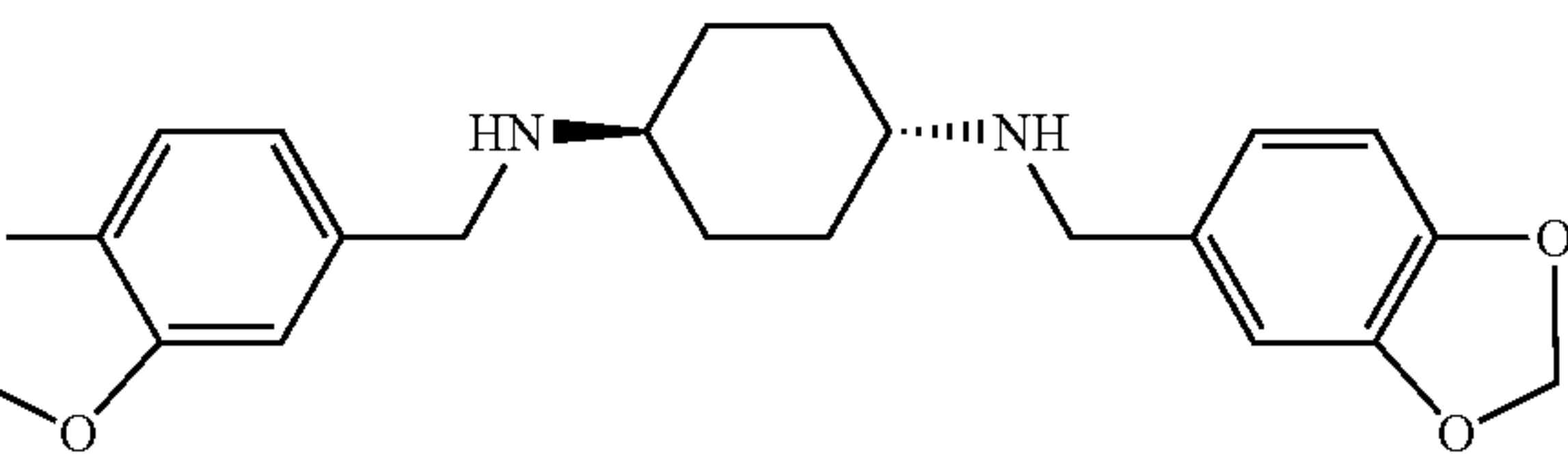
N,N'-bis(3,4-methylenedioxybenzyl)-trans-1,4- diaminocyclohexane
