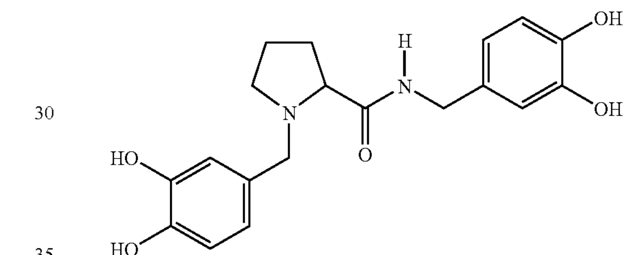
N-(3,4-dihydroxybenzyl)proline 3,4-dihydroxy-benzylamide
