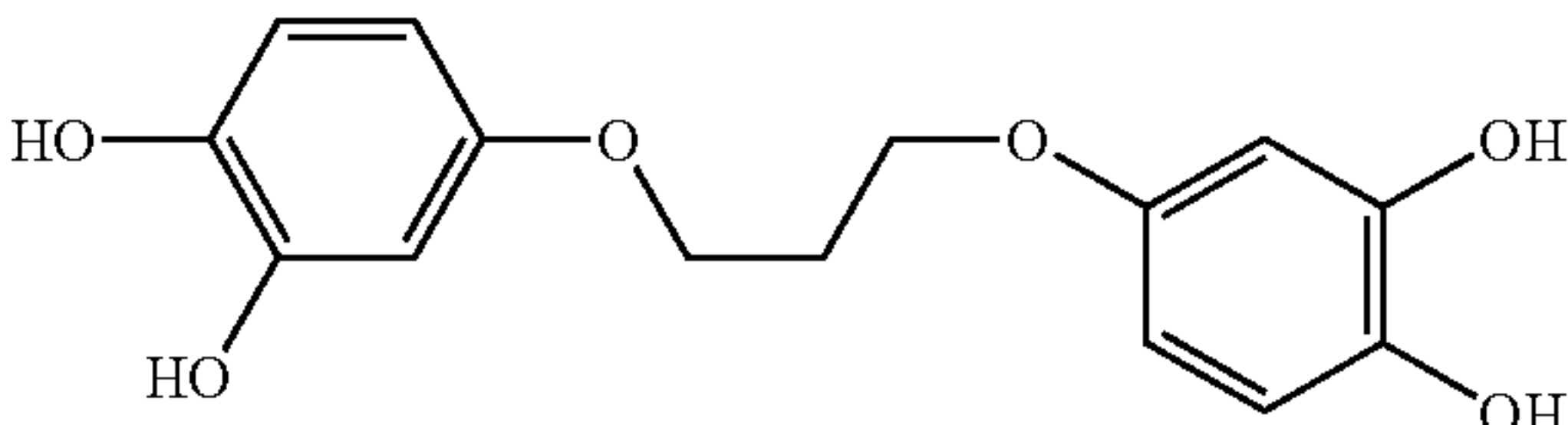
1,3-bis(3,4-dihydroxyphenoxy)propane
