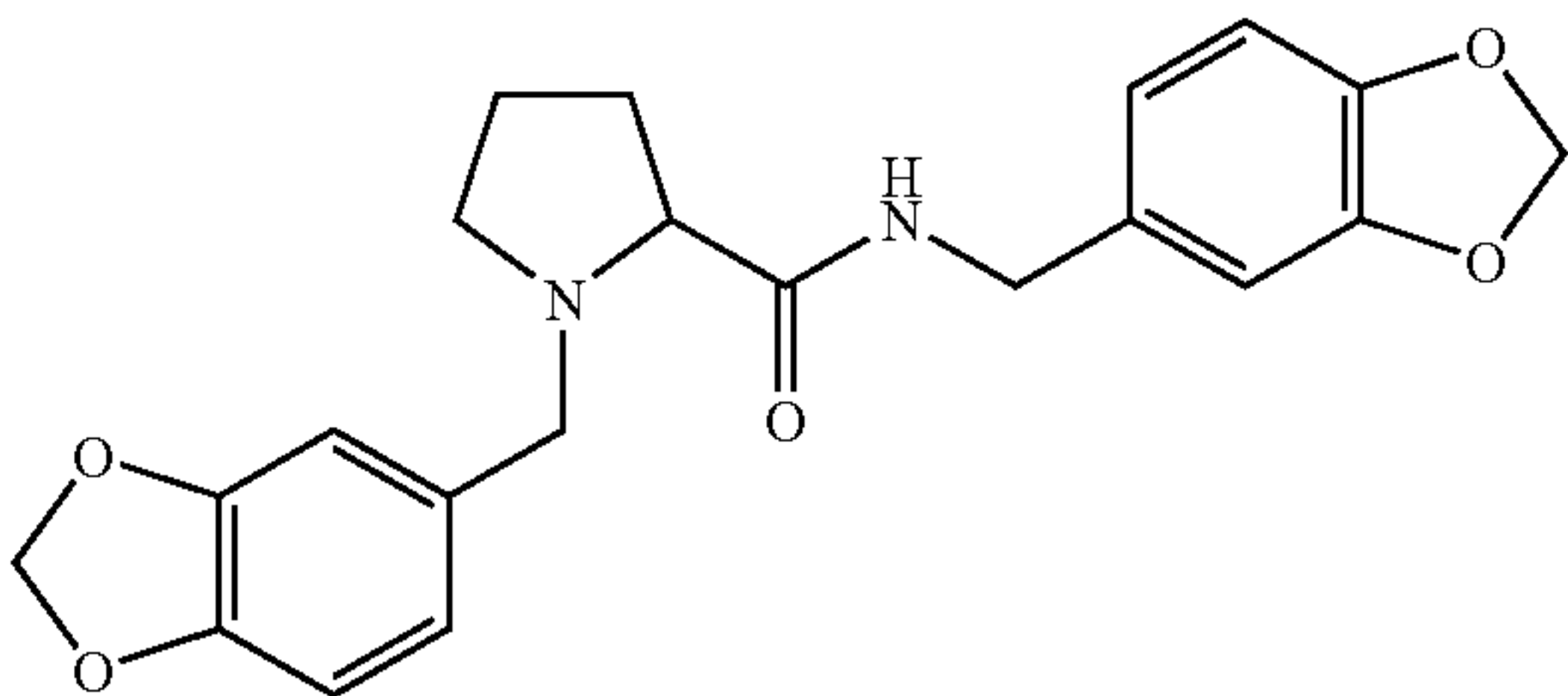
N-(3,4-methylenedioxybenzyl)proline 3,4- methylenedioxybenzylamide
