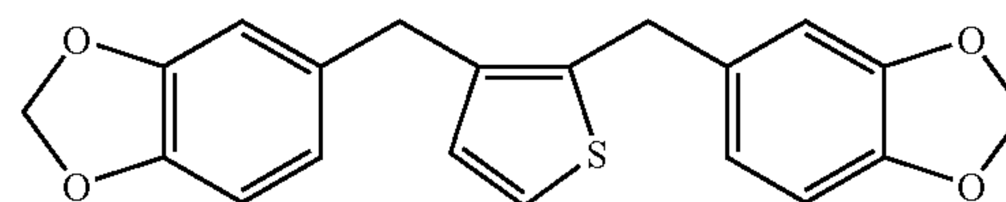
2,3-bis(3,4-methylenedioxybenzyl)-thiophene
