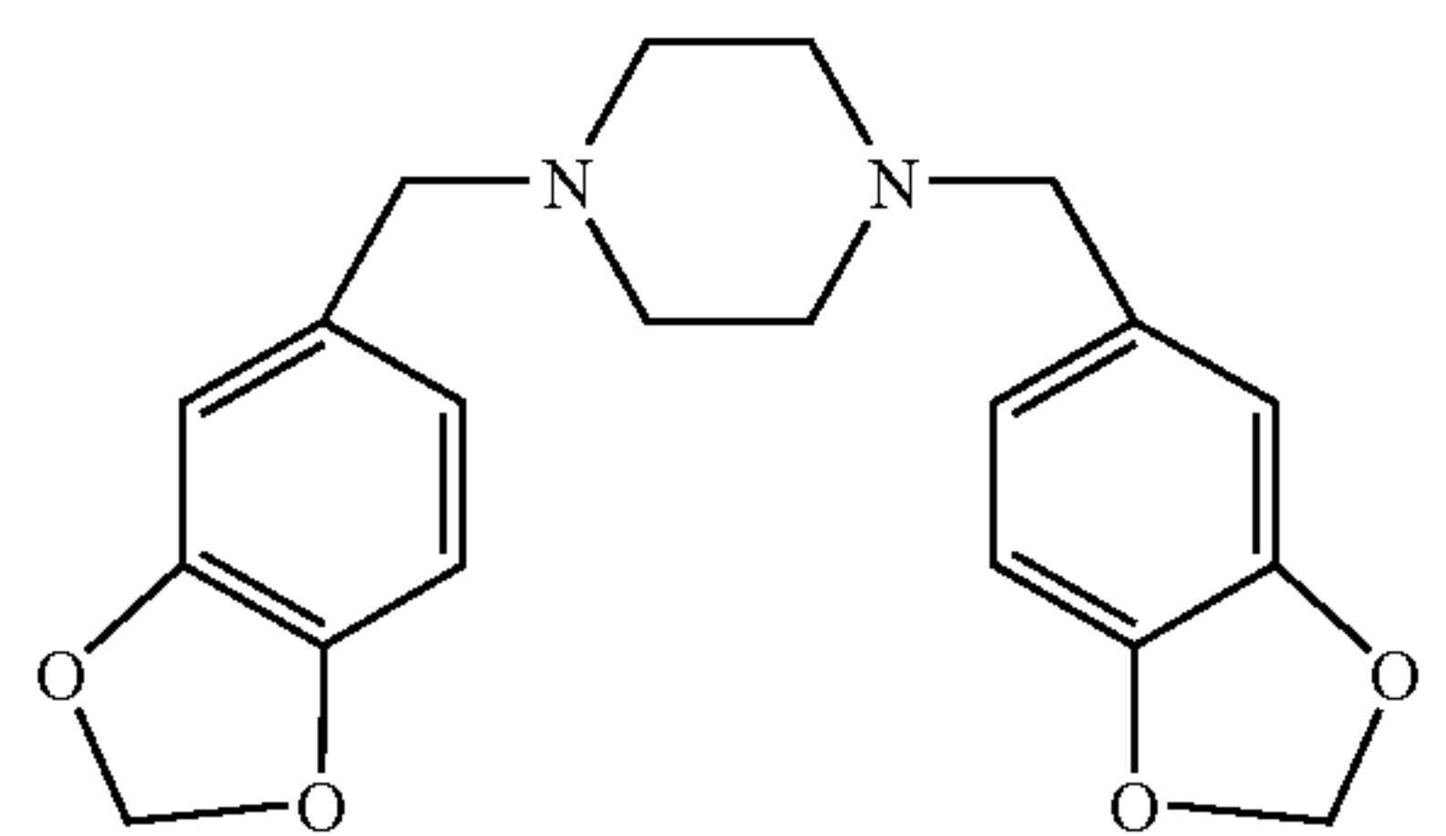
1,4-bis(3,4-methylenedioxybenzyl)piperazine
