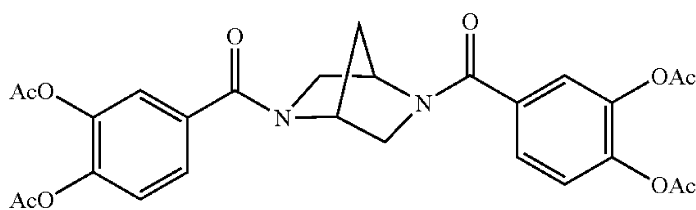
2,5-bis(3,4-diacetoxybenzoyl)-2,5-diaza[2,2,1]- bicycloheptane
