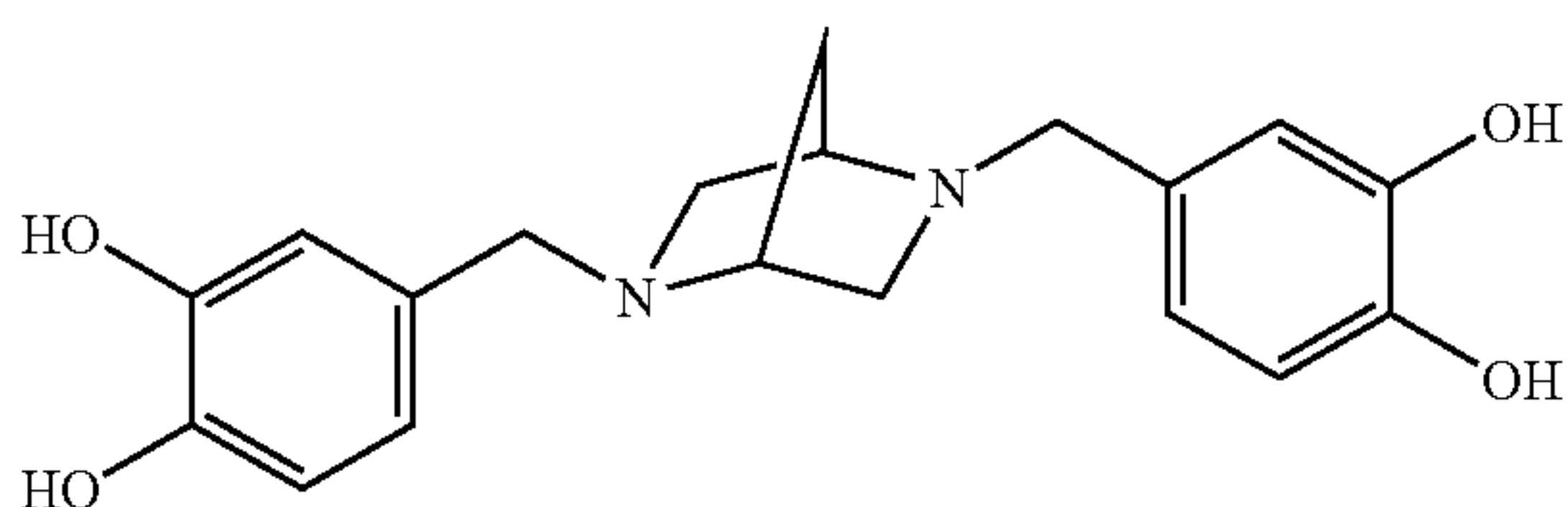
2,5-bis(3,4-dihydroxybenzyl)-2,5-diaza-[2.2.1]-bicycloheptane
