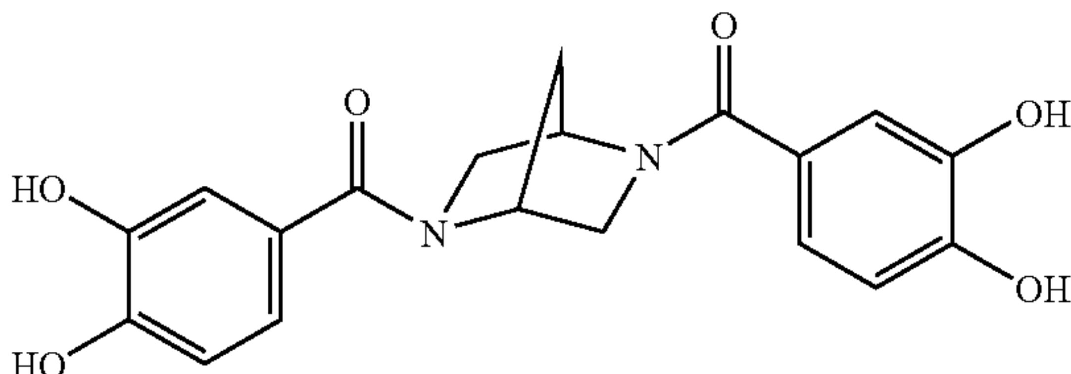
2,5-bis(3,4-dihydroxybenzoyl)-2,5-diaza-[2.2.1]-bicycloheptane
