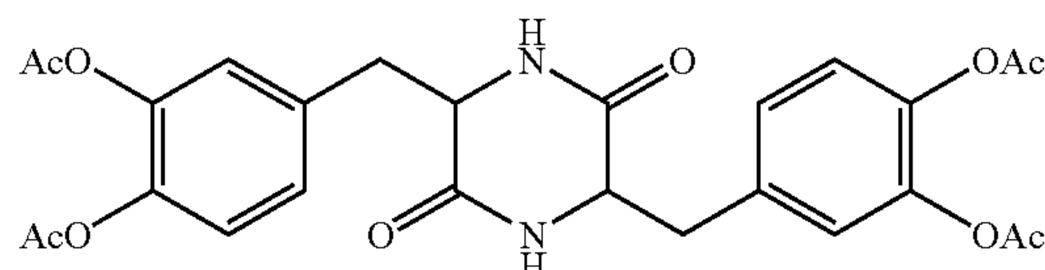
3,6-bis(3,4-diacetoxybenzyl)-2,5- diketopiperazine
