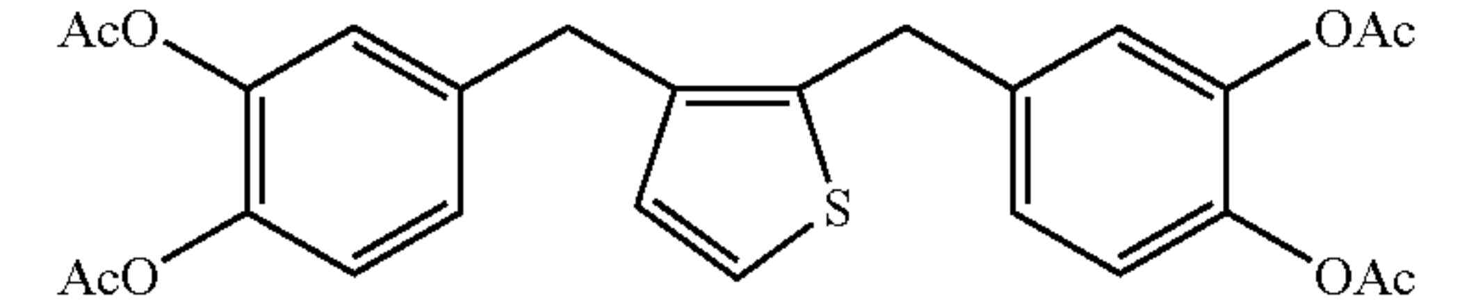
2,3-bis(3,4-diacetoxybenzyl)-thiophene
