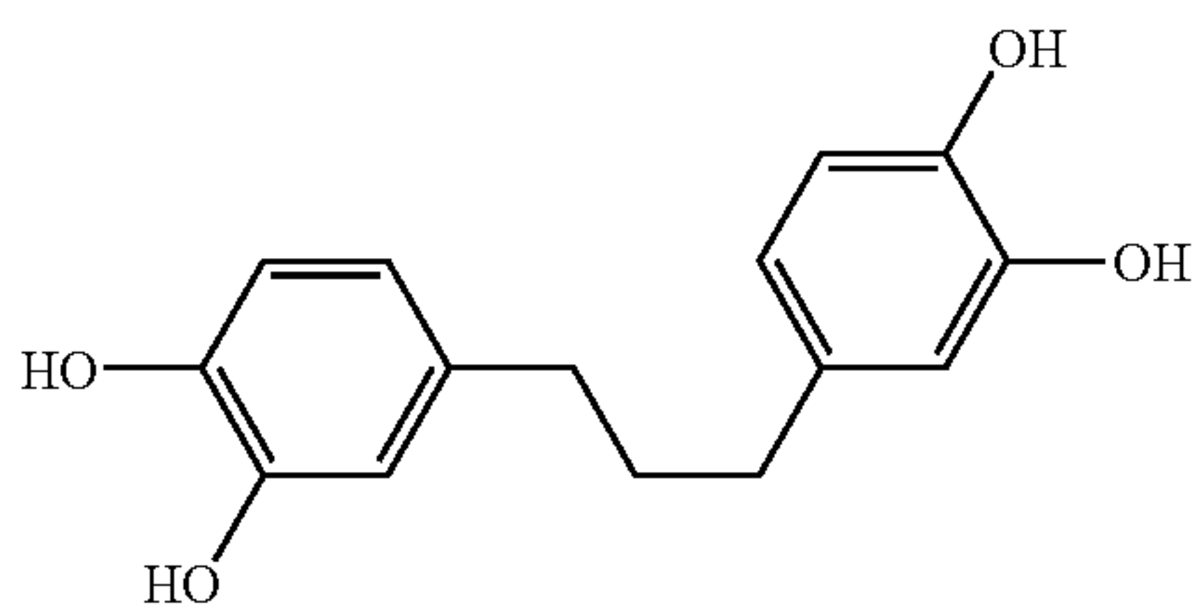
1,3-bis(3,4-dihydroxyphenyl)propane
