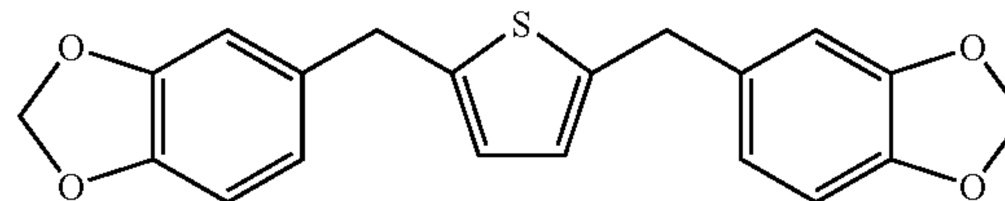
2,5-bis(3,4-methylenedioxybenzyl)-thiophene
