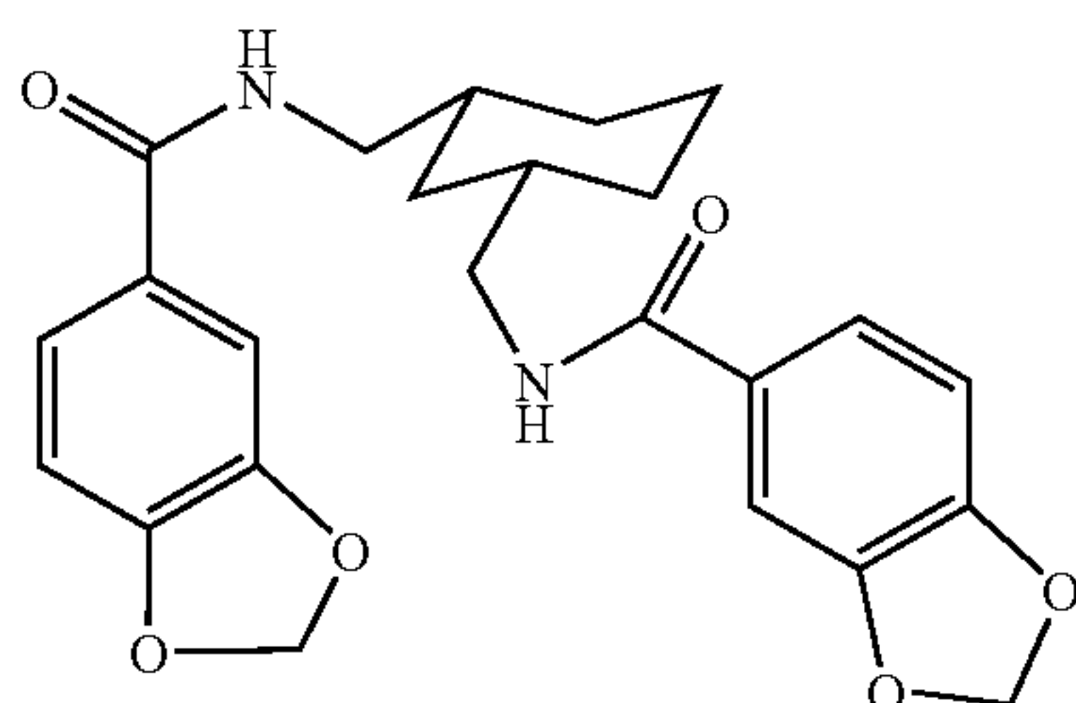
N,N'-bis(3,4-methylenedioxybenzoyl)-cis-1,3-bis-(aminomethyl)cyclohexane
