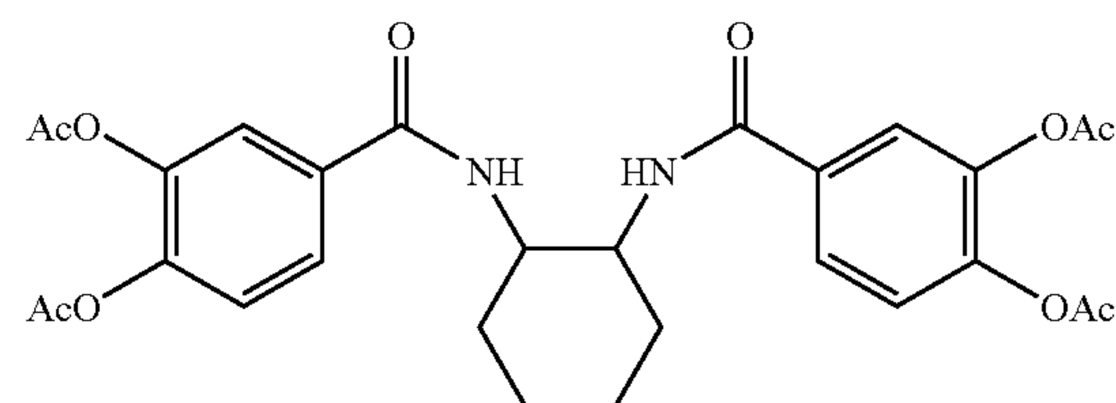
N,N'-bis(3,4-diacetoxybenzoyl)-trans- diaminocyclohexane
