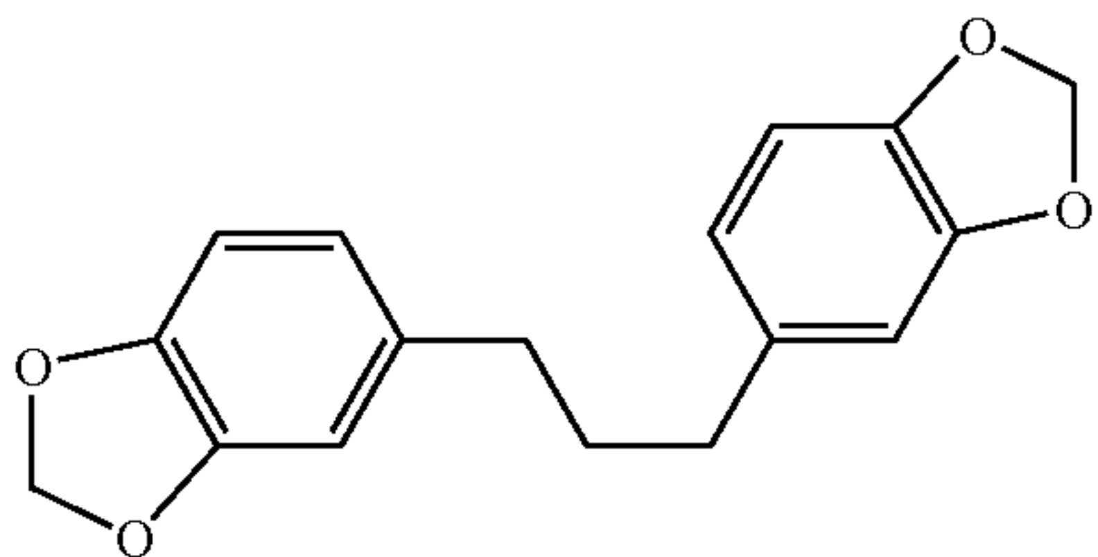
1,3-bis(3,4-methylenedioxyphenyl)propane
