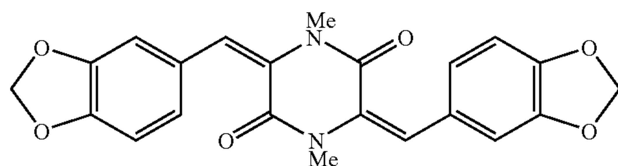
3,6-bis(3,4-methylenedioxybenzylidene)-1,4-dimethyl-2,5-diketopiperazine
