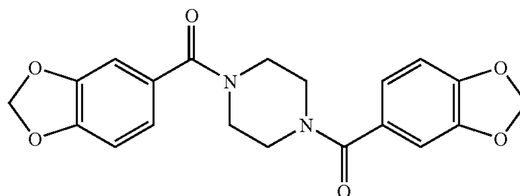
1,4-bis(3,4-methylenedioxybenzoyl)-piperazine
