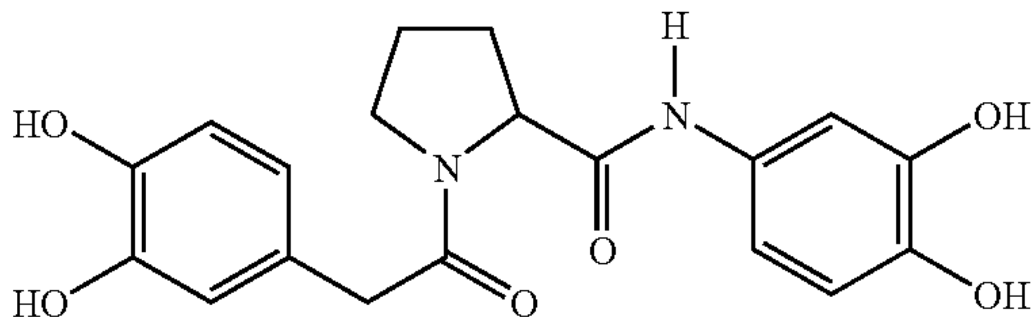
N-(3,4-hydroxyphenylacetyl)proline-3,4-di-hydroxyanilide
