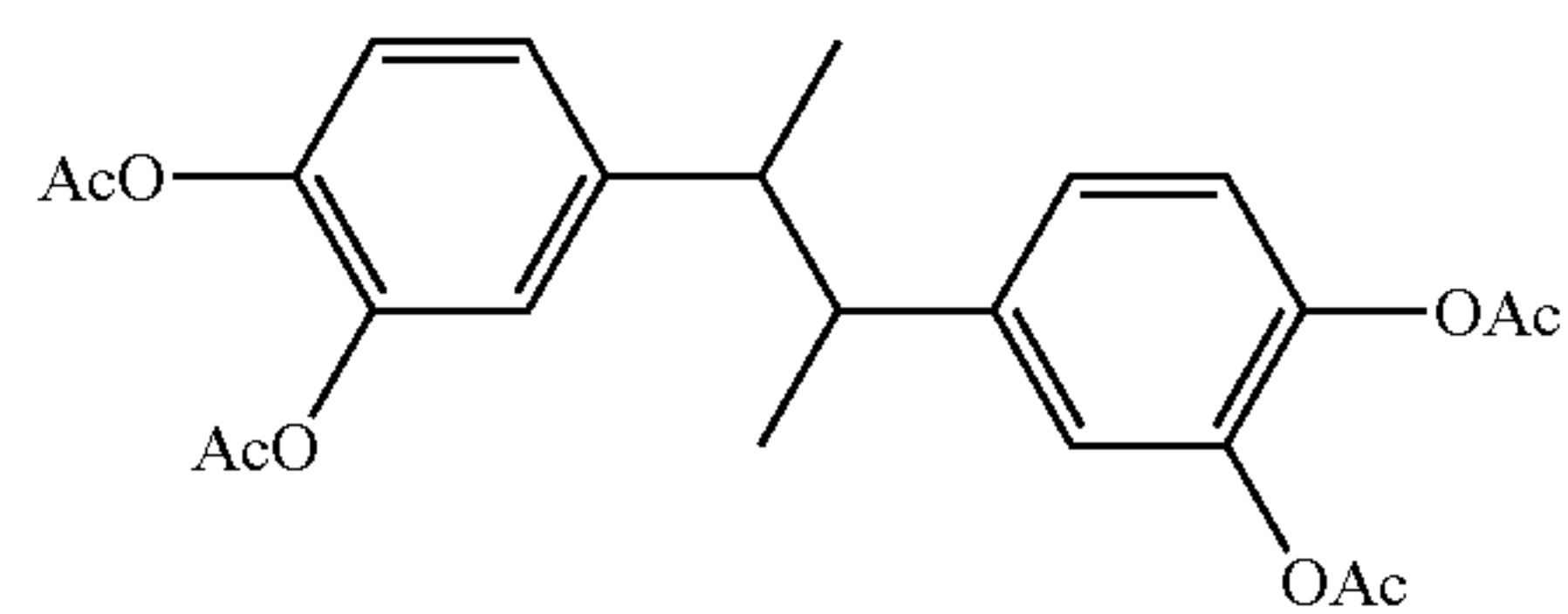
2,3-bis(3,4-diacetoxyphenyl)-butane
