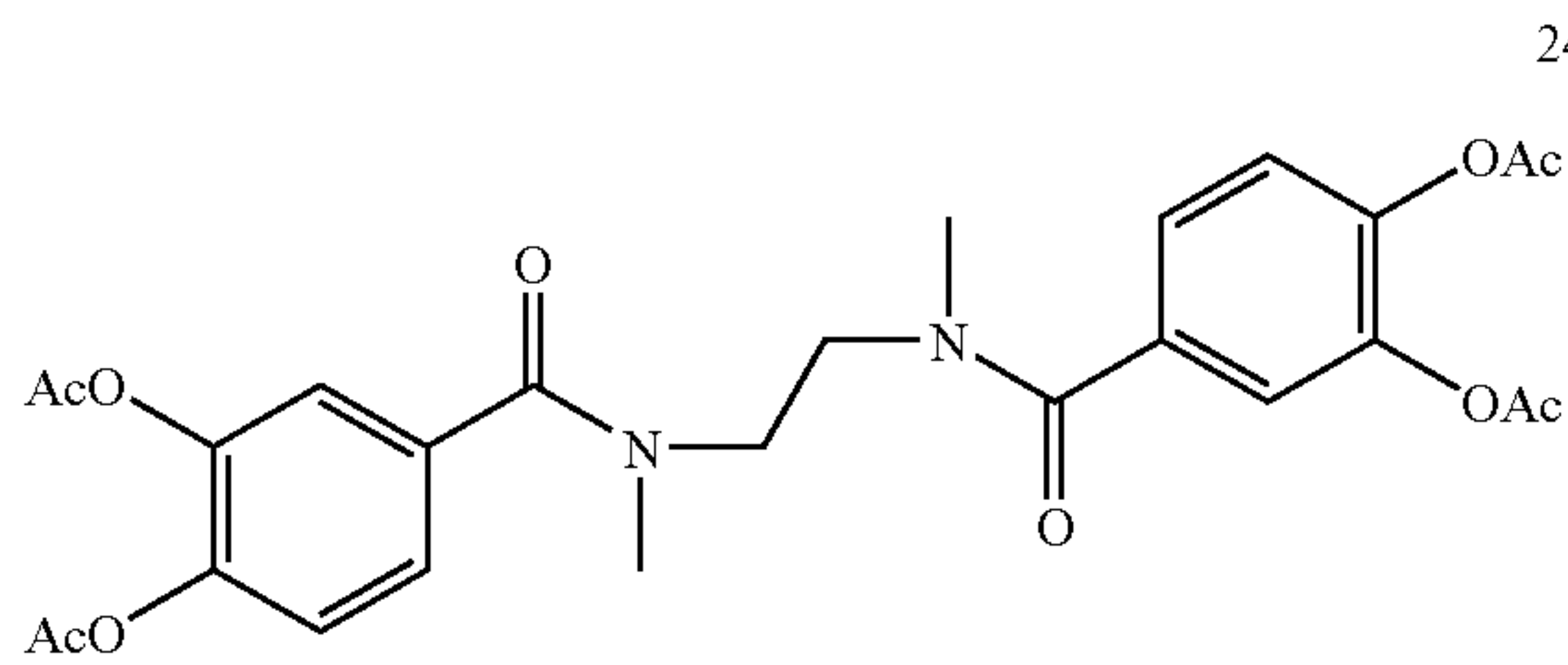
N,N'-bis(3,4-diacetoxybenzoyl)-N,N'-dimethyl(-) ethylenediamine
