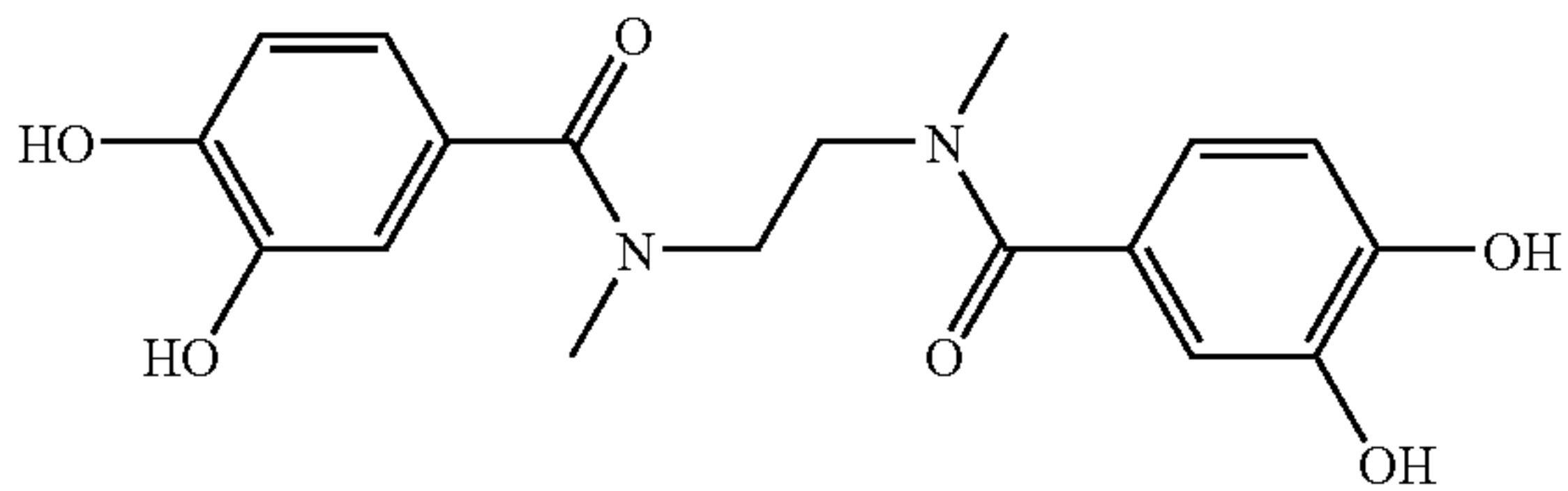
N,N'-bis(3,4-dihydroxybenzoyl)-N,N'-dimethylethylenediamine
