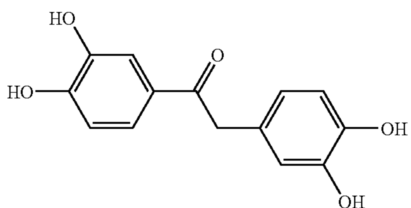
3,4,3',4'-Tetrahydroxydesoxybenzoin
