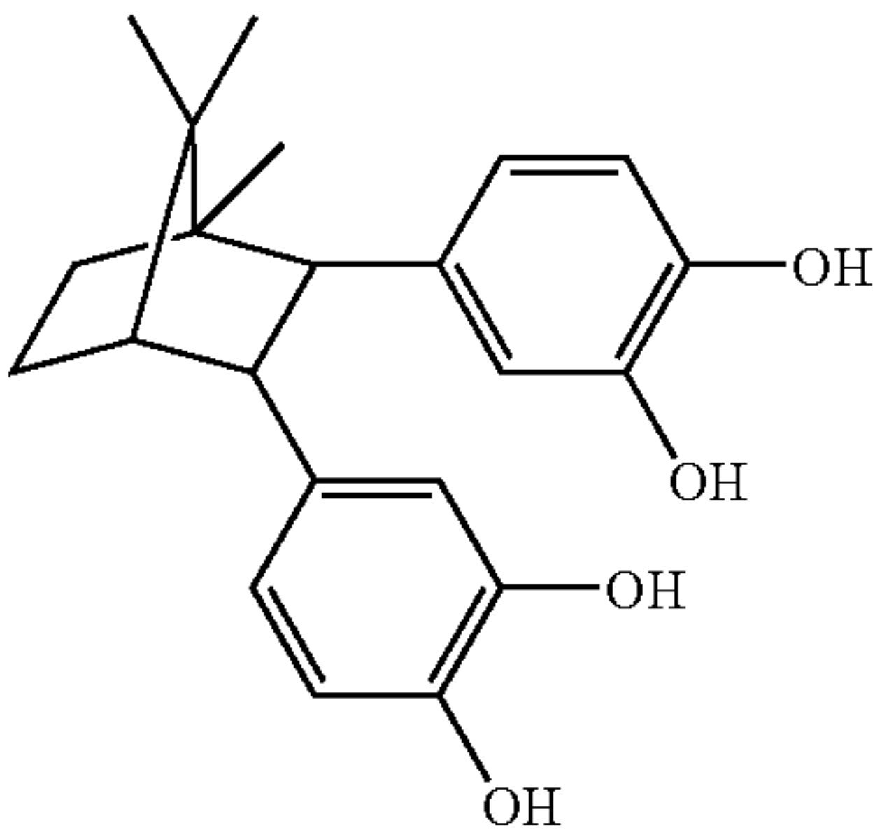
2,3-bis(3,4-dihydroxyphenyl)-1,7,7-trimethylbicyclo[2.2.1]heptane
