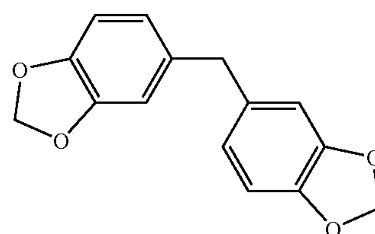
1,1-bis(3,4-methylenedioxyphenyl)methane
