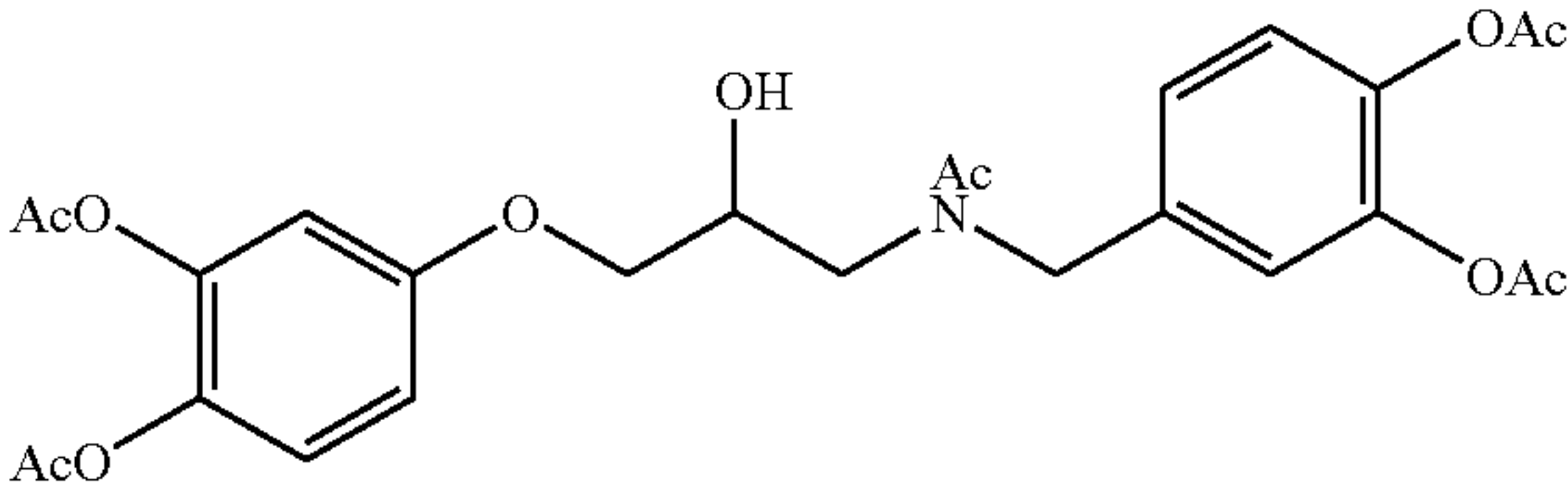
N-acetyl-N-(3,4-diacetoxybenzyl)-3-(3,4-diacetoxy(-) phenoxy)-2-hydroxypropylamine
