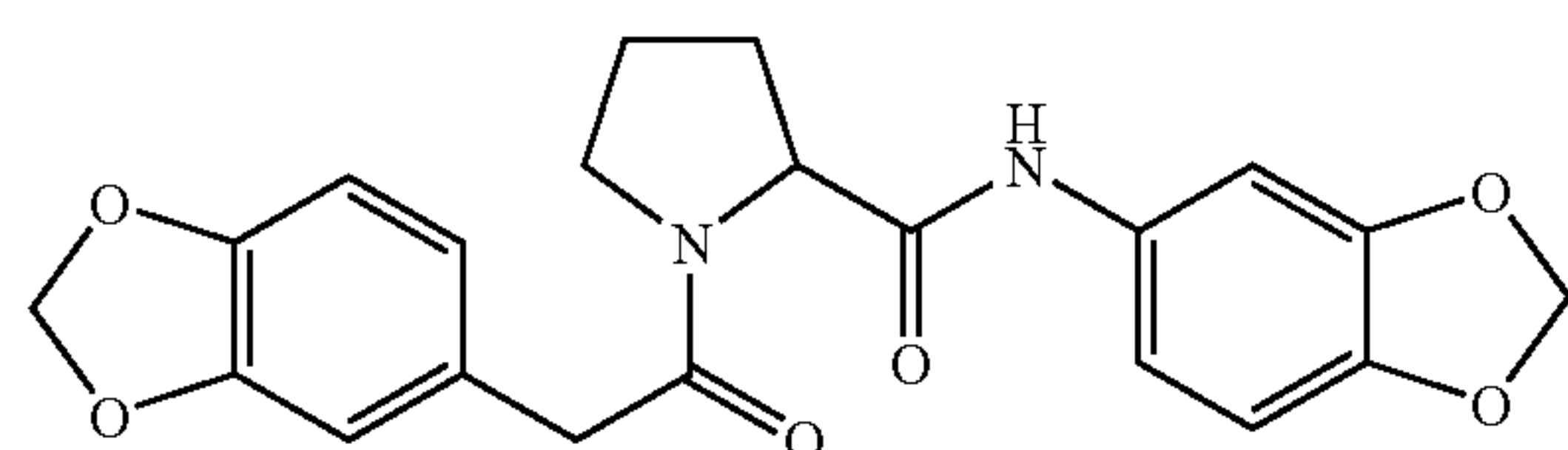
N-(3,4-methylenedioxyphenylacetyl)-proline-3,4-methylenedioxyanilide
