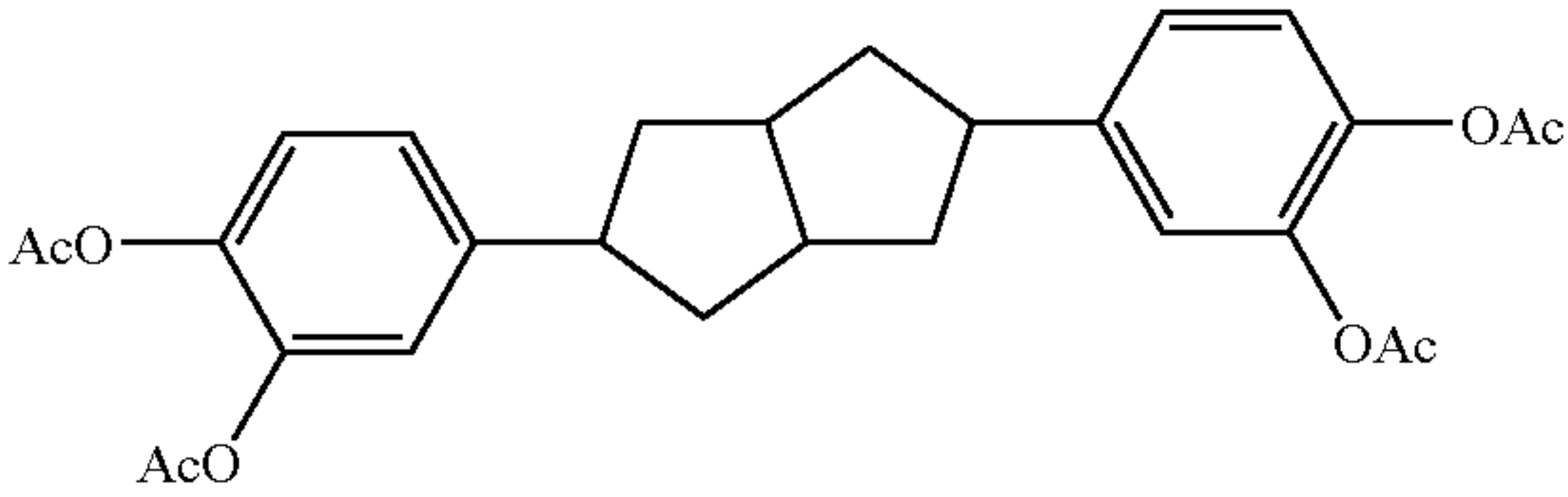
3,7-bis(3,4-diacetoxyphenyl)-bicyclo[3,3,0] (-)octane
