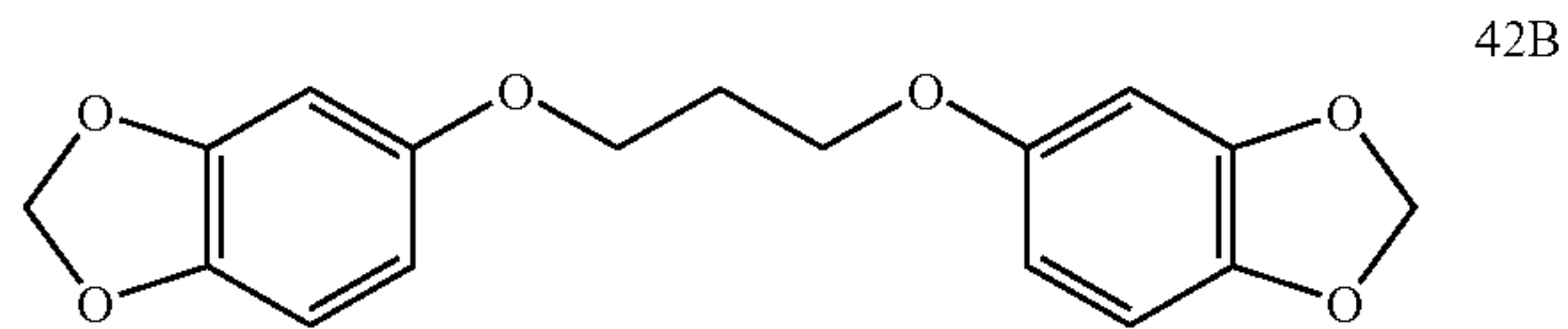
1,3-bis(3,4-methylenedioxyphenoxy)-propane
