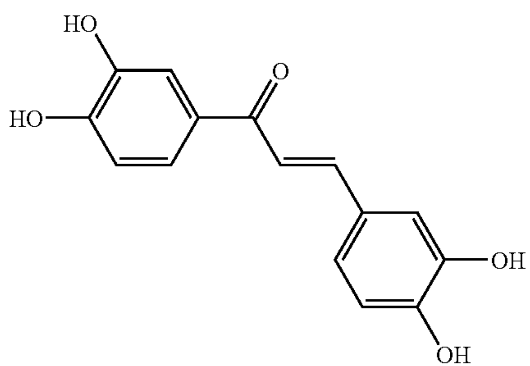
3,4,3',4'-Tetrahydroxychalcone
