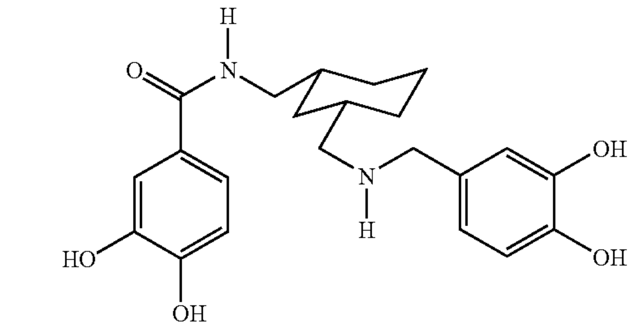
N,N'-bis(3,4-dihydroxybenzoyl)-cis-1,3-bis-(aminomethyl)cyclohexane
