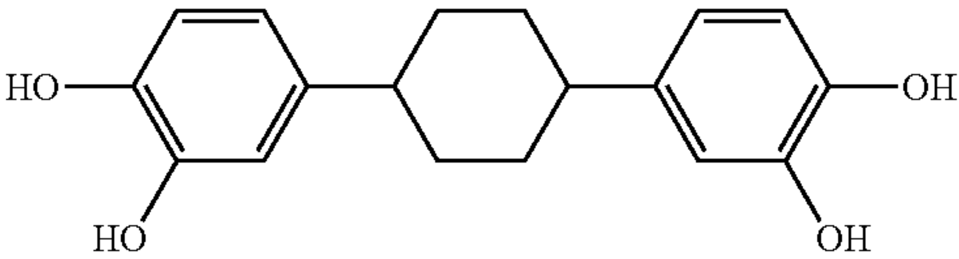
1,4-bis(3,4-dihydroxyphenyl)cyclohexane
