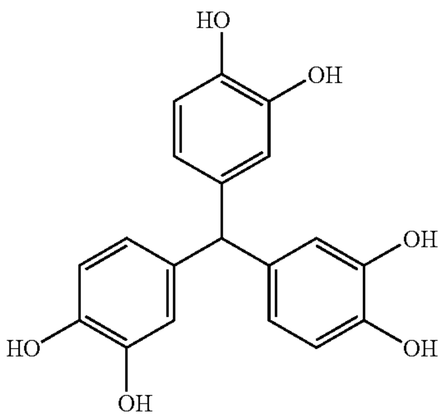
Tris-(3,4-dihydroxybenzyl)methane
