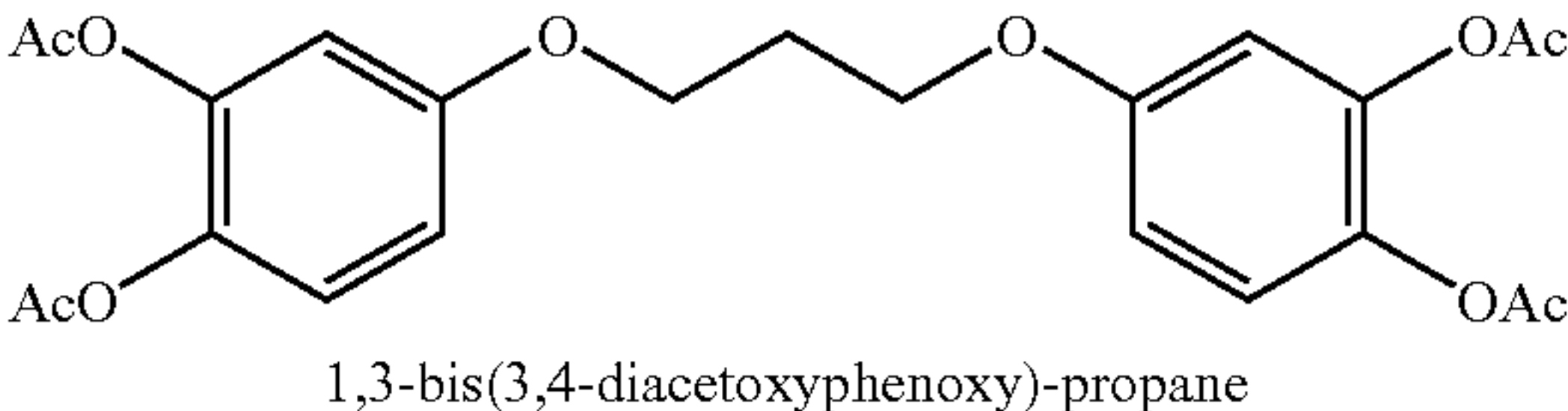
1,3-bis(3,4-diacetoxyphenoxy)-propane
