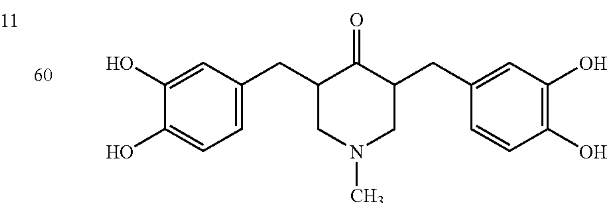
3,5-bis(3,4-dihydroxybenzyl)-1-methyl-4-piperidinone
