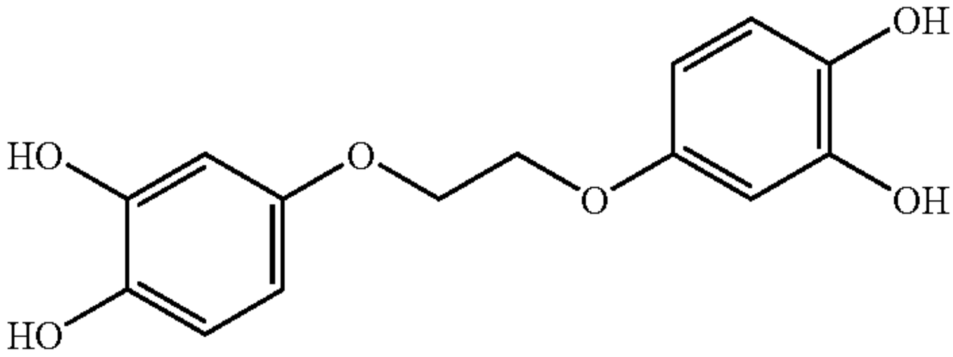
1,2-bis(3,4-dihydroxyphenoxy)ethane
