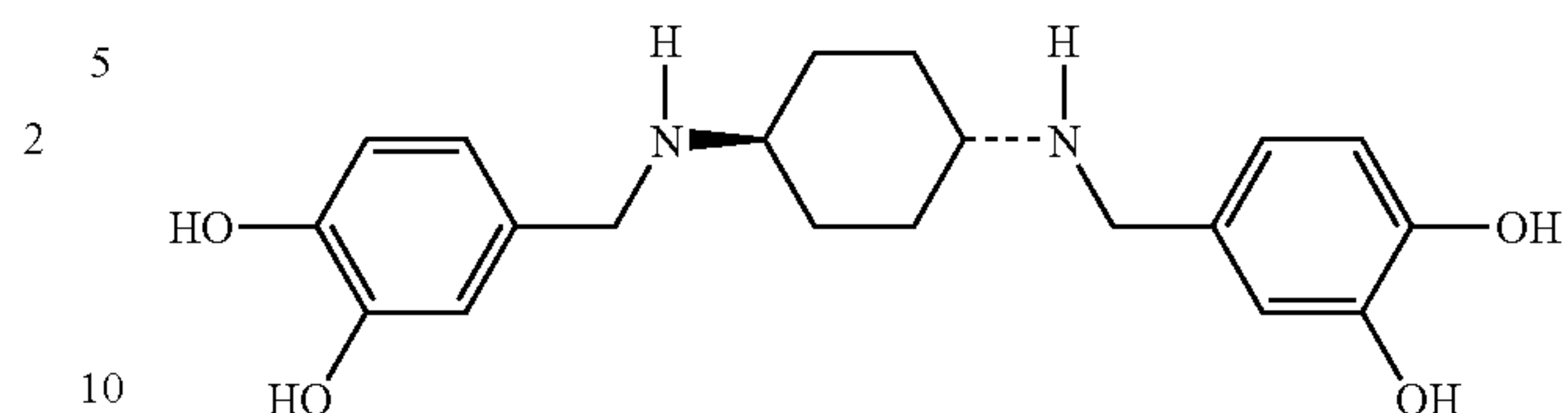
N,N'-bis(3,4-dihydroxybenzyl)-trans-1,4-diaminocyclohexane
