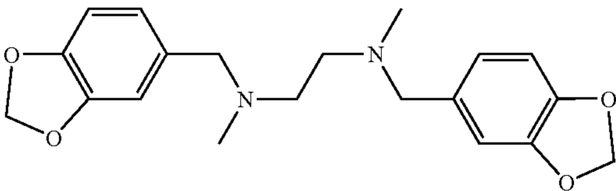
N,N'-bis(3,4-methylenedioxybenzyl)- N,N'-dimethyl-ethylenediamine
