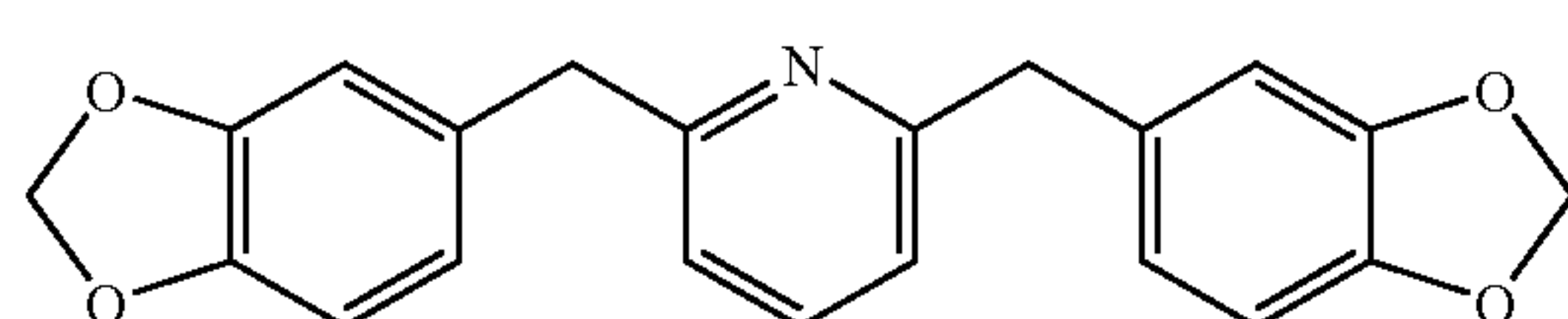
2,6-bis(3,4-methylenedioxybenzyl)-pyridine
