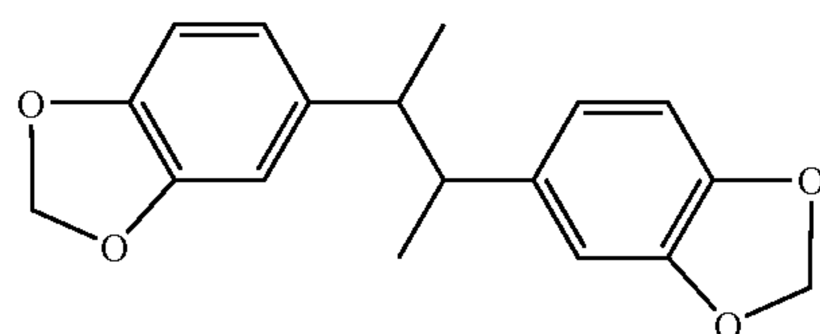
2,3-bis(3,4-methylenedioxyphenyl)-butane
