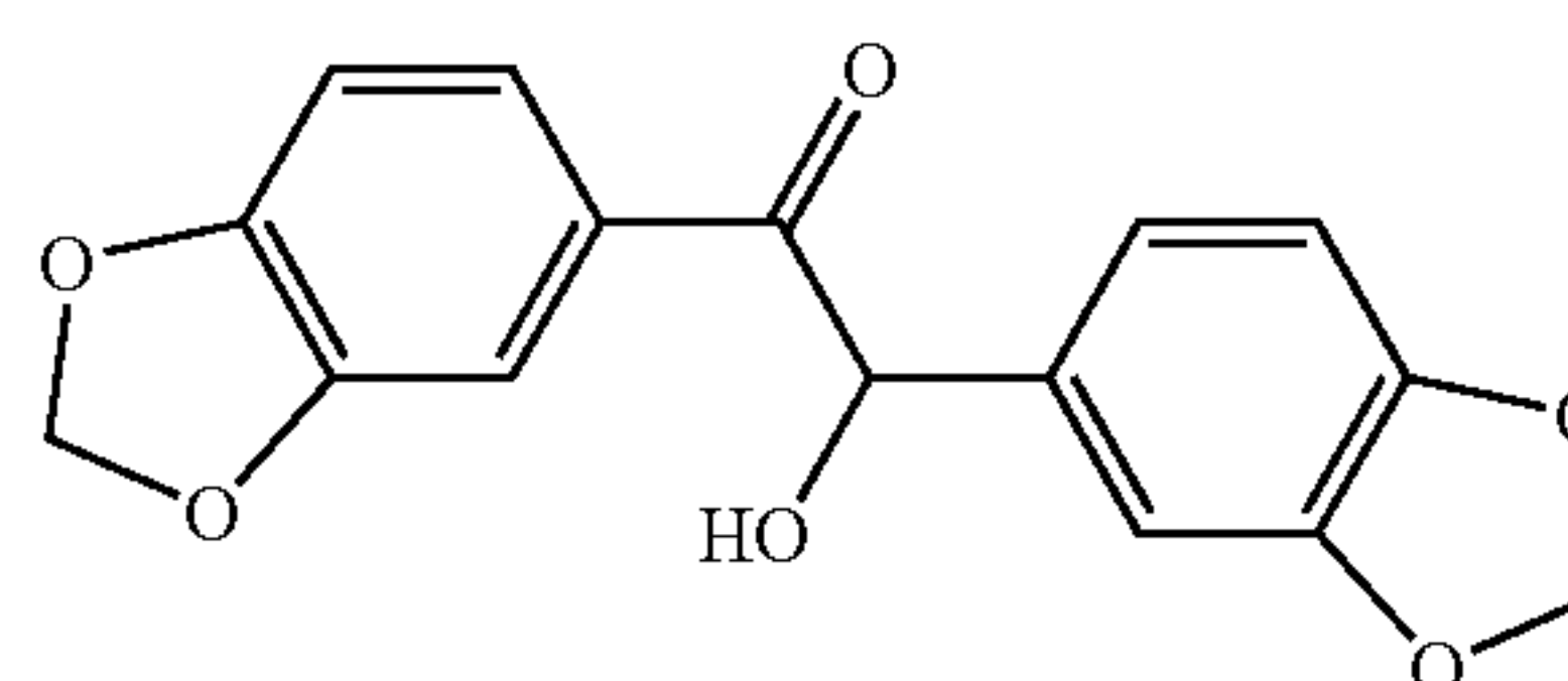
bis(3,4-methylenedioxy)benzoin
