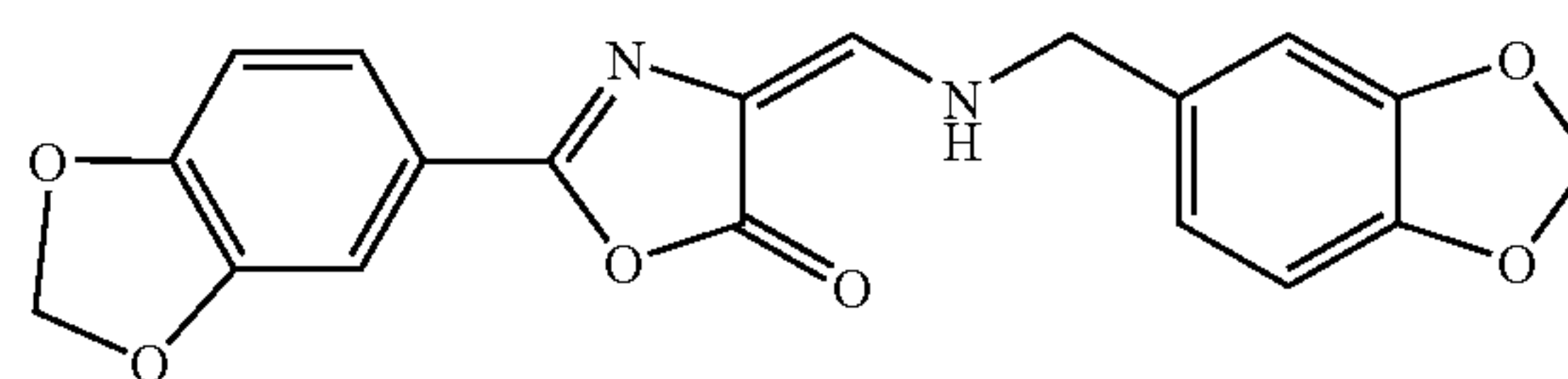
4-(3,4-methylenedioxybenzylaminomethylene)-2-(3,4-methylenedioxyphenyl)oxazolin-5-one
