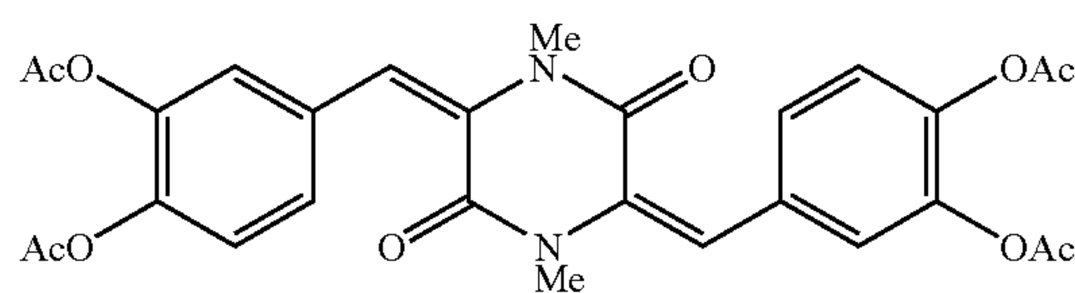
3,6-bis(3,4-diacetoxybenzylidene)-1,4- dimethyl-2,5-diketopiperazine
