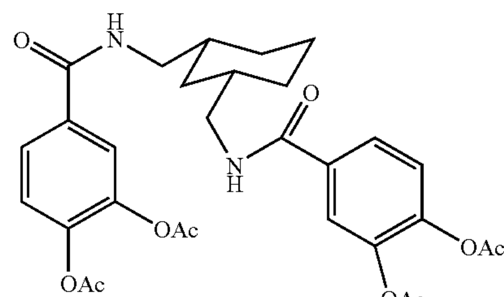
N,N'-bis(3,4-diacetoxybenzoyl)-cis- 1,3-bis-(aminomethyl)cyclohexane
