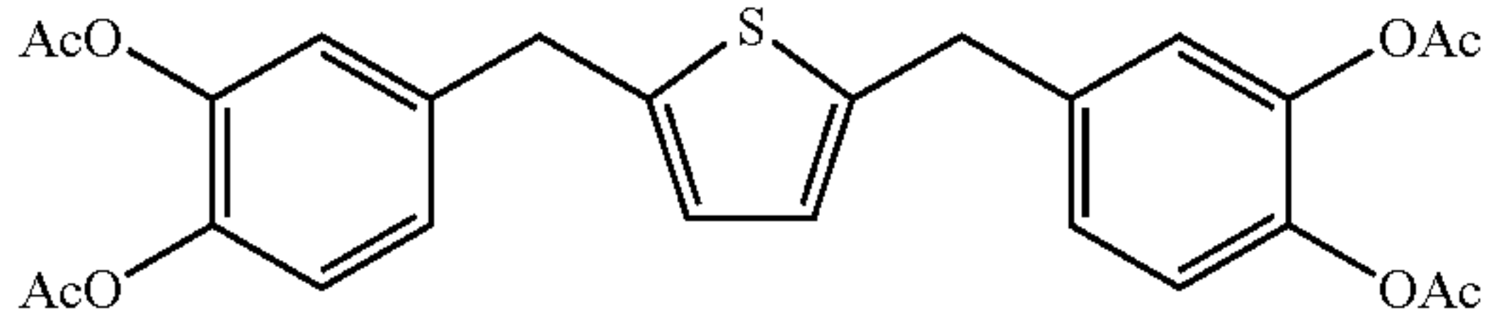
2,5-bis(3,4-diacetoxybenzyl)-thiophene
