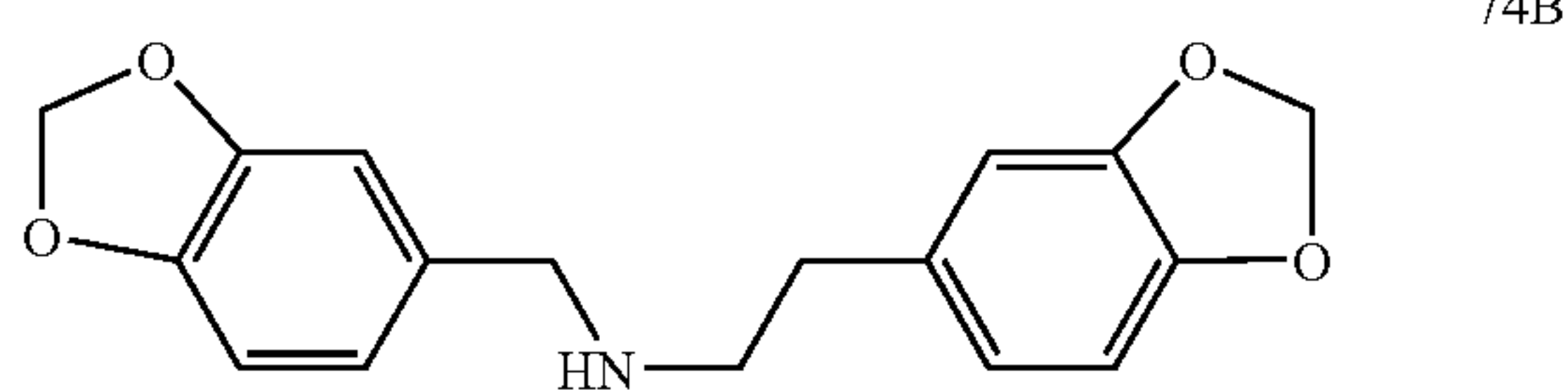
N-(3,4-methylenedioxybenzyl)-3,4-methylenedioxyphenethylamine
