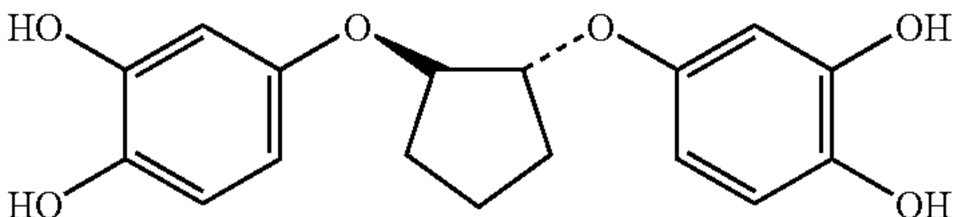
trans-1,2-bis(3,4-dihydroxyphenoxy)-cyclopentane
