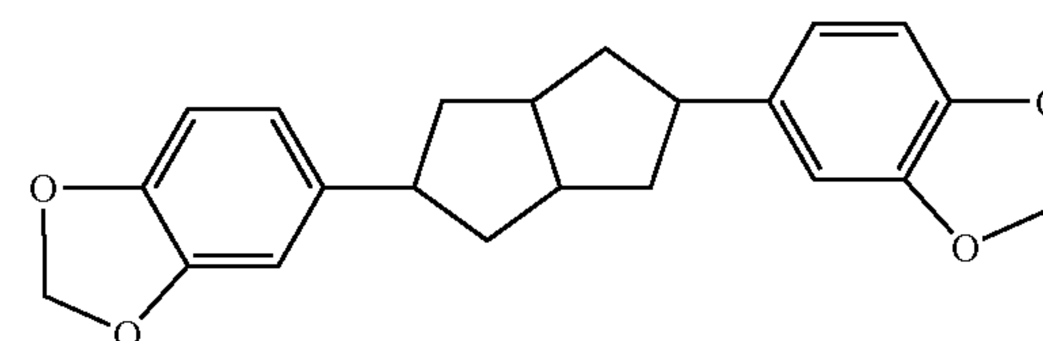
3,7-bis(3,4-methylenedioxyphenyl)-bicyclo[3,3,0] (-)octane
