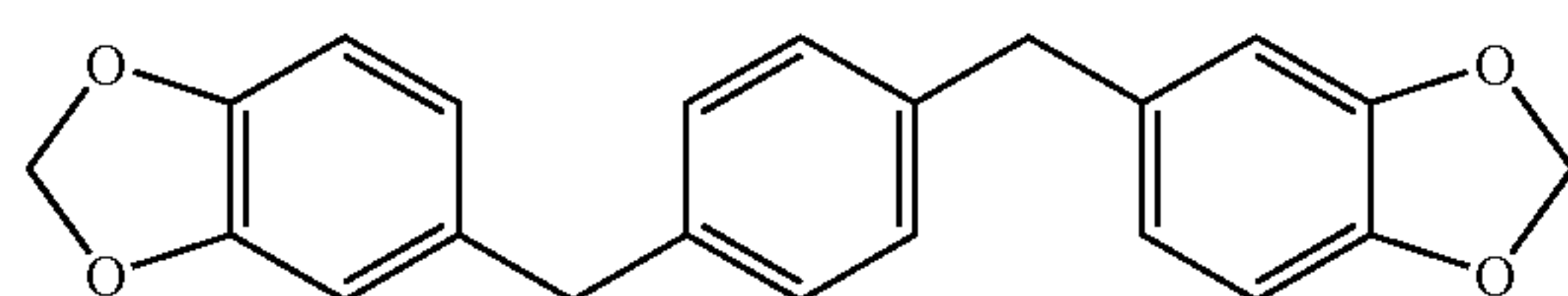
1,4-bis(3,4-methylenedioxybenzyl)-benzene
