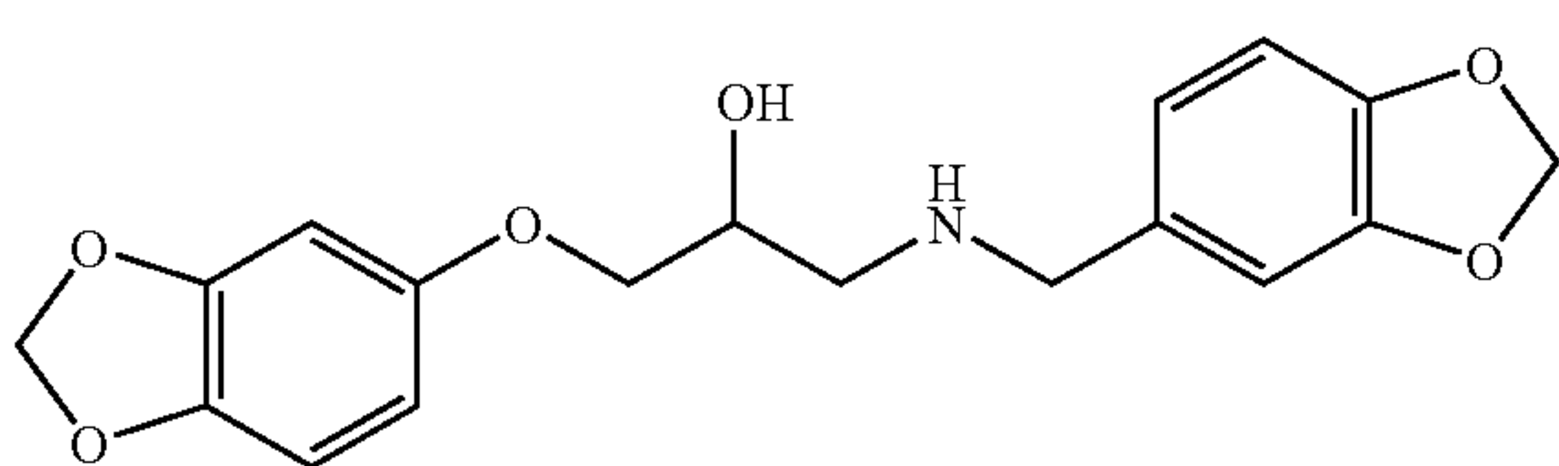
N-(3,4-methylenedioxybenzyl)-3-(3,4-methylenedioxy(-)phenoxy)-2-hydroxypropylamine
