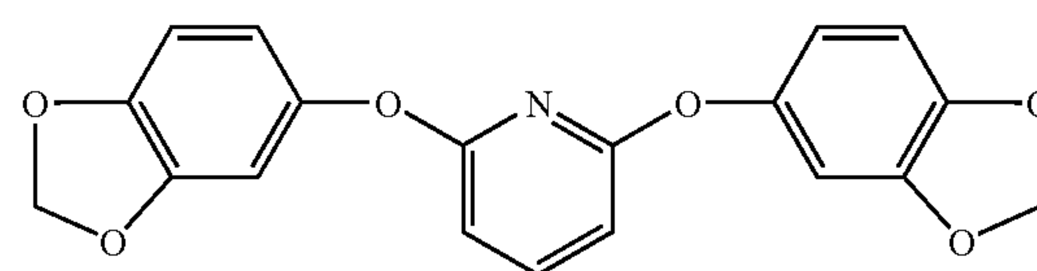
2,6-bis(3,4-methylenedioxyphenoxy)-pyridine
