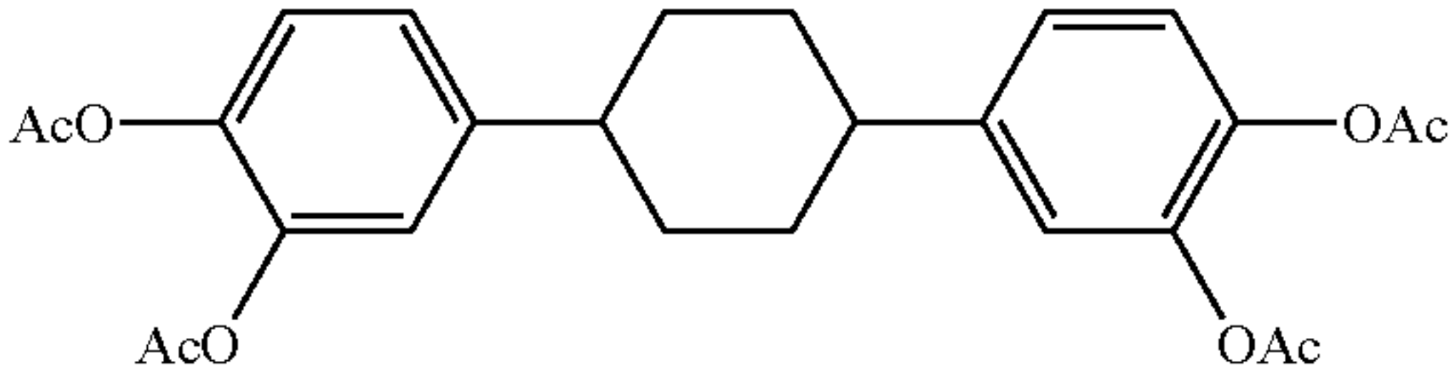
1,4-bis(3,4-diacetoxyphenyl)-cyclohexane
