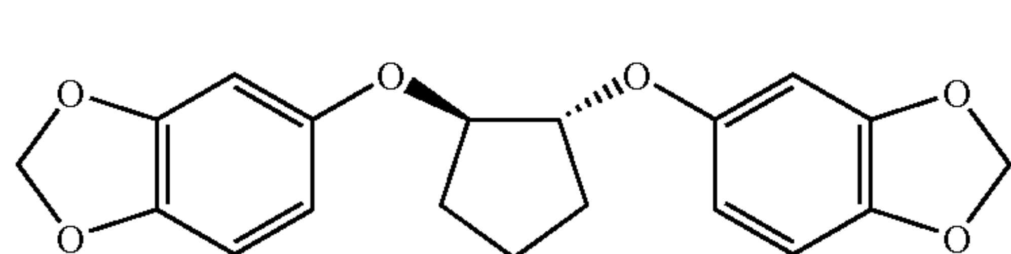
trans-1,2-bis(3,4-methylenedioxyphenoxy)-(-)-cyclopentane
