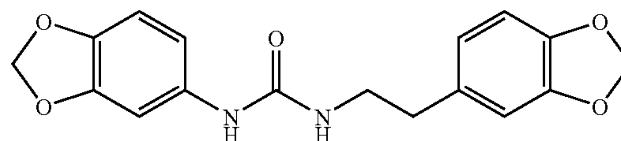
1-(3,4-methylenedioxyphenyl)-3-(3,4-methylenedioxyphenethyl) urea
