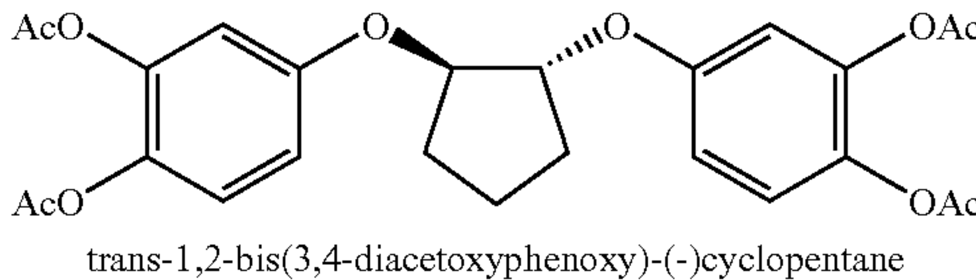
trans-1,2-bis(3,4-diacetoxyphenoxy)-(-)-cyclopentane
