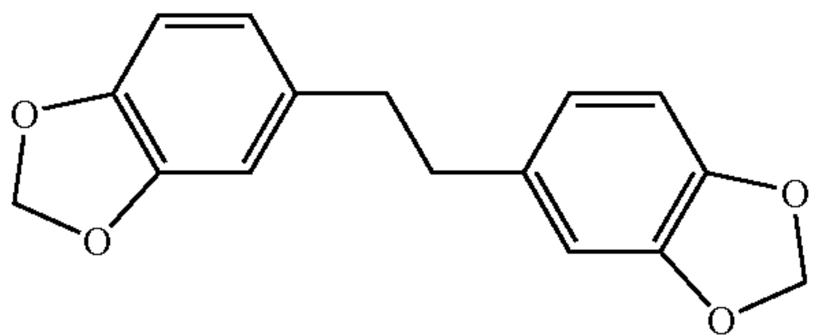
1,2-bis(3,4-methylenedioxyphenyl)ethane
