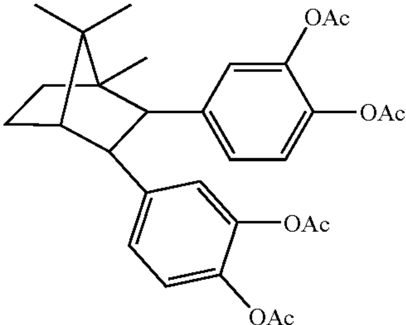
2,3-bis(3,4-diacetoxyphenyl)-1,7,7-trimethyl- bicyclo[2,2,1]heptane
