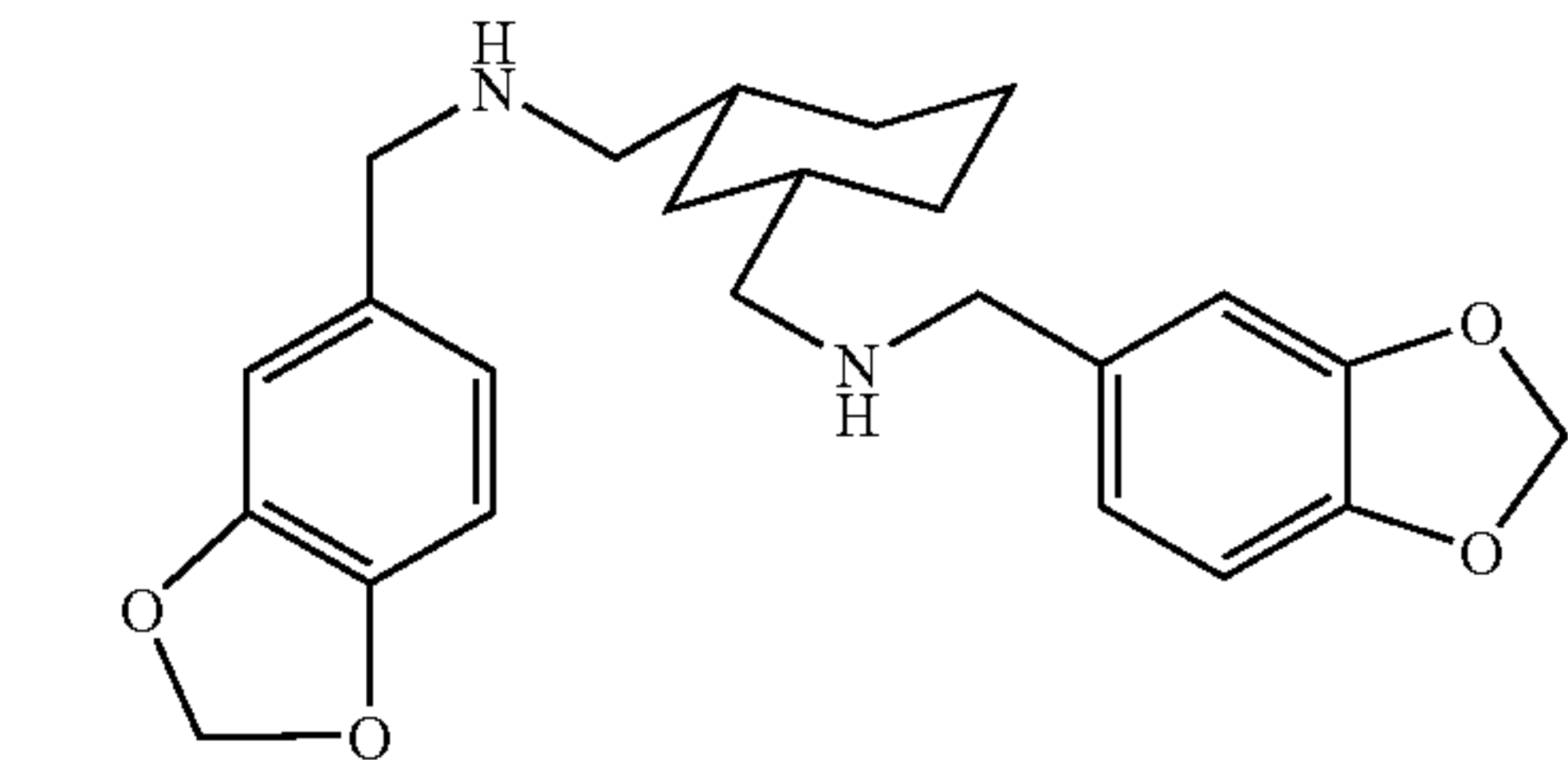
N,N'-bis(3,4-methylenedioxybenzyl)-cis- 1,3-bis-(aminomethyl)cyclohexane
