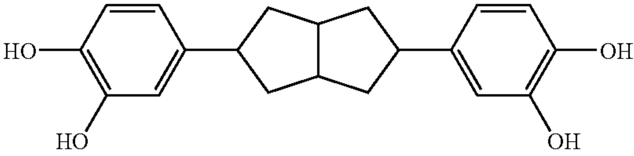
2,5-bis(3,4-dihydroxybenzoyl)bicyclo[3.3.0](-)octane
