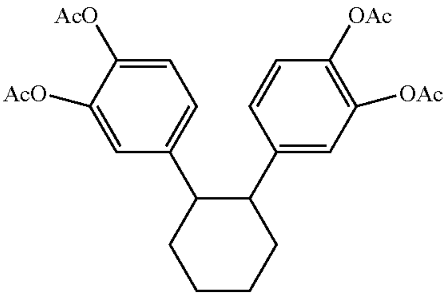
1,2-bis(3,4-diacetoxyphenyl)-cyclohexane
