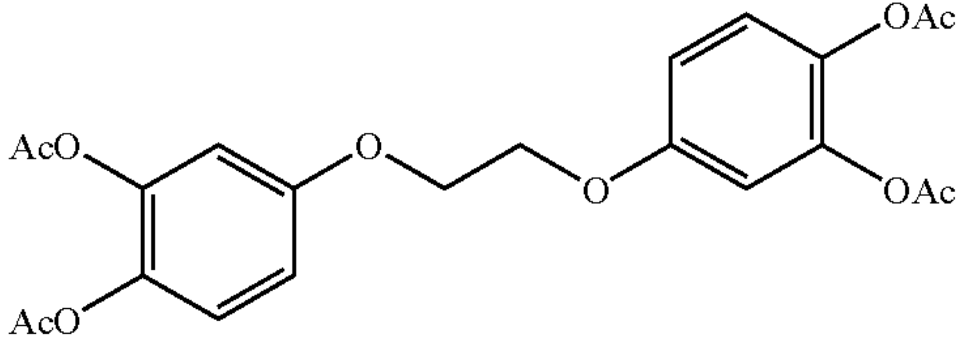
1,2-bis(3,4-diacetoxyphenoxy)-ethane
