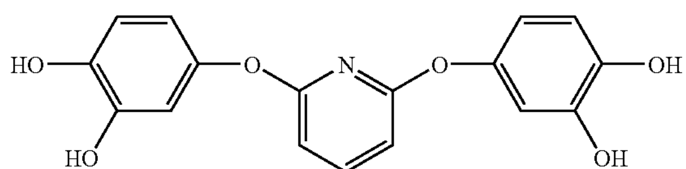
2, 6-bis(3,4-dihydroxyphenoxy)pyridine
