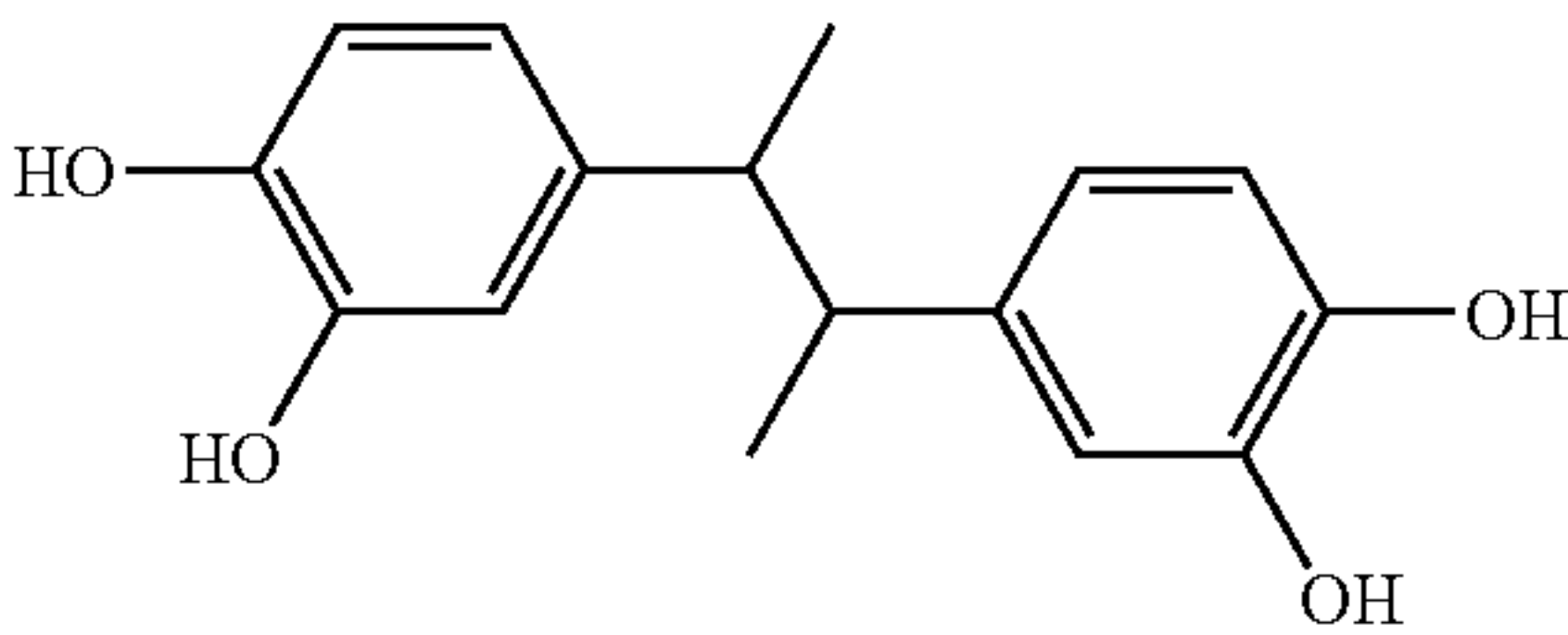
2,3-bis(3,4-dihydroxyphenyl)butane
