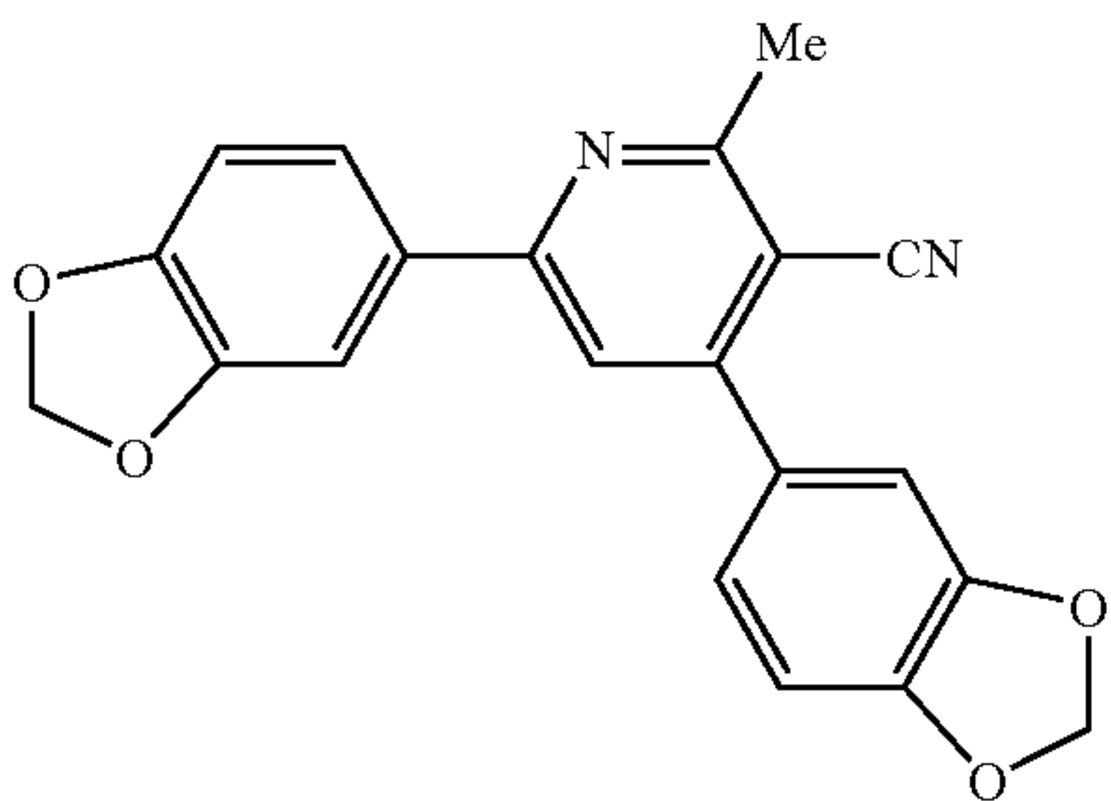
4,6-bis(3,4-methylenedioxyphenyl)-3-cyano-2-methylpyridine
