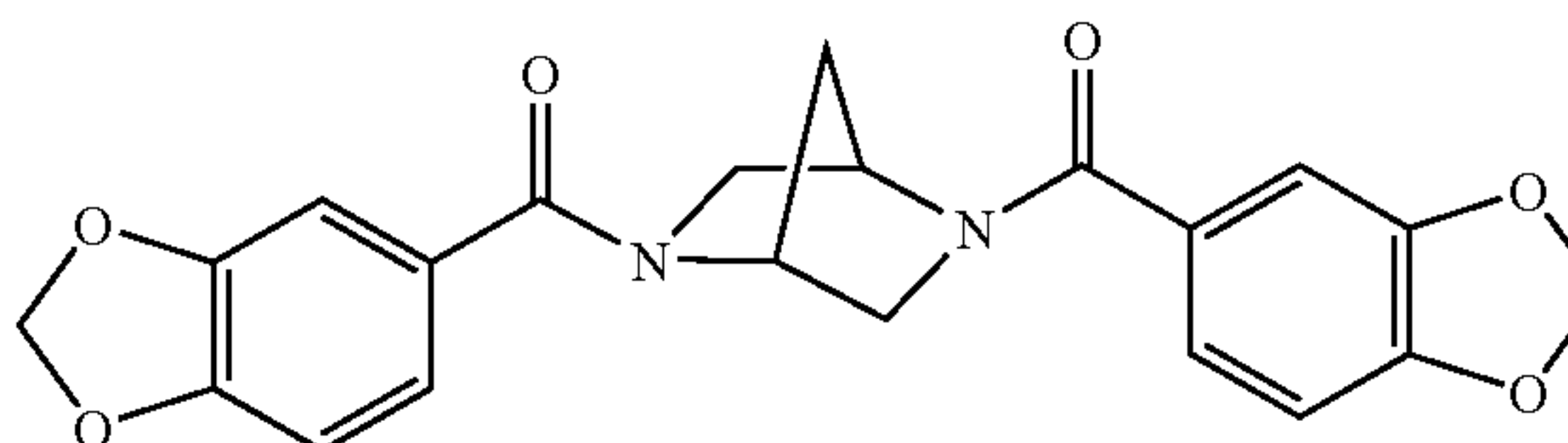
2,5-bis(3,4-methylenedioxybenzoyl)-2,5-diaza[2,2,1]-bicycloheptane
