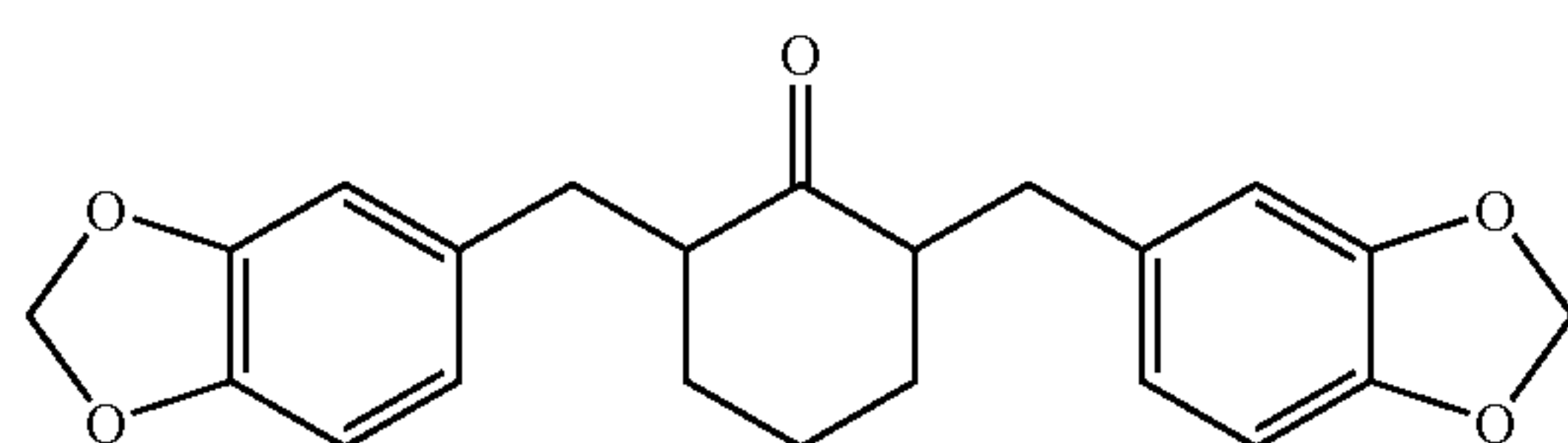
2,6-bis(3,4-methylenedioxybenzyl)cyclohexanone
