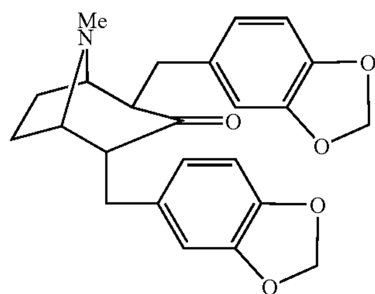
2,4-bis(3,4-methylenedioxybenzyl)-3-tropinone
