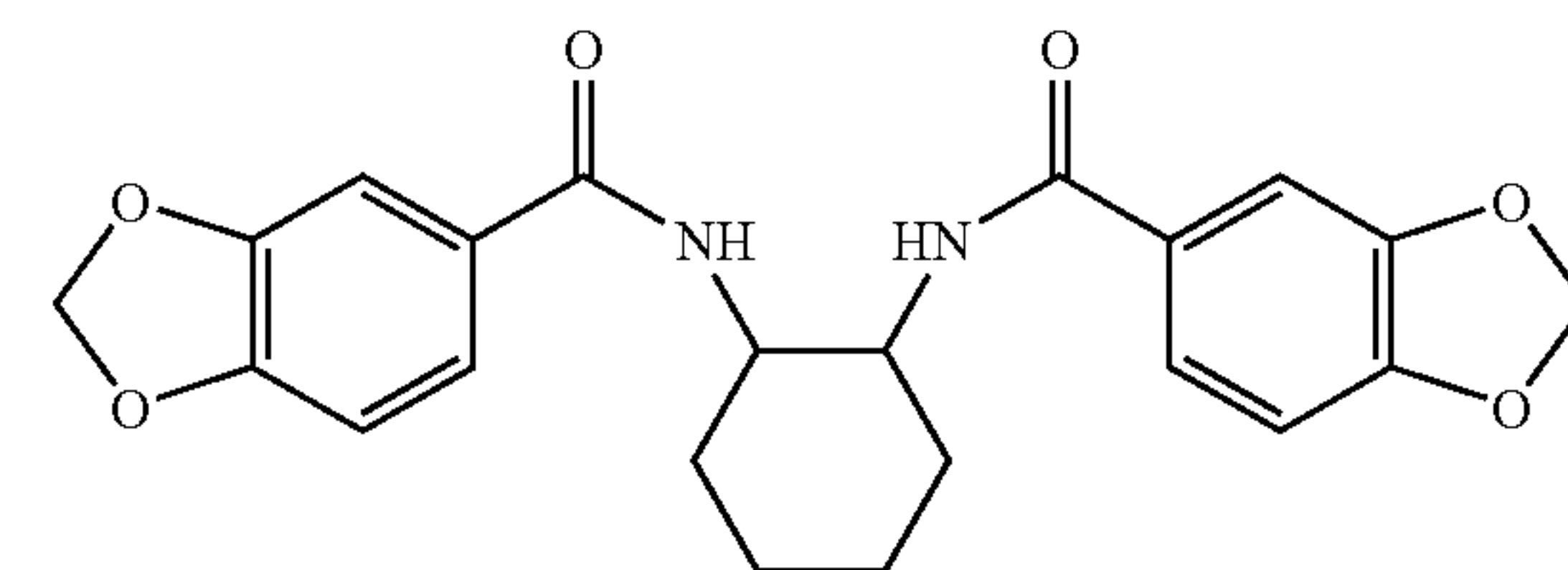
N,N'-bis(3,4-methylenedioxybenzoyl)-trans-diaminocyclohexane
