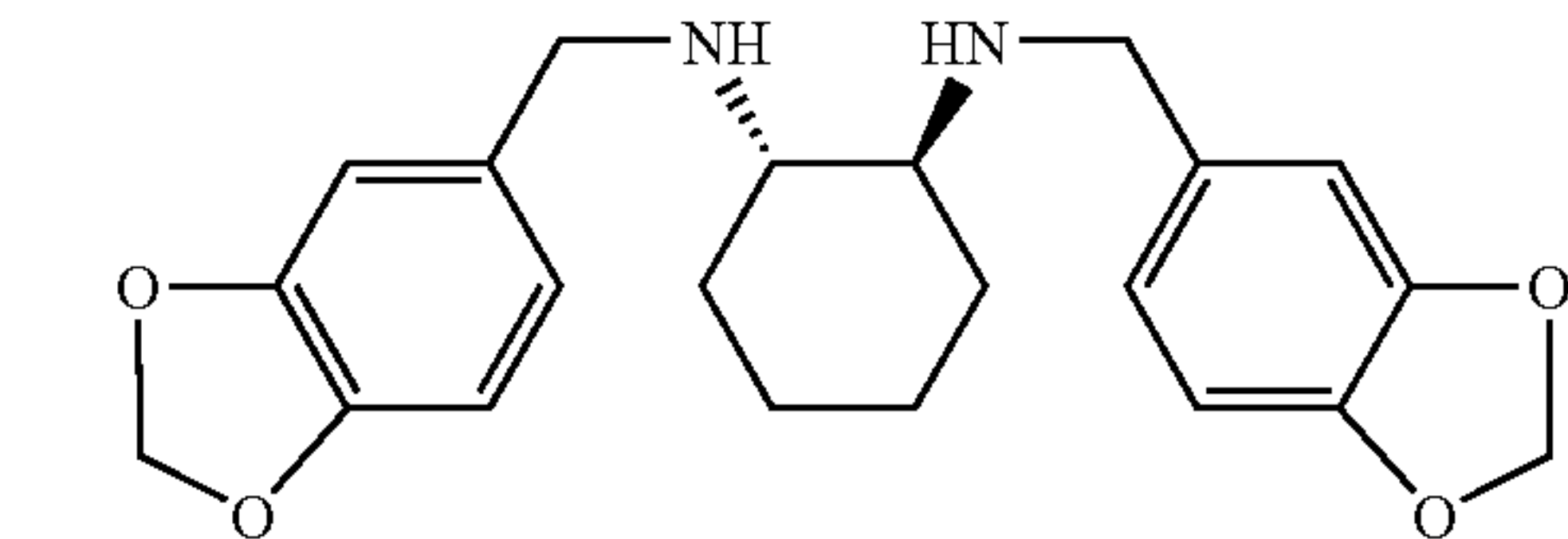
N,N'-bis(3,4-methylenedioxybenzyl)-trans-1,2- diaminocyclohexane
