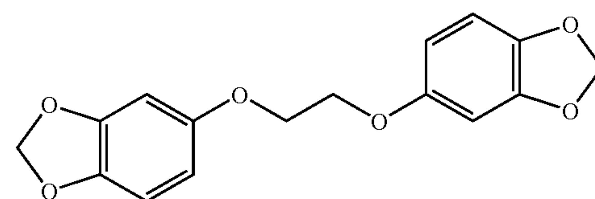
1,2-bis(3,4-methylenedioxyphenoxy)-ethane
