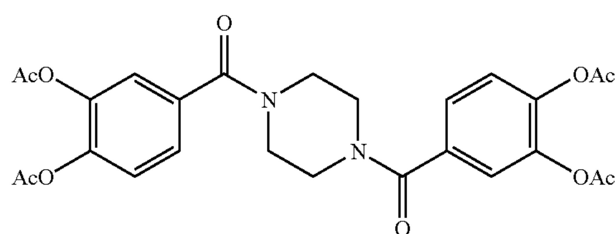
1,4-bis(3,4-diacetoxybenzoyl)-piperazine
