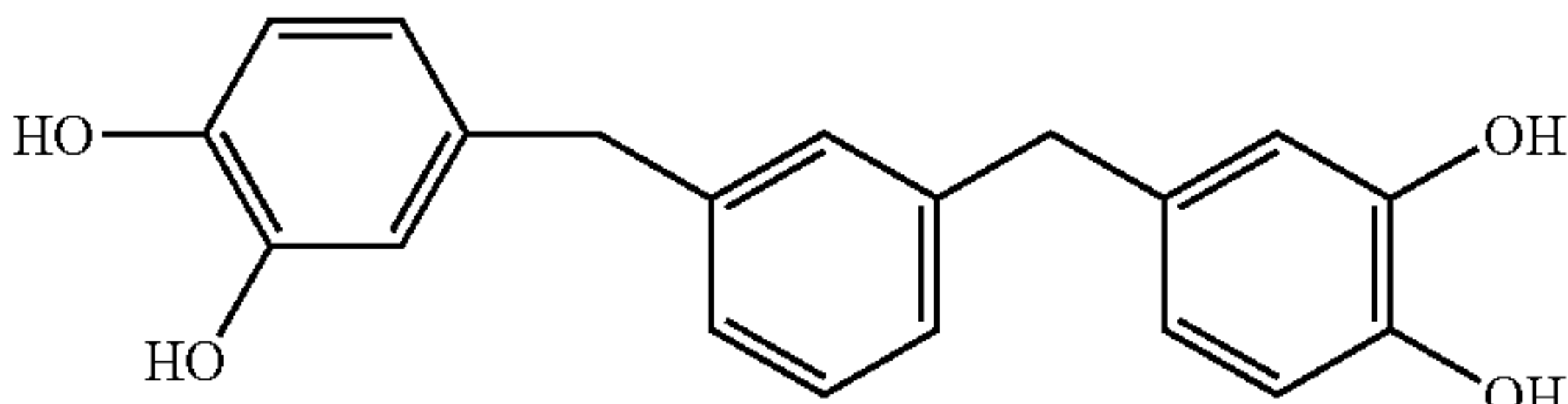
1,3-bis(3,4-dihydroxybenzyl)-benzene
