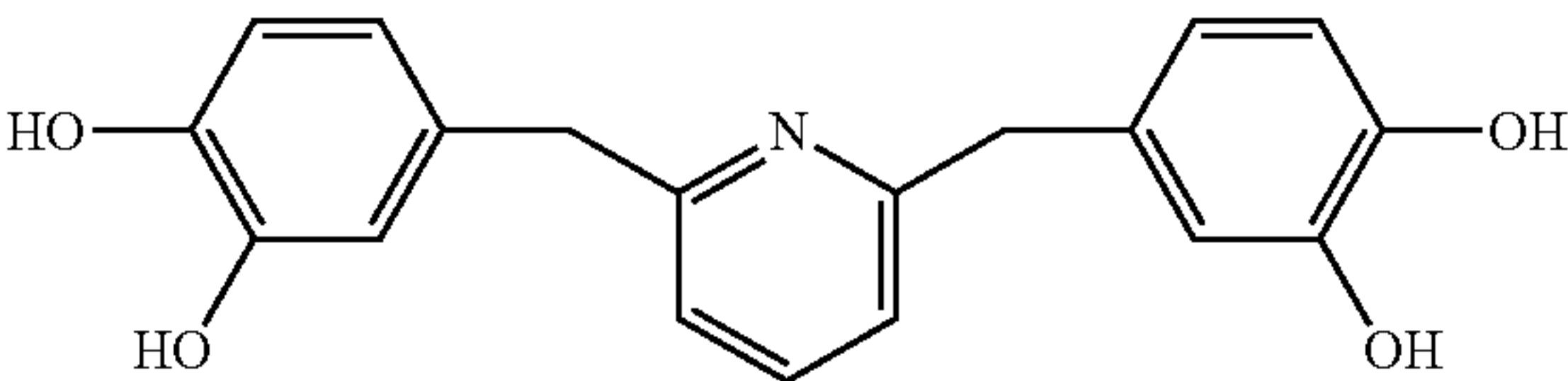
2,6-bis(3,4-dihydroxybenzyl)pyridine
