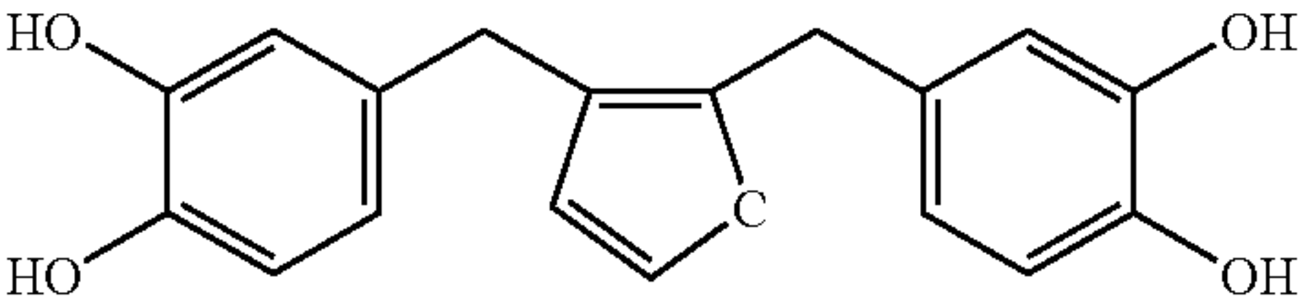
2,3-bis(3,4-dihydroxybenzyl)thiophene
