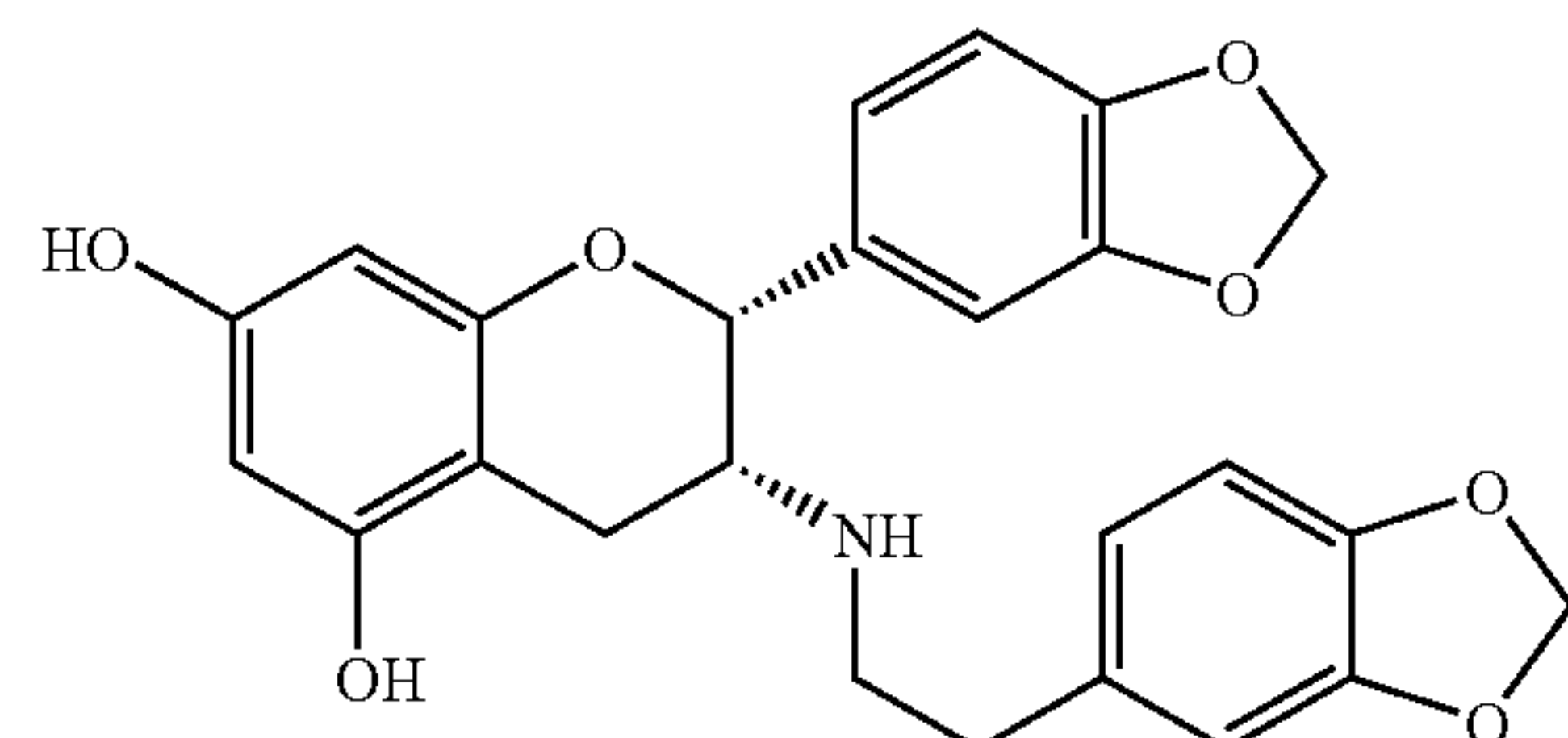
3-deoxy-3-(3,4-methylenedioxyphenethyl)-aminoepicatechin
