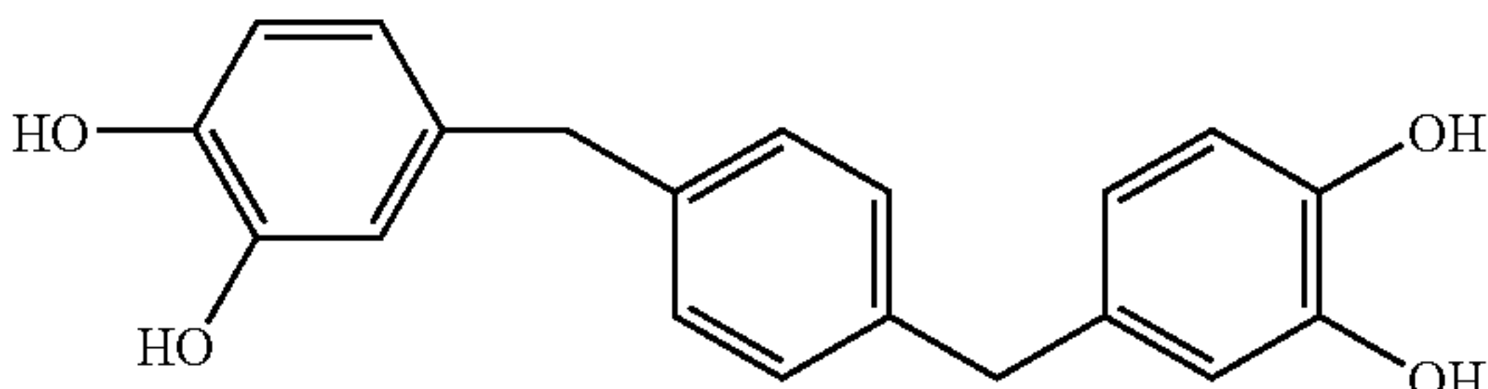
1,4-bis(3,4-dihydroxybenzyl)-benzene
