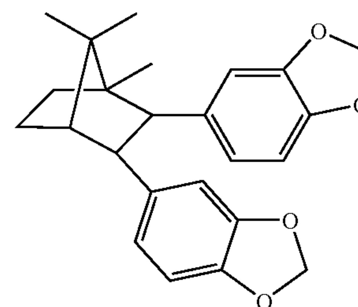
2,3-bis(3,4-methylenedioxyphenyl)-1,7,7-trimethyl- bicyclo[2,2,1]heptane
