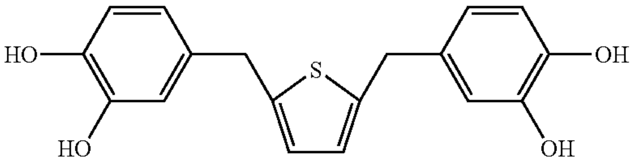
2,5-bis(3,4-dihydroxybenzyl)thiophene
