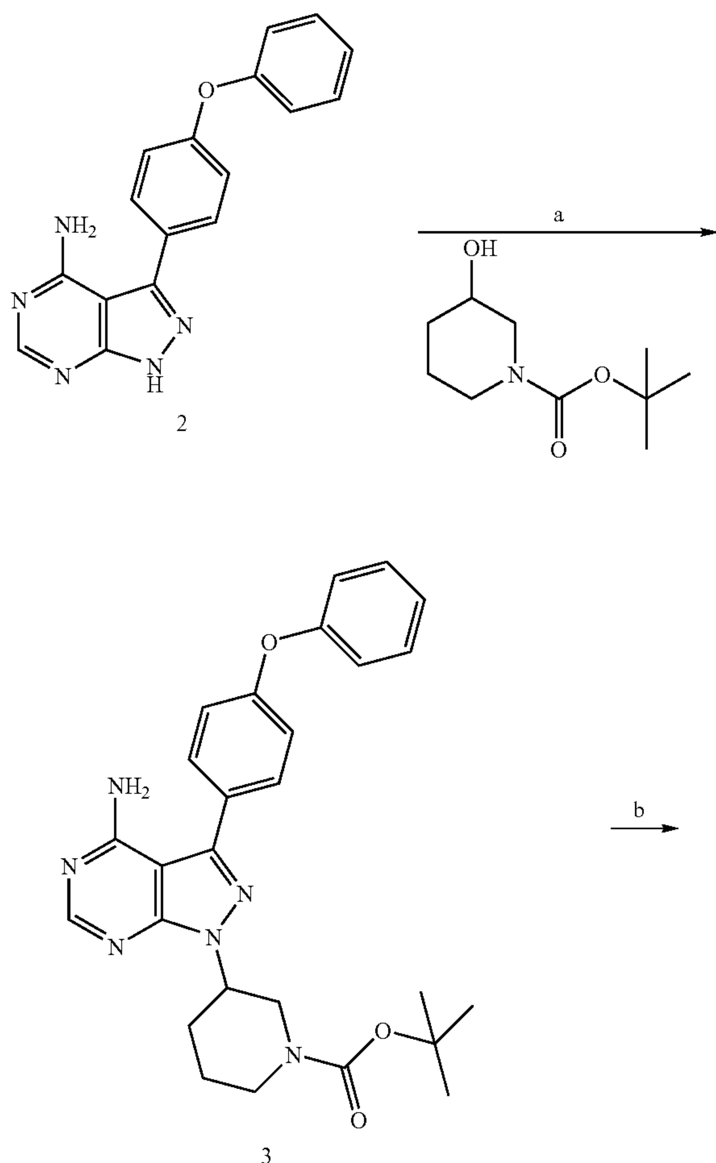
Scheme 1.
