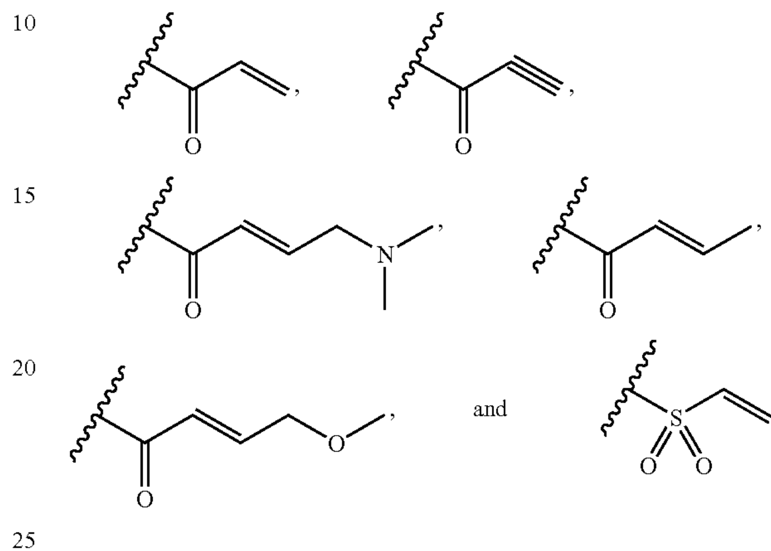
Formula (B)
