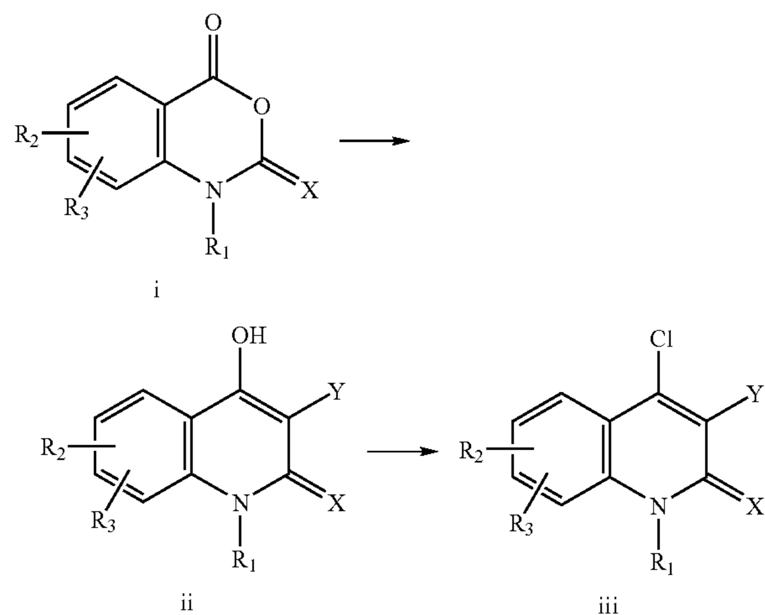
Reaction Scheme 1
