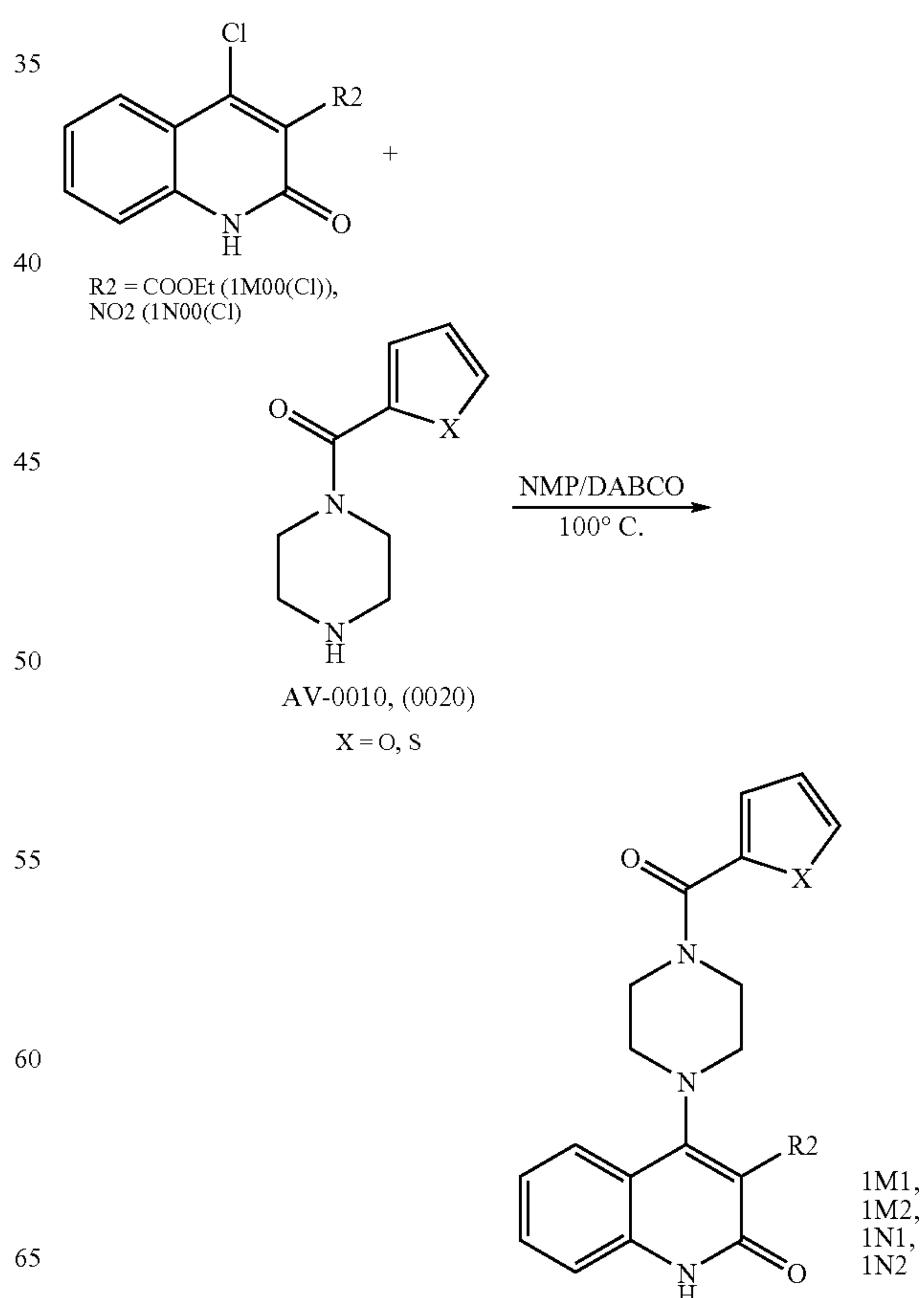
Reaction Scheme 12
