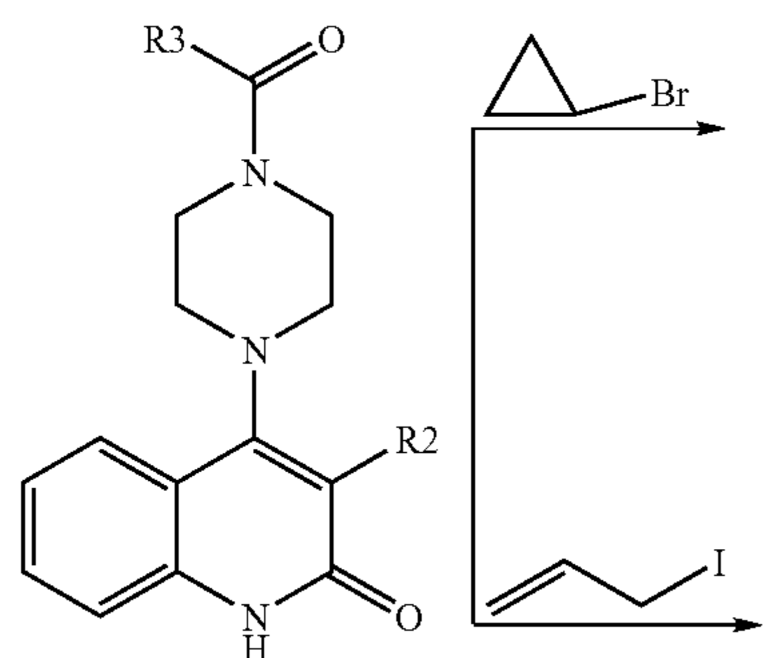
Reaction Scheme 8
