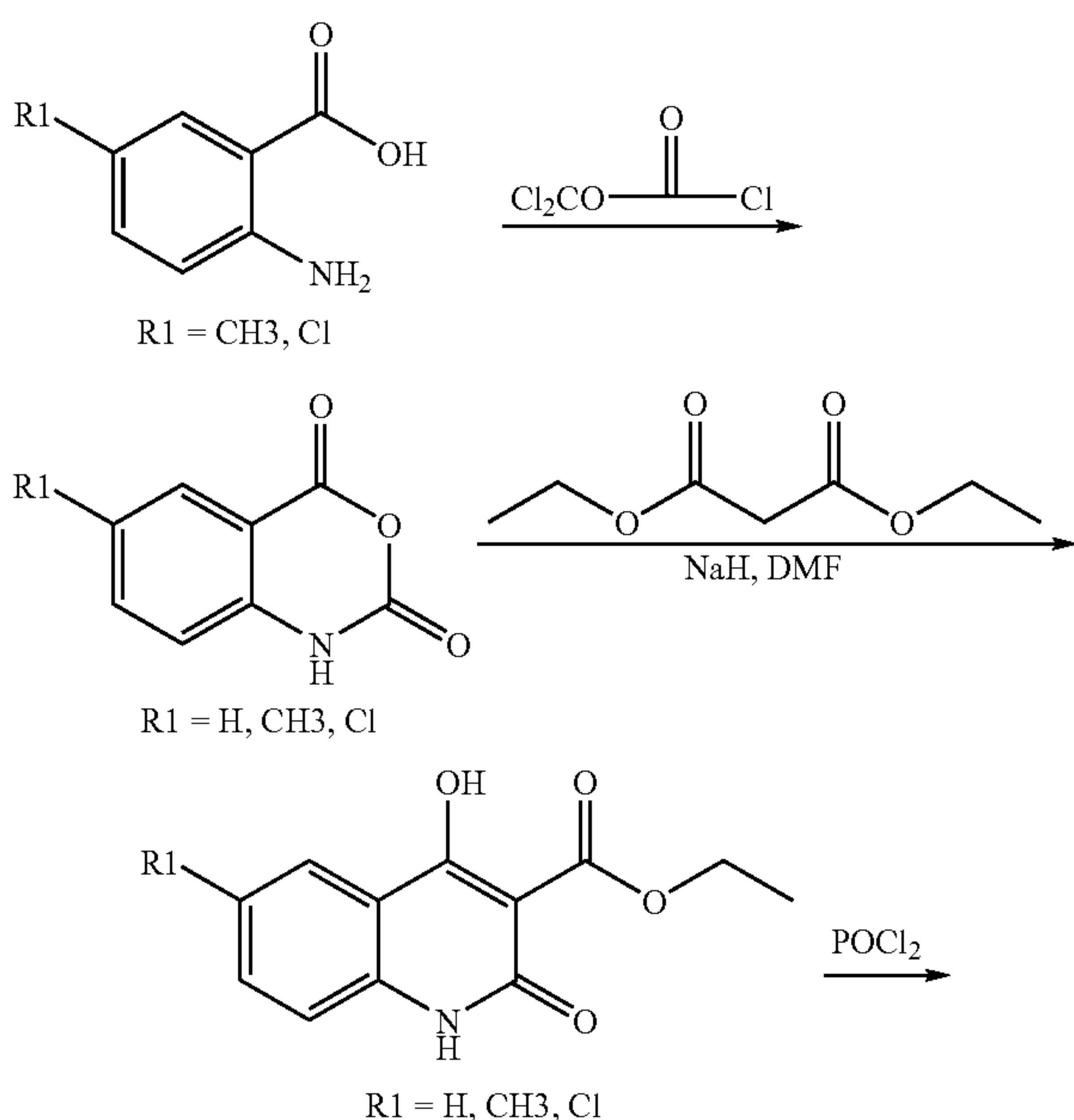
Reaction Scheme 21
