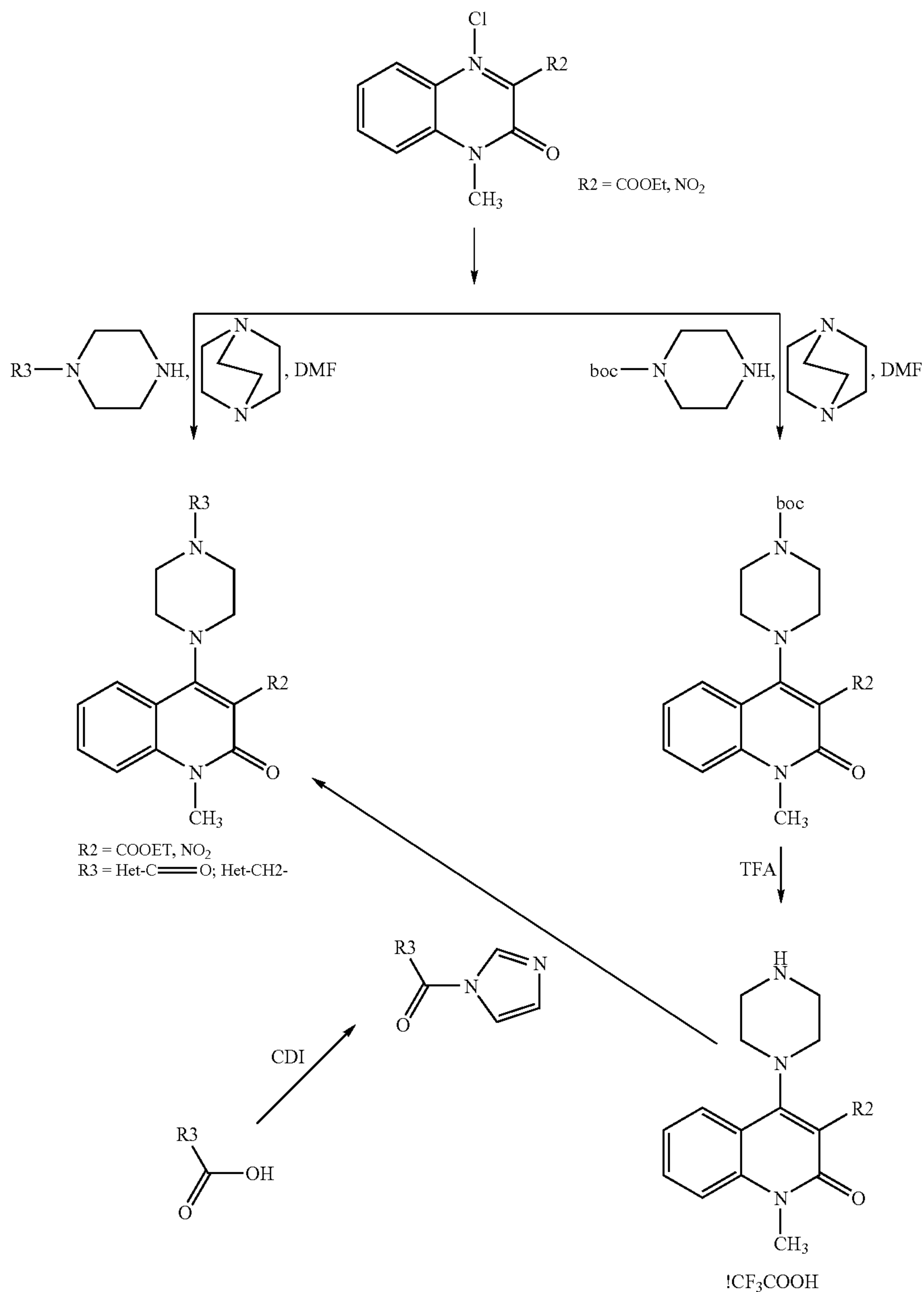
Reaction Scheme 10
