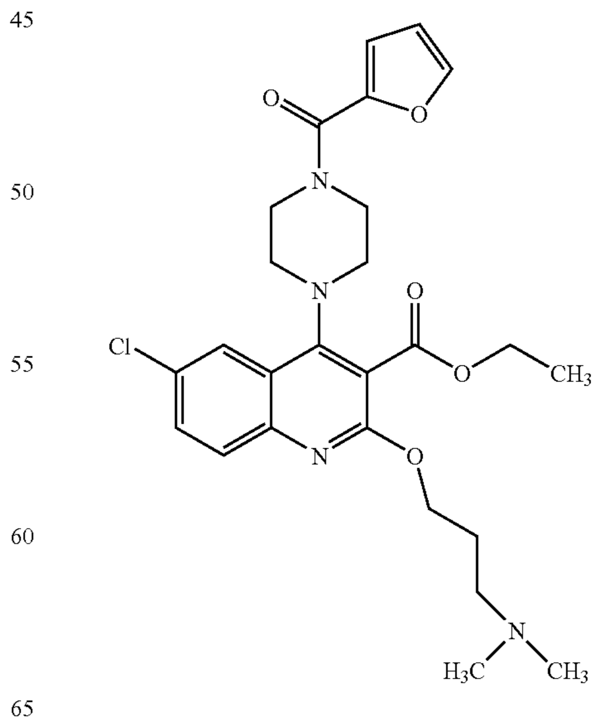
Compound 328
