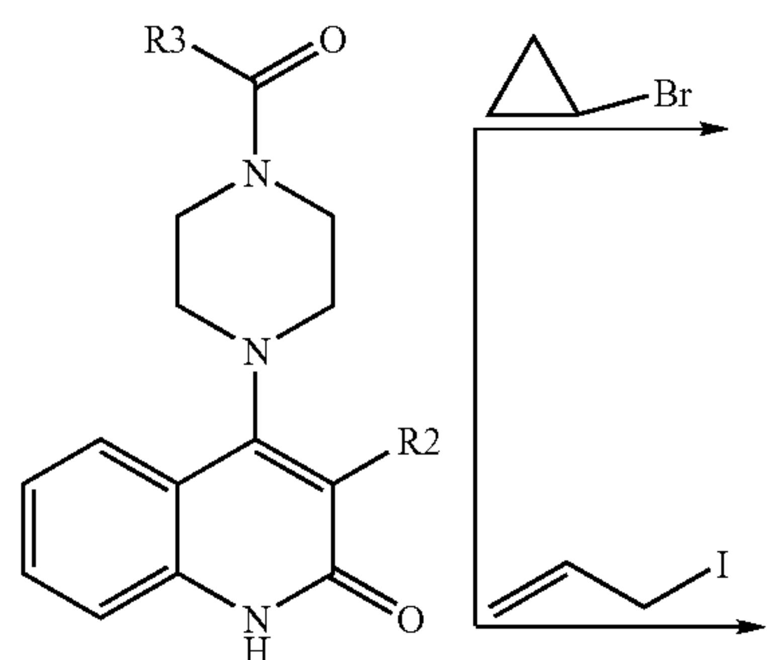
Reaction Scheme 8
