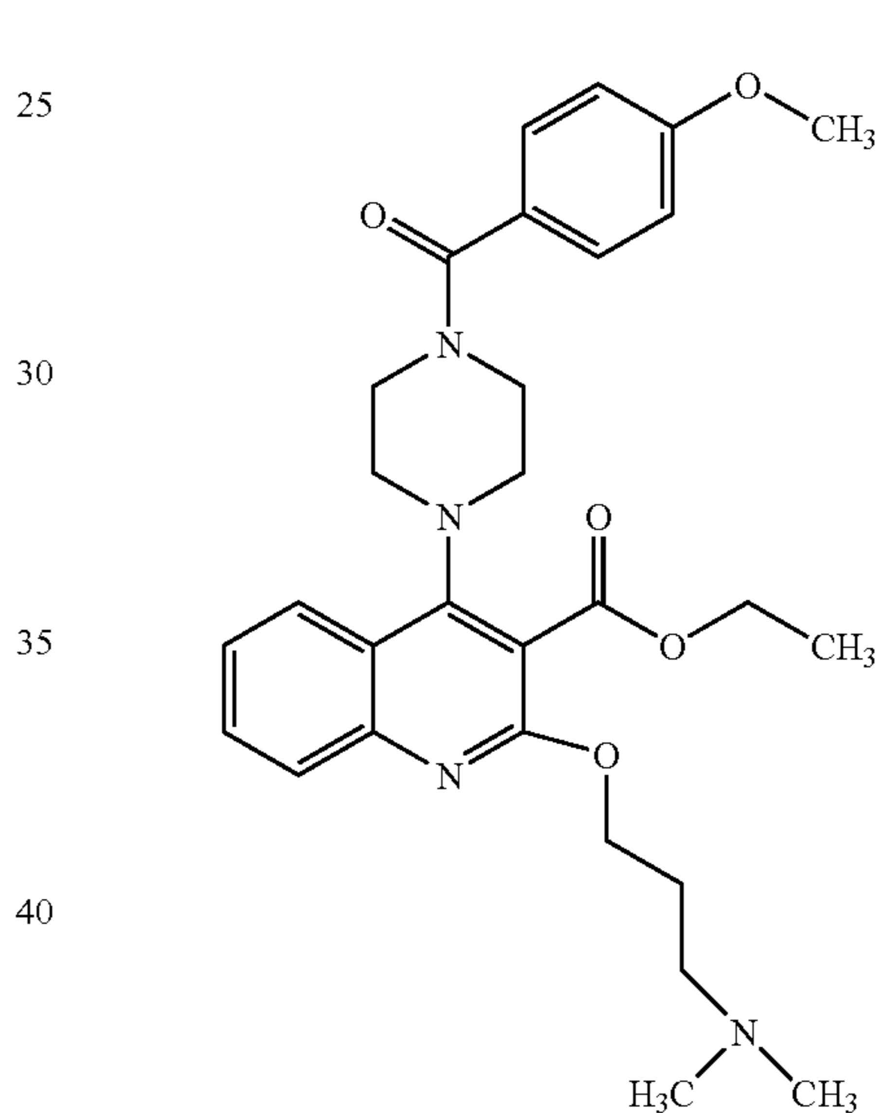
Compound 327
