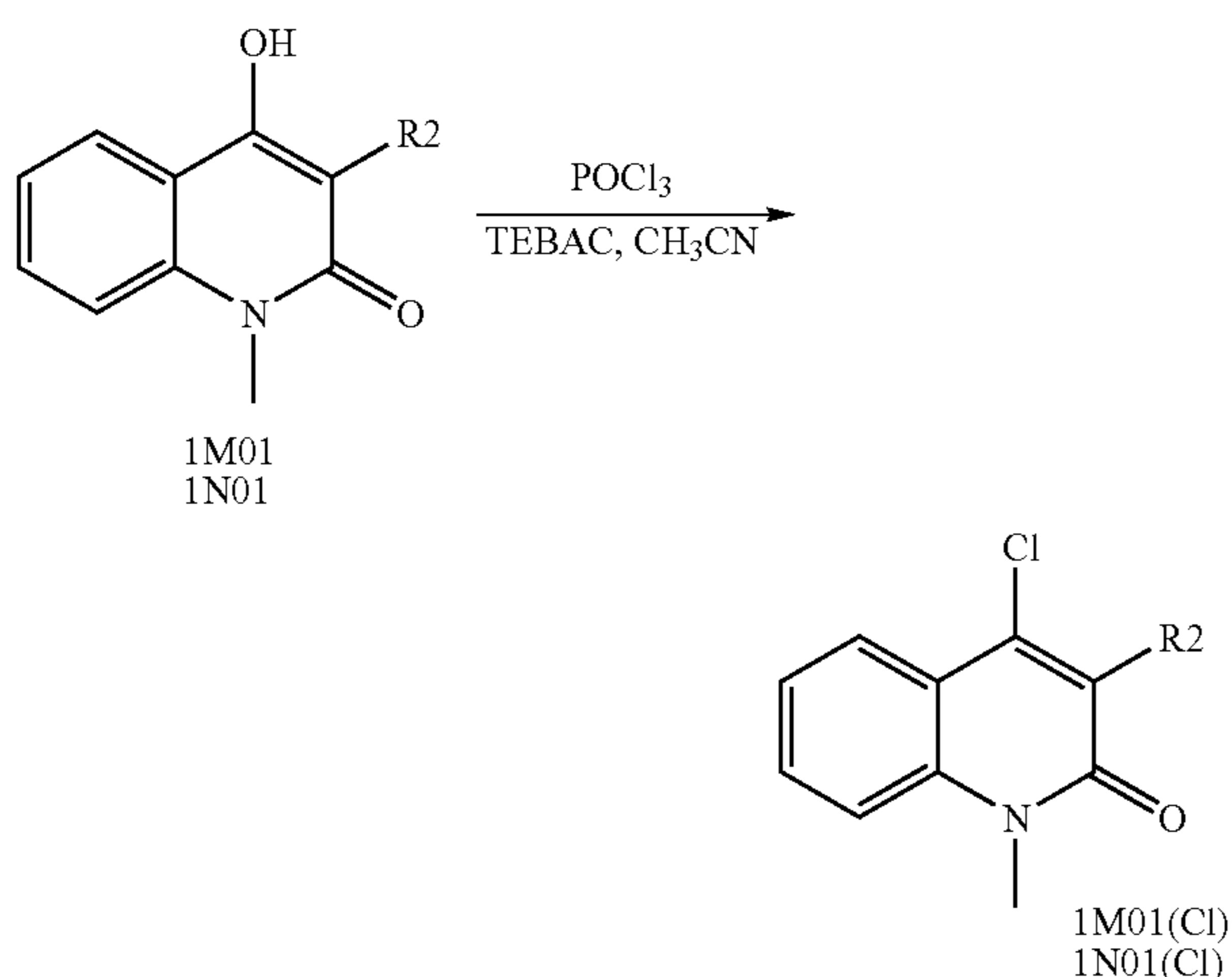
Reaction Scheme 14
