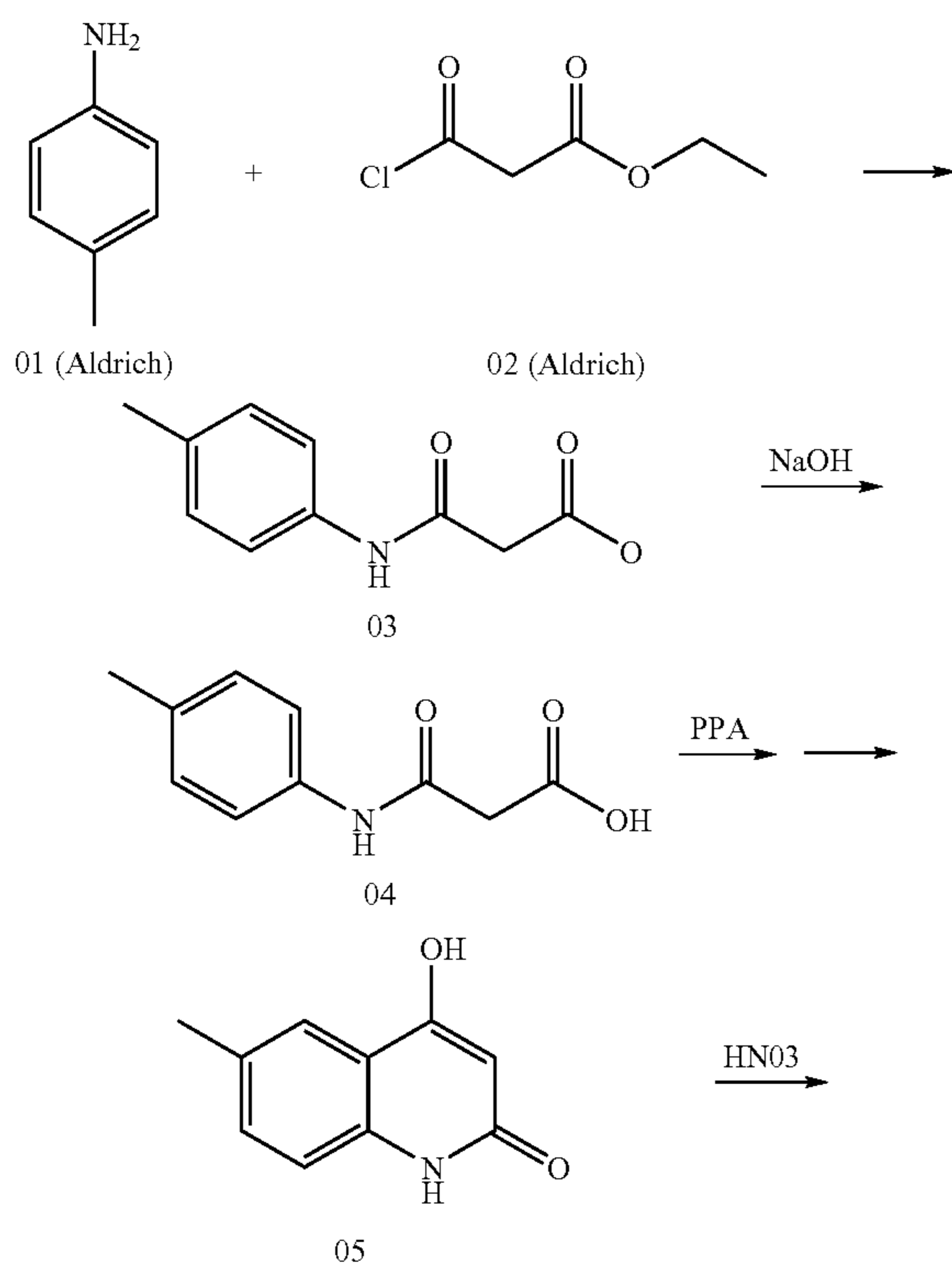
Reaction Scheme 25
