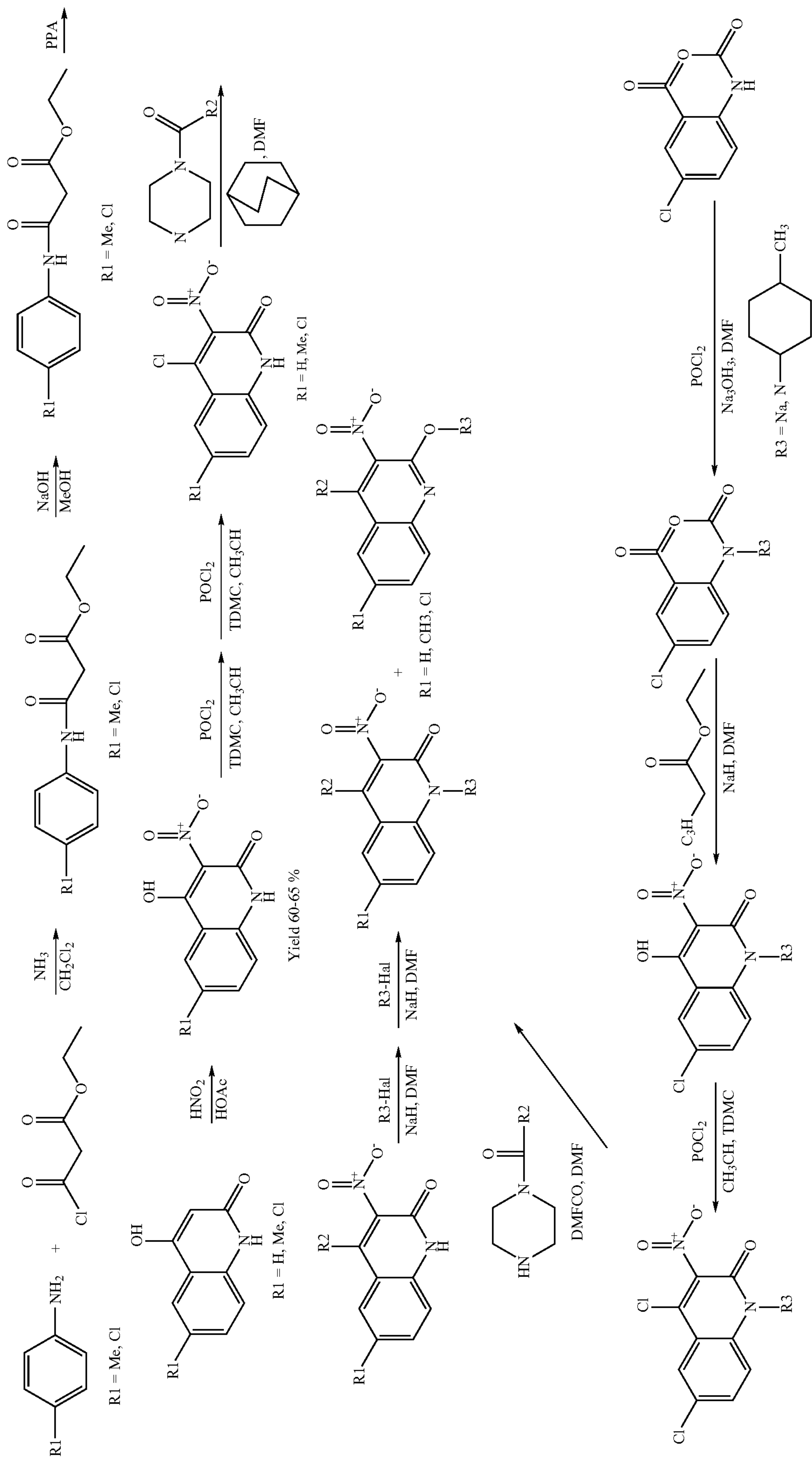
Reaction Scheme 22
