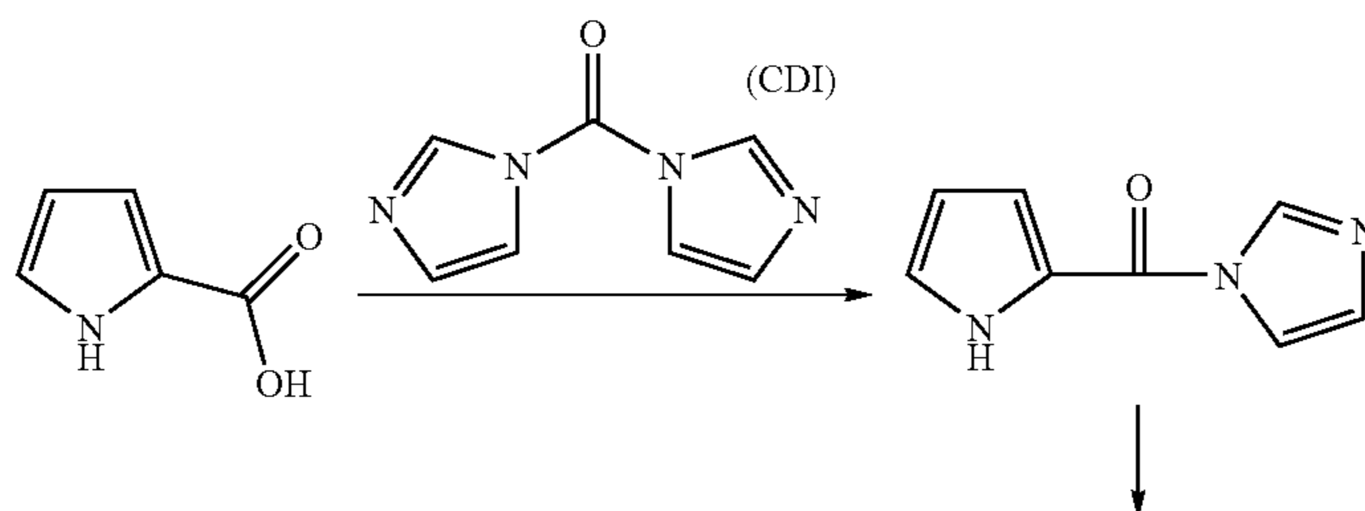
Reaction Scheme 17
