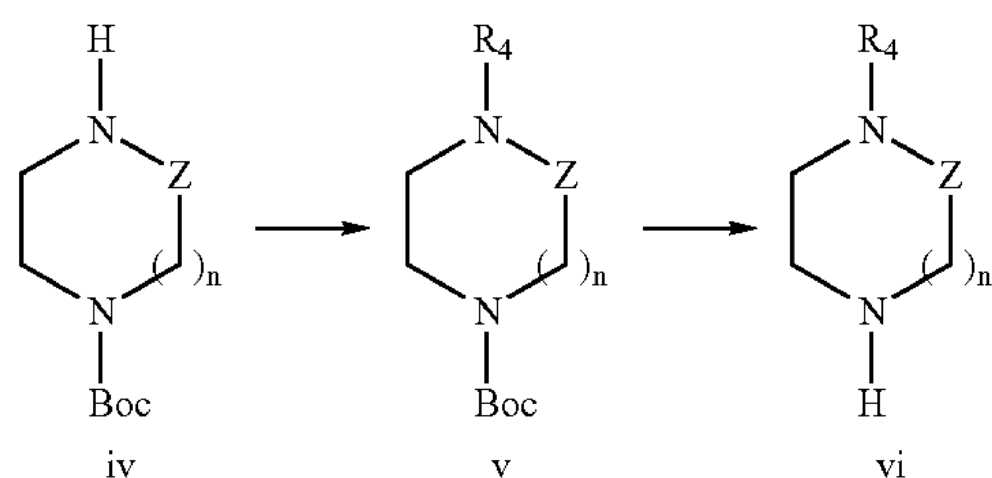
Reaction Scheme 2
