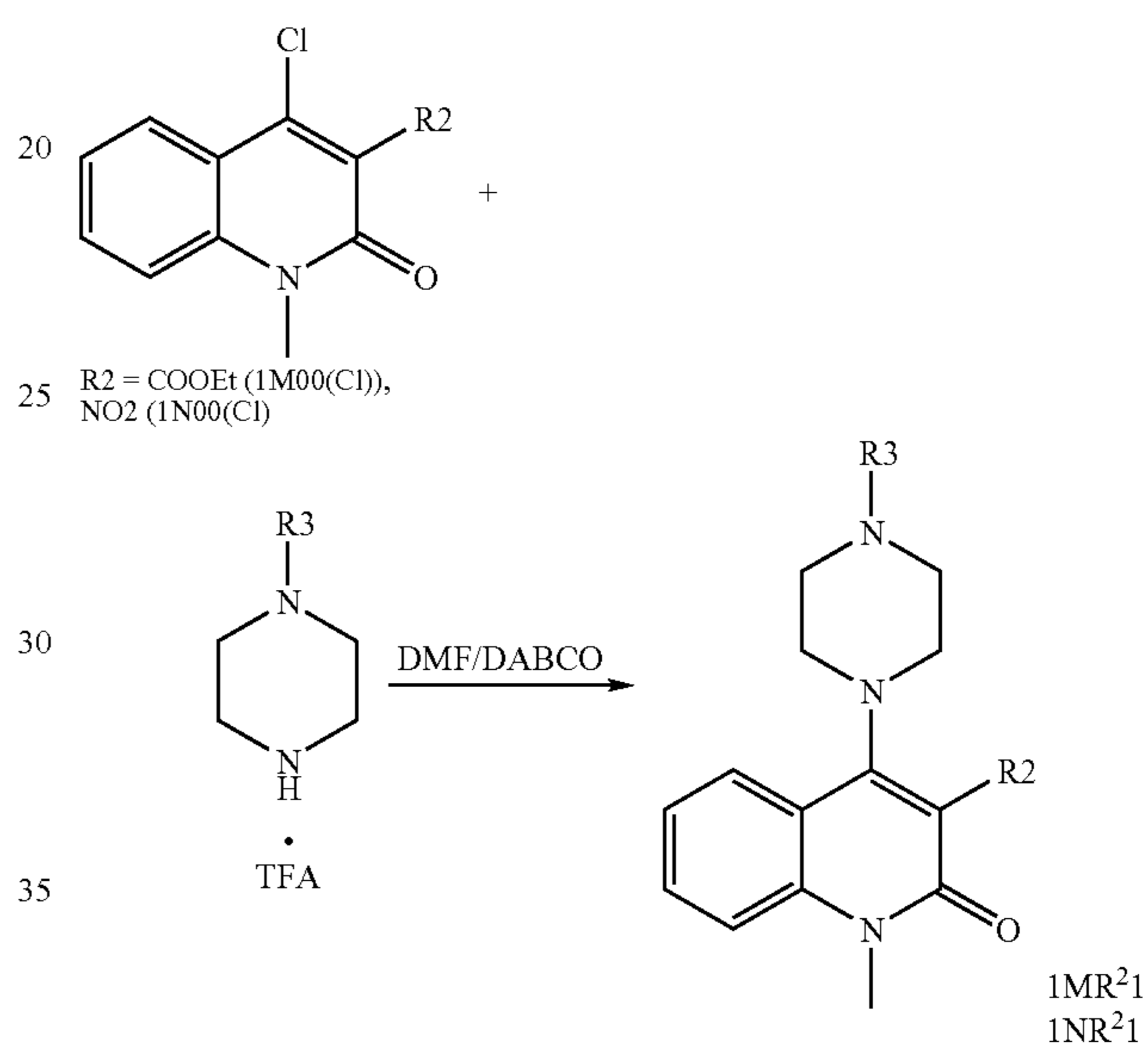
Reaction Scheme 16
