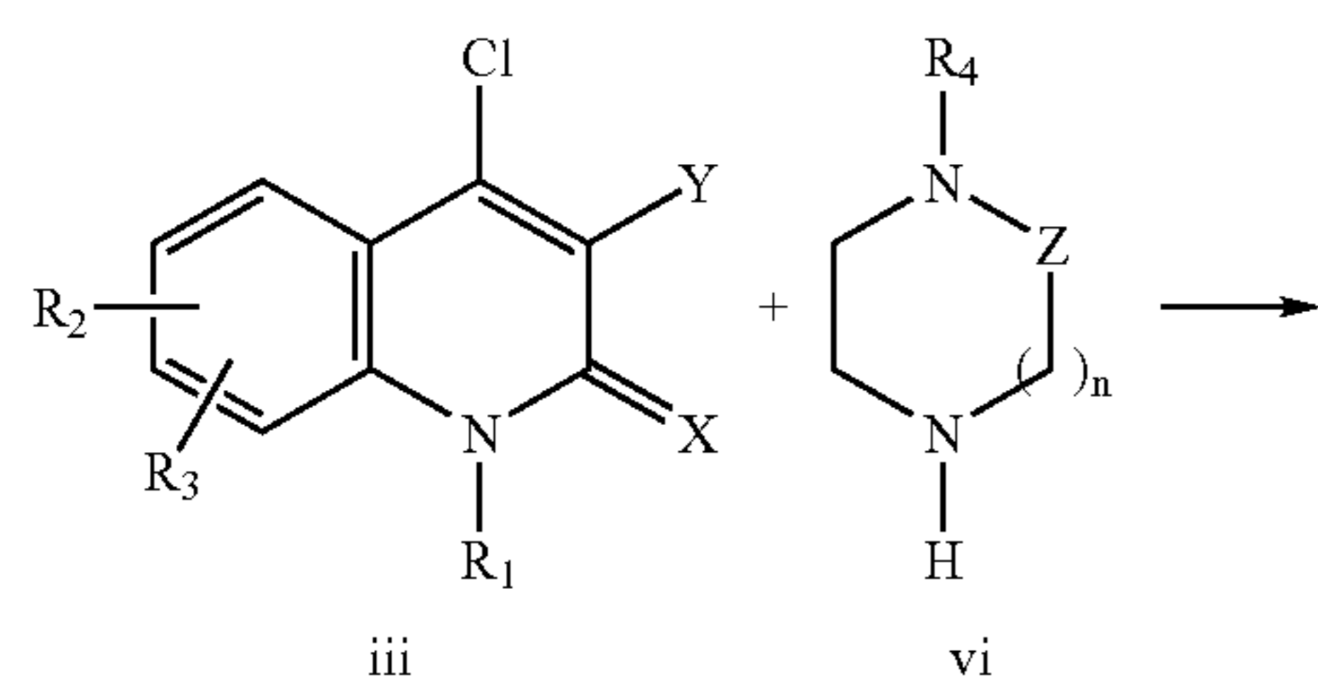
Reaction Scheme 3
