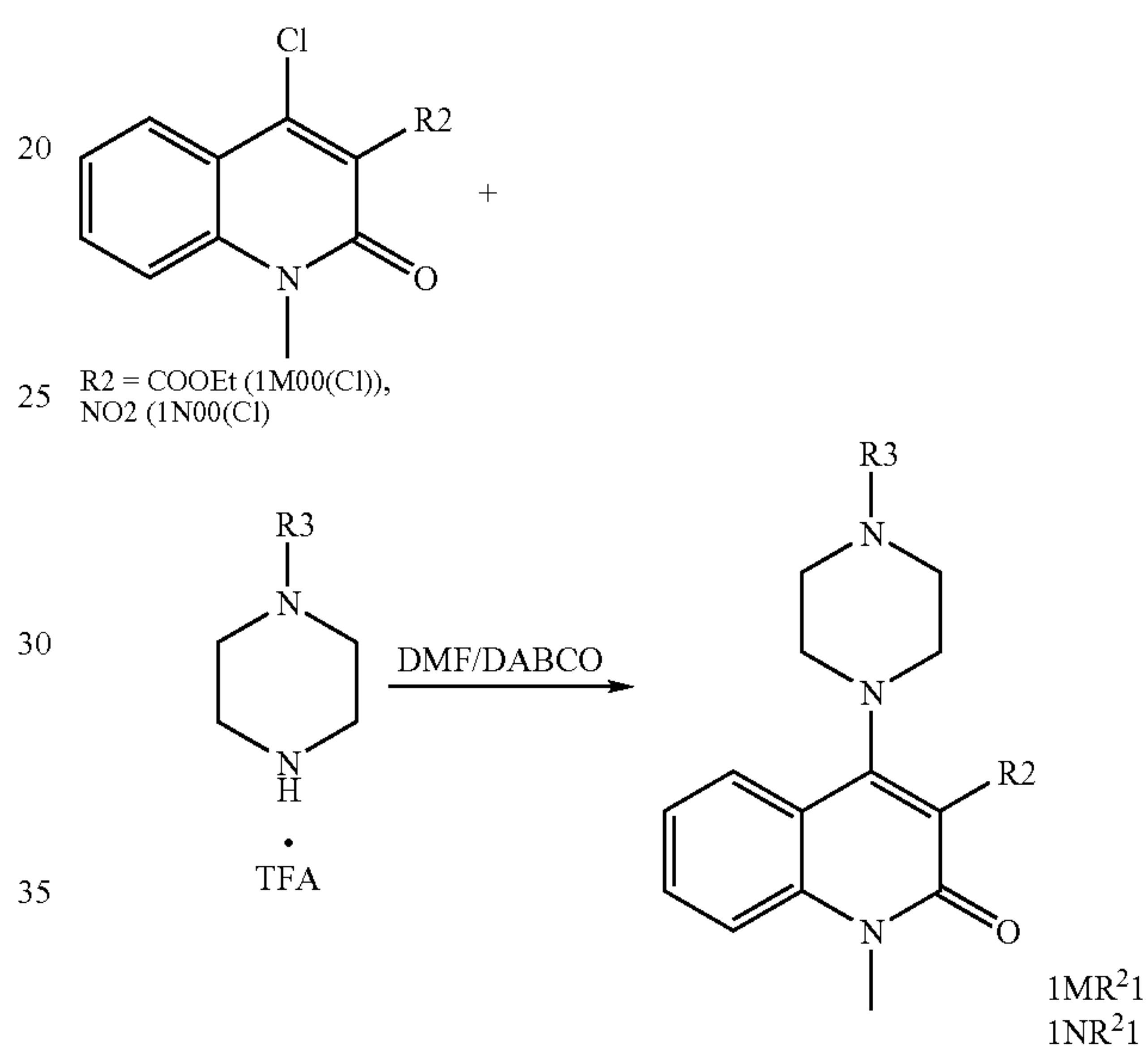
Reaction Scheme 16
