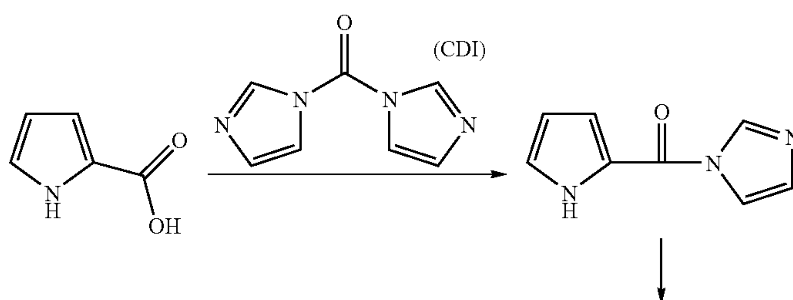
Reaction Scheme 17
