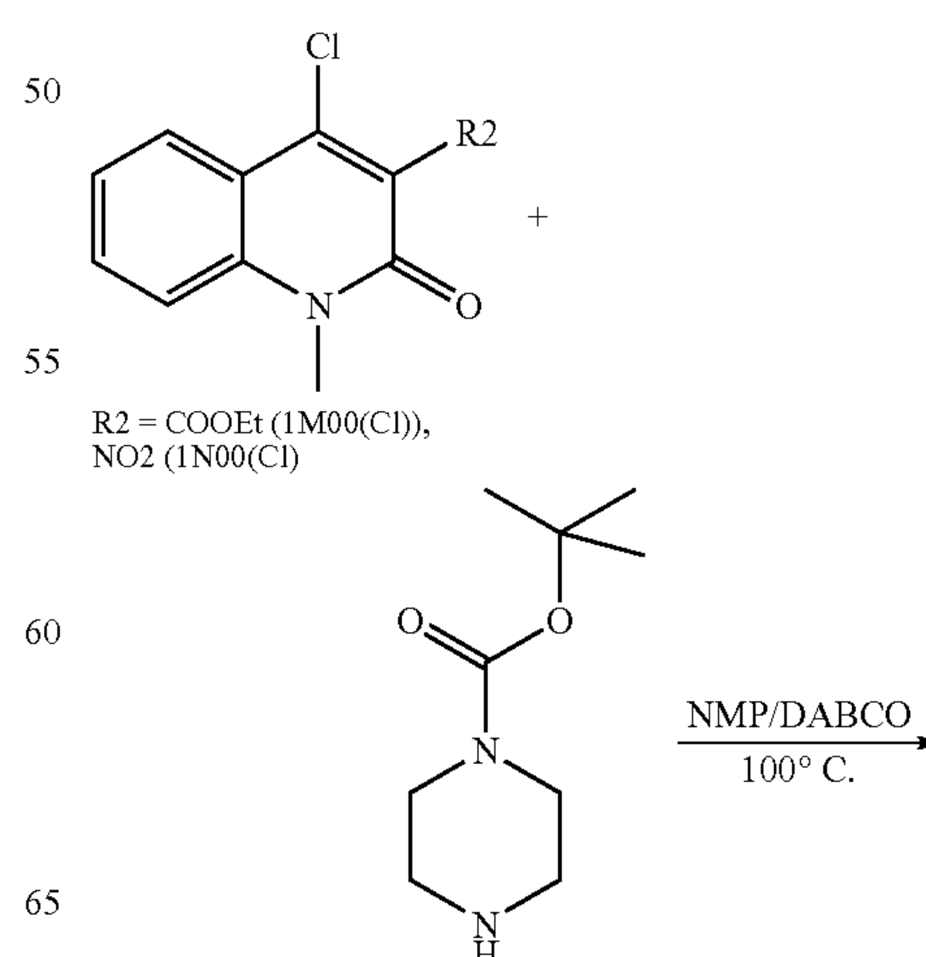
Reaction Scheme 15
