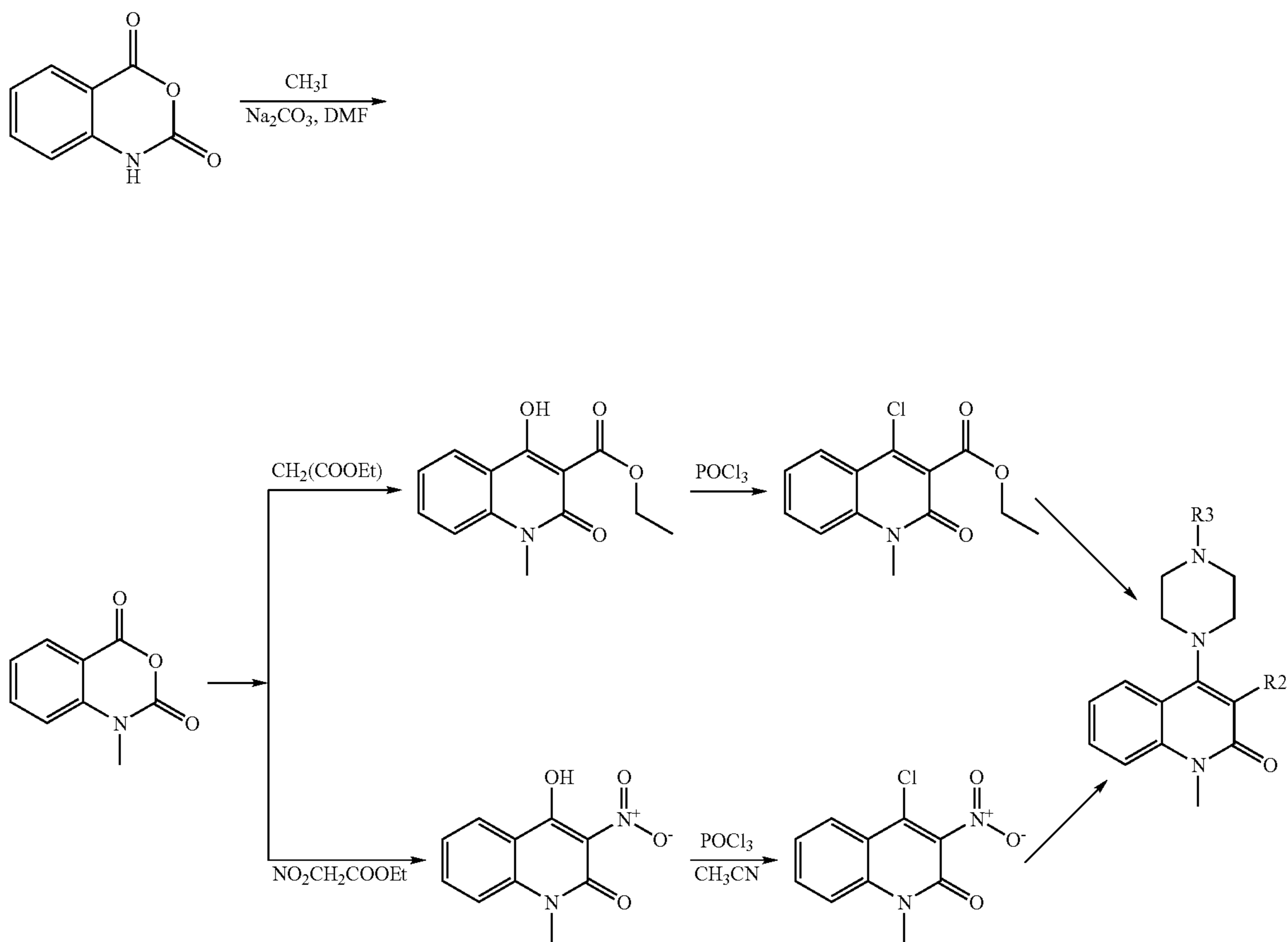
Reaction Scheme 9
