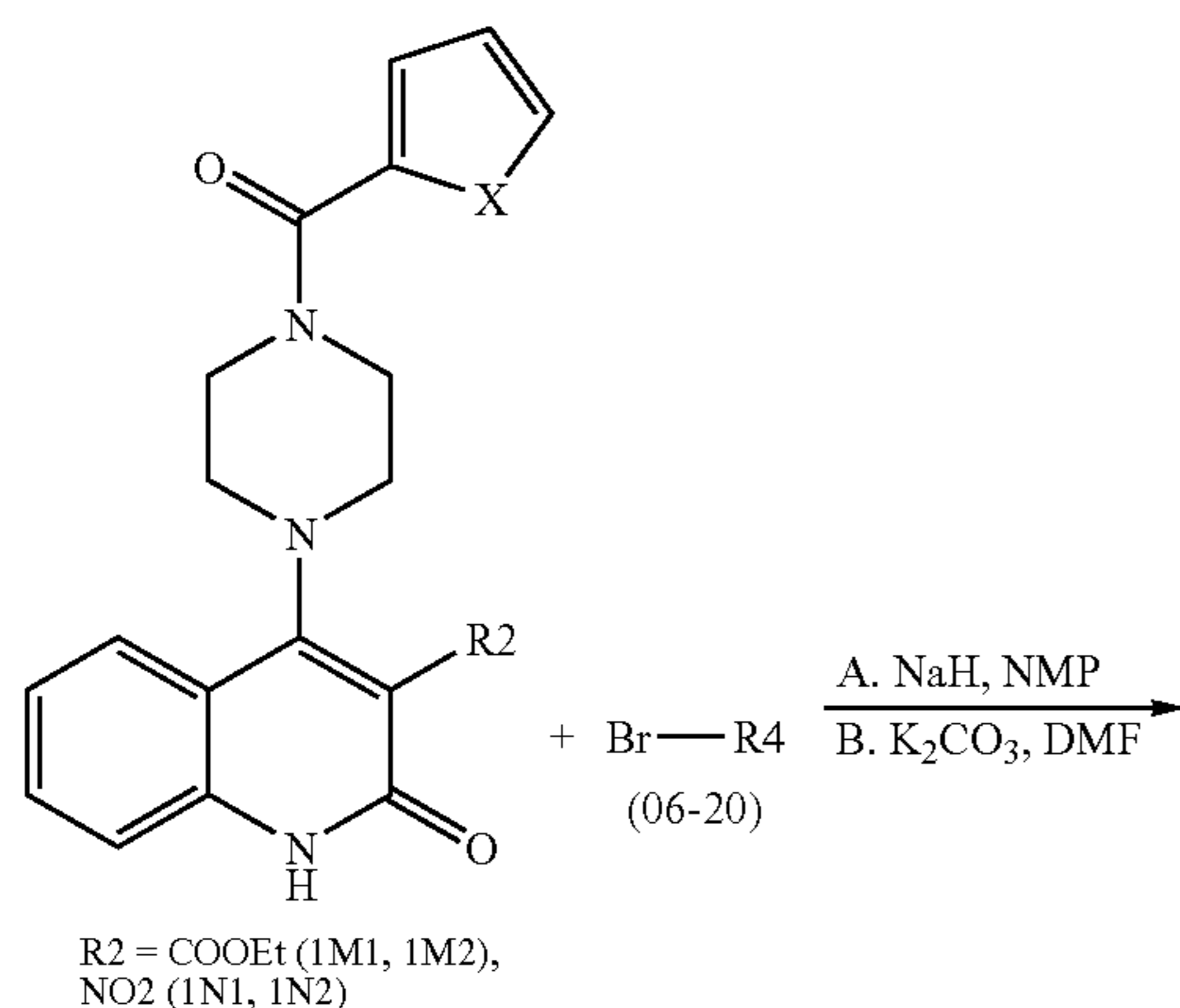
Reaction Scheme 13
