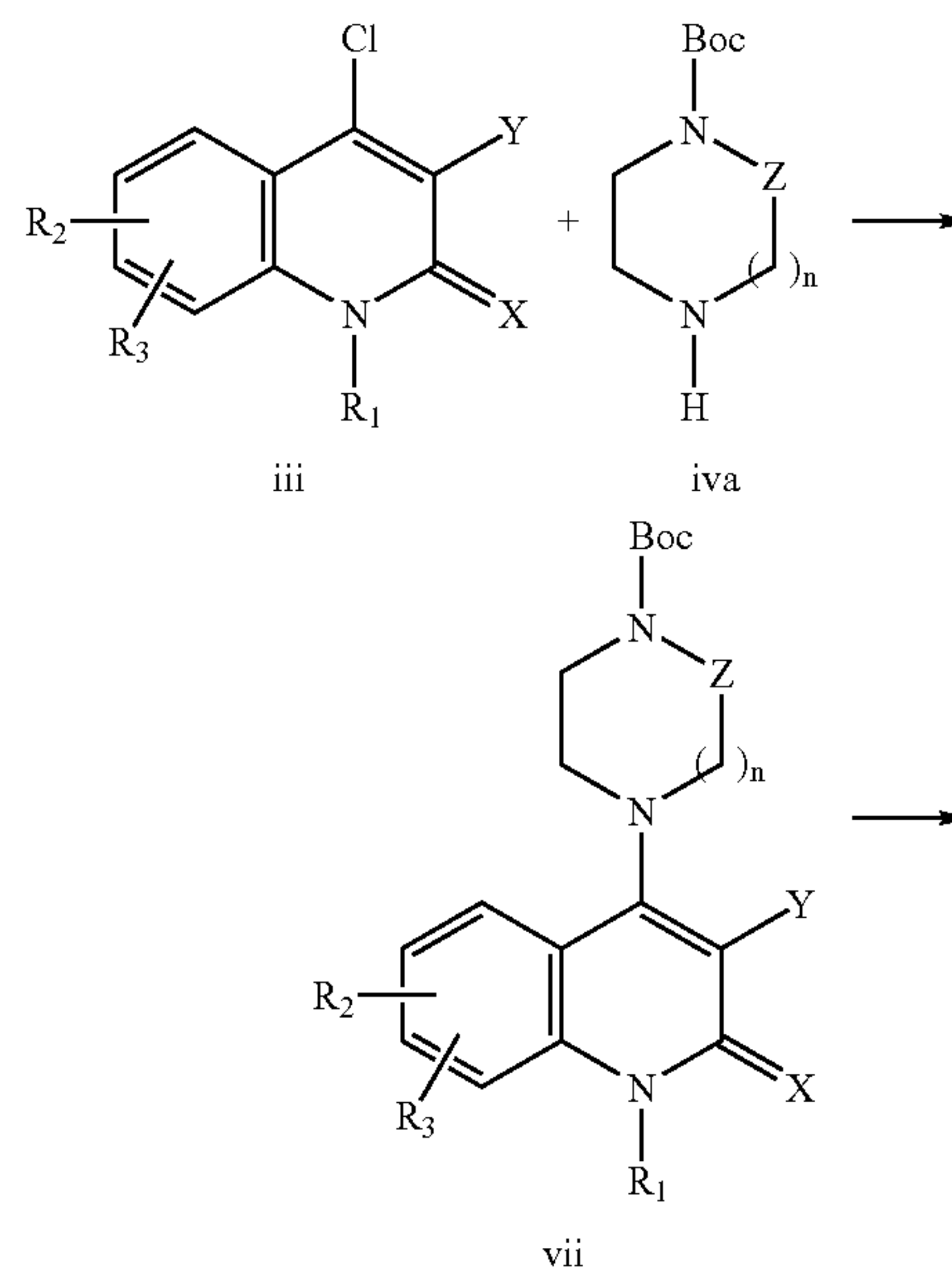
Reaction Scheme 4
