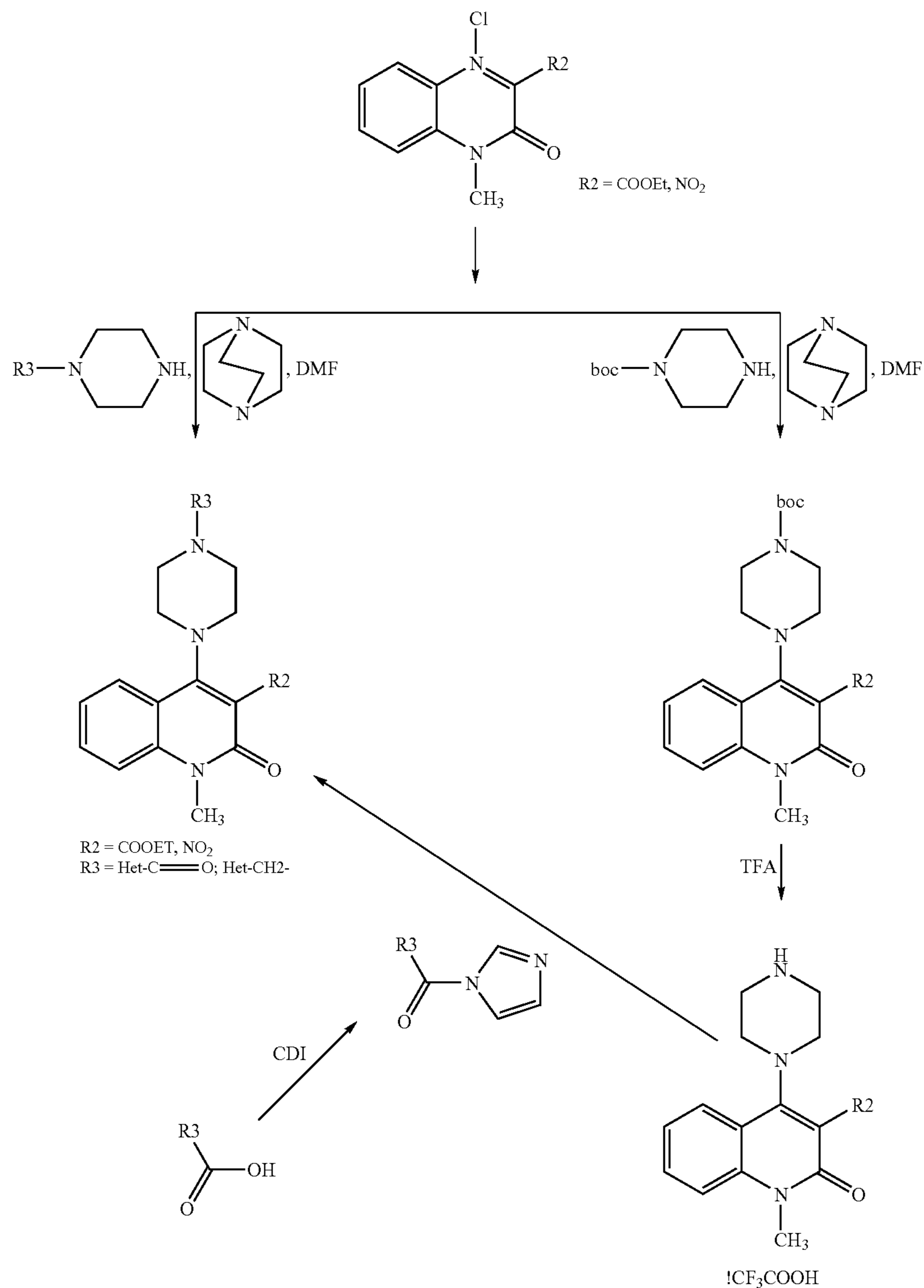
Reaction Scheme 10
