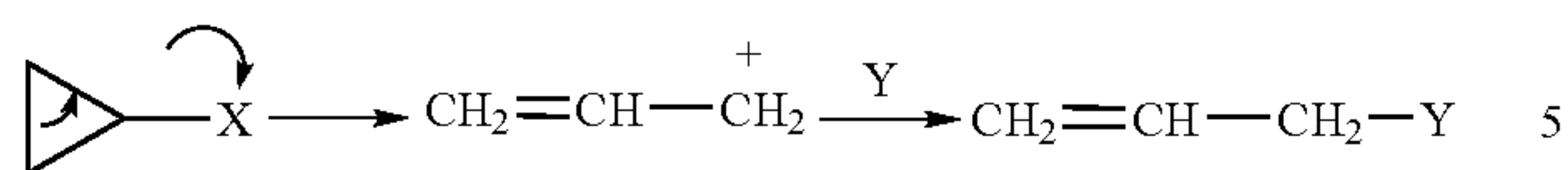
Reaction Scheme 7
