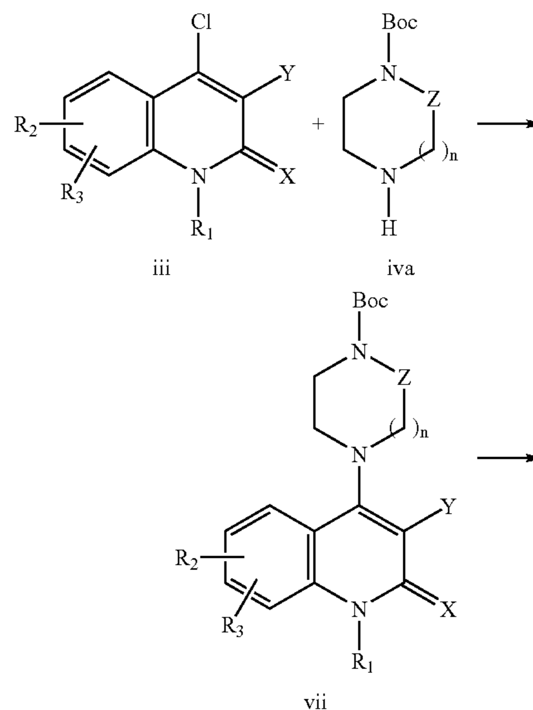
Reaction Scheme 4
