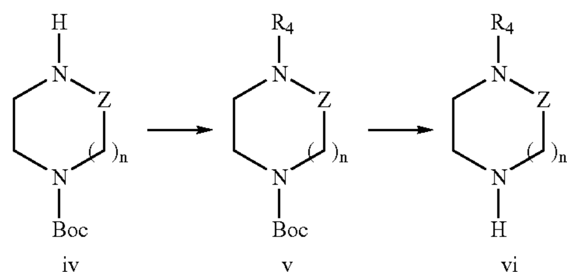
Reaction Scheme 2
