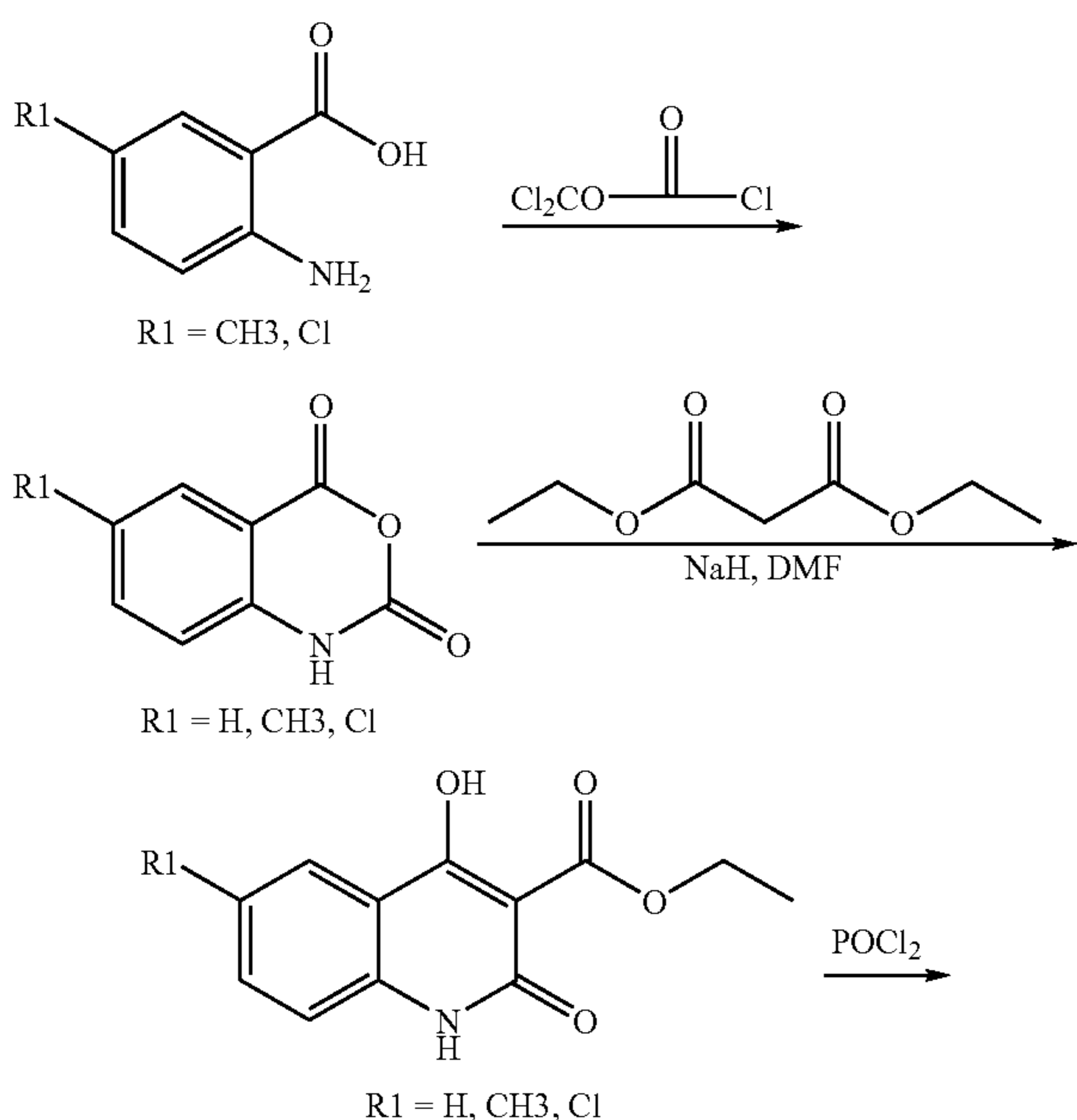
Reaction Scheme 21
