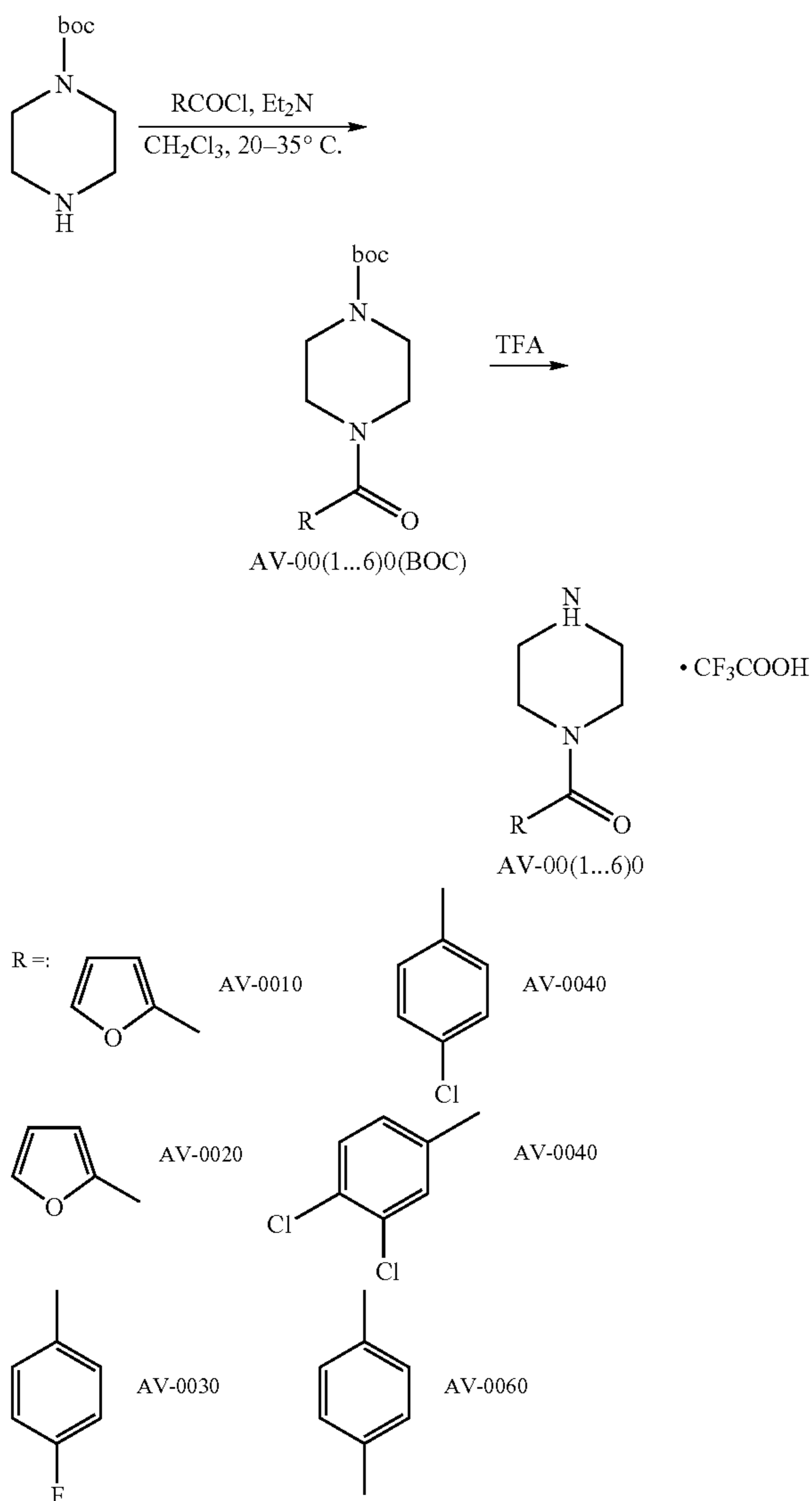
Reaction Scheme 23
