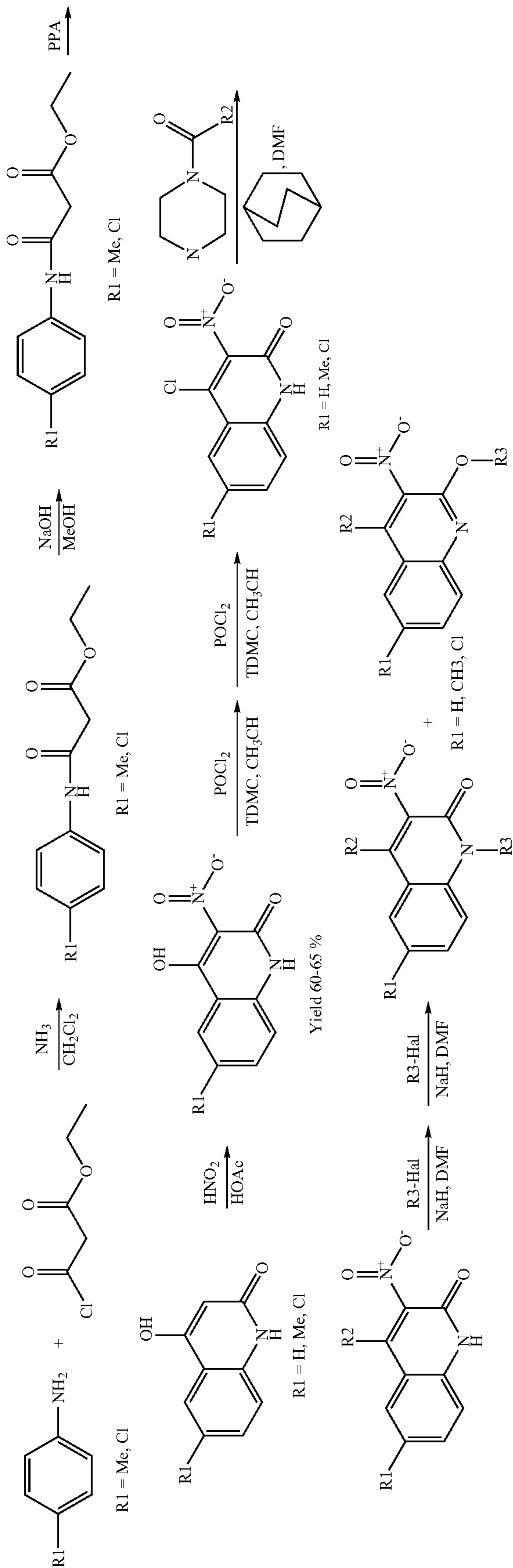
Reaction Scheme 22
