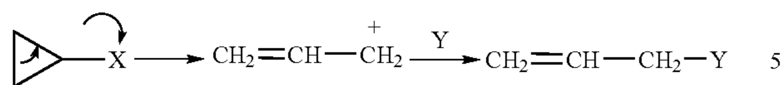
Reaction Scheme 7
