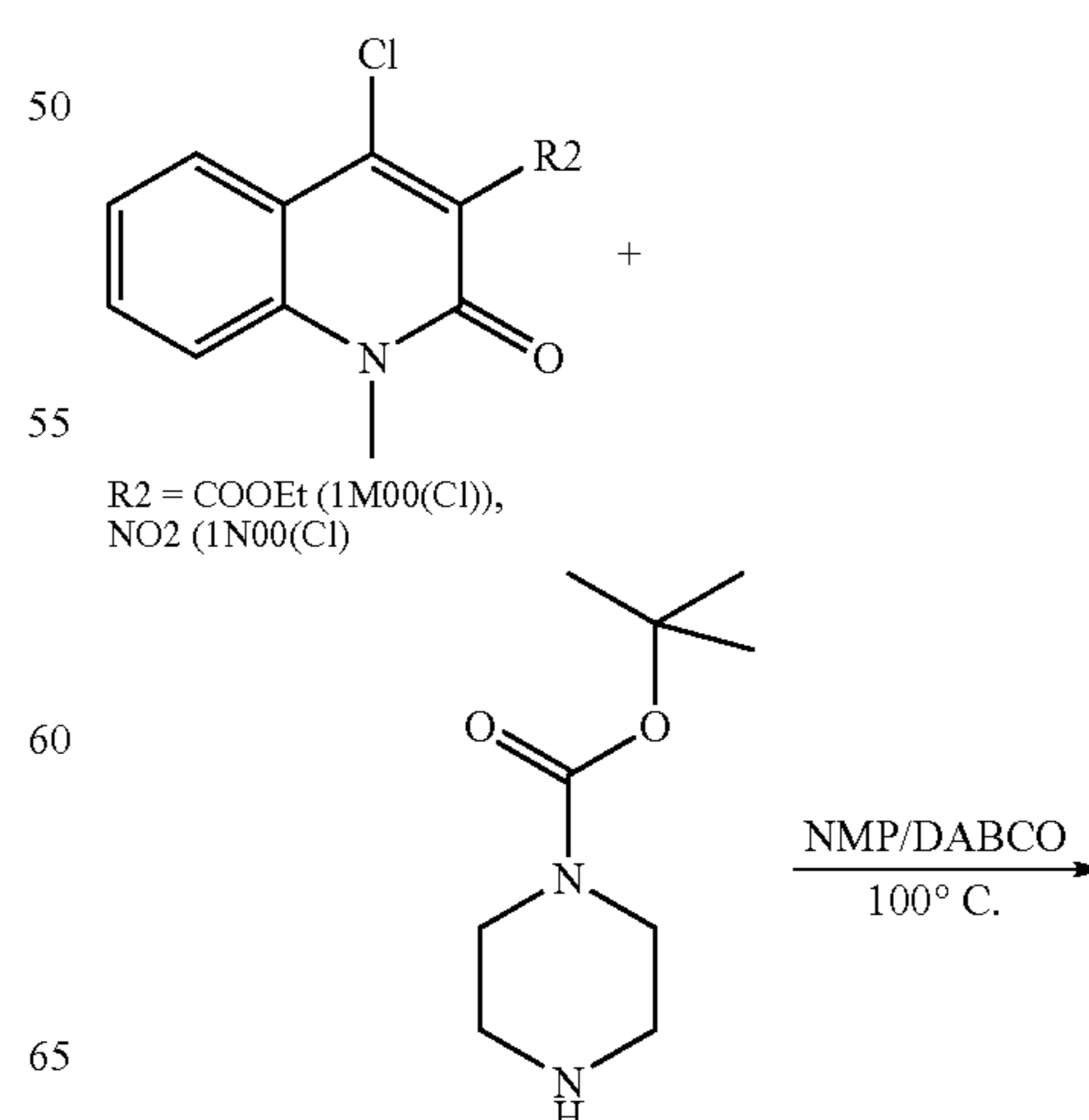
Reaction Scheme 15
