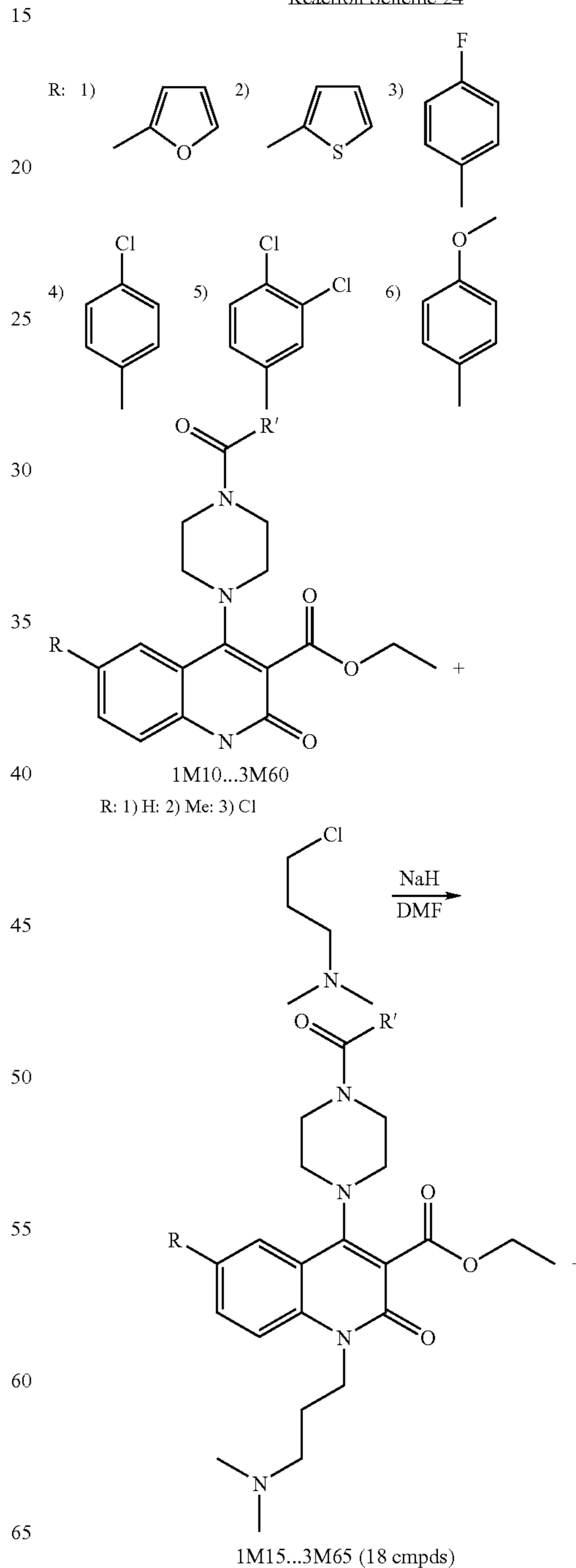
Reaction Scheme 24
