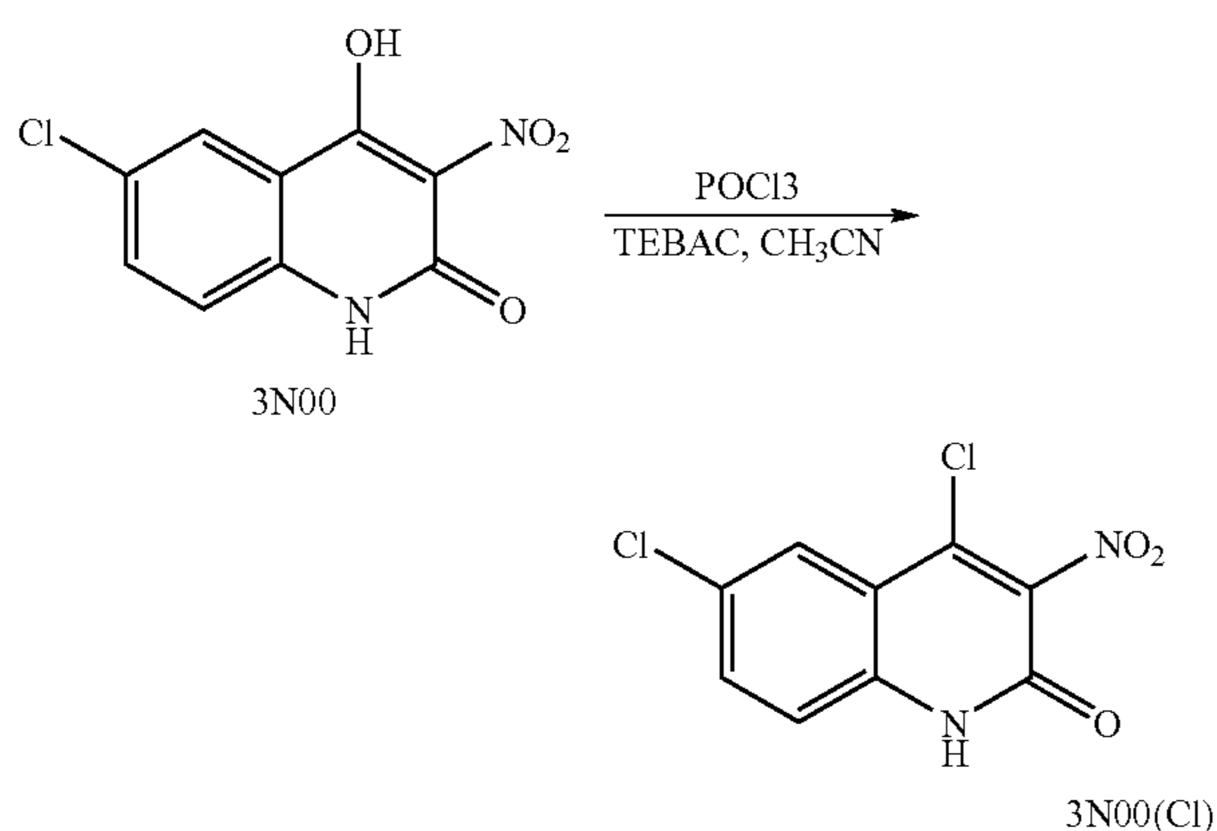
Reaction Scheme 27
