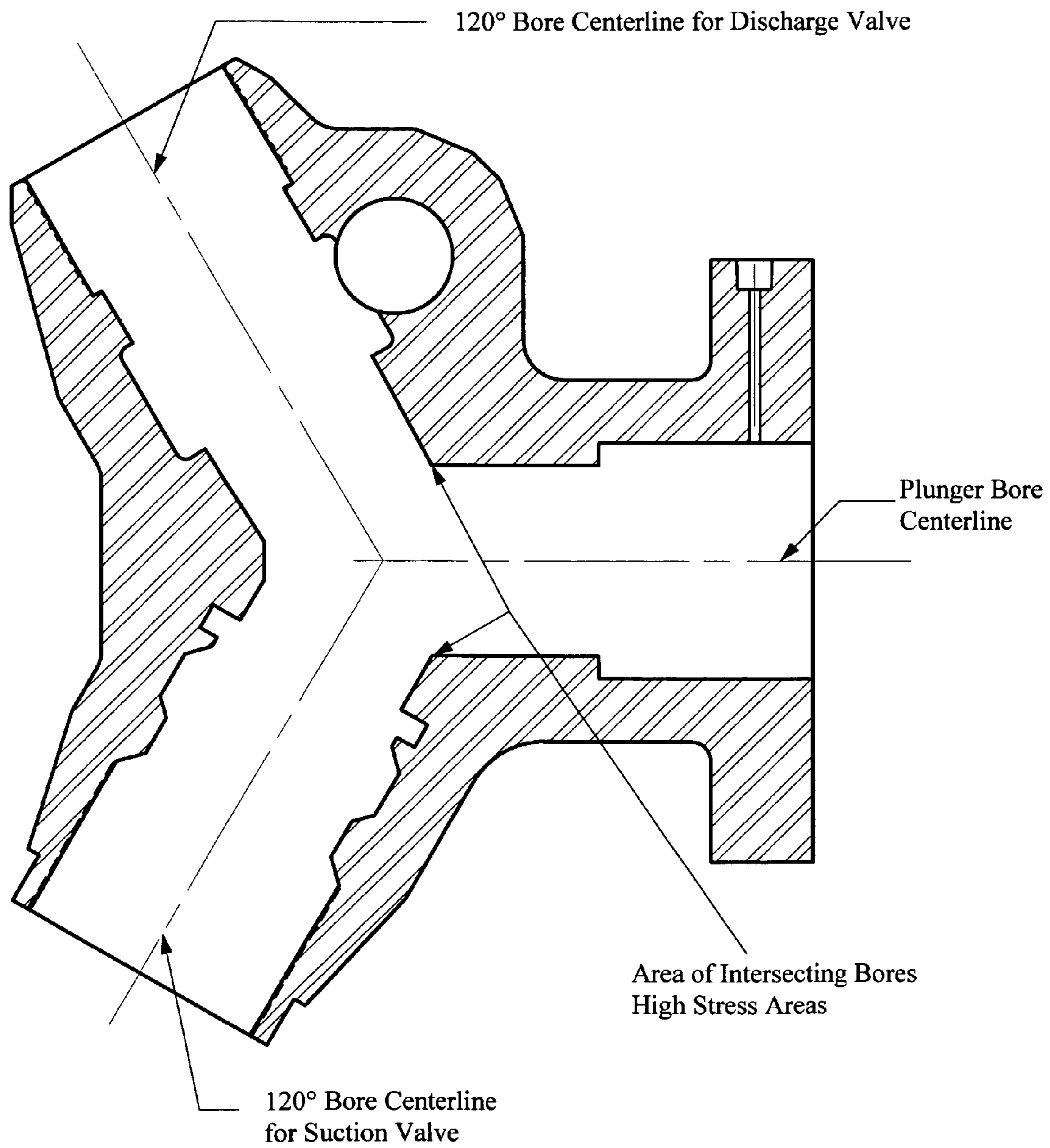
Y-Block Plunger Pump Housing
