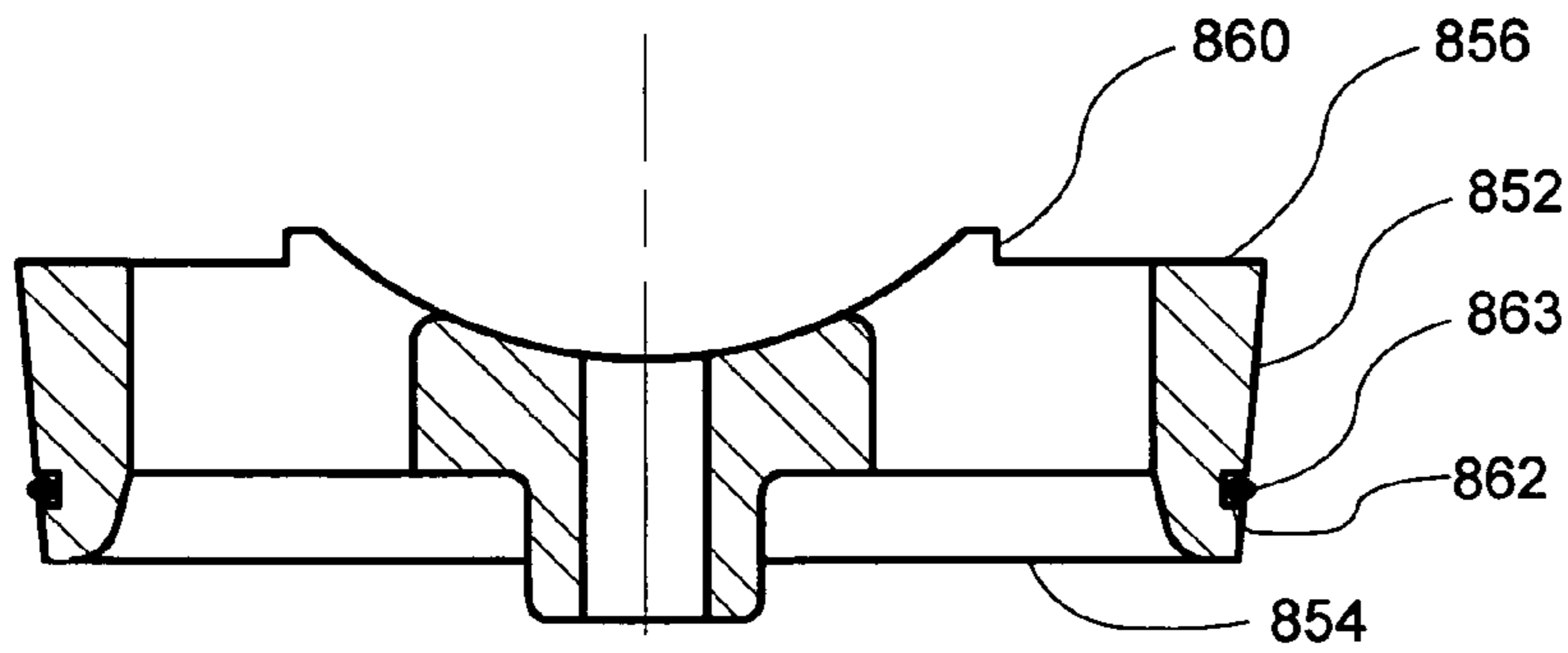
(Section C-C of Figure 11A)
