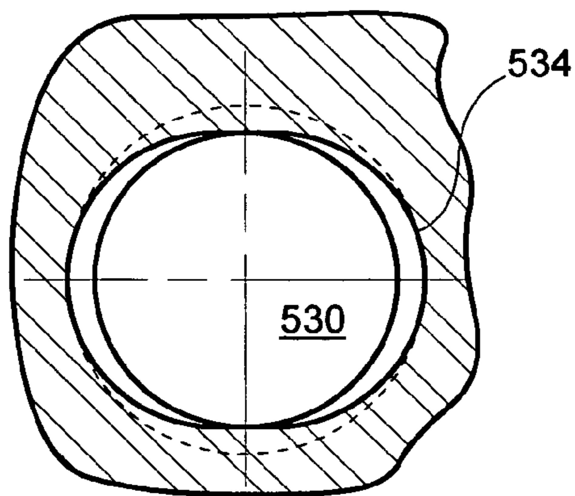
(Section D-D of Figure 7A) Figure 7D
