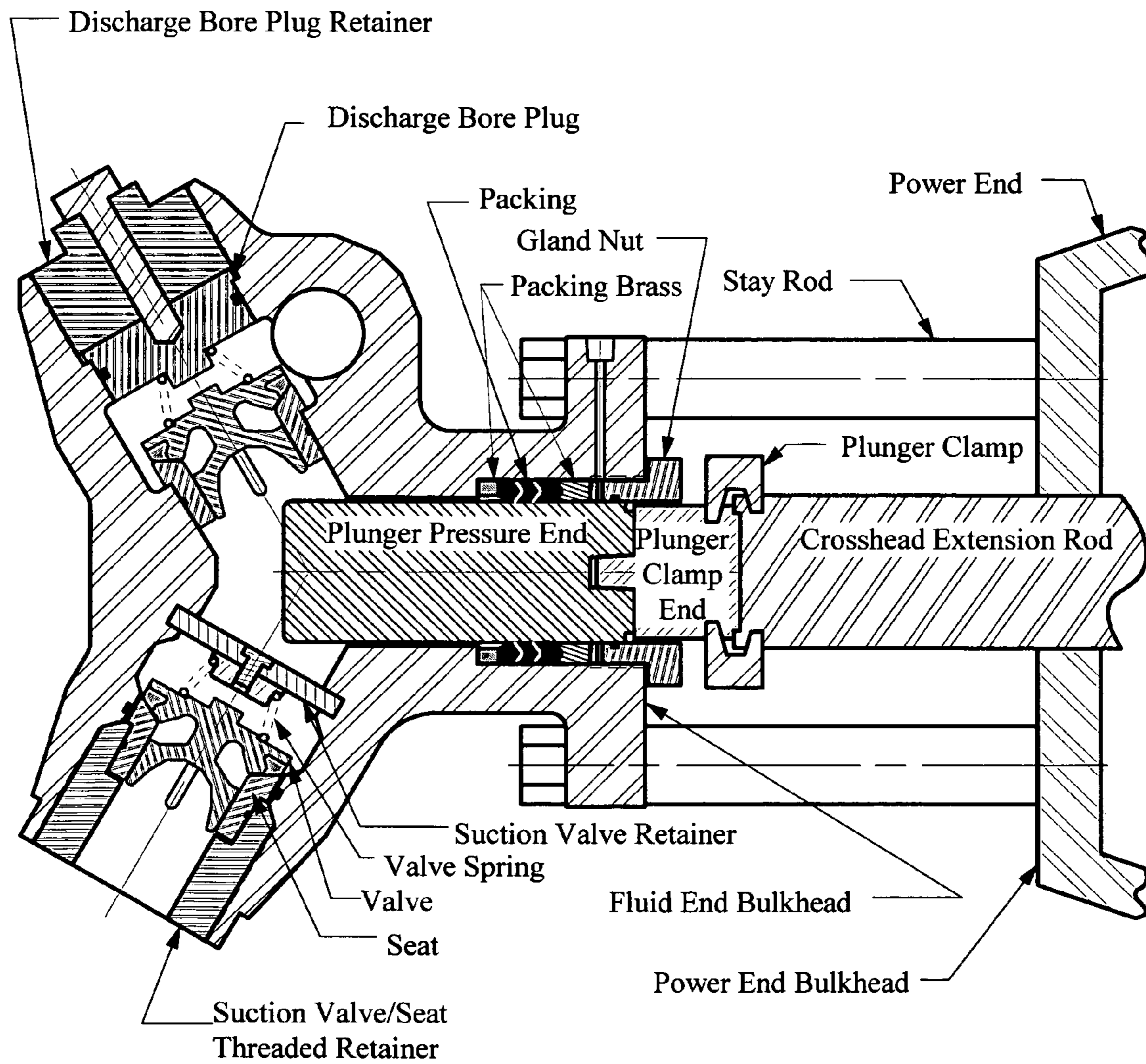
Y-Block Fluid Section
