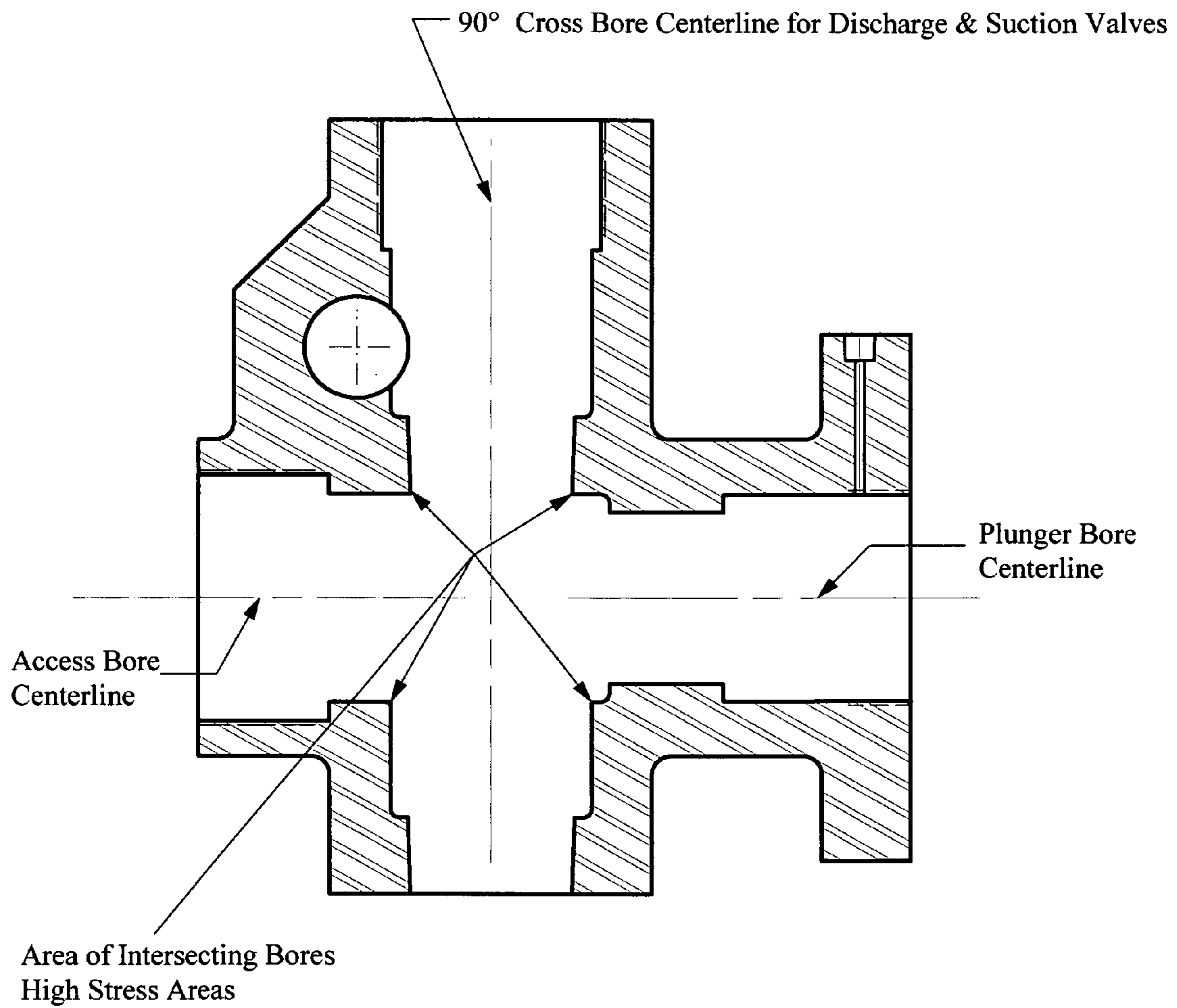
Conventional Plunger Pump Housing
