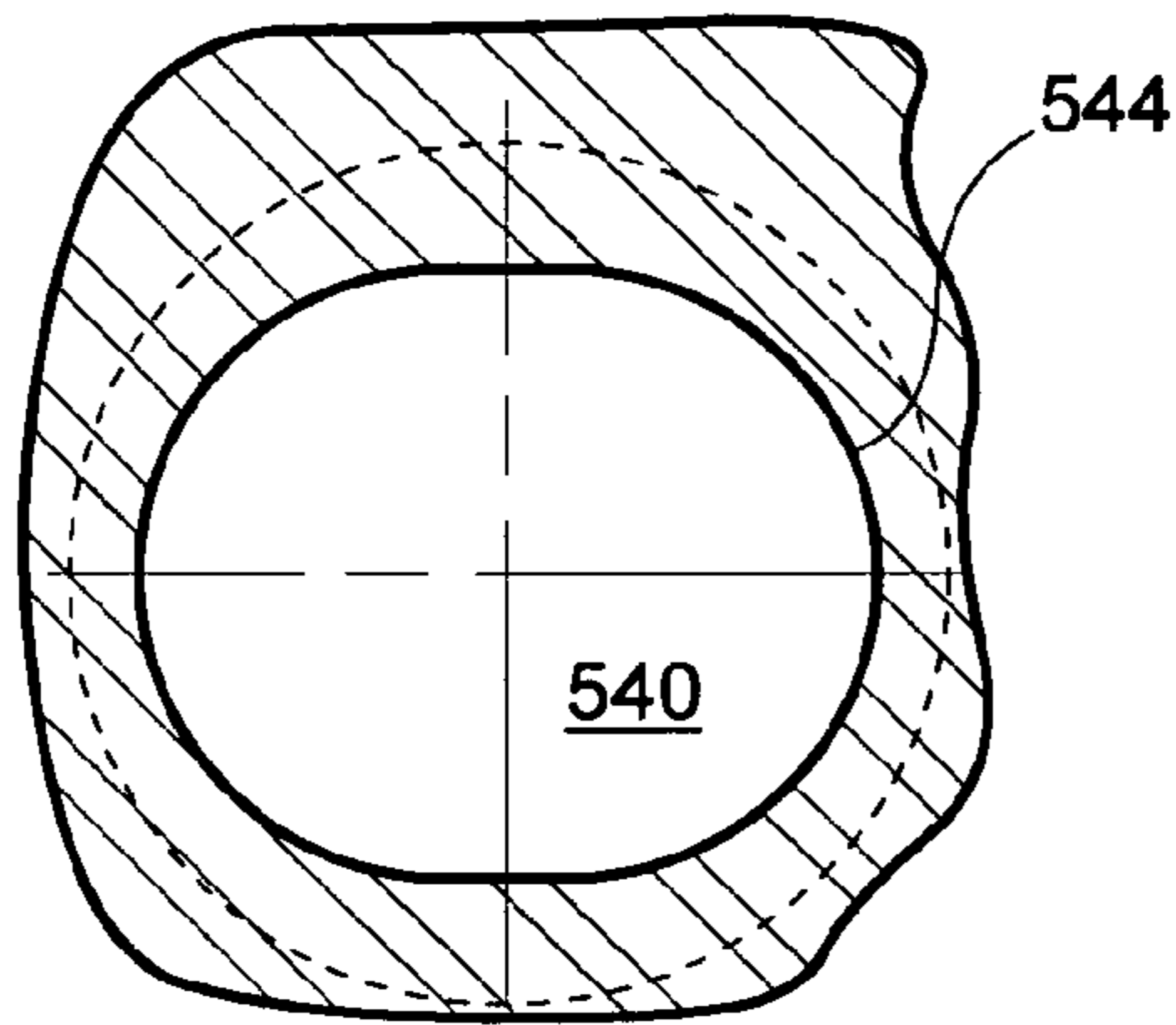
(Section B-B of Figure 7A) Figure 7B
