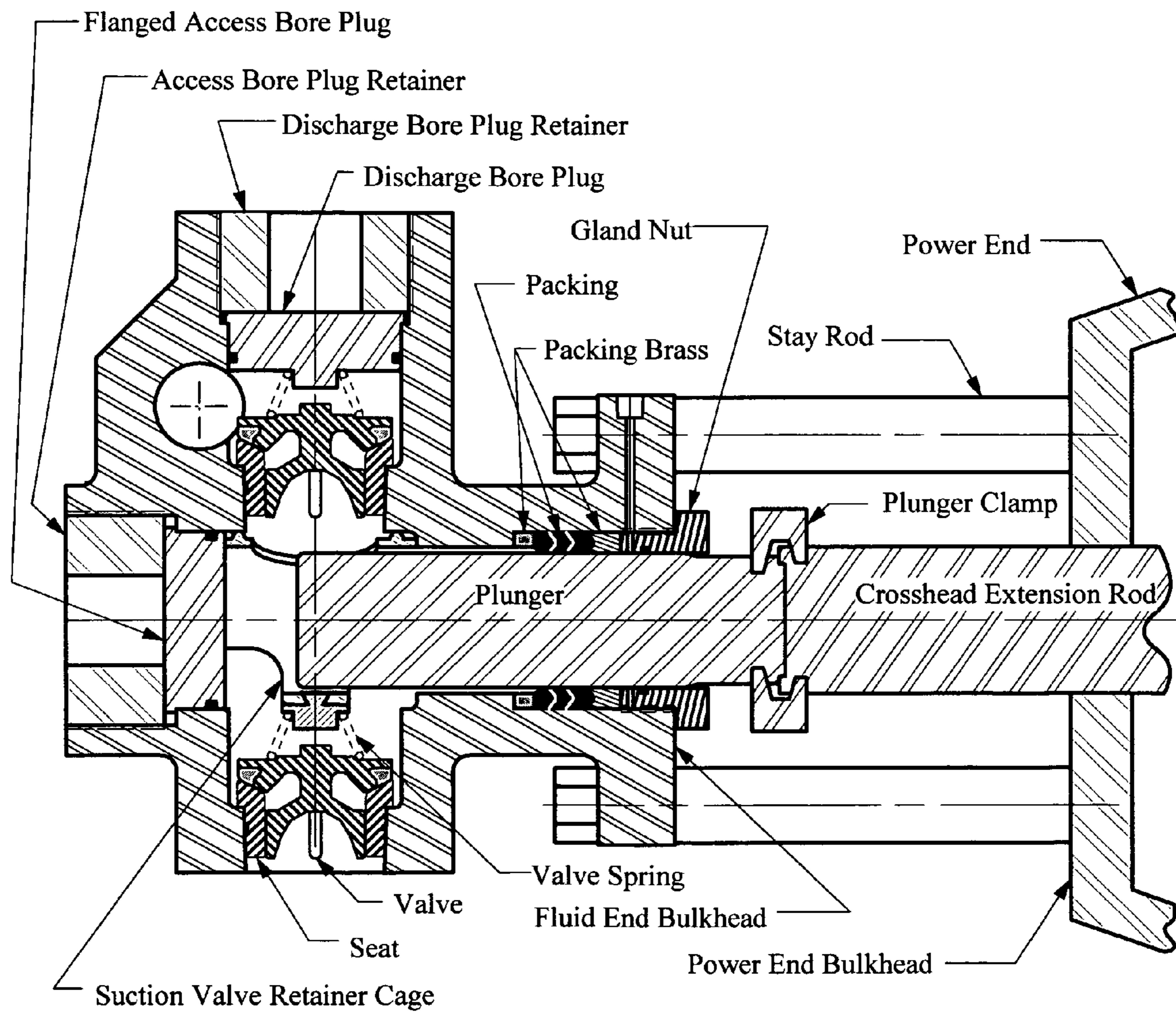
Typical Fluid Section Figure 1
