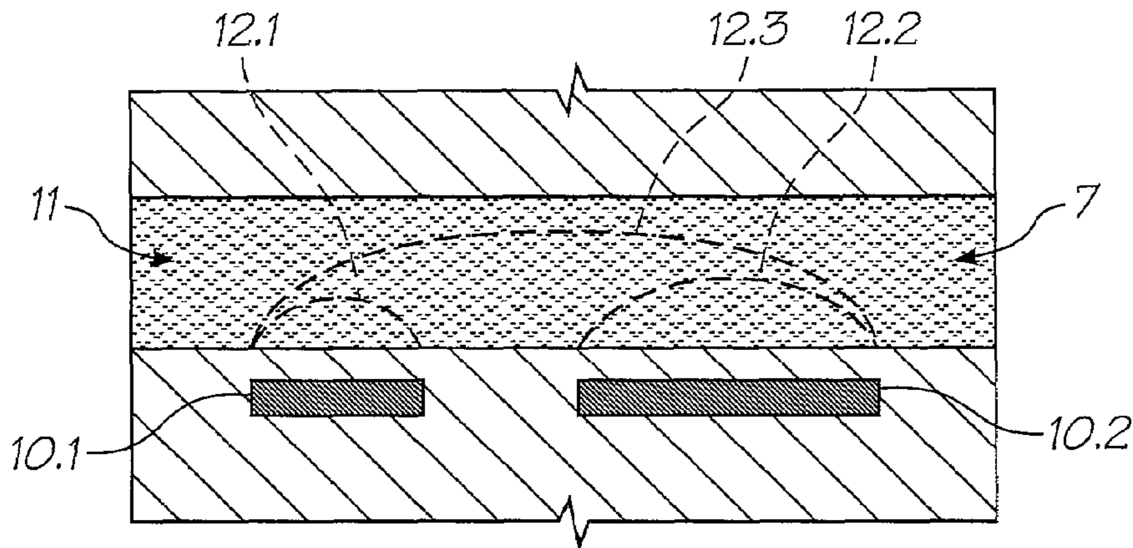
FIG. 52 (PRIOR ART)
