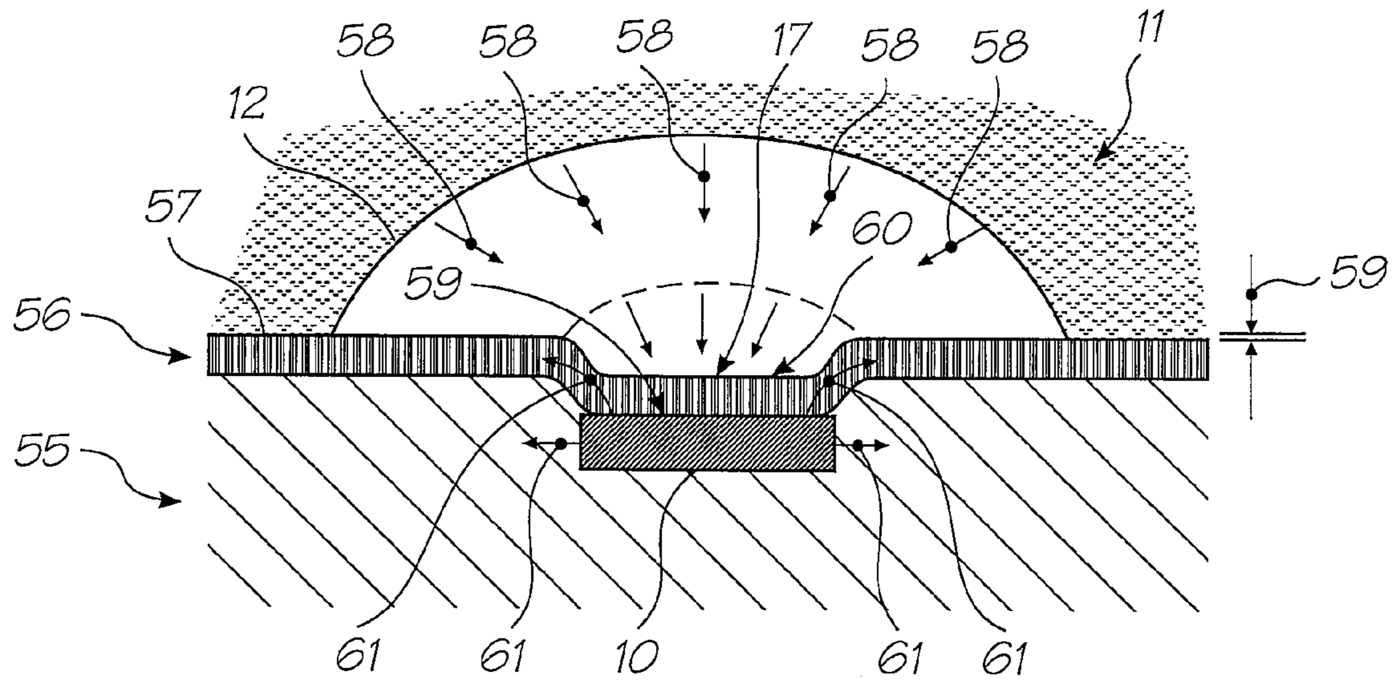
FIG. 47 (PRIOR ART)
