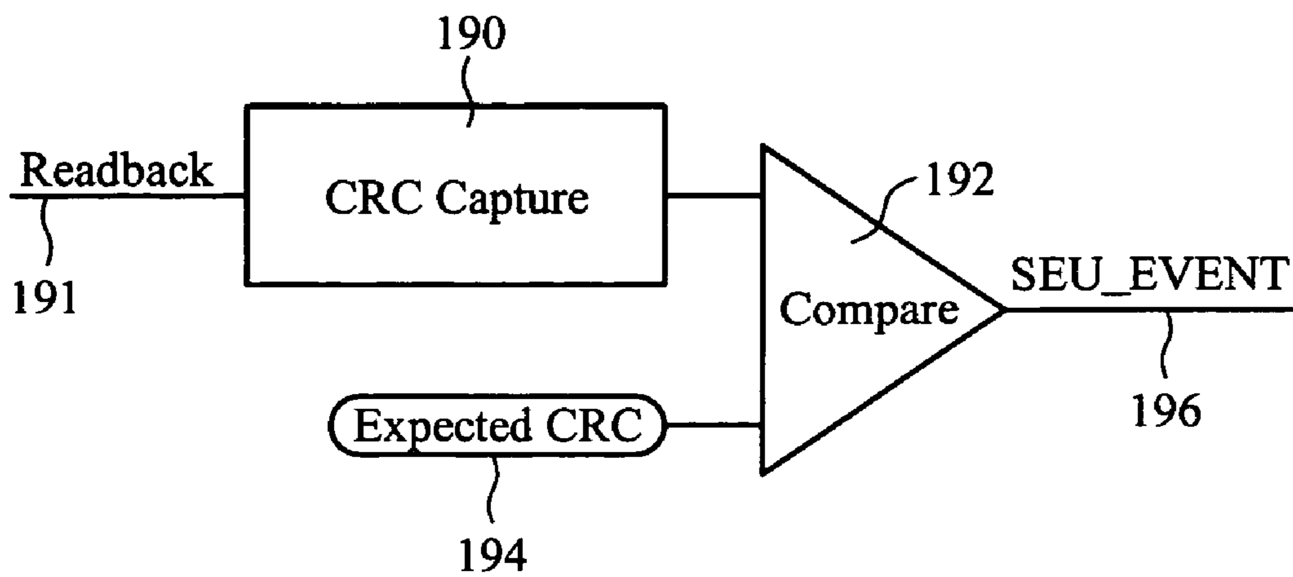
Readback CRCComparator
