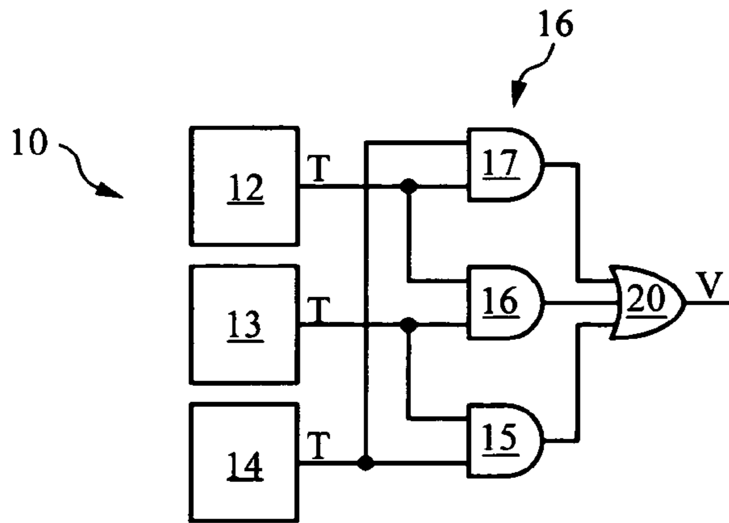
Triple Redundancy with Voting
