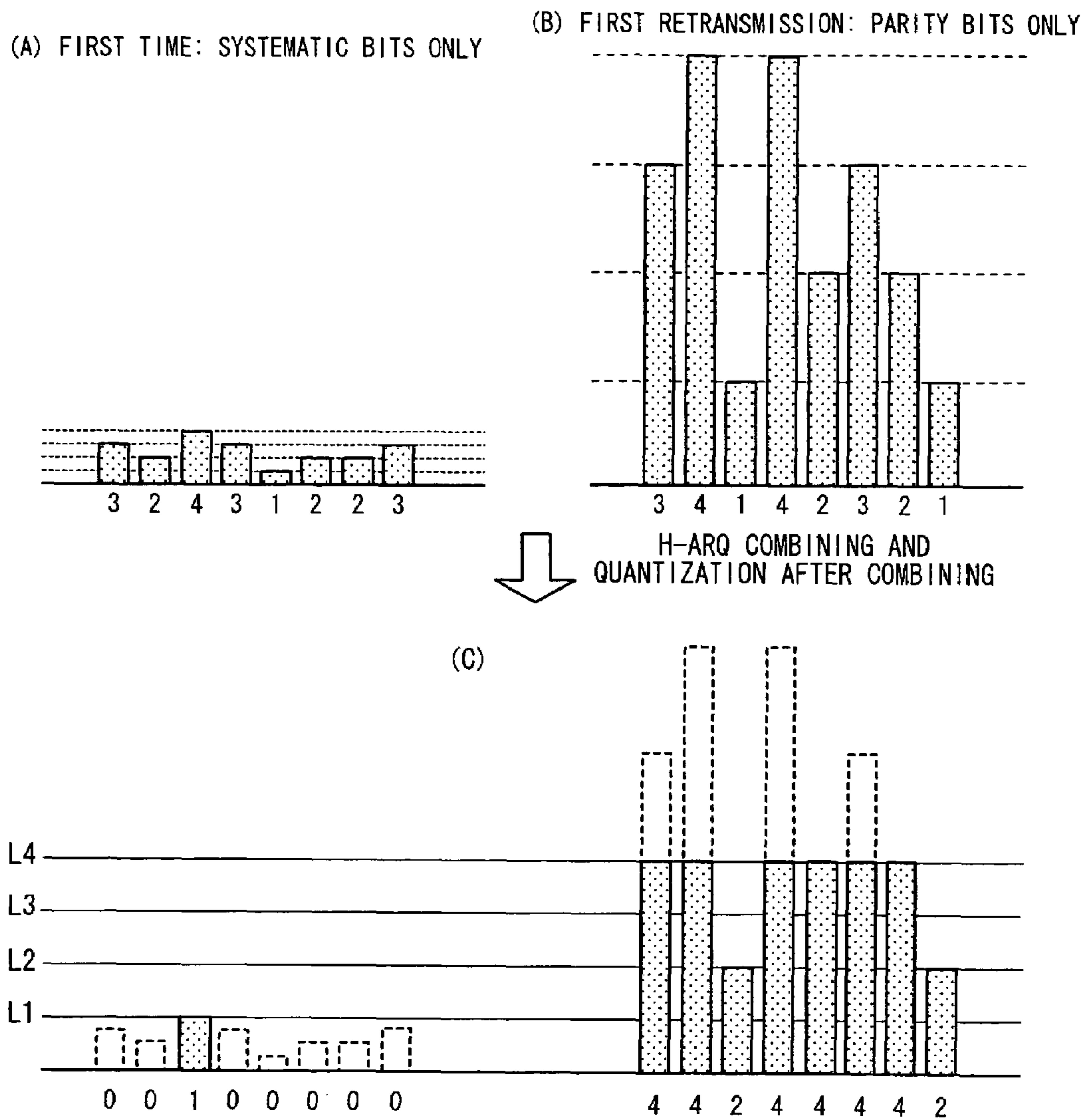
FIG. 29 PRIOR ART
