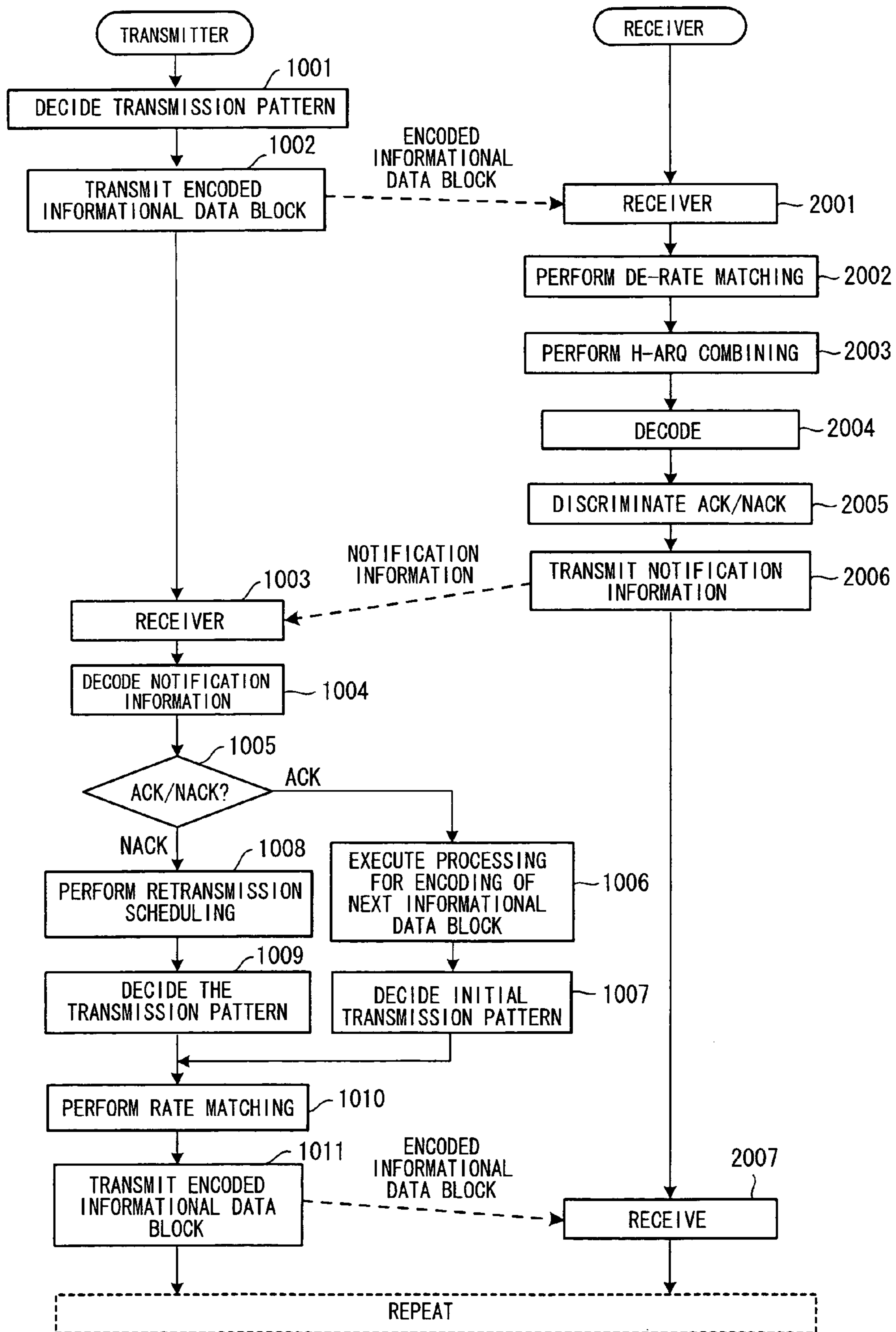
FIG. 30 PRIOR ART
