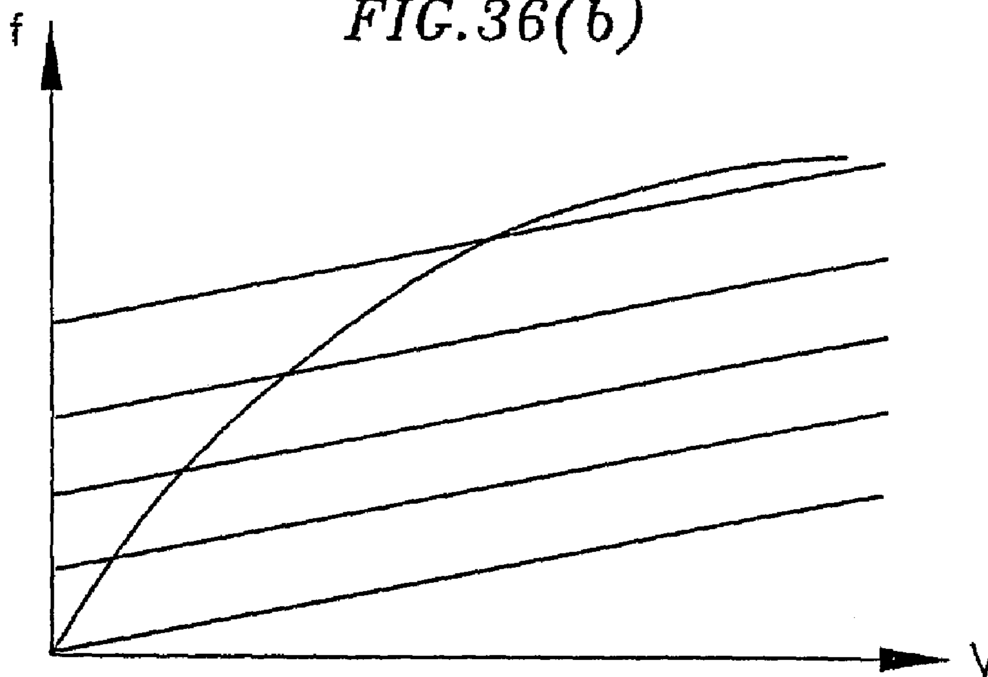
SEGMENTED VCO TUNING CURVE
