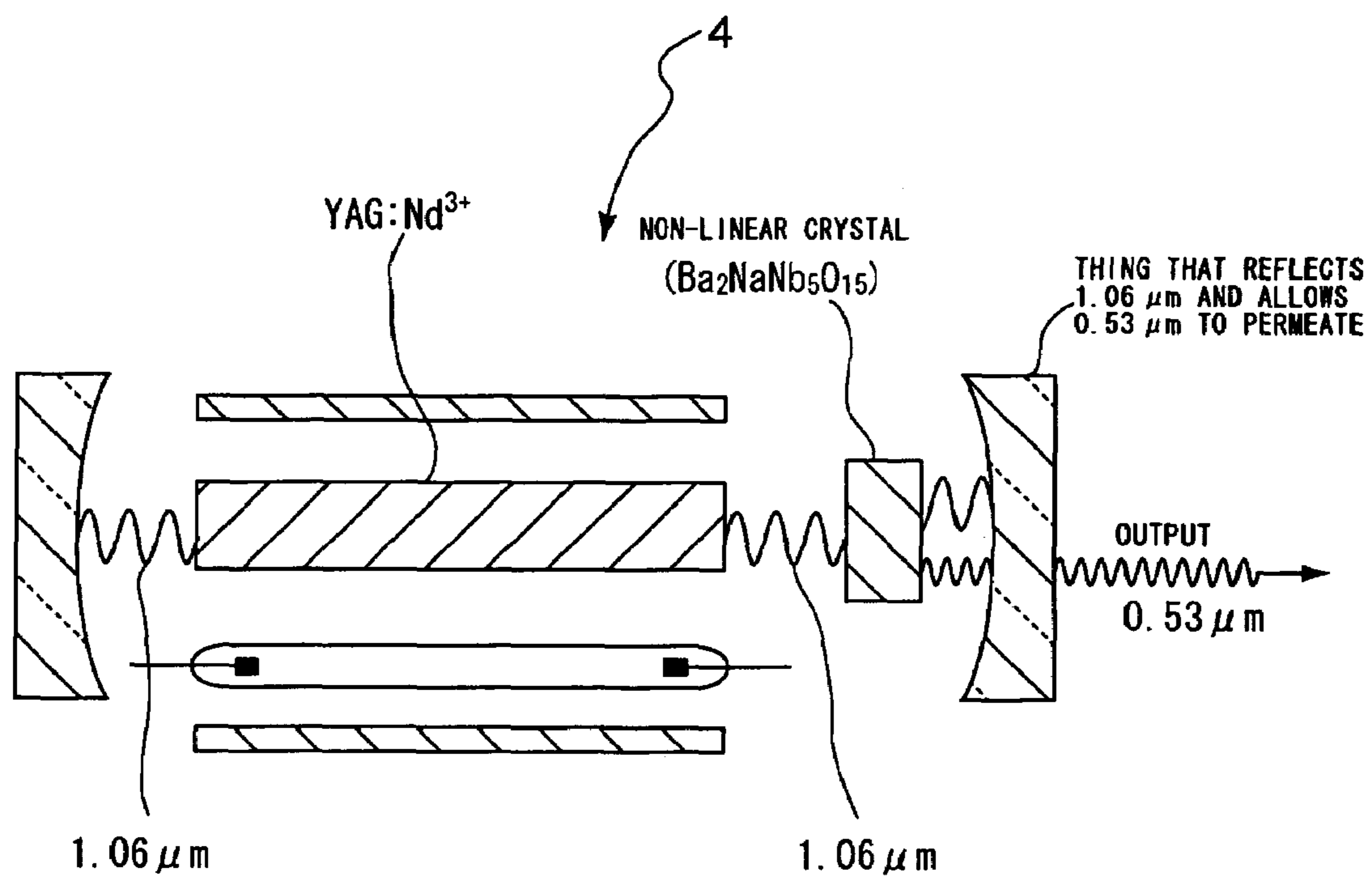
CONSTITUTION OF HARMONICS OSCILLATING SOLID LASER USING NON-LINEAR CRYSTAL (OUTPUT OF GREEN 0.53 μm)
