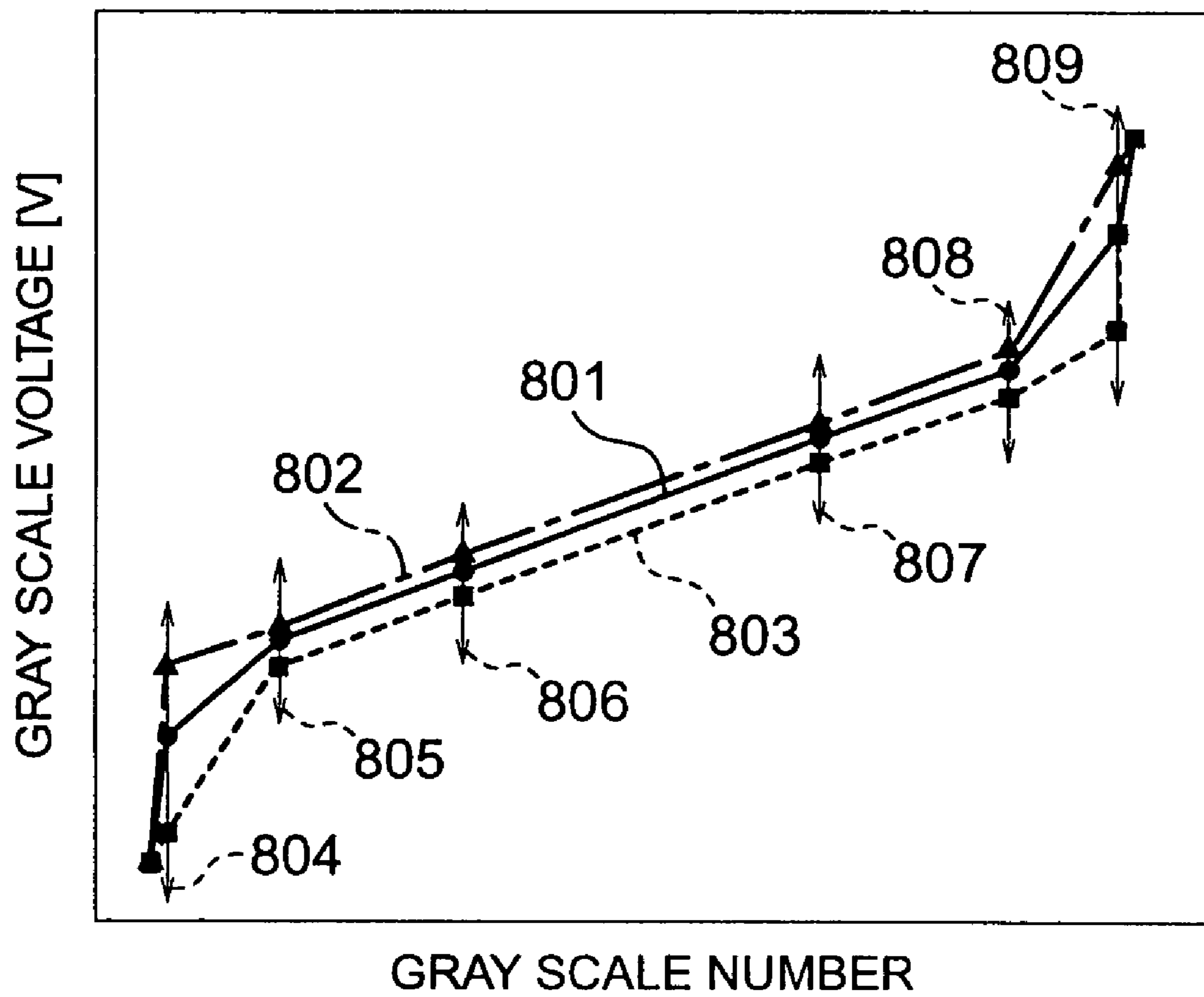
EFFECT OF MICRO ADJUSTMENT REGISTER
