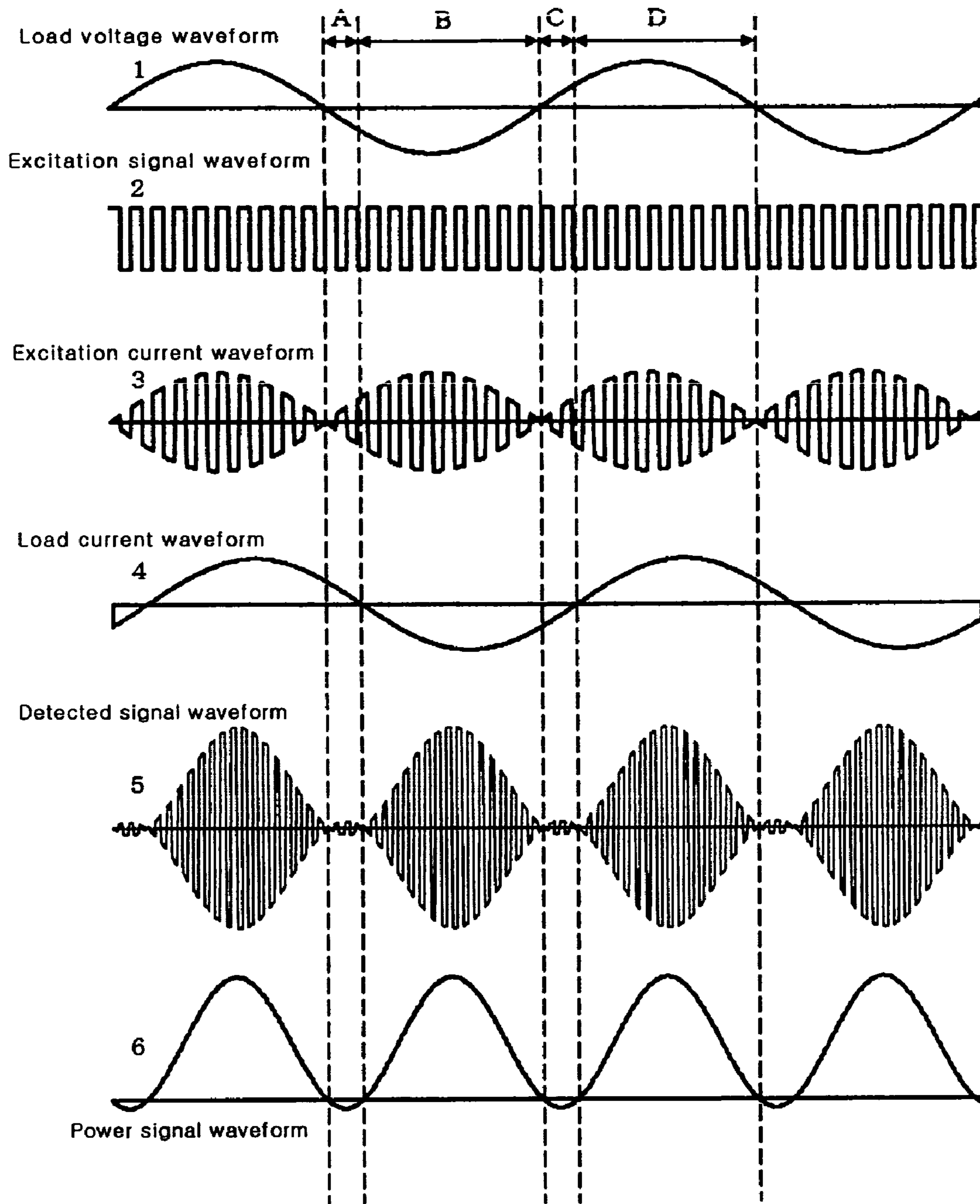
Waveforms explaining operations of power sensor according to claim 2 of the present invention
