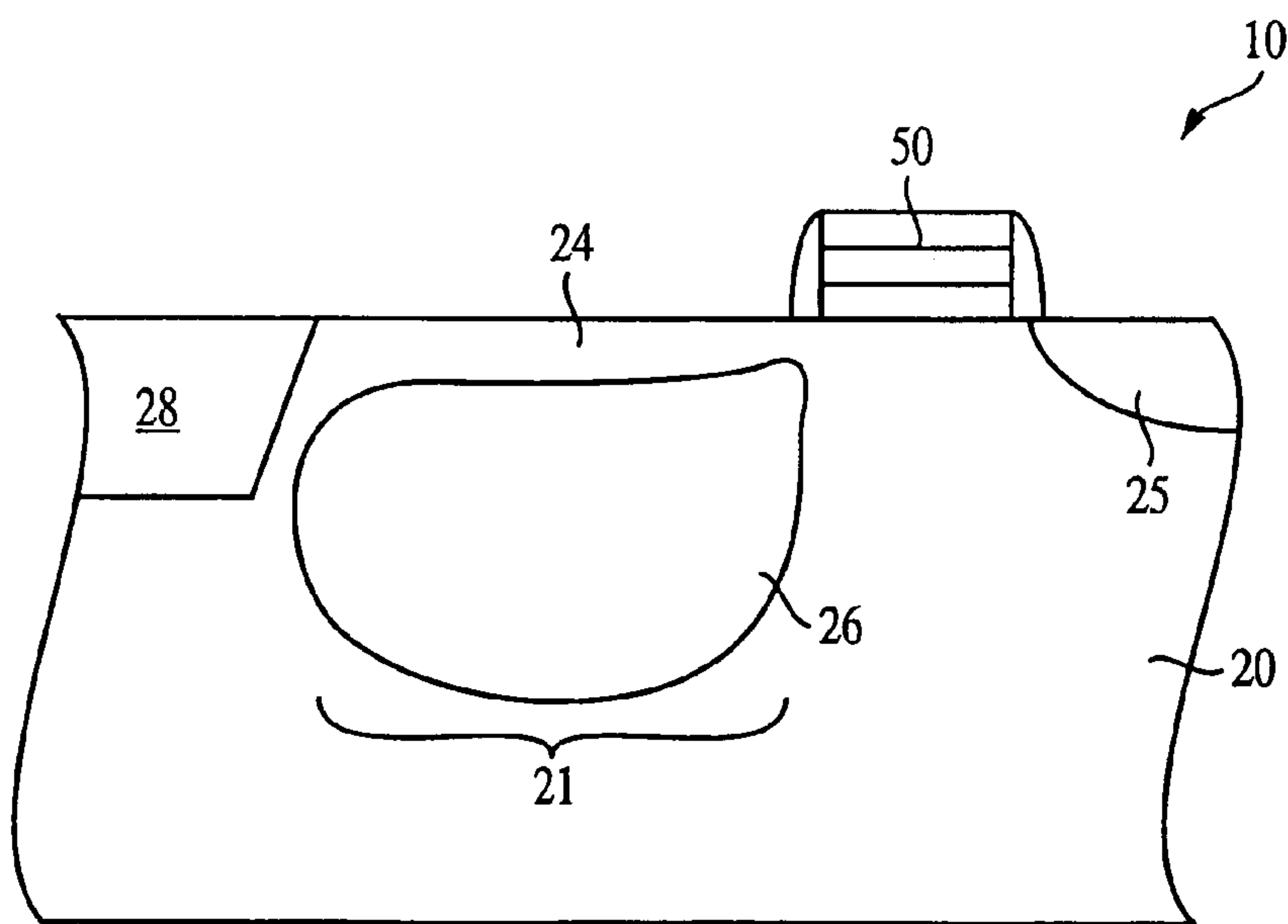
FIG. 2 PRIOR ART
