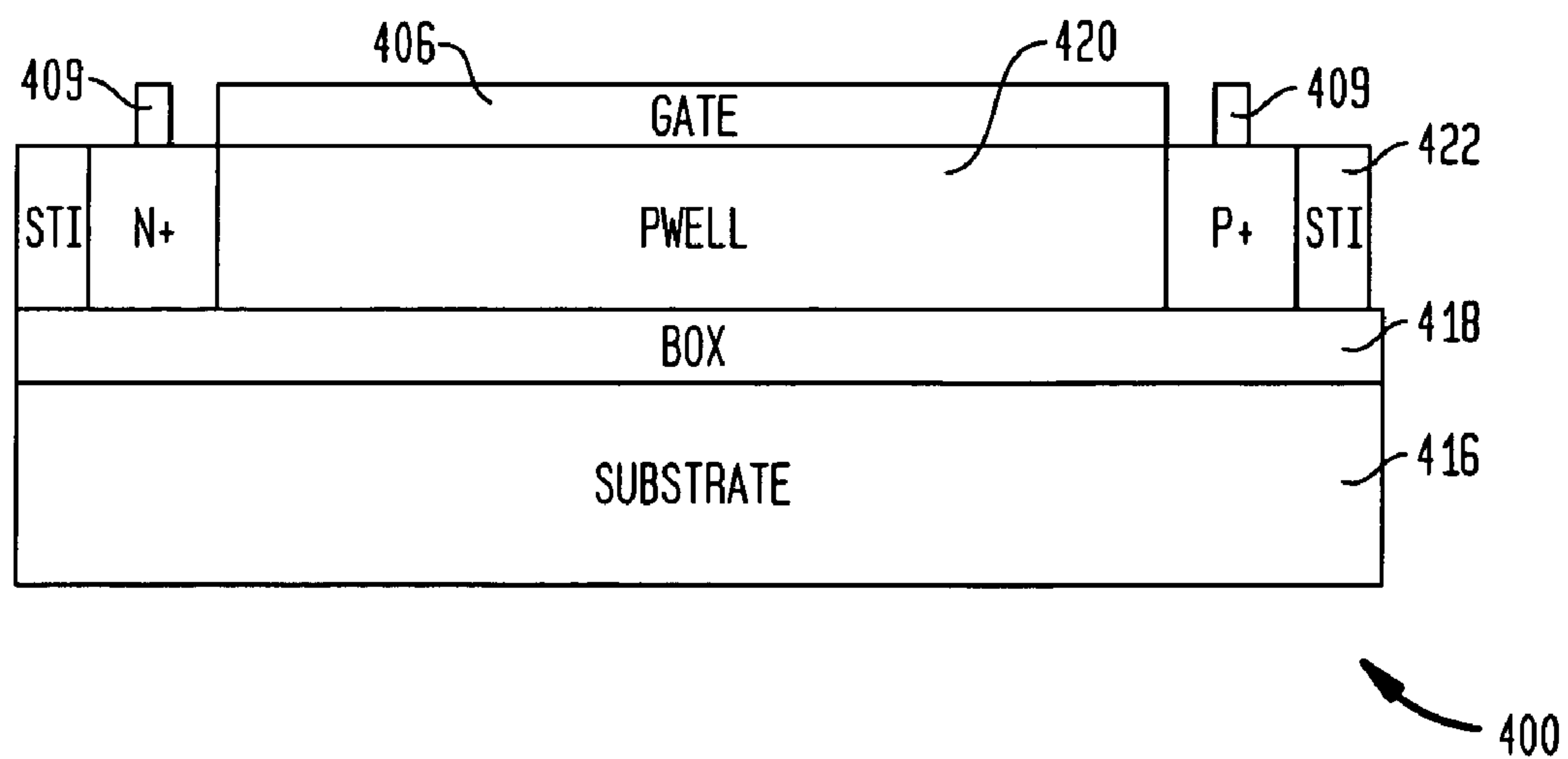
FIG. 4D CROSSECTION C
