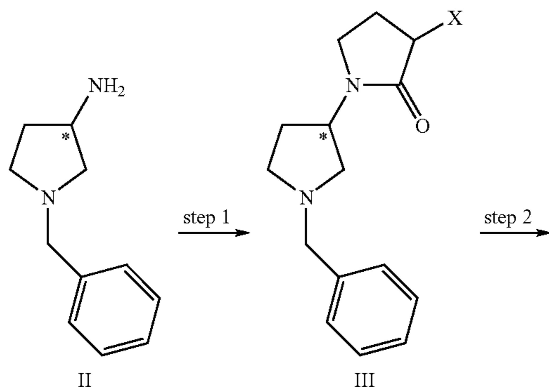
Reaction scheme 1:
