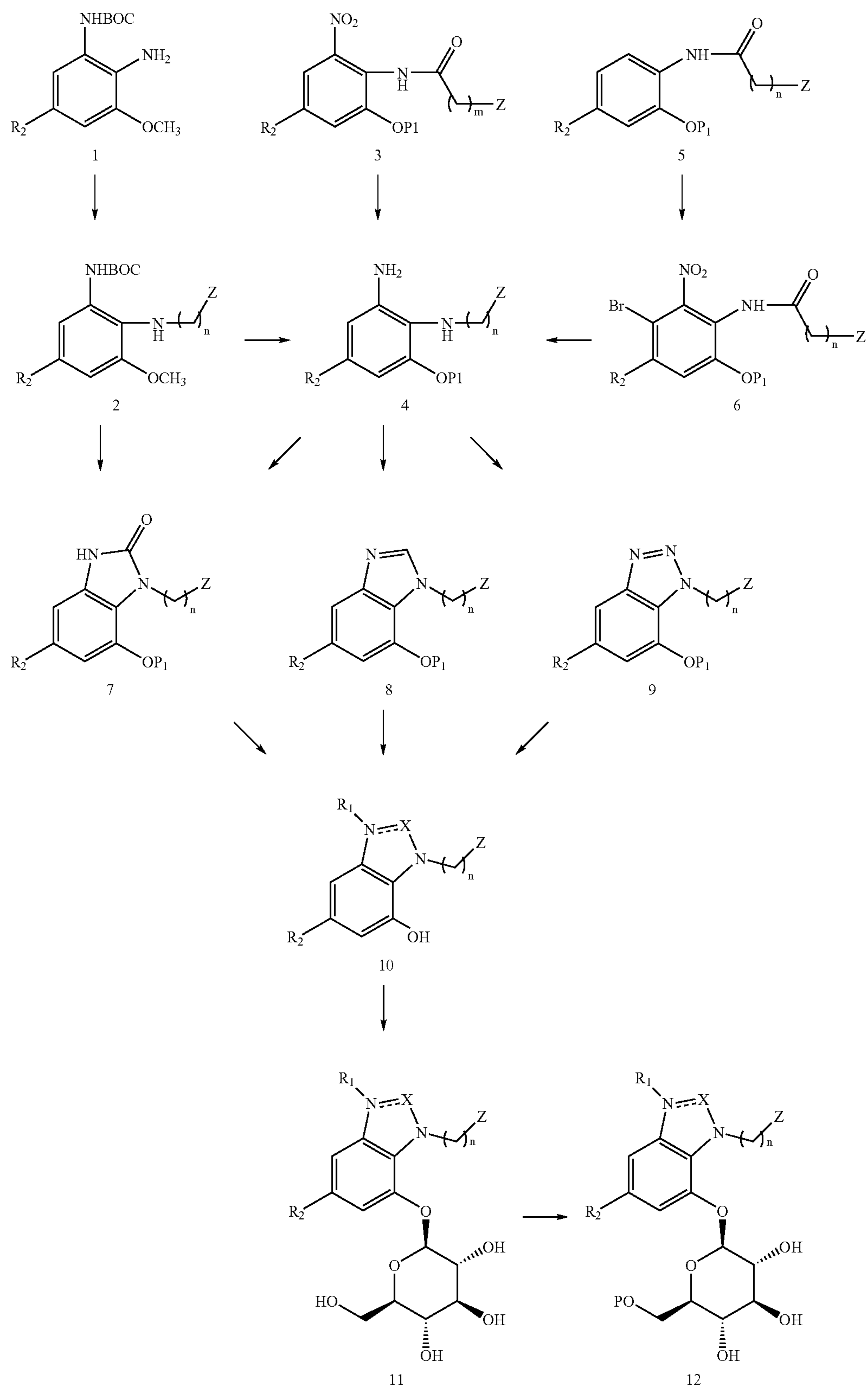
Scheme 1
