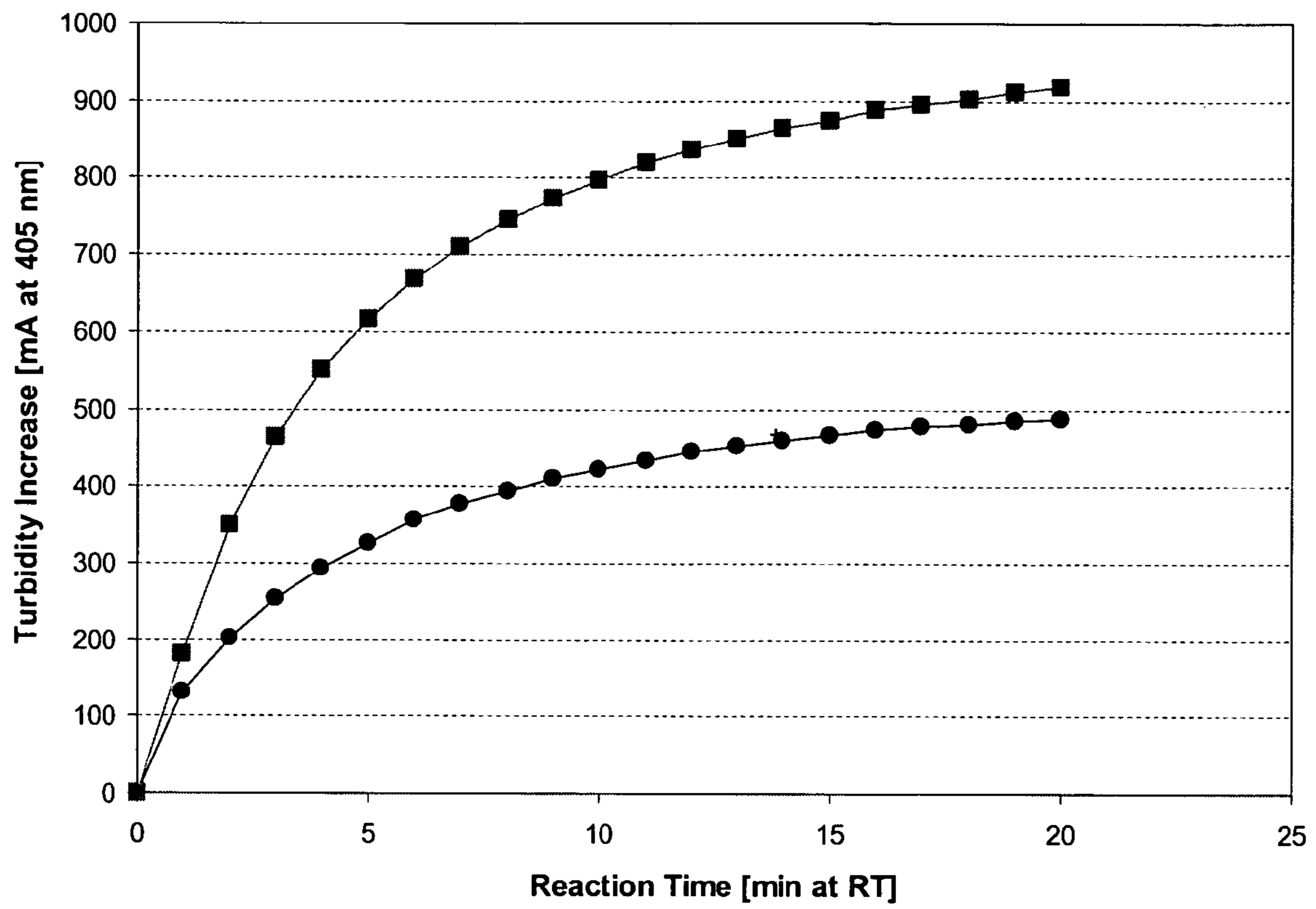
Fig. 7c: Reaction kinetic
