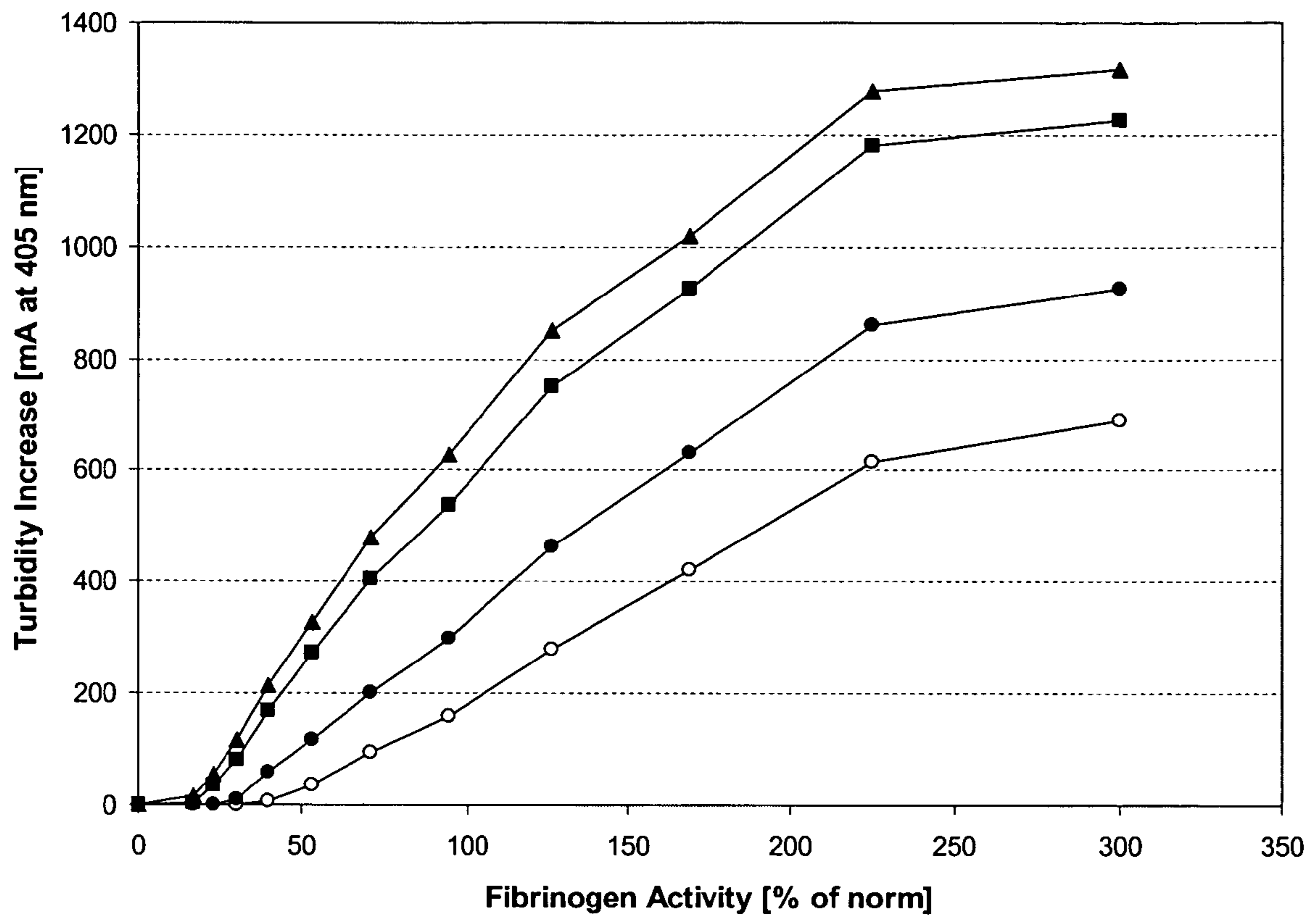
Fig. 9c: FIFTA-linearity
