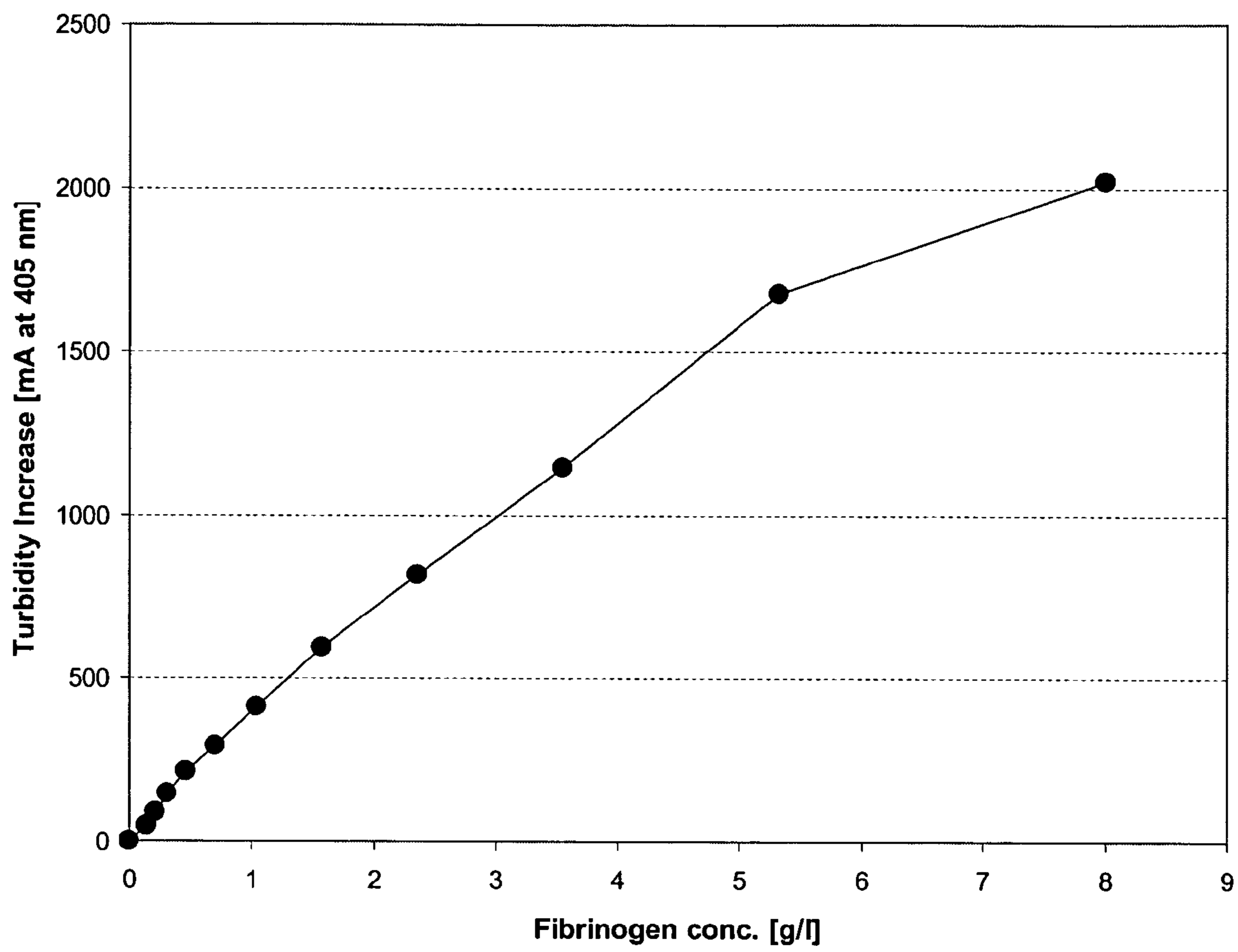
Fig. 22c: FIATA linearity
