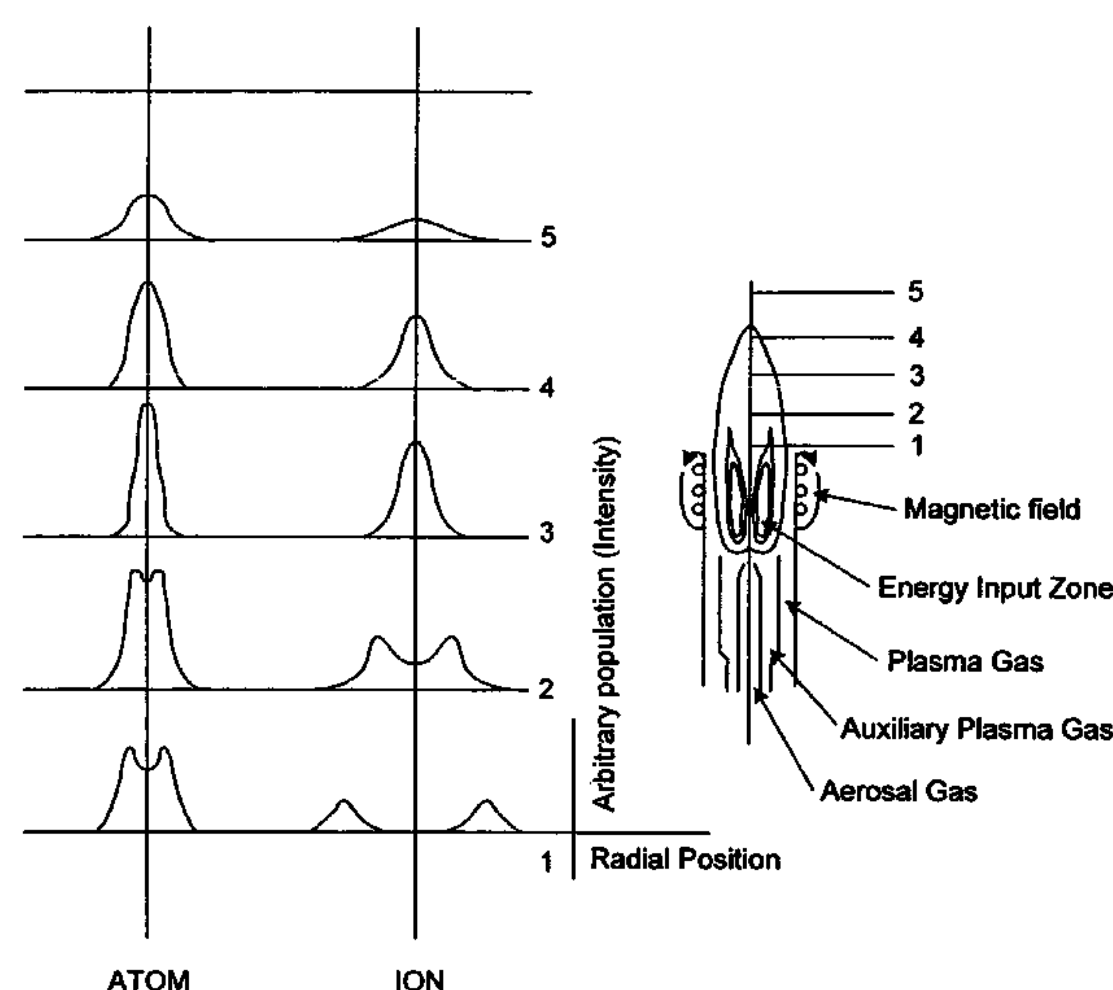
Atom and Ion Distribution in the ICP
