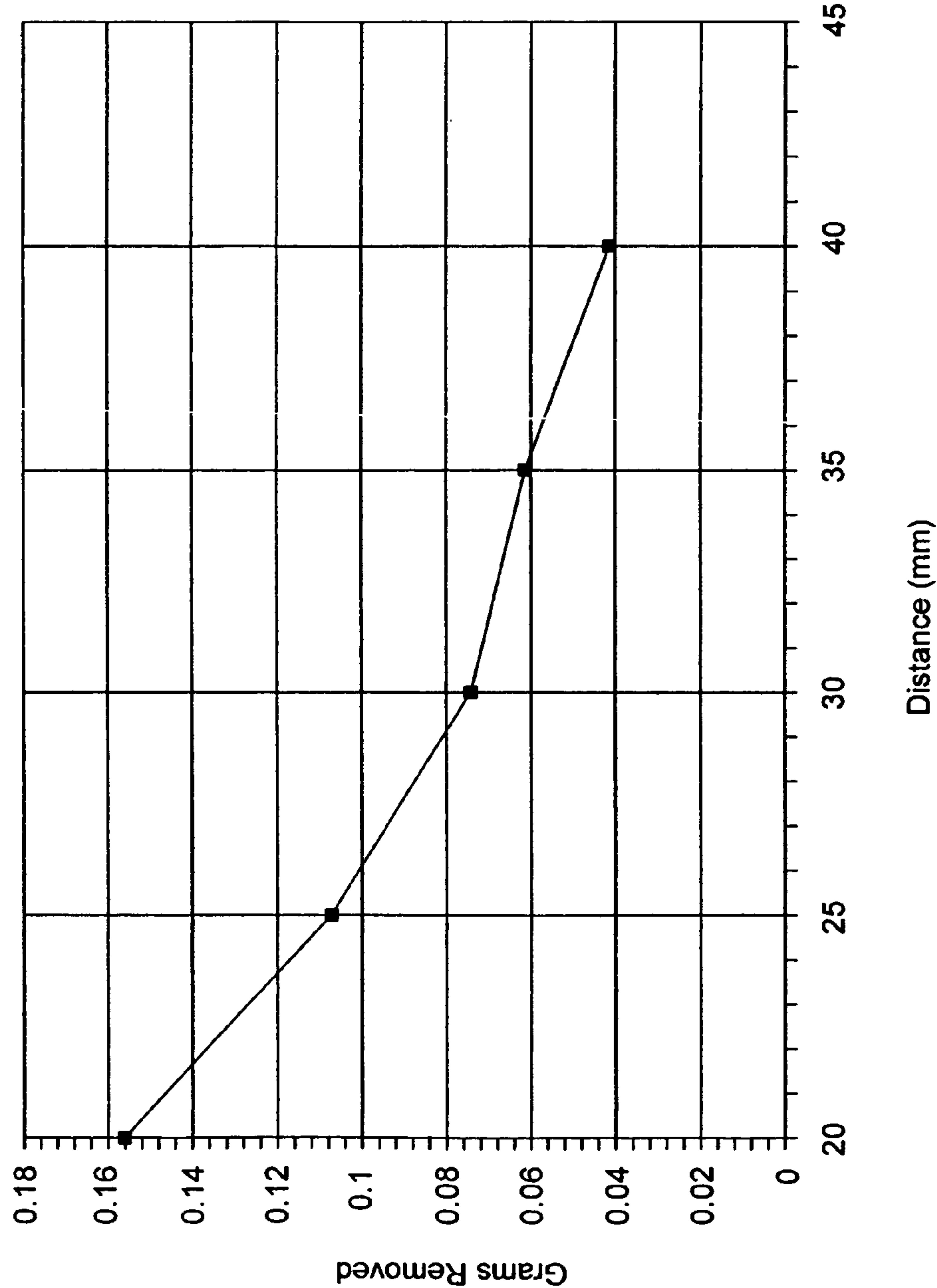
Effect of Distance from Plasma
