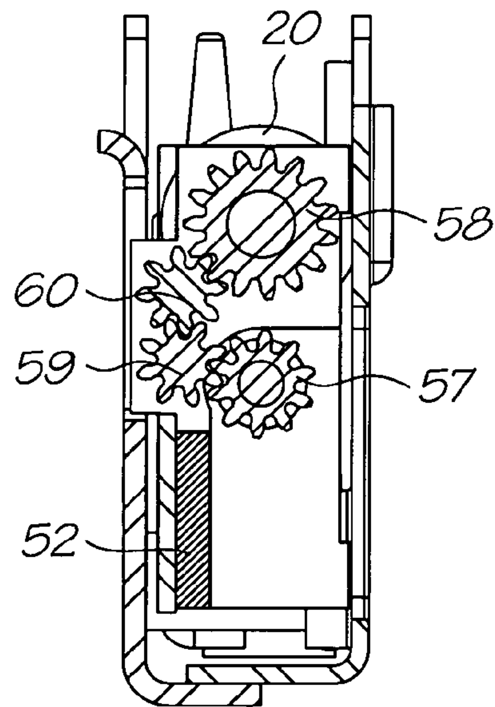
Section B-B
