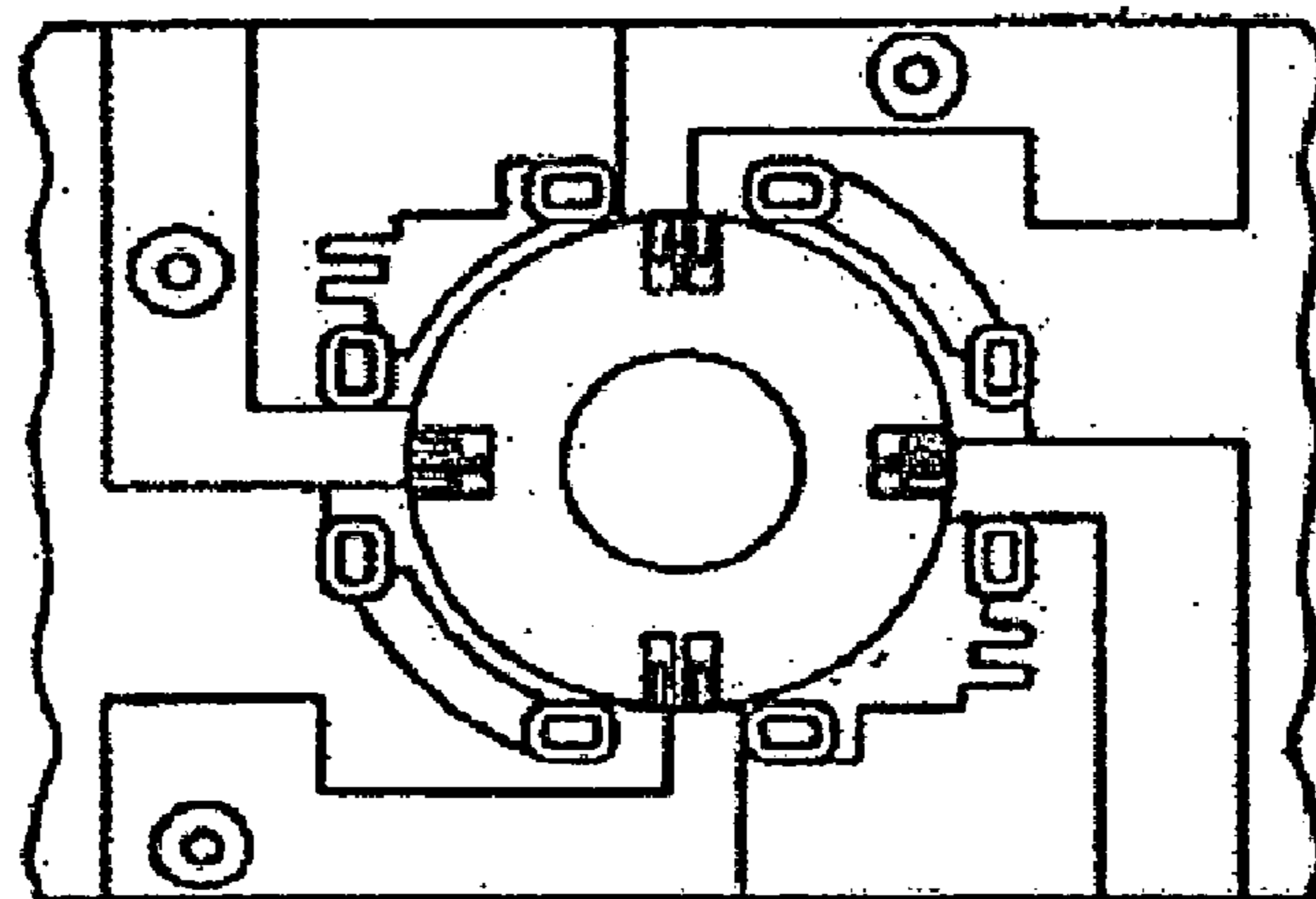
-PRIOR ART- FIG. 11B mems pressure sensor
