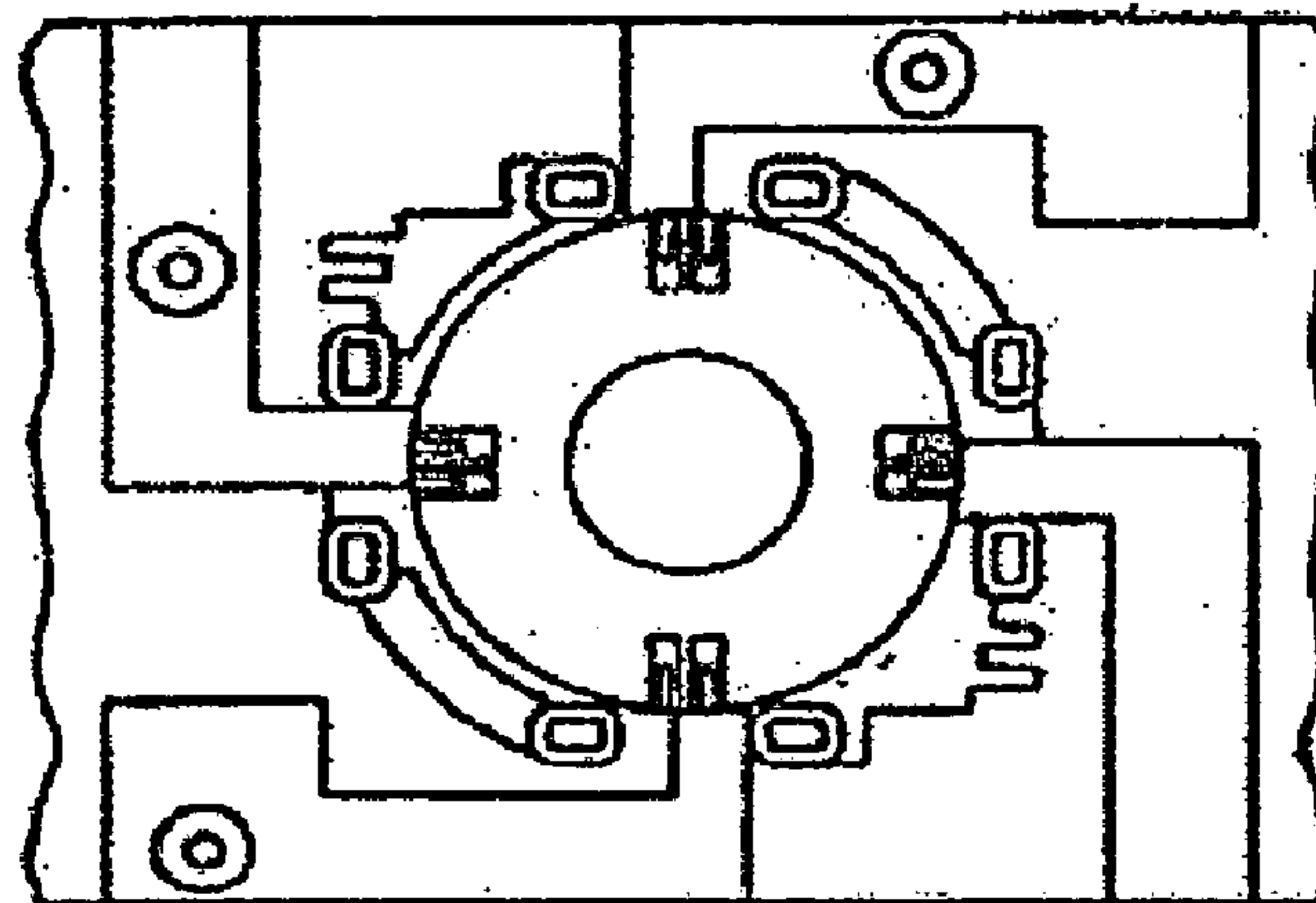
-PRIOR ART- FIG. 11B mems pressure sensor
