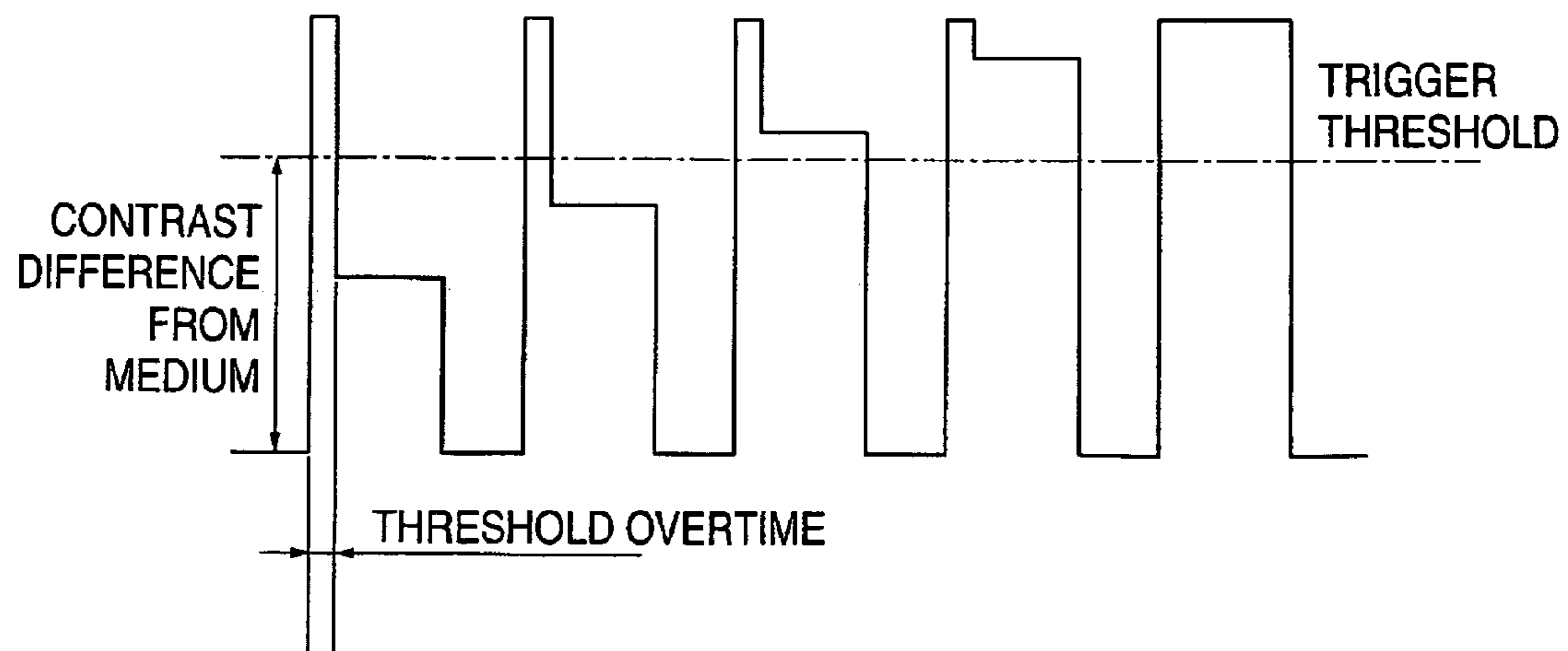
PHOTODIODE OUTPUTS FOR BK PART
