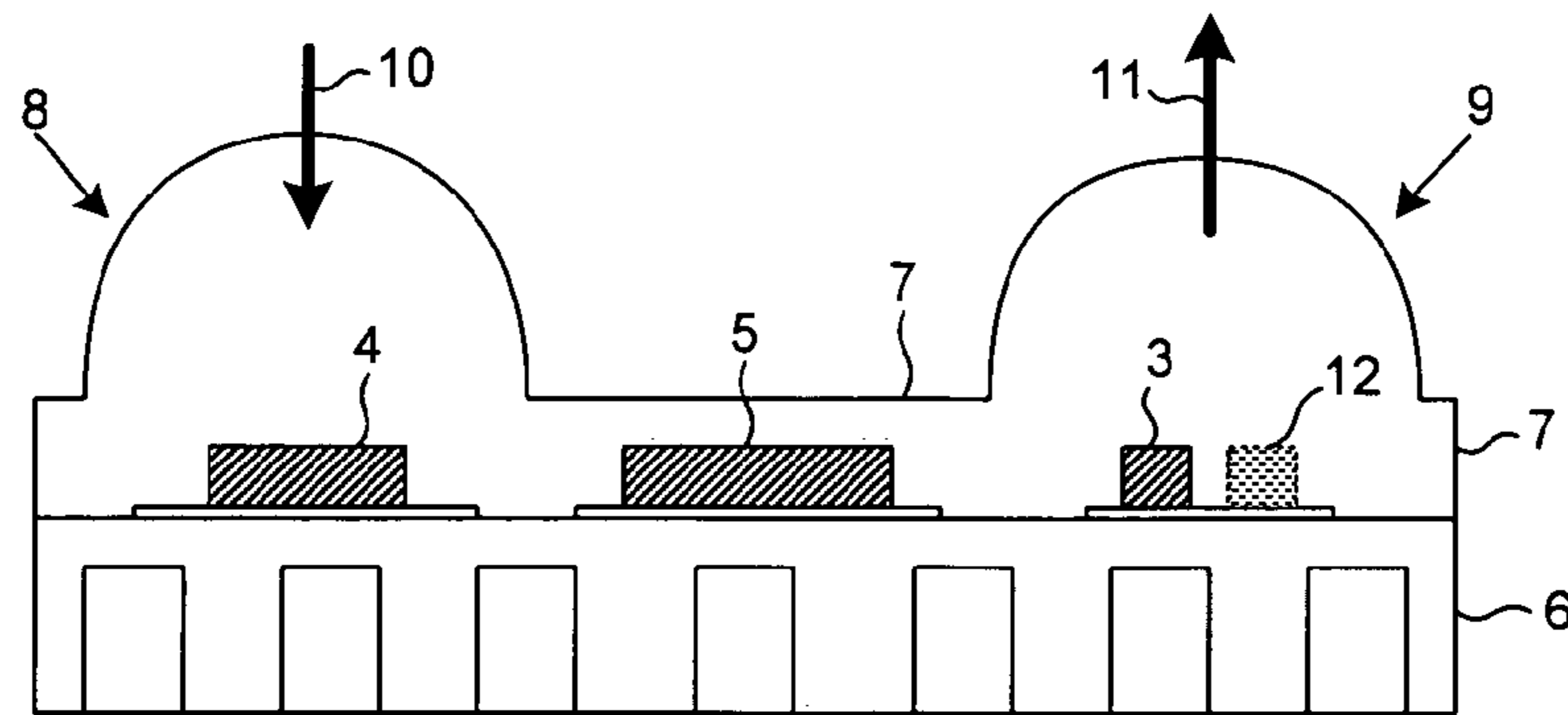
FIG. 2 (PRIOR ART)
