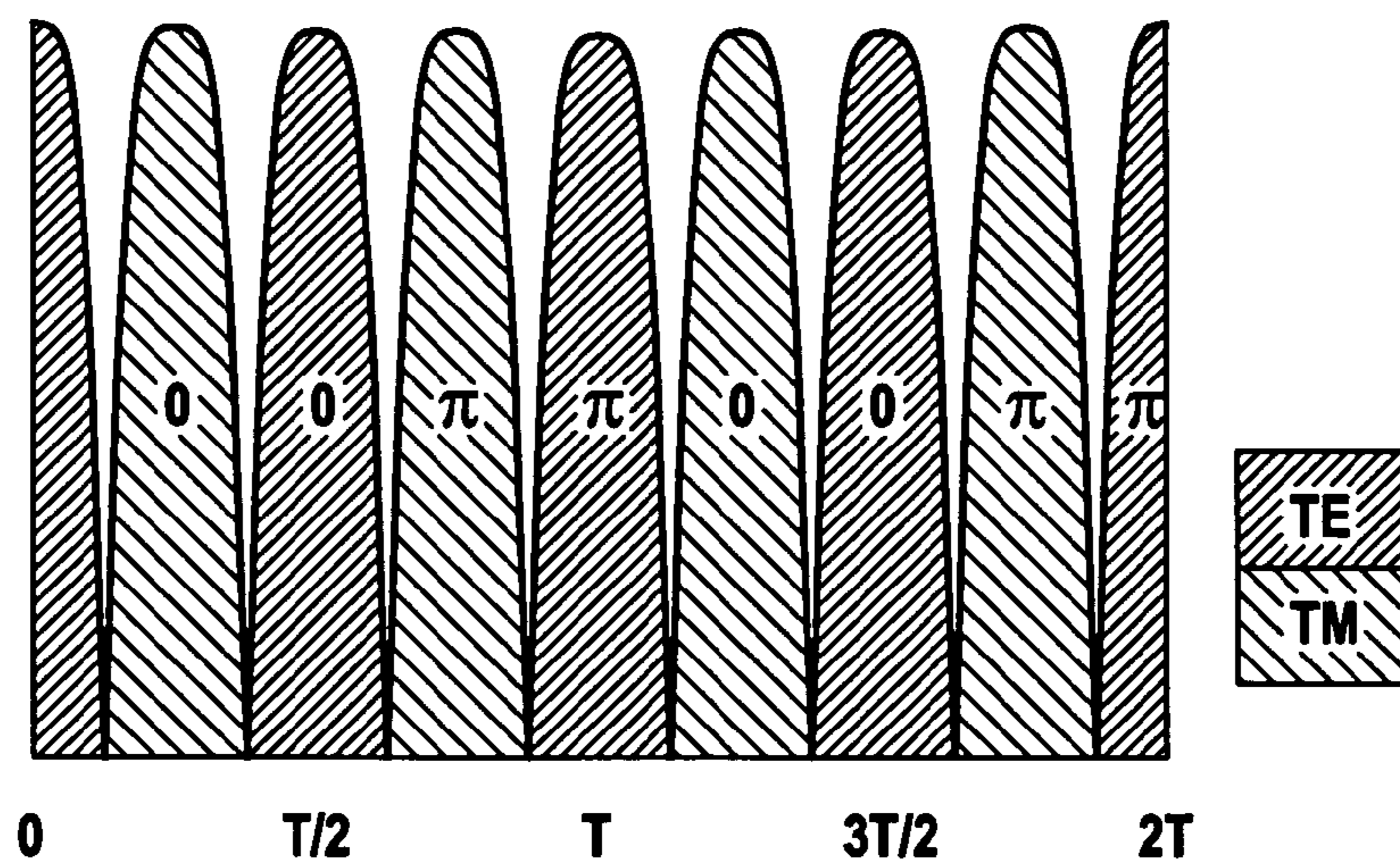
Pulses stream at 4F_{\text{clock}} after OTDM (Coding section omitted for demonstration)
