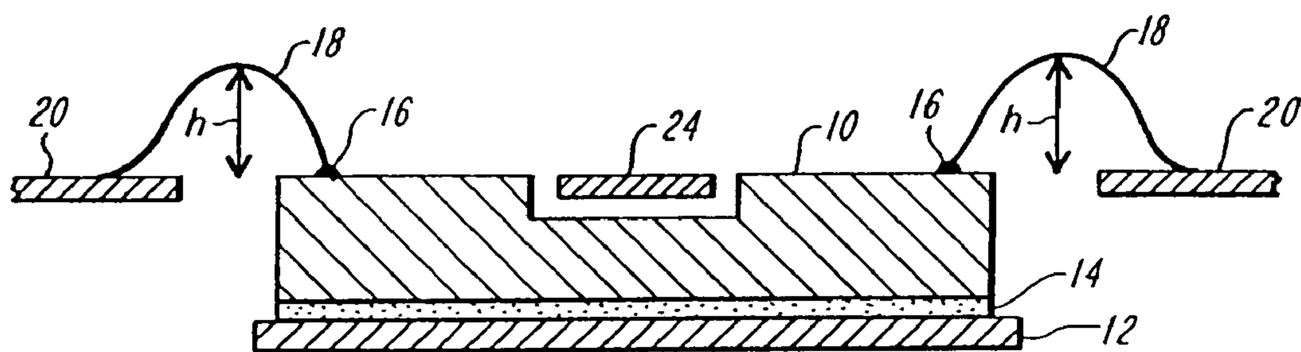
FIG. 1 (PRIOR ART)
