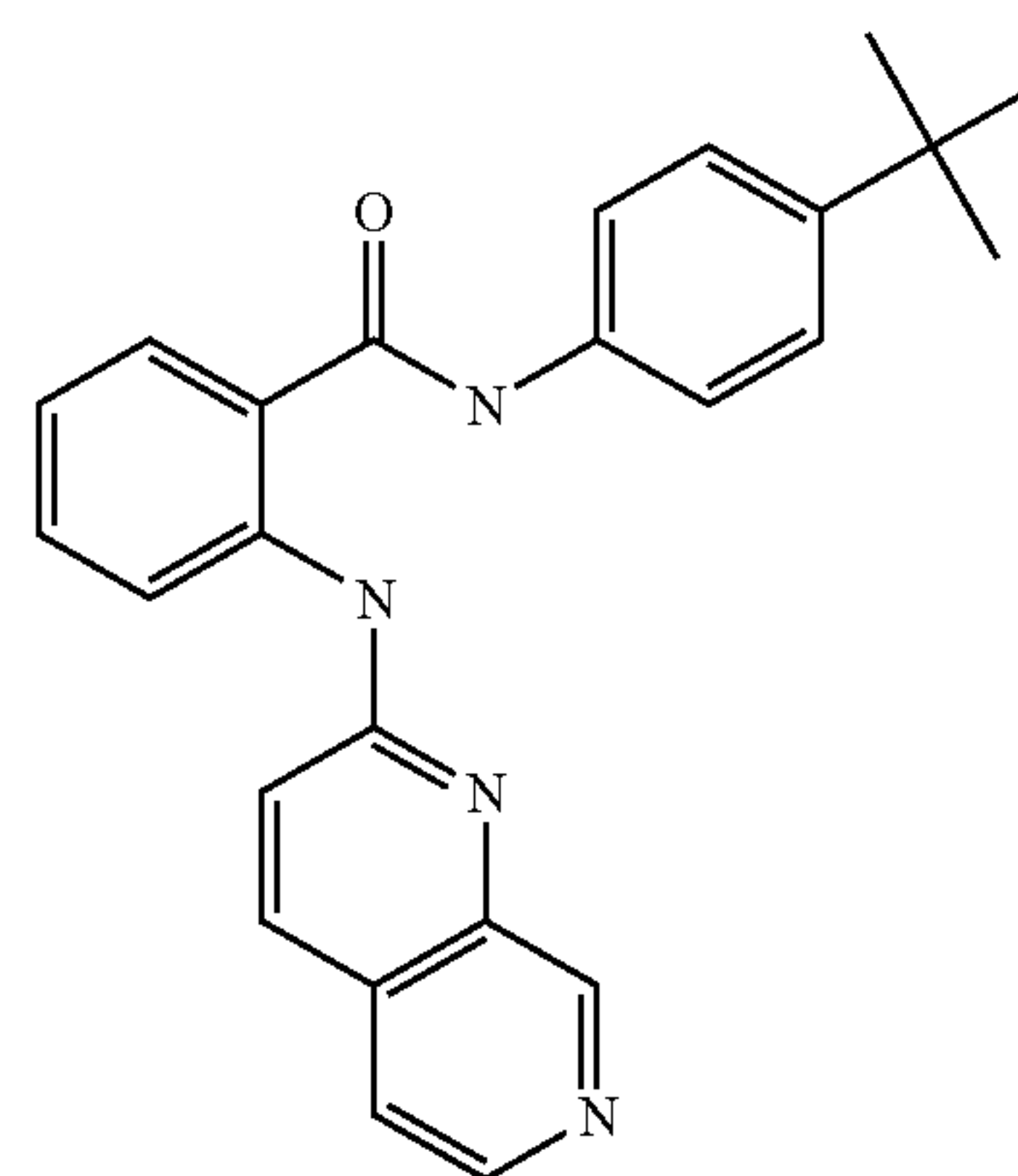
N-(4-tert-Butyl-phenyl)-2-([1,7]naphthyridin-2-ylamino)-benzamide
