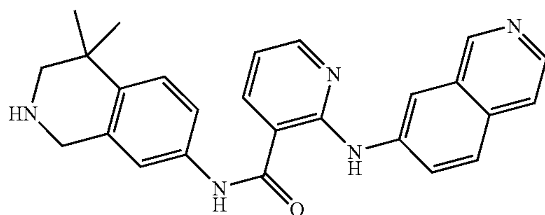
N-(4,4-Dimethyl-1,2,3,4-tetrahydro-isoquinolin-7-yl)-2-(isoquinolin-7-ylamino)-nicotinamide
