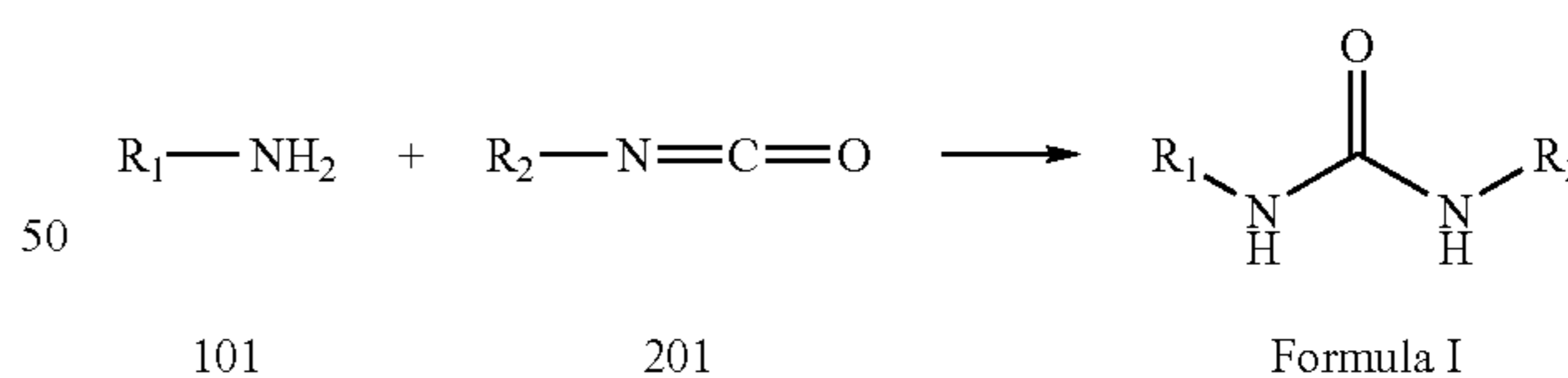
REACTION SCHEME 2
