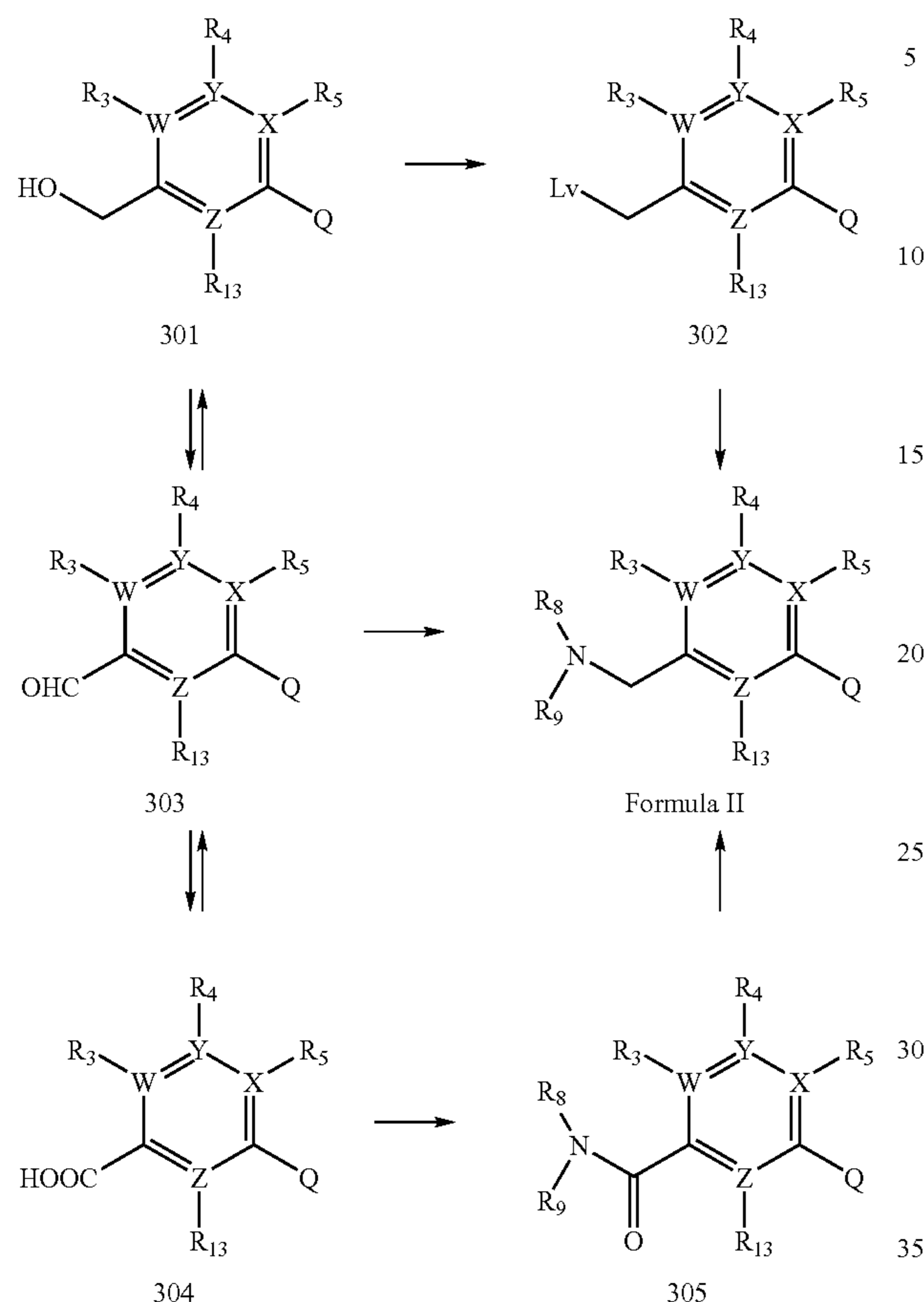
REACTION SCHEME 3
