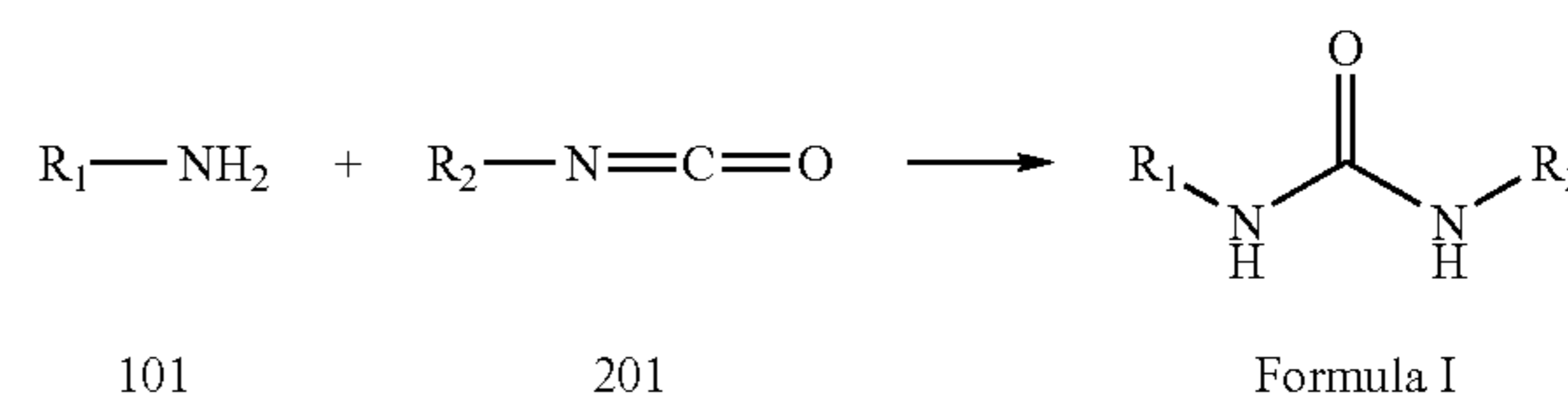
REACTION SCHEME 2
