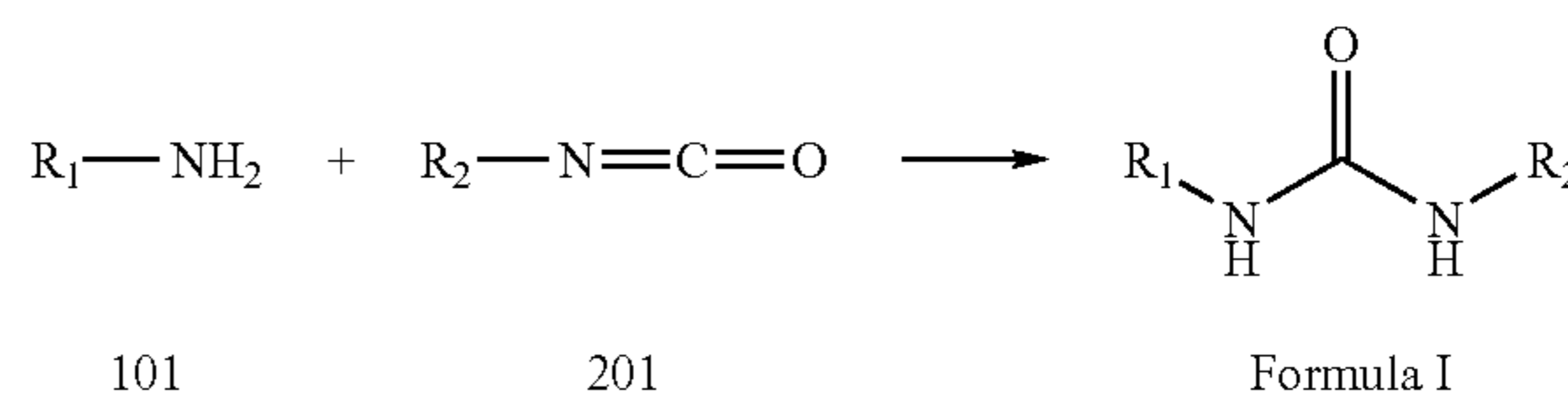
REACTION SCHEME 2
