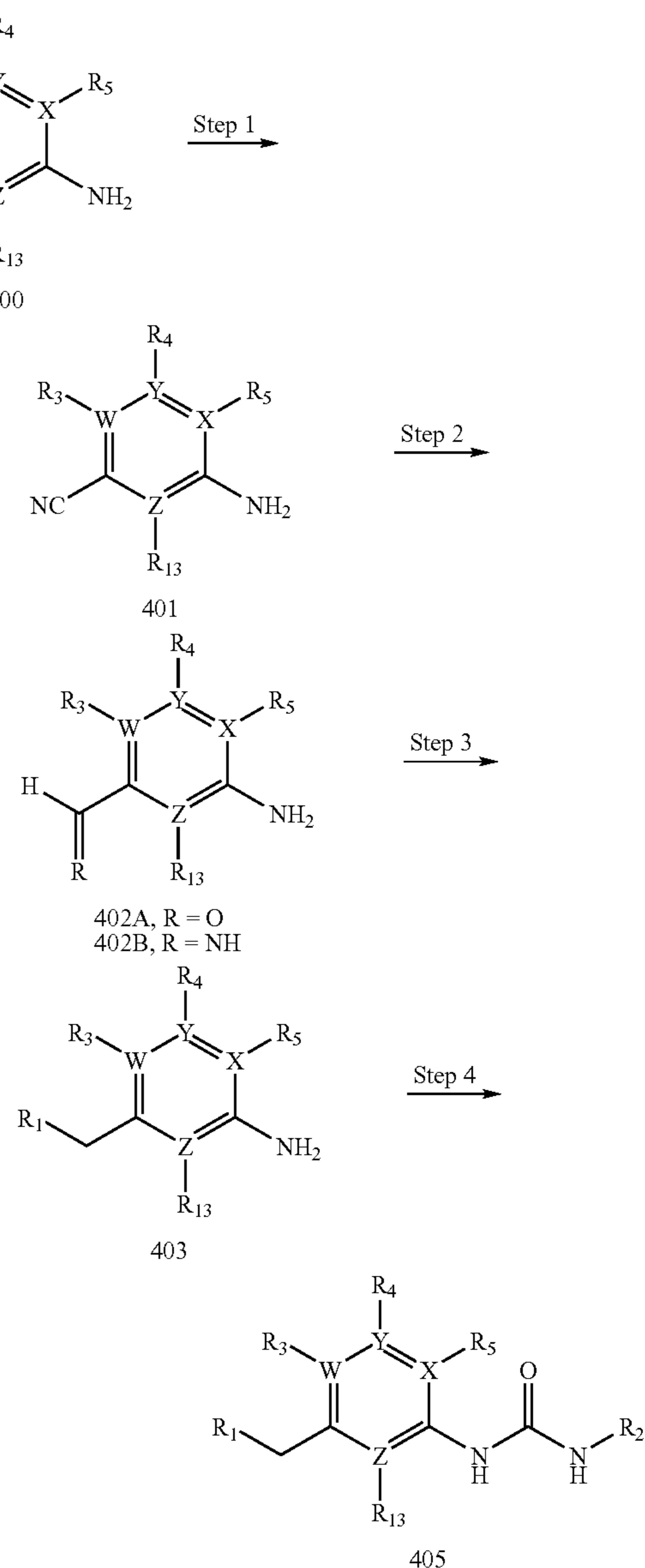
Reaction Scheme 4
