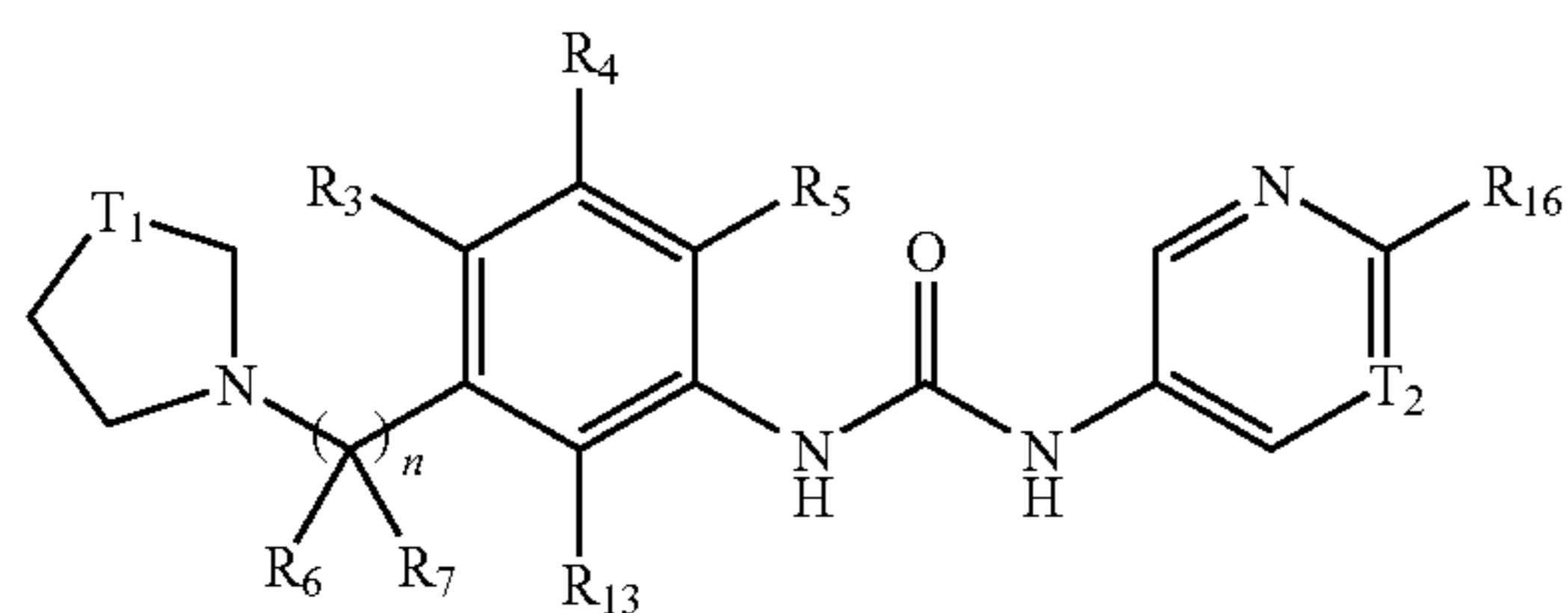
Formula Id
