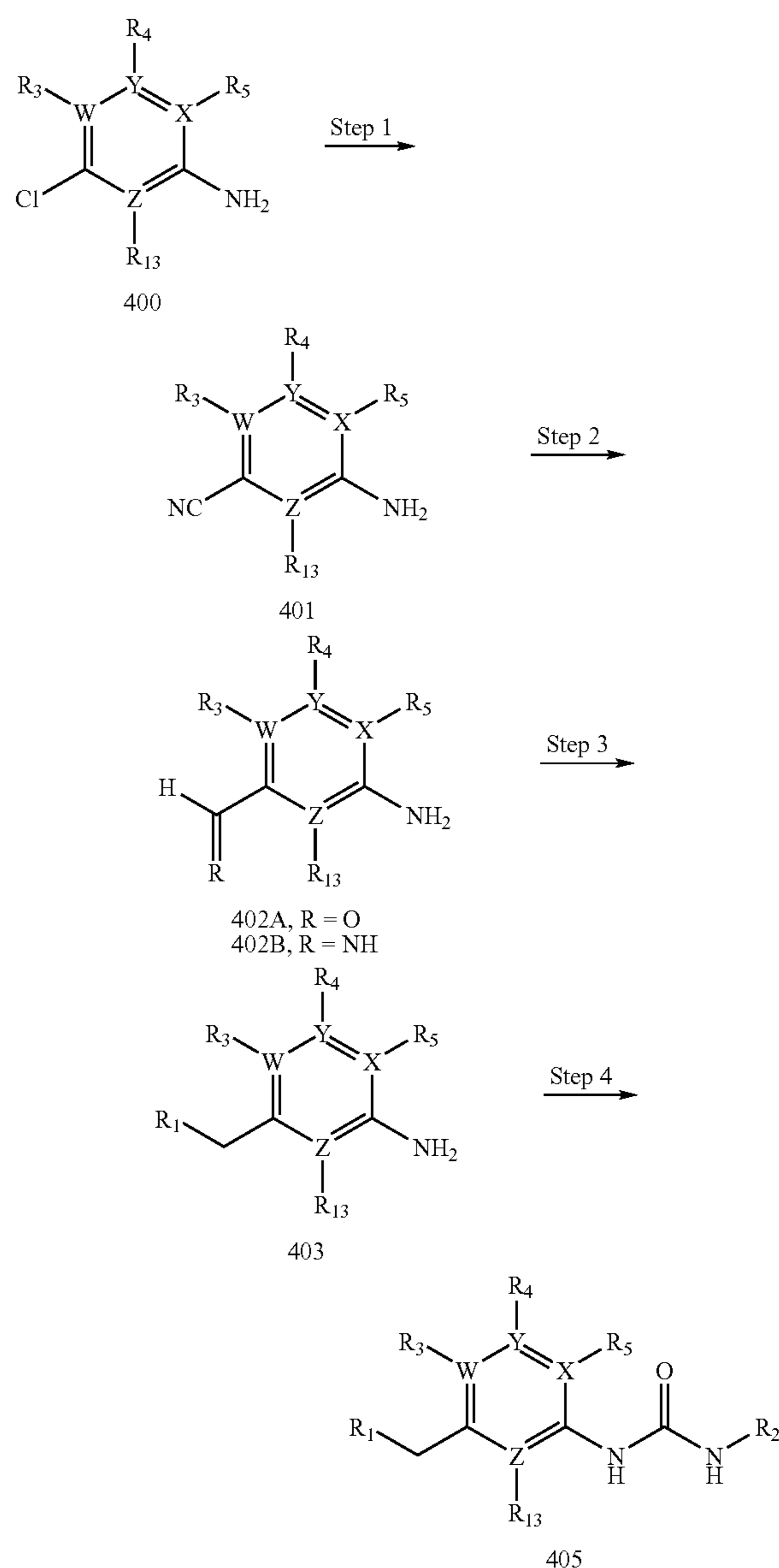
Reaction Scheme 4
