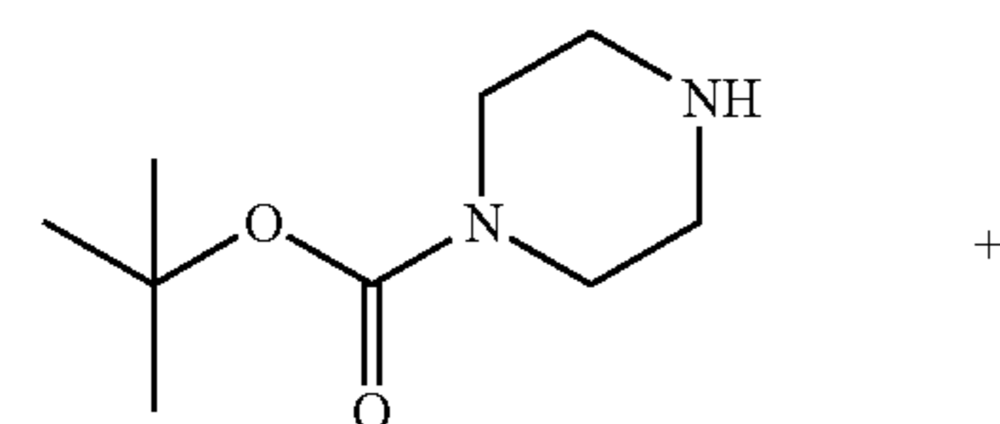
tert-butyl piperazine-1-carboxylate
