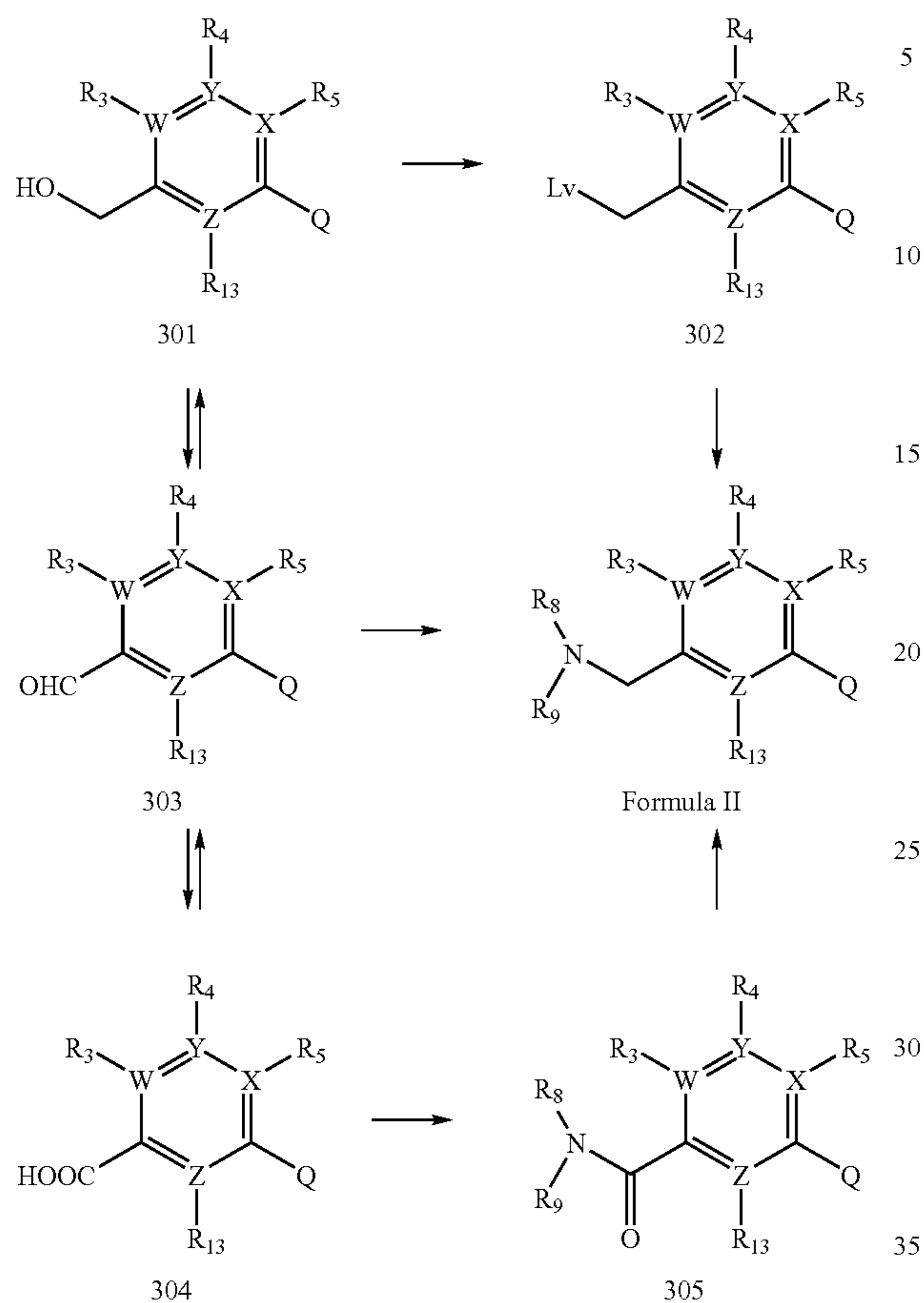
REACTION SCHEME 3
