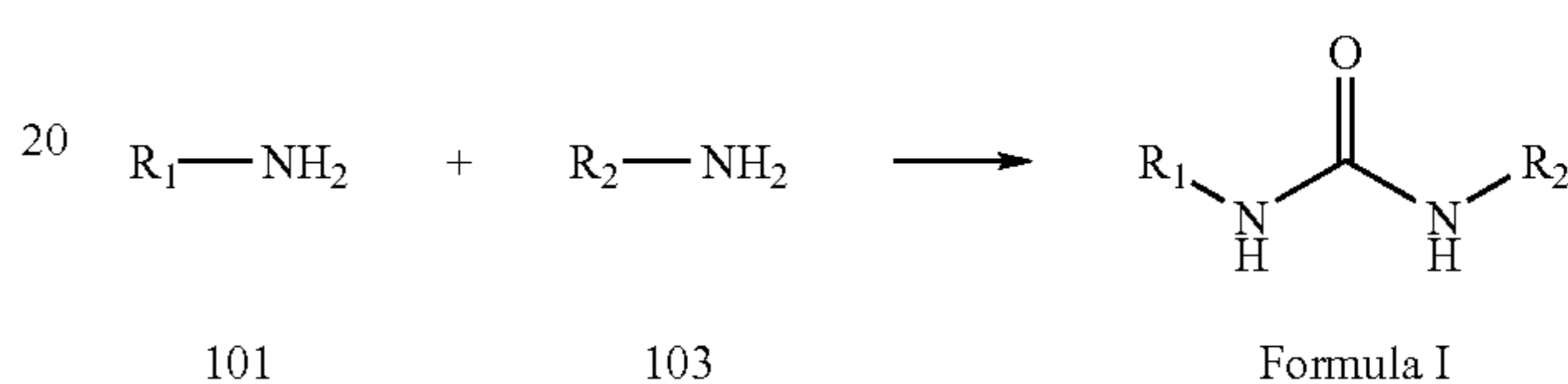
REACTION SCHEME 1
