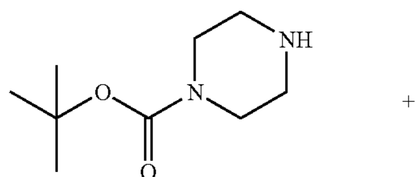
tert-butyl piperazine-1-carboxylate
