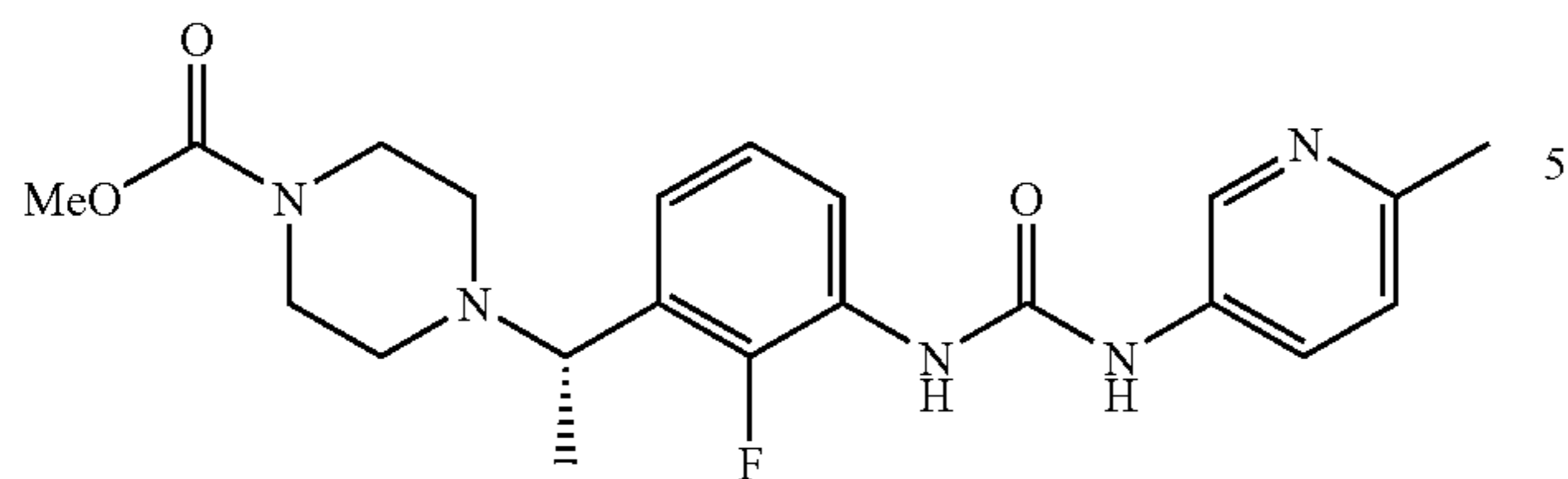
(S)-methyl 4-(1-(2-fluoro-3-(3-(6-methylpyridin-3-yl)ureido)phenyl)ethyl)piperazine-1-carboxylate
