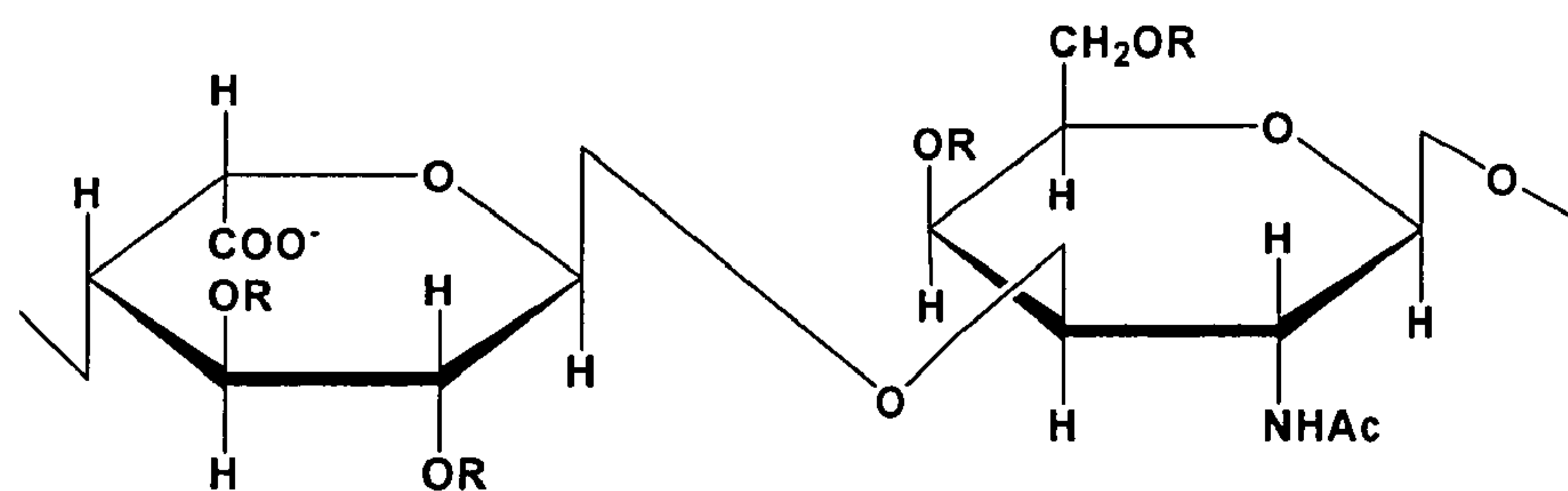
Dermatan Sulfate
