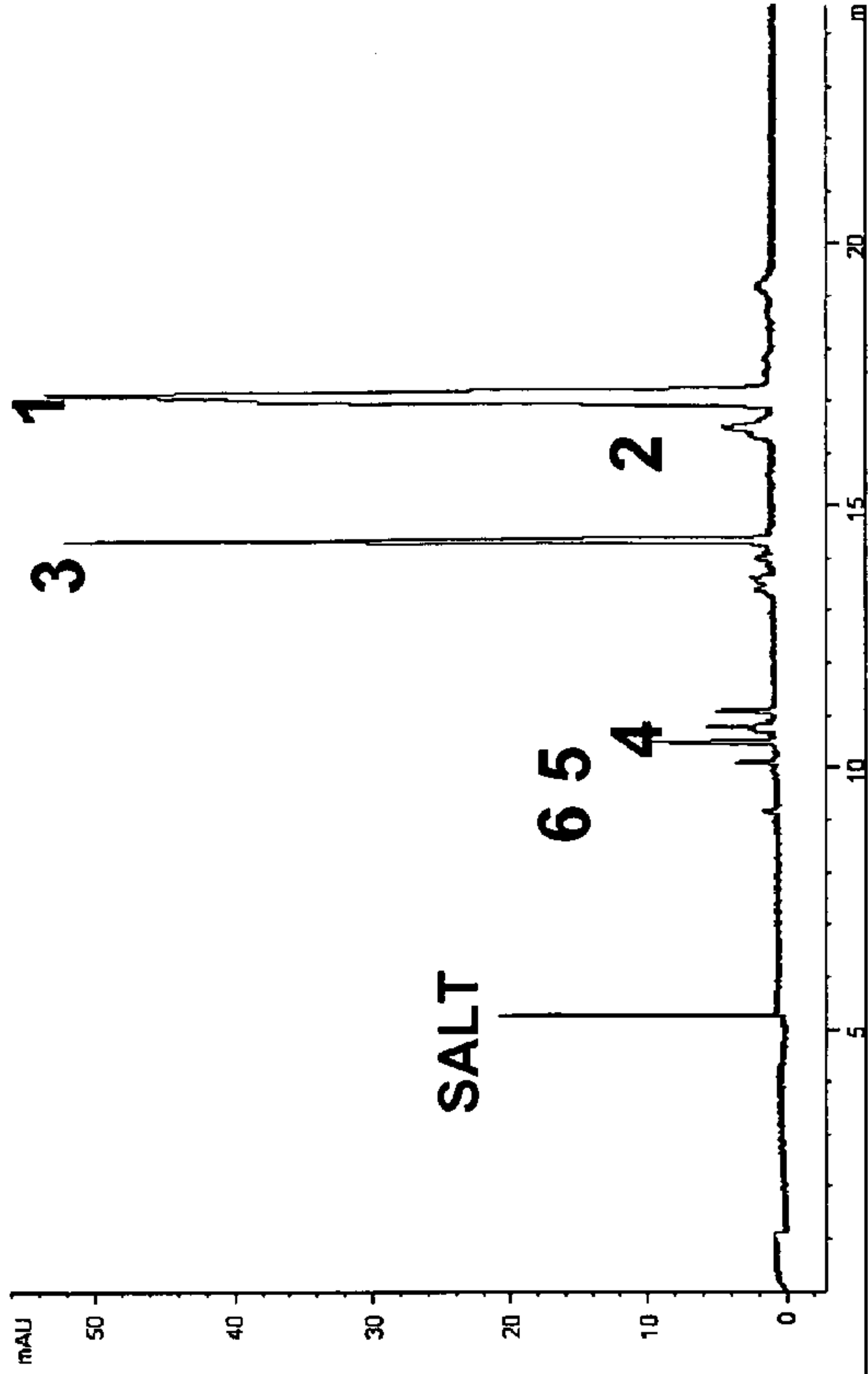
Dermatan Sulfate
