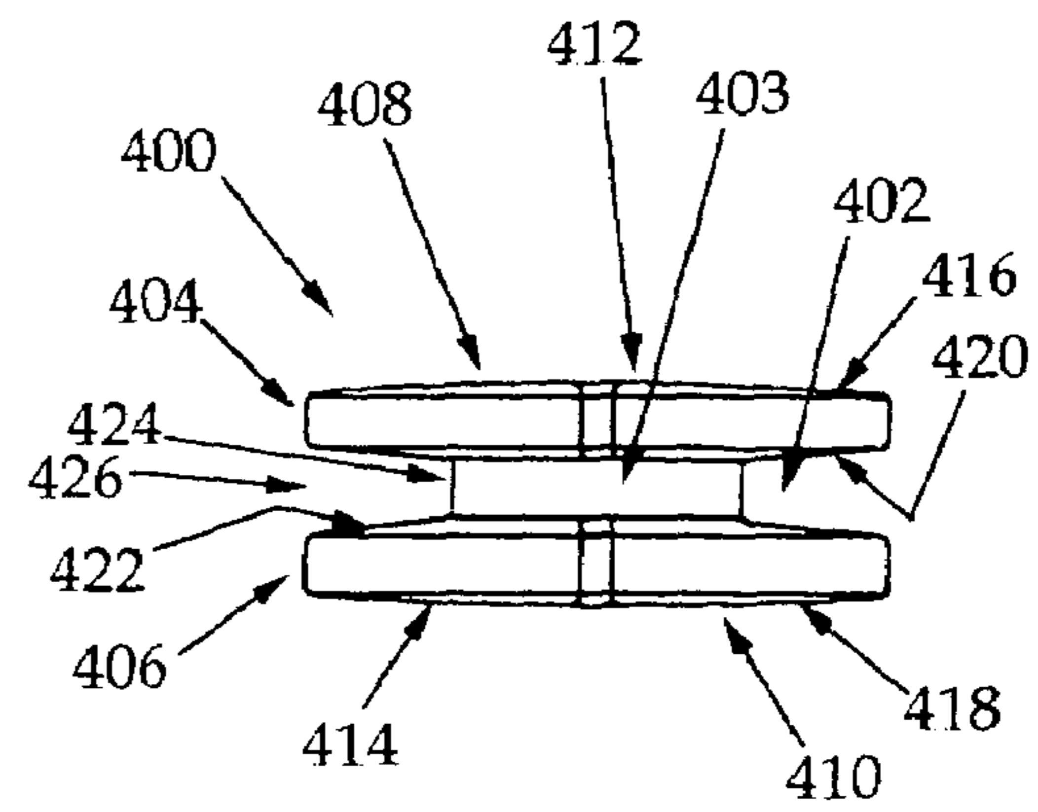
Section B-B
