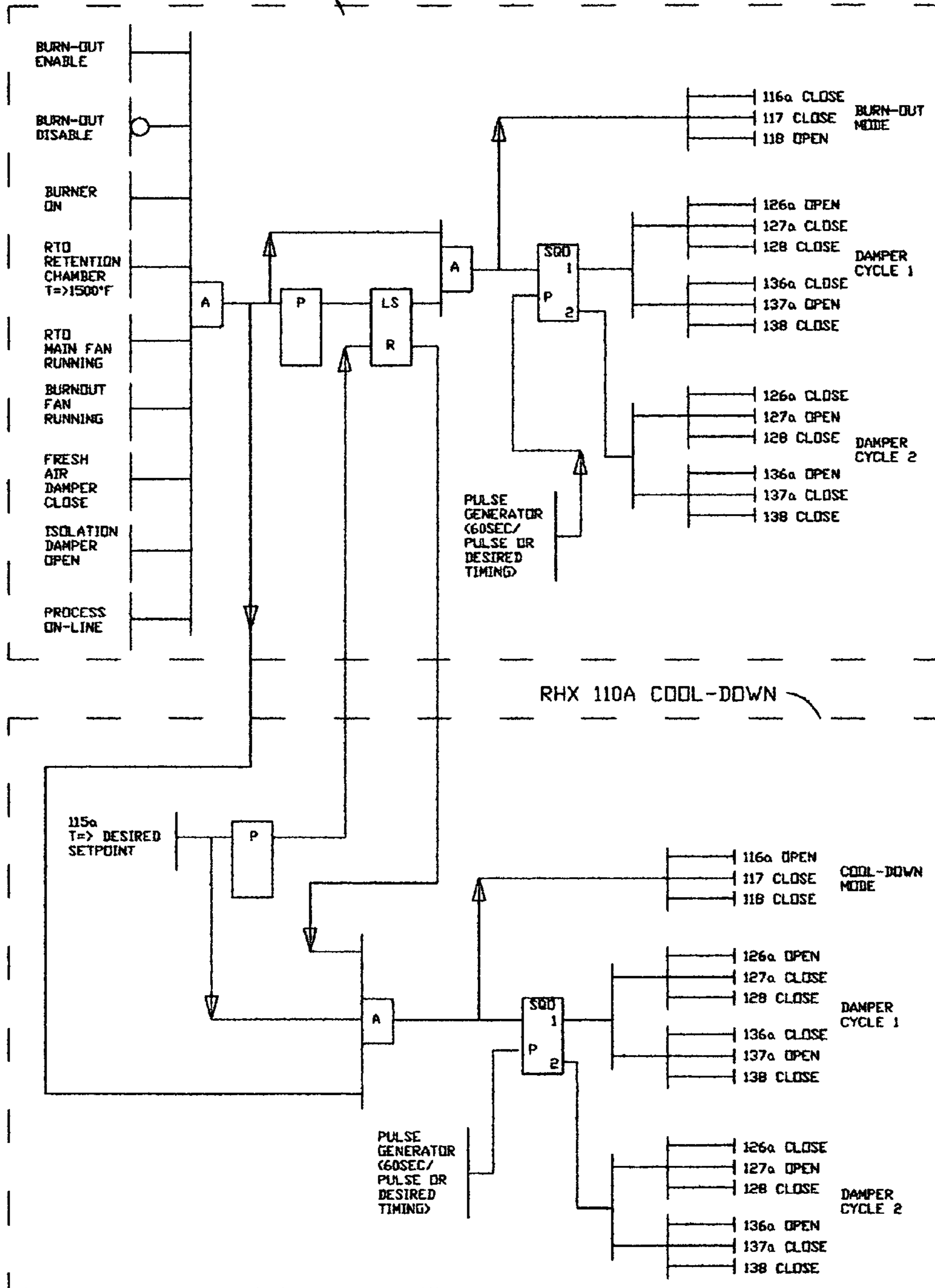
RHX 110A BURN-OUT LOGIC
