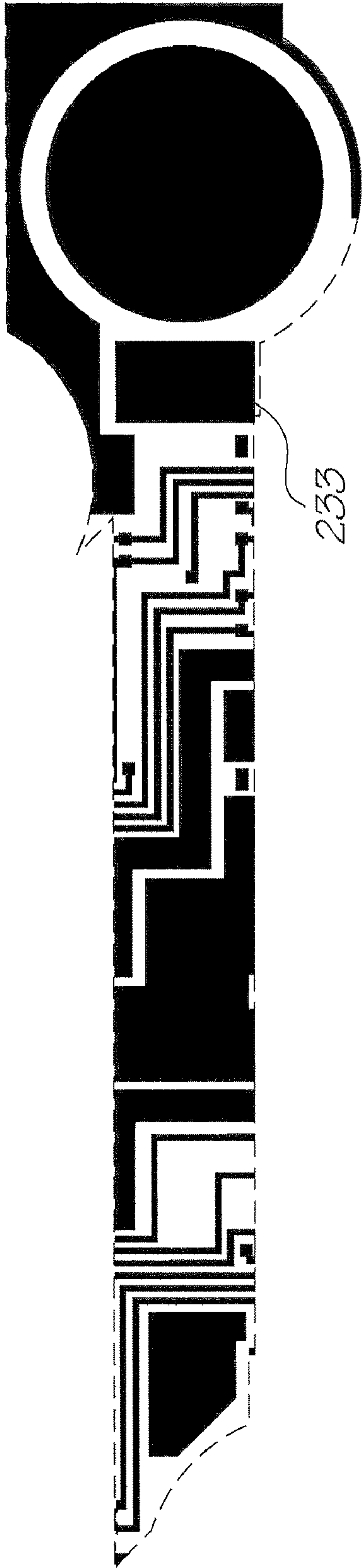
Metal 2 mask
