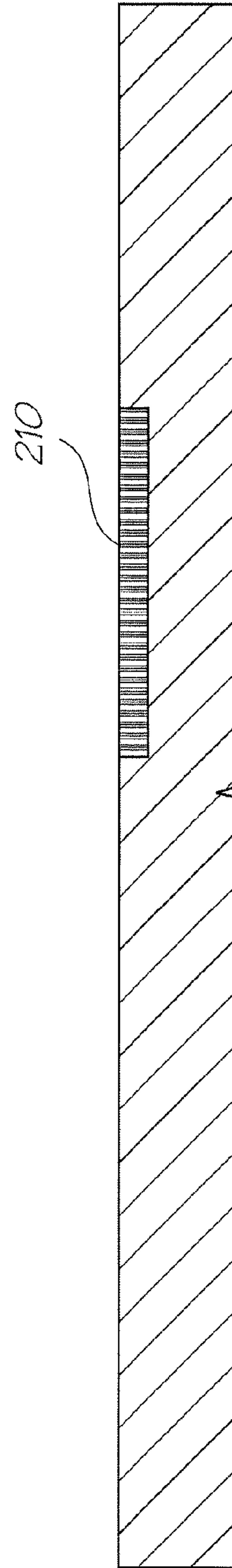
Implant N-Well
