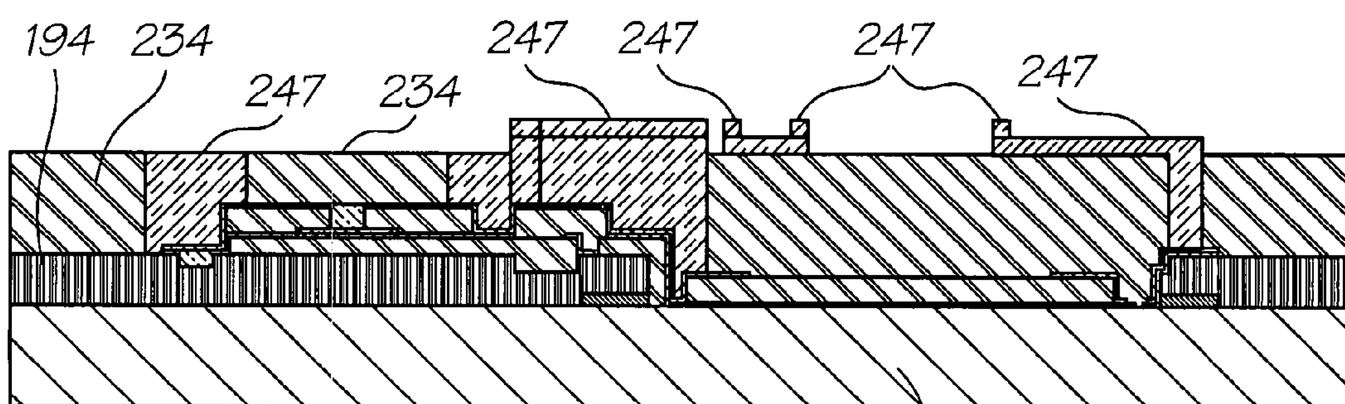
1 micron nozzle roof etch of \text{Si}_x\text{N}_y\text{H}_z
