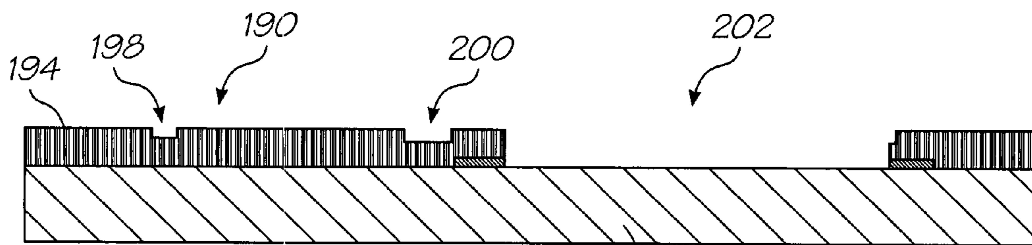
CMOS complete
