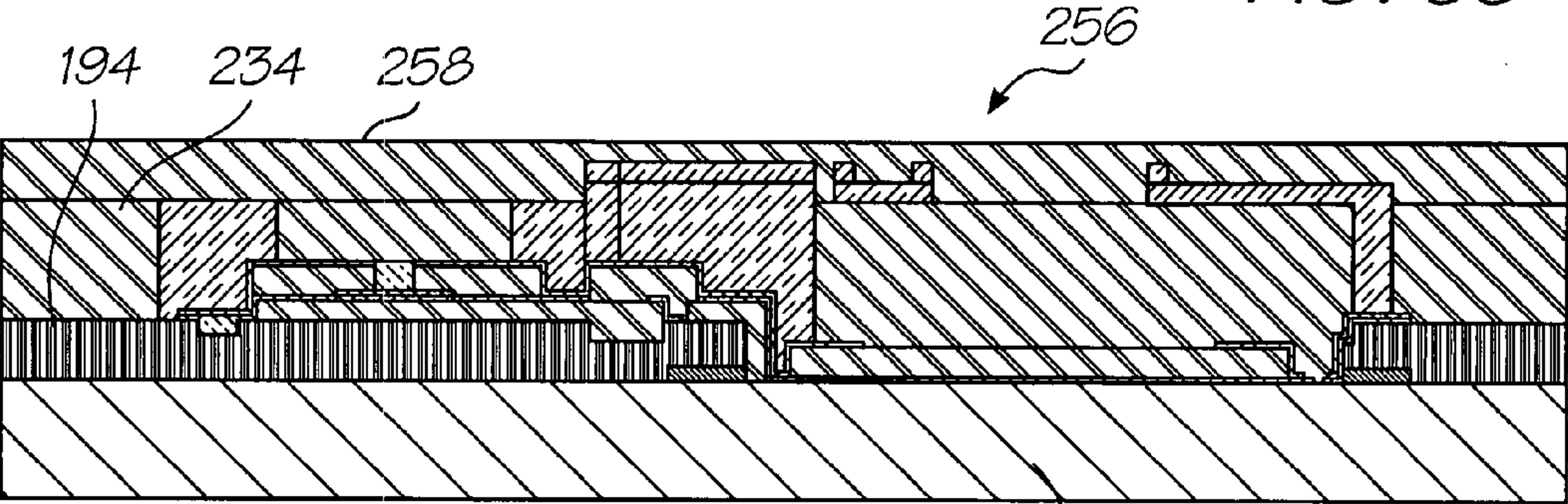
3 micron sacrificial protective polyimide
