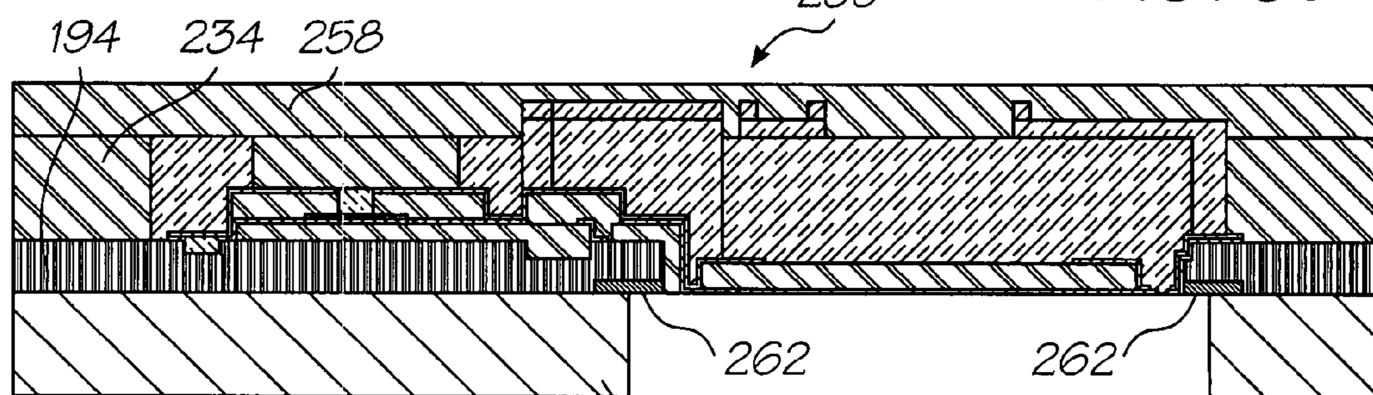
Back-etch using Bosch process
