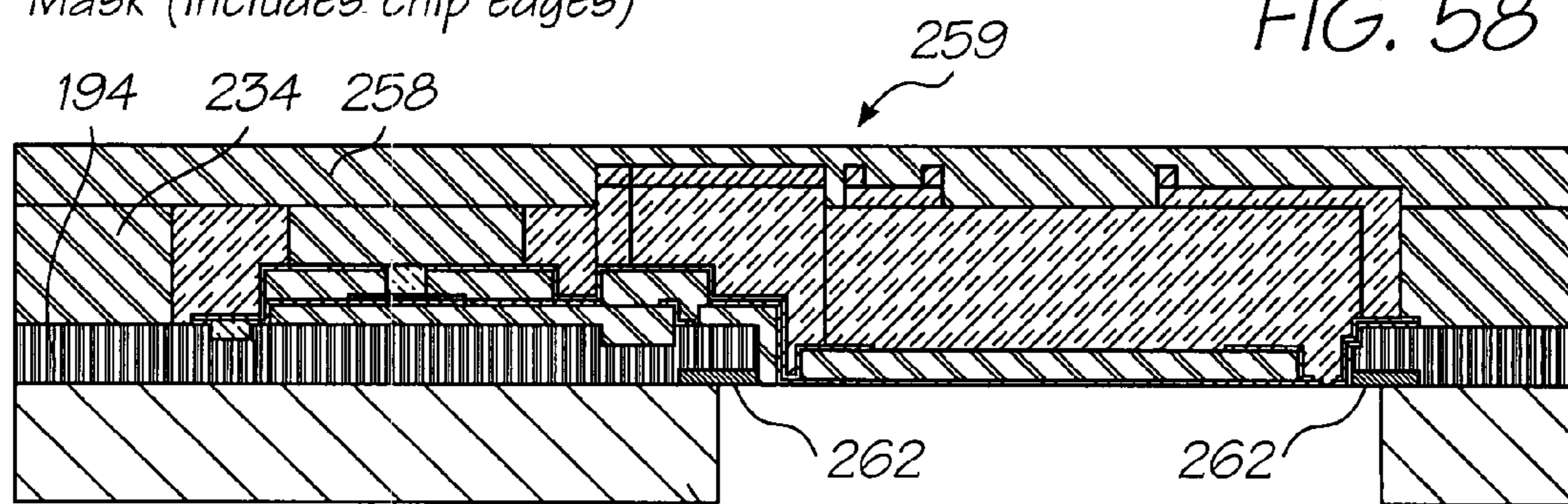
Back-etch using Bosch process
