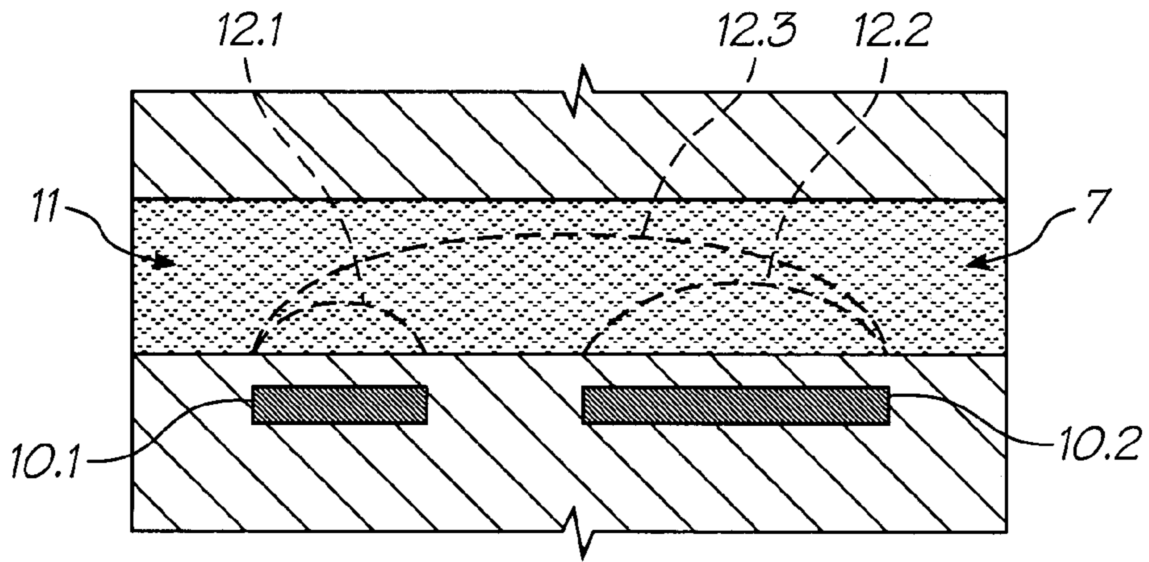
FIG. 52 (PRIOR ART)
