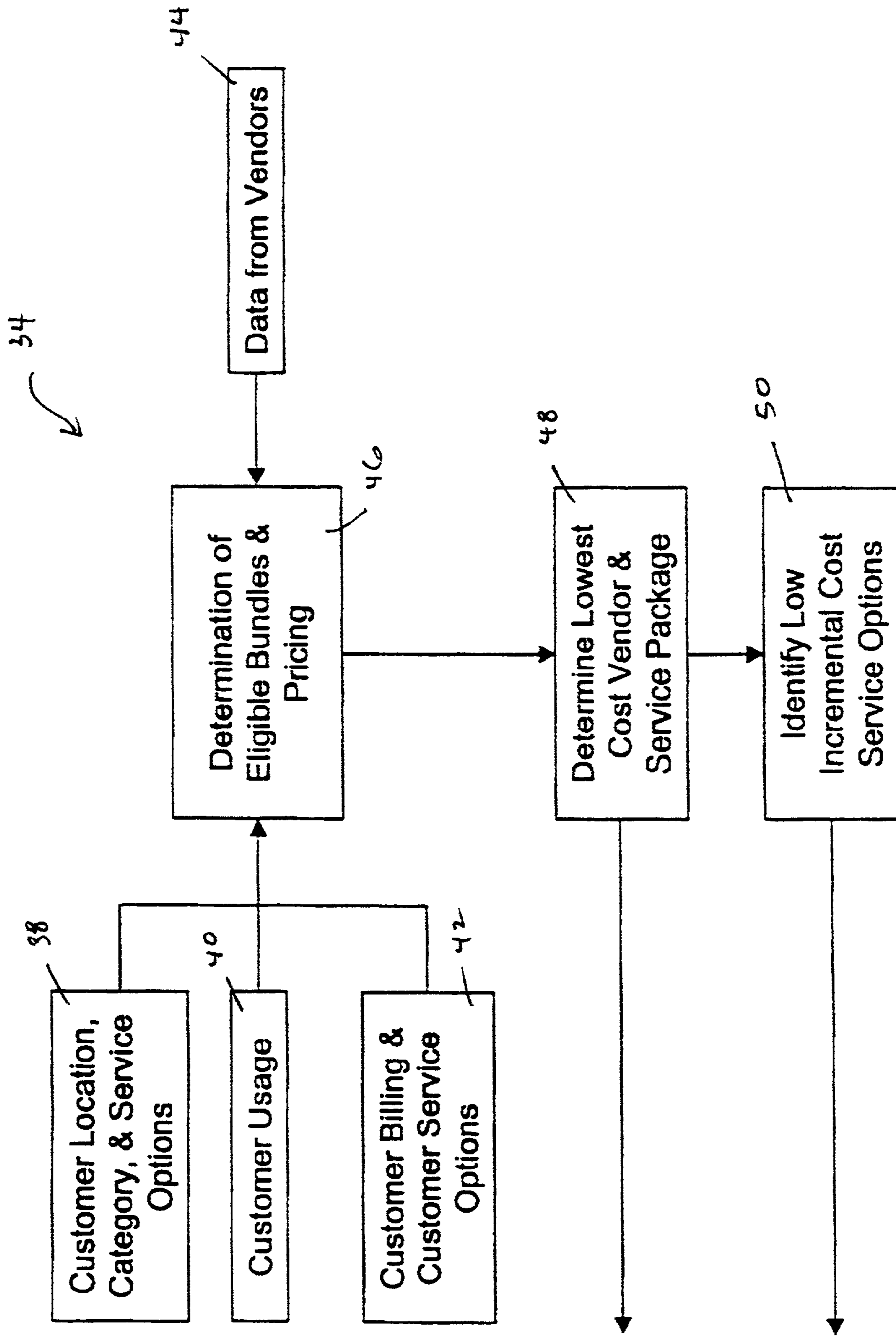
Figure 3: Optimizer
