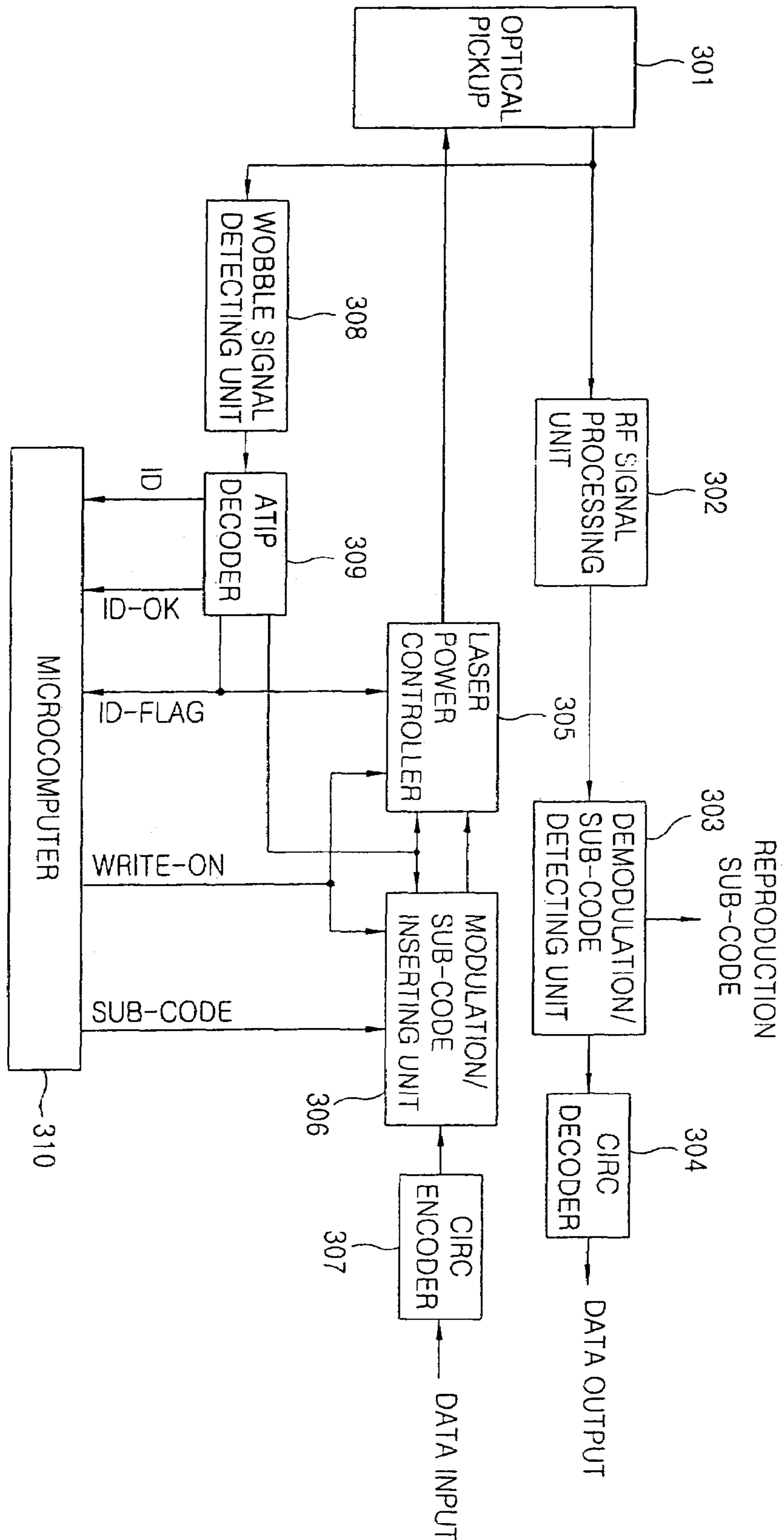
FIG. 3 CONVENTIONAL ART
