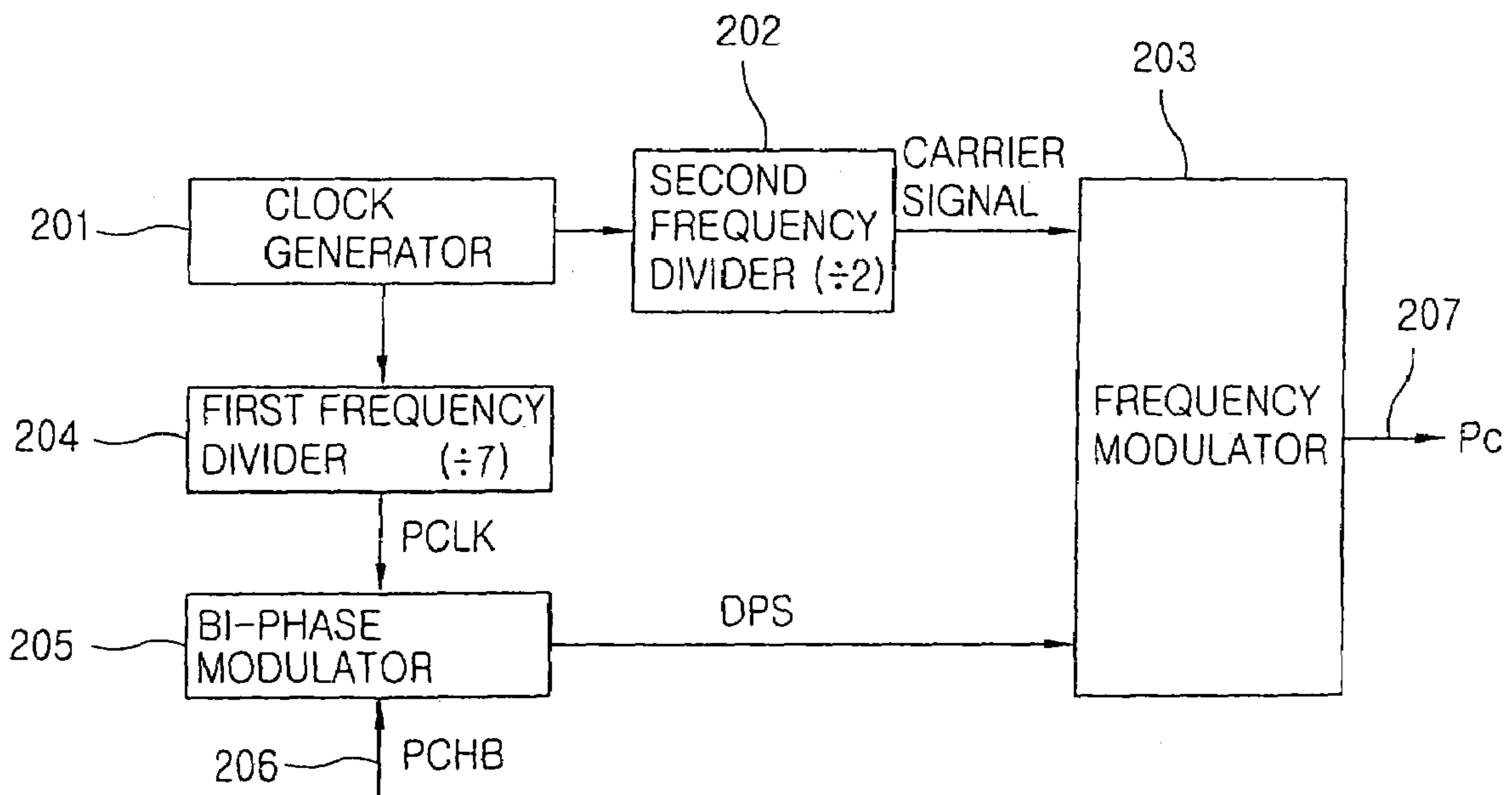
FIG. 2 CONVENTIONAL ART
