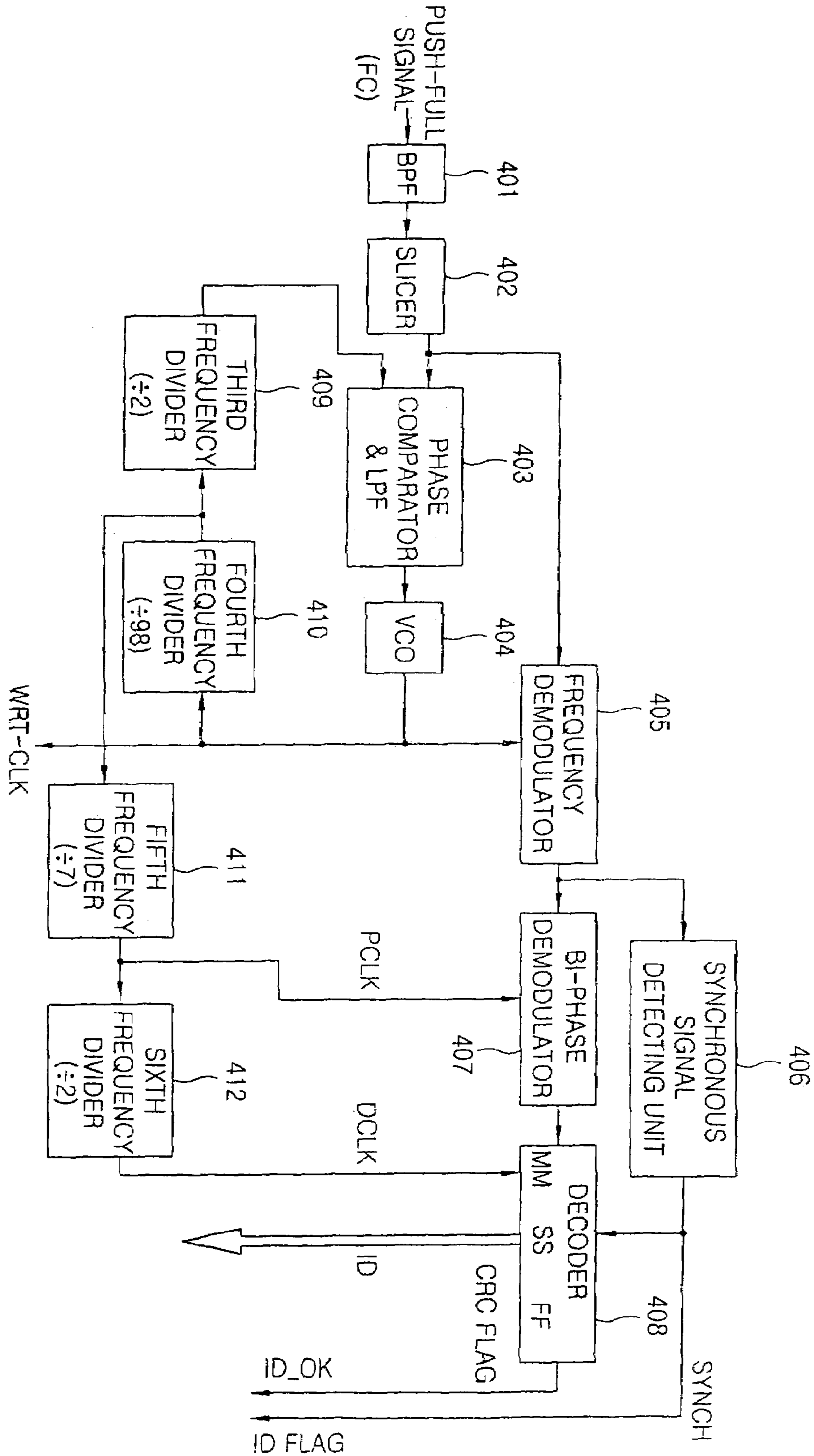
FIG. 4 CONVENTIONAL ART
