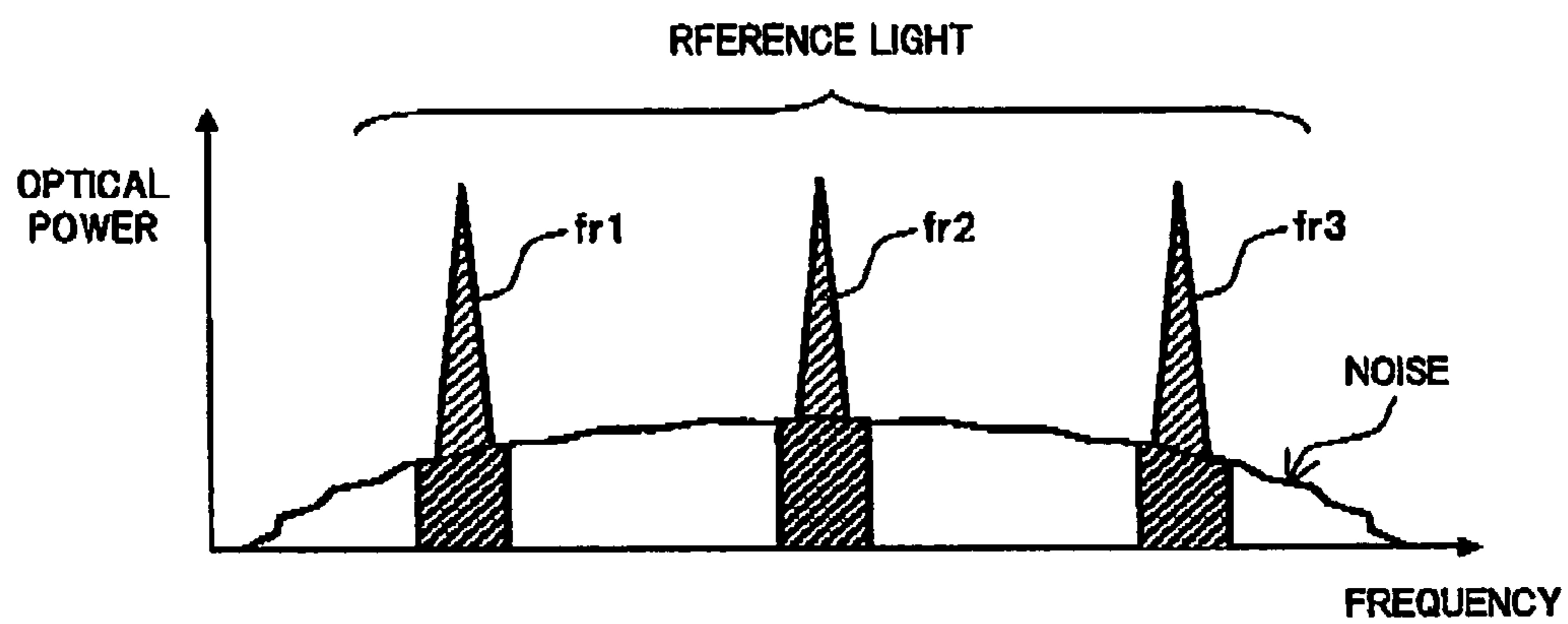
DIAGRAM EXPLAINING OPTICAL DETECTION IN EMBODIMENT 1-1
