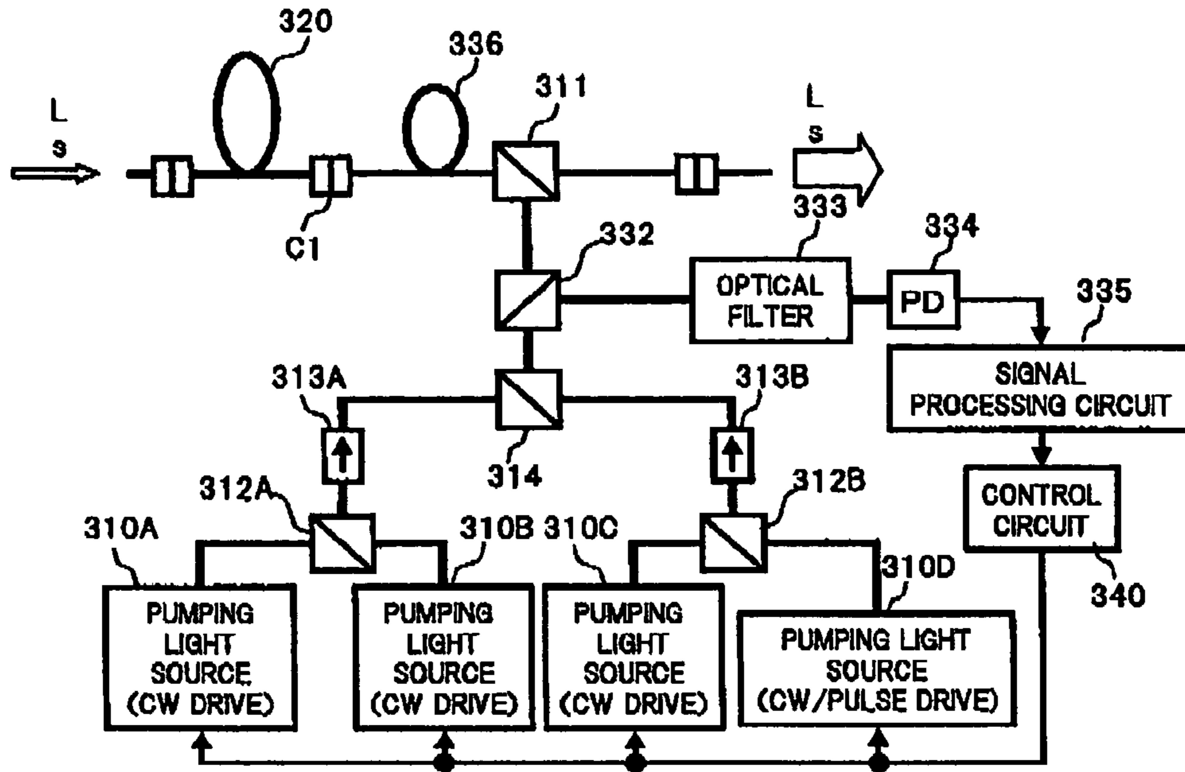
CONFIGURATION OF EMBODIMENT 3-3 OF PRESENT INVENTION
