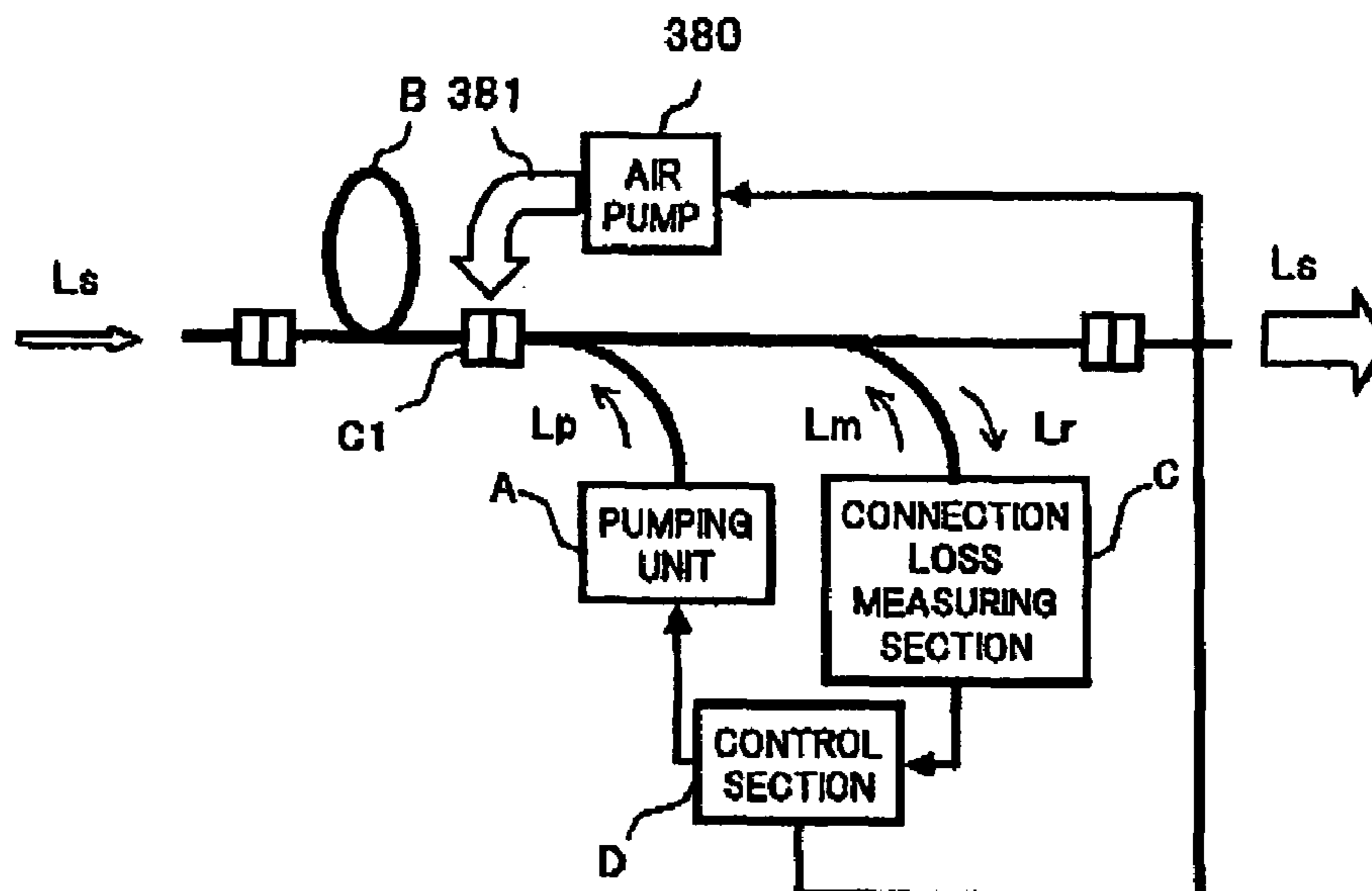
CONFIGURATION OF EMBODIMENT 3-5 OF PRESENT INVENTION
