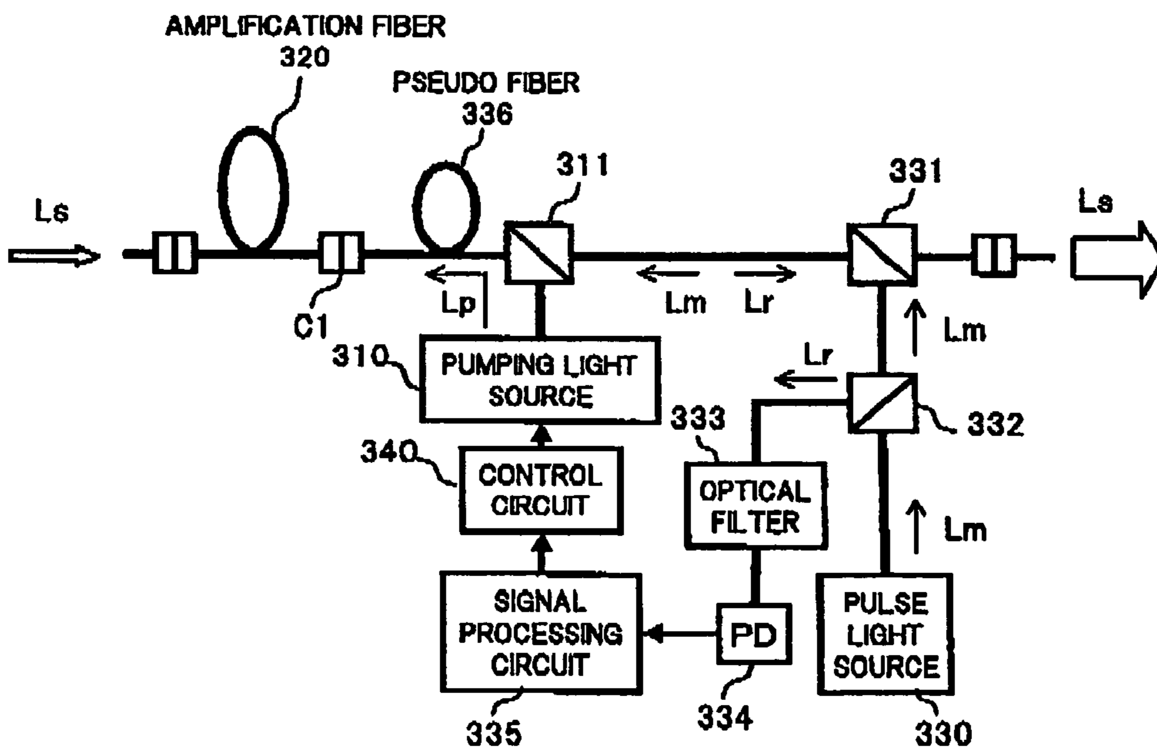
CONFIGURATION OF EMBODIMENT 3-1 OF PRESENT INVENTION
