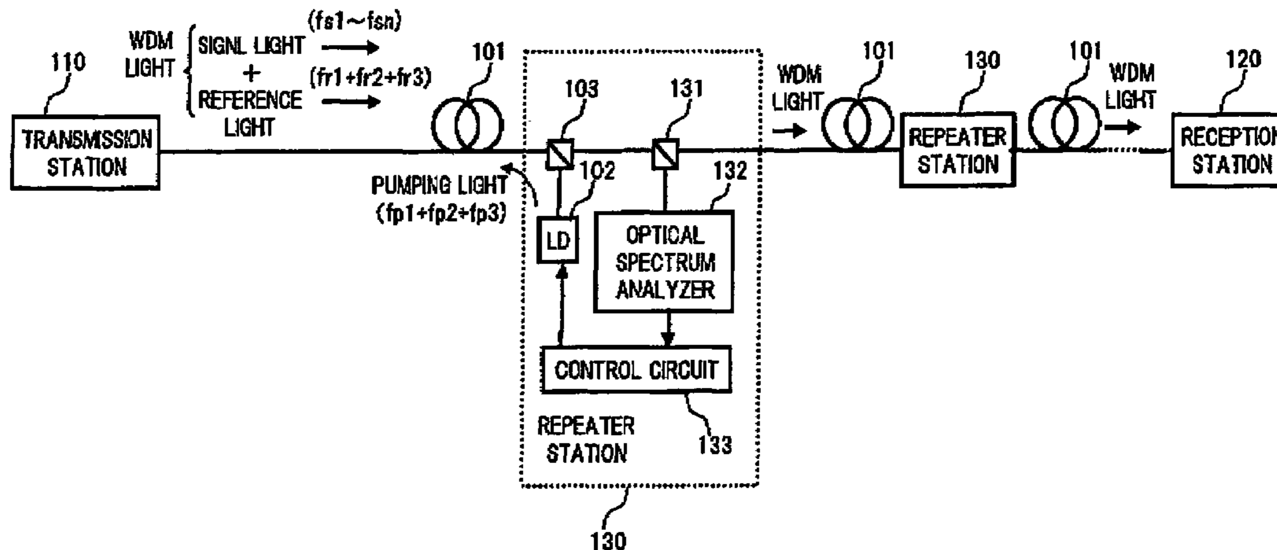
BLOCK DIAGRAM OF OPTICAL TRANSMISSION SYSTEM ACCORDING TO EMBODIMENT 1-1 OF PRESENT INVENTION
