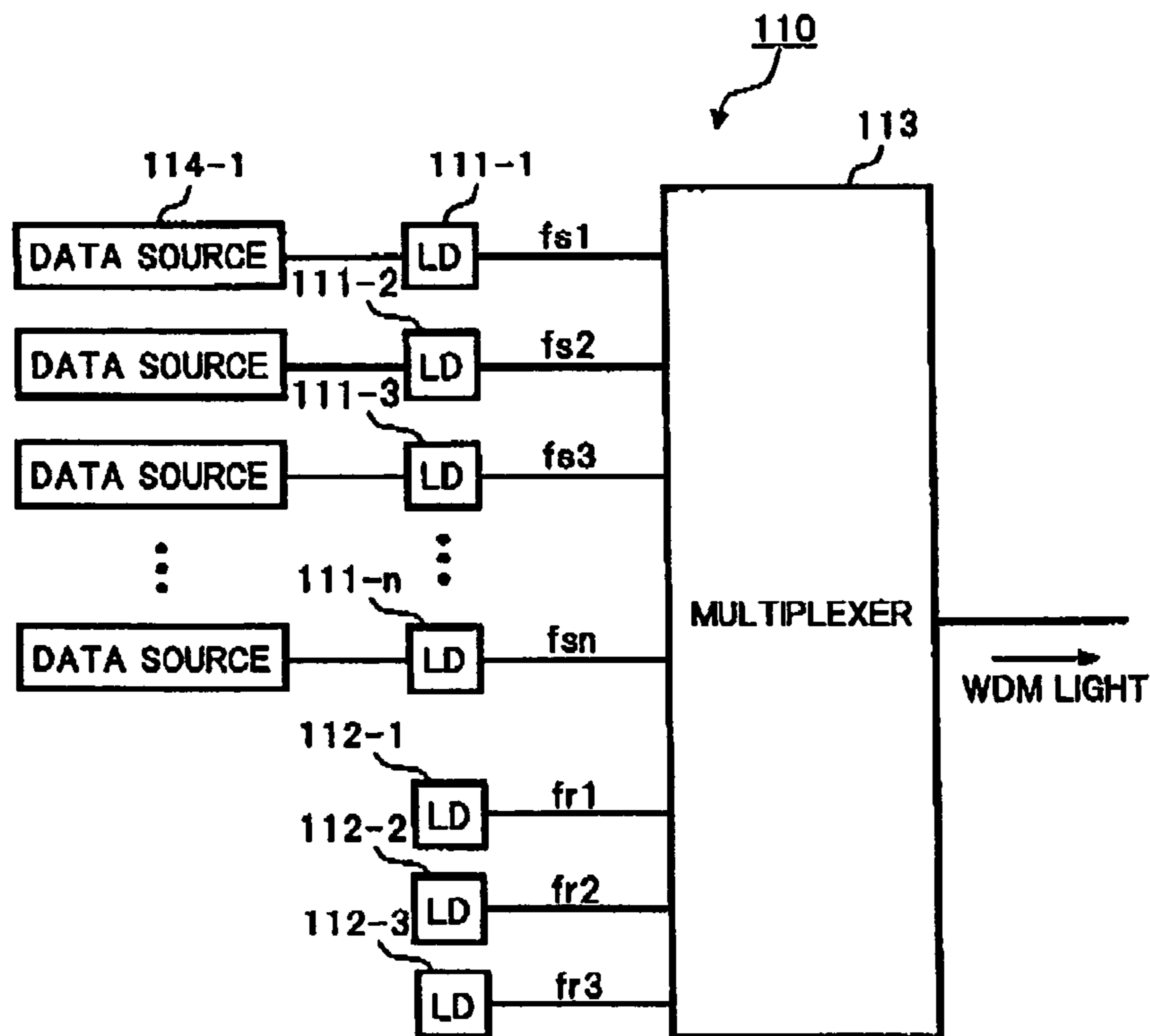
BLOCK DIAGRAM OF TRANSMISSION STATION
