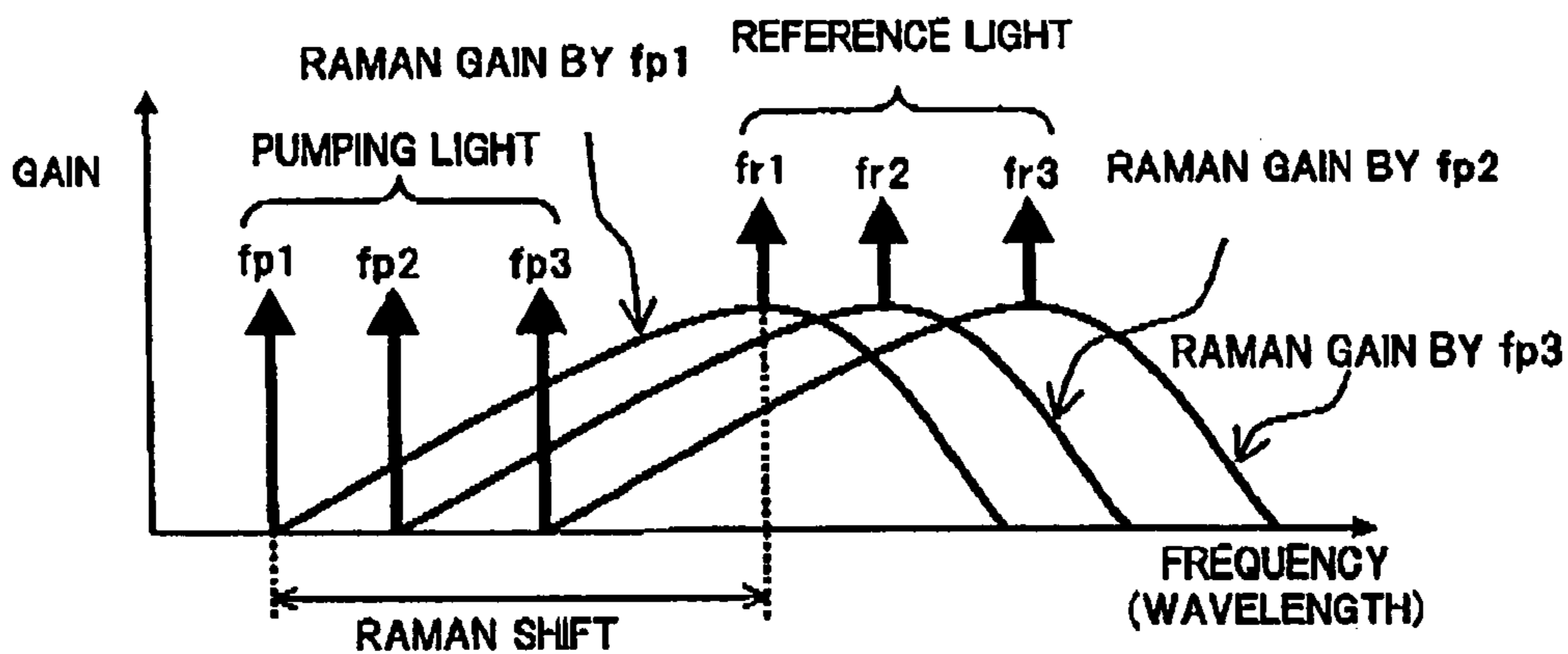
DIAGRAM EXPLAINING ARRANGING METHOD OF REFERENCE LIGHT
