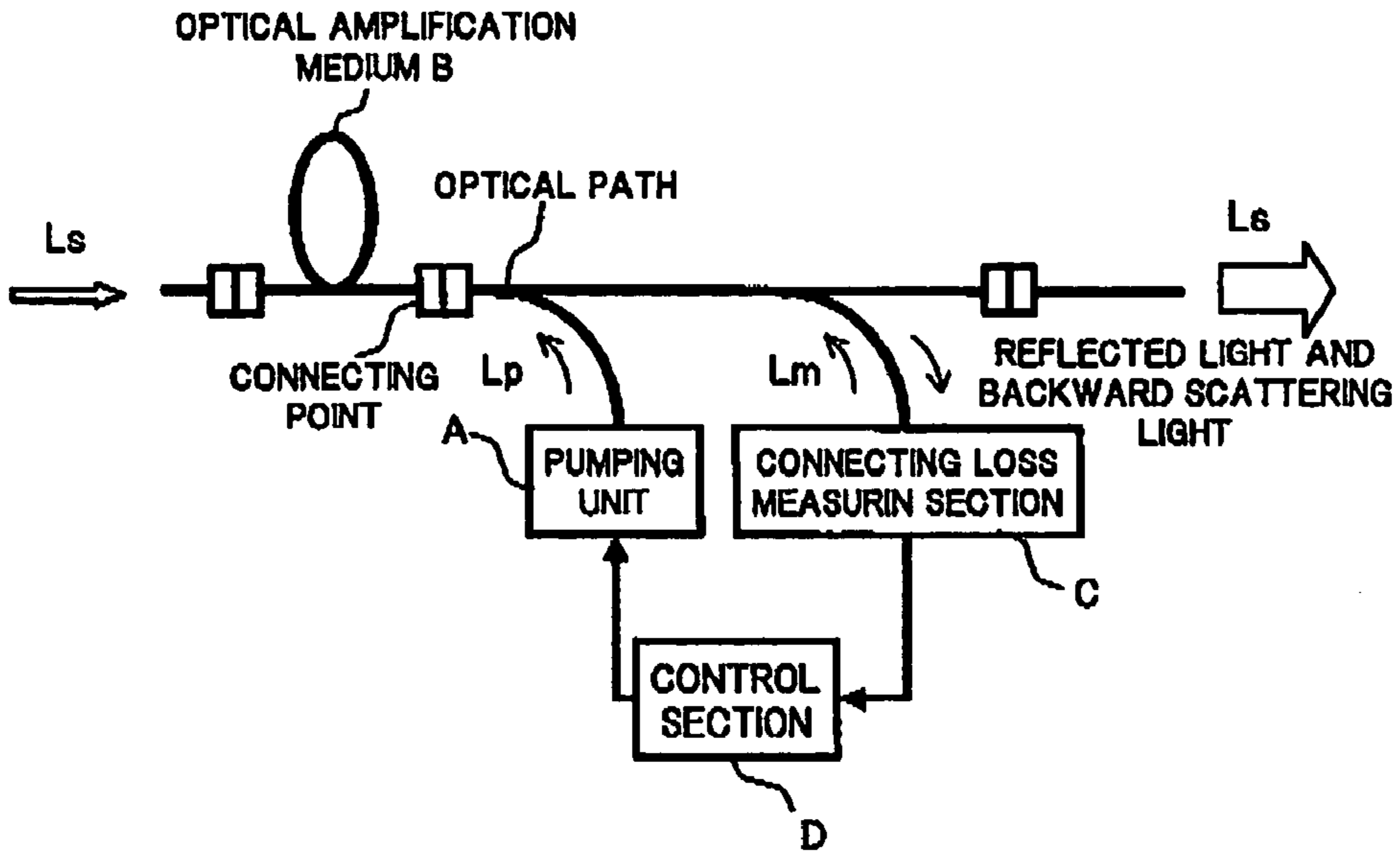
BASIC CONFIGURATION OF EMBODIMENT 3 OF PRESENT INVENTION
