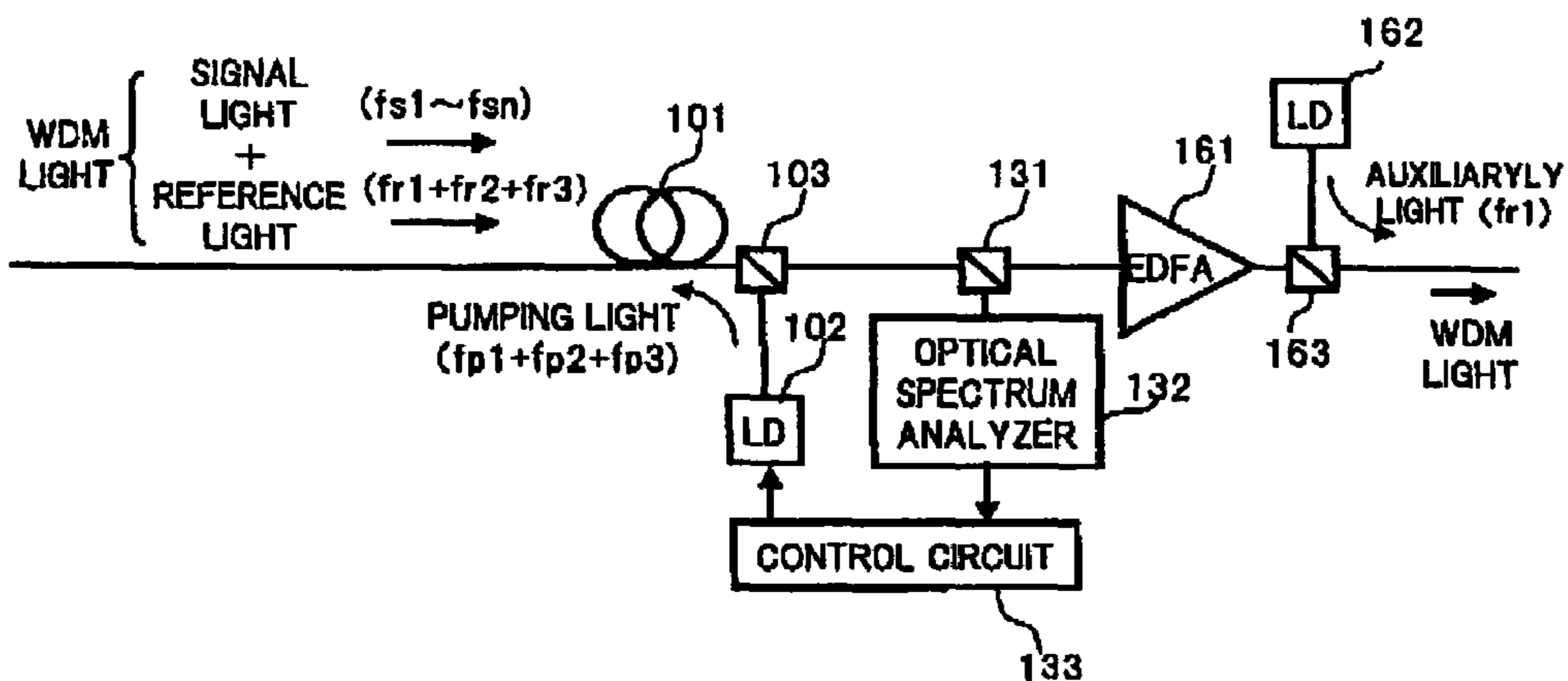
BLOCK DIAGRAM OF REPEATER STATION OF OPTICAL TRANSMISSION SYSTEM ACCORDING TO EMBODIMENT 1-2
