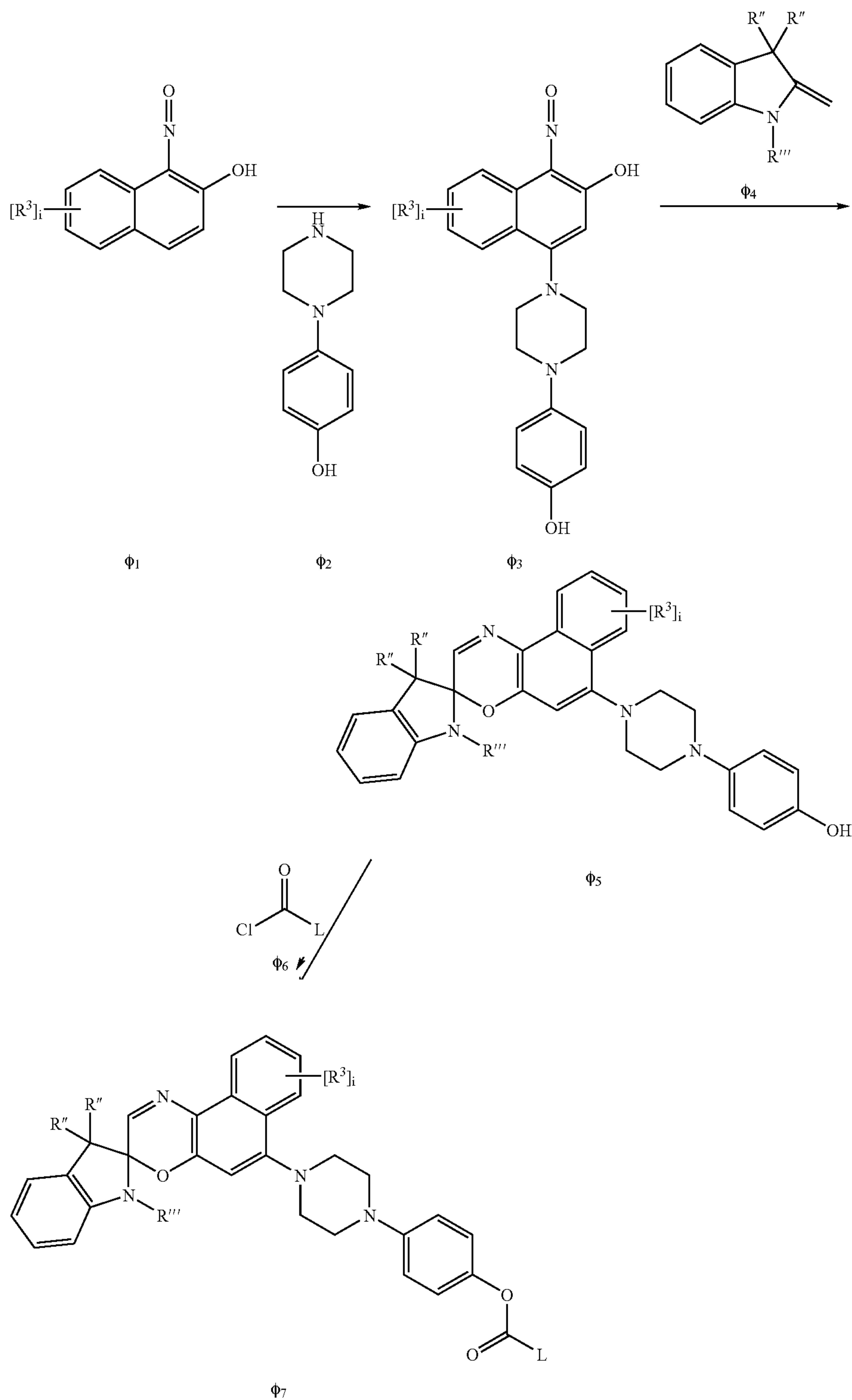
Reaction Sequence J
