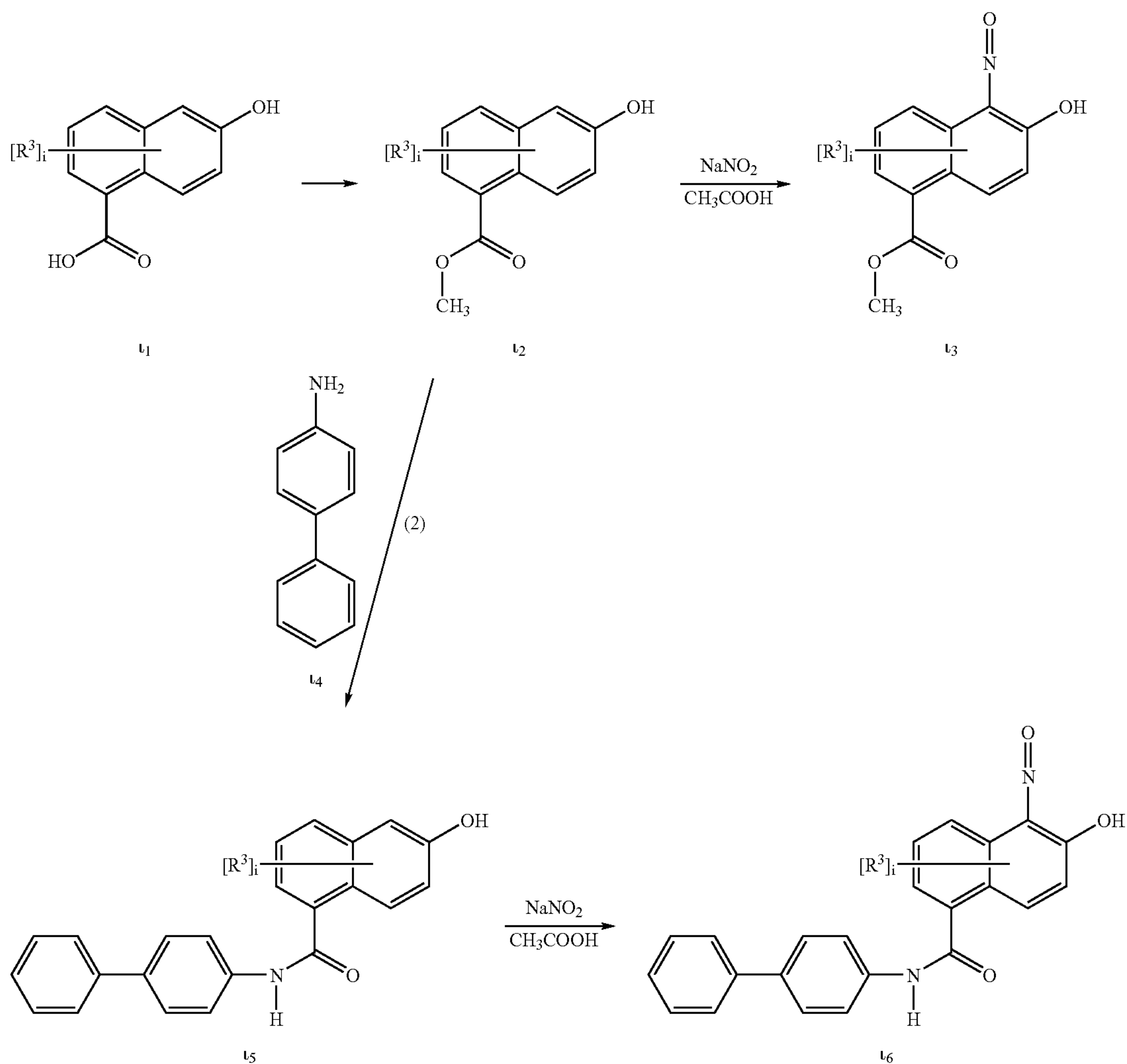
Reaction Sequence I
