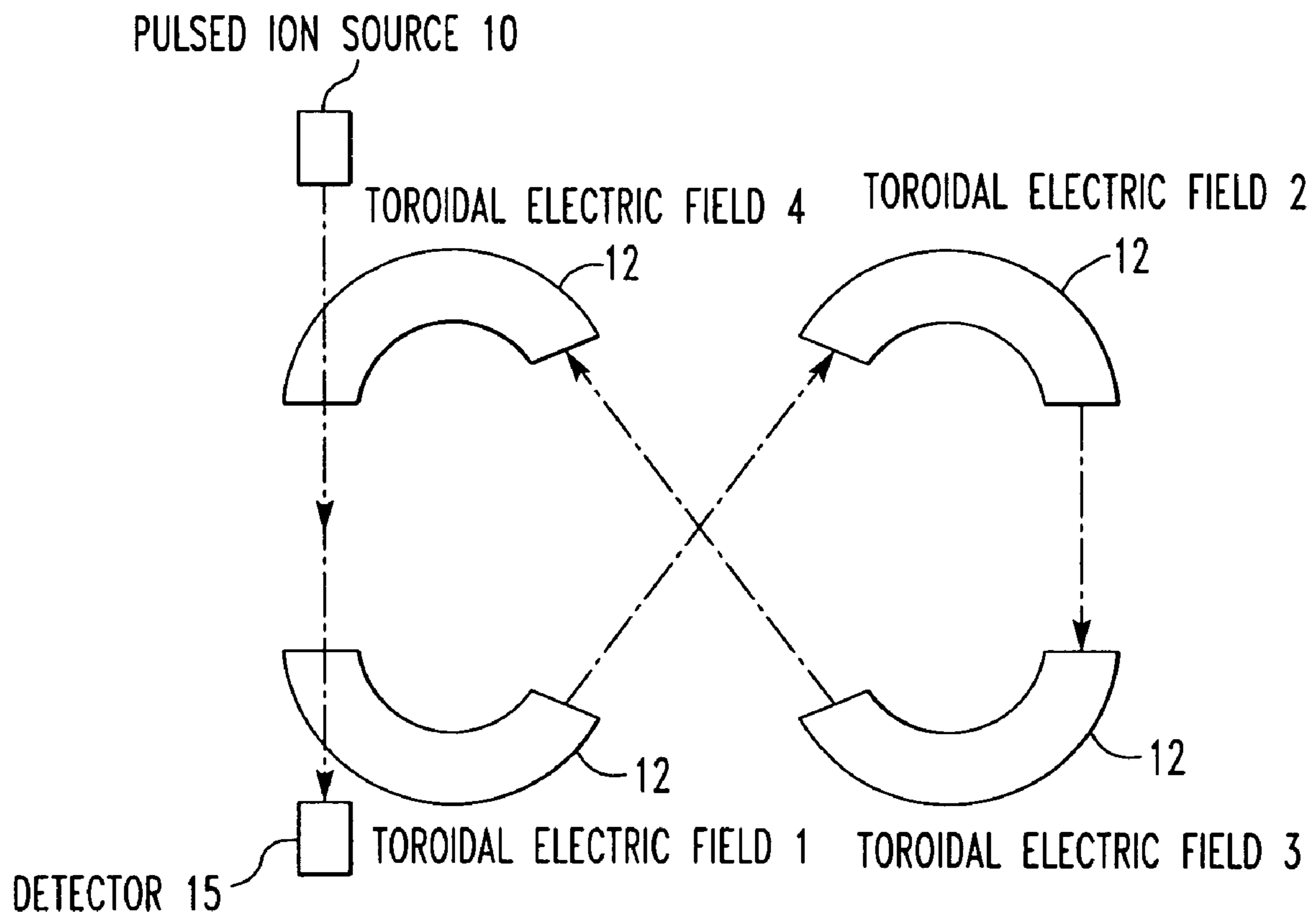
FIG. 28 PRIOR ART
