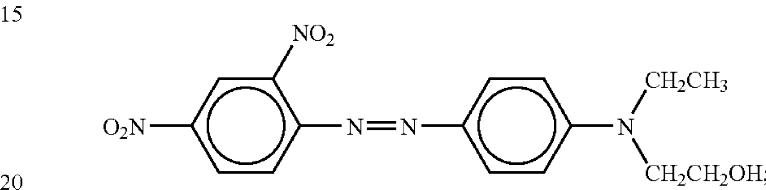
Disperse Red 98 (C.I. 11191), of the formula
