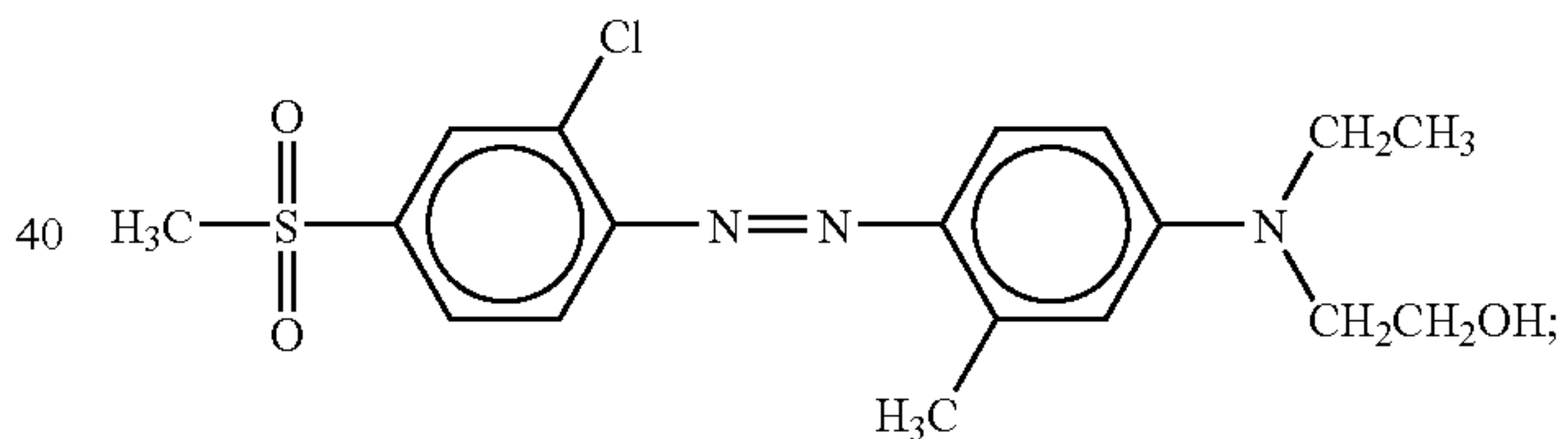
Disperse Red 97 (Cl. 11232), of the formula
