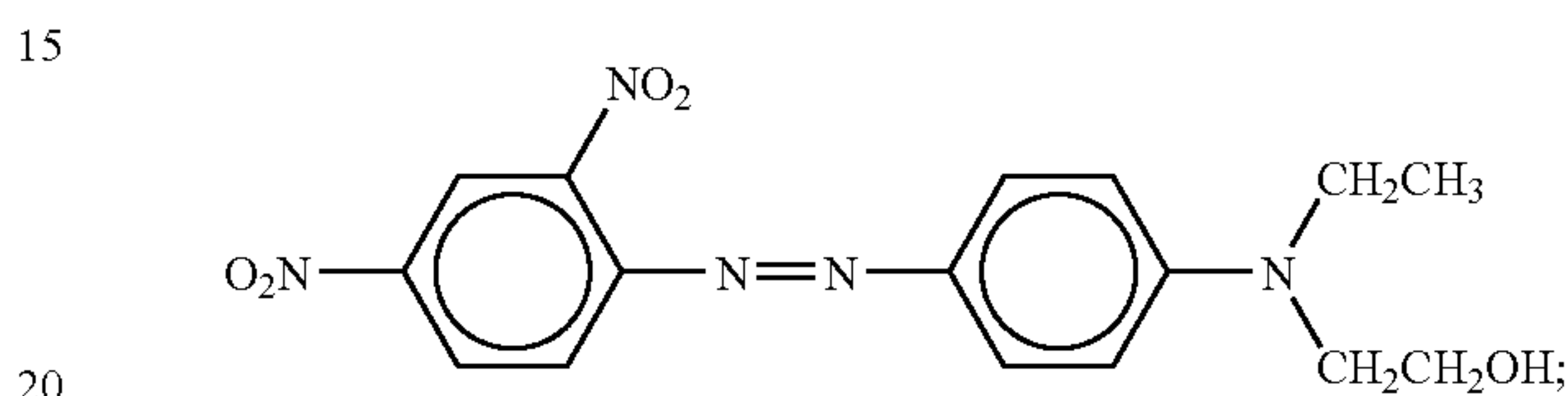
Disperse Red 98 (C.I. 11191), of the formula
