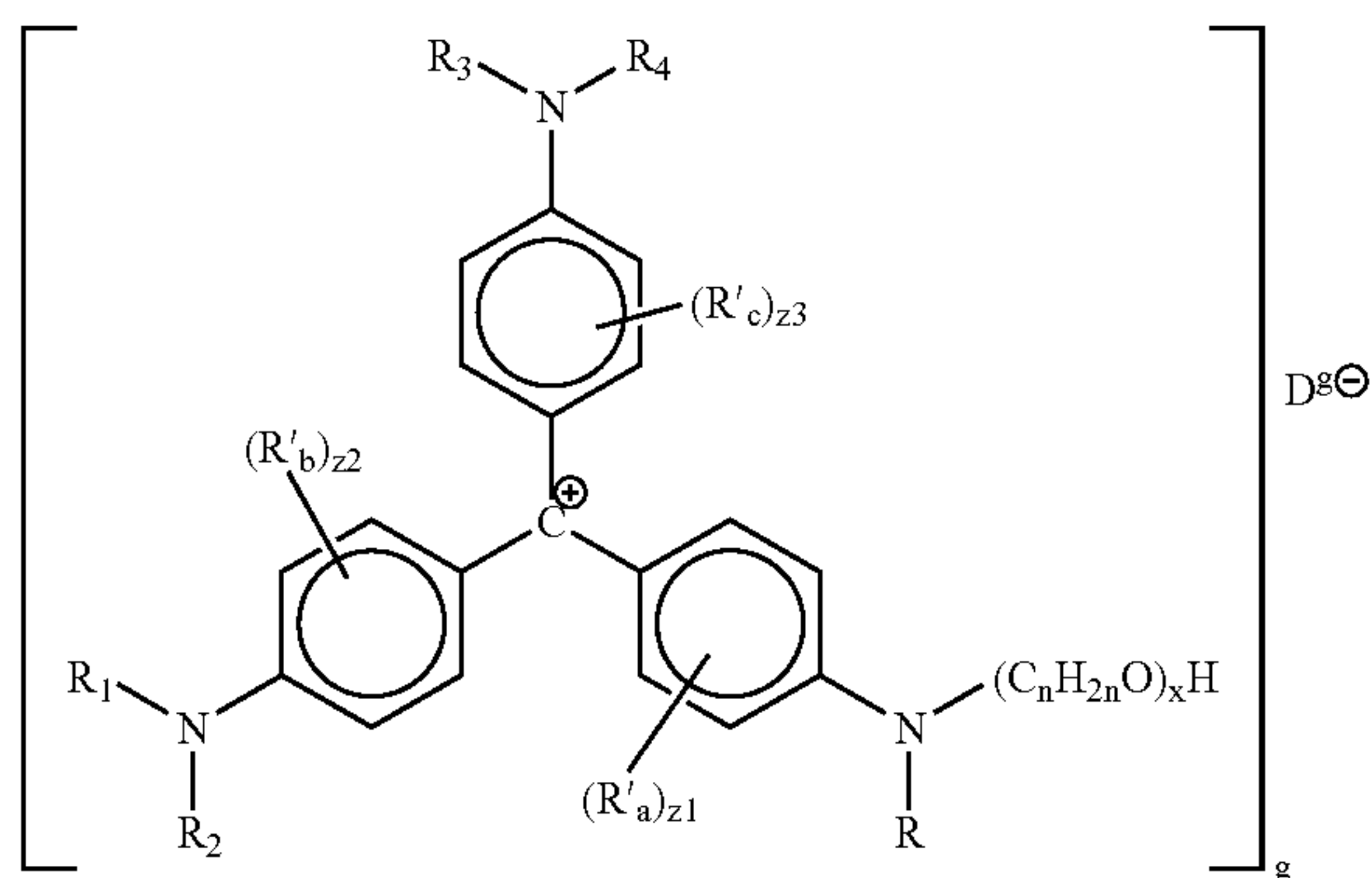
Disperse Blue 34 (C.I. 61510), of the formula
