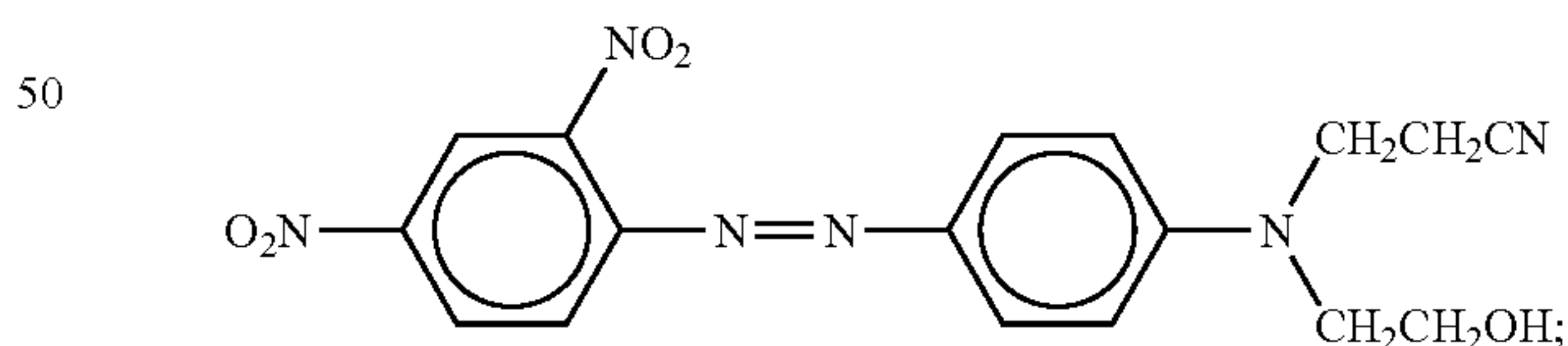
colorants of the formulae
