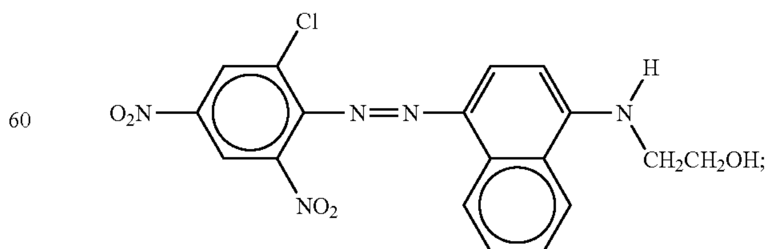
Disperse Blue 8 (C.I. 60742), of the formula
