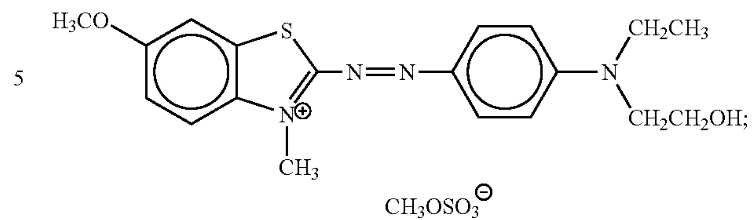
Disperse Red 8 (C.I. 11113), of the formula
