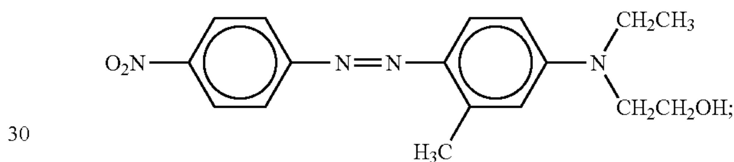
Disperse Red 109 (C.I. 11192), of the formula
