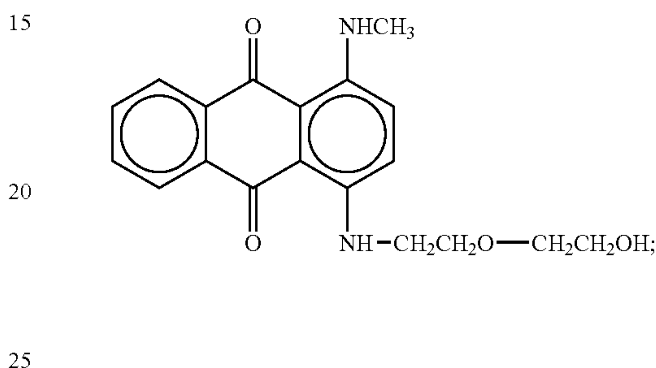
Disperse Red 156 (C.I. 11235), of the formula
