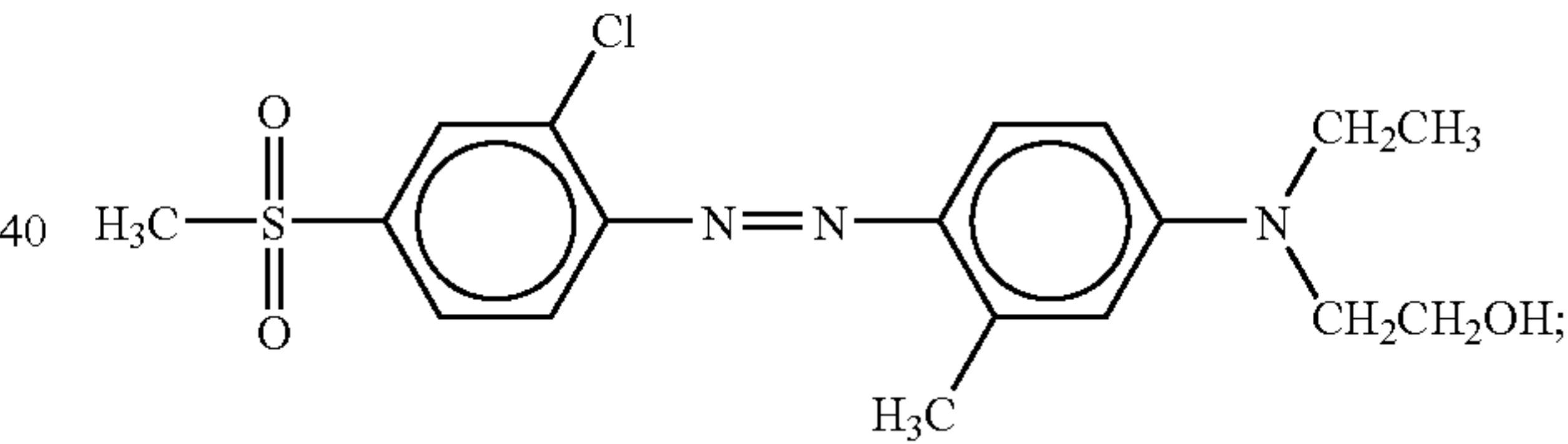
Disperse Red 97 (Cl. 11232), of the formula
