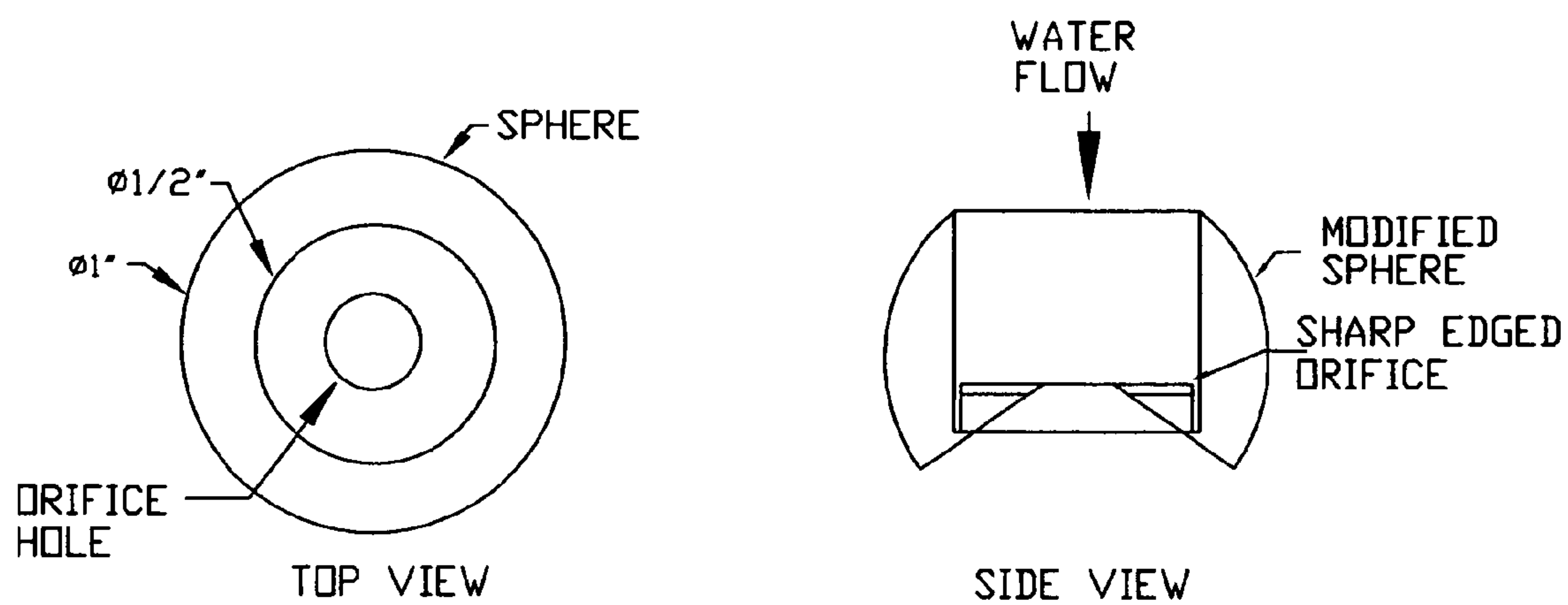
MODIFIED ORIFICE ASSEMBLY FIG 11 AMMENDED
