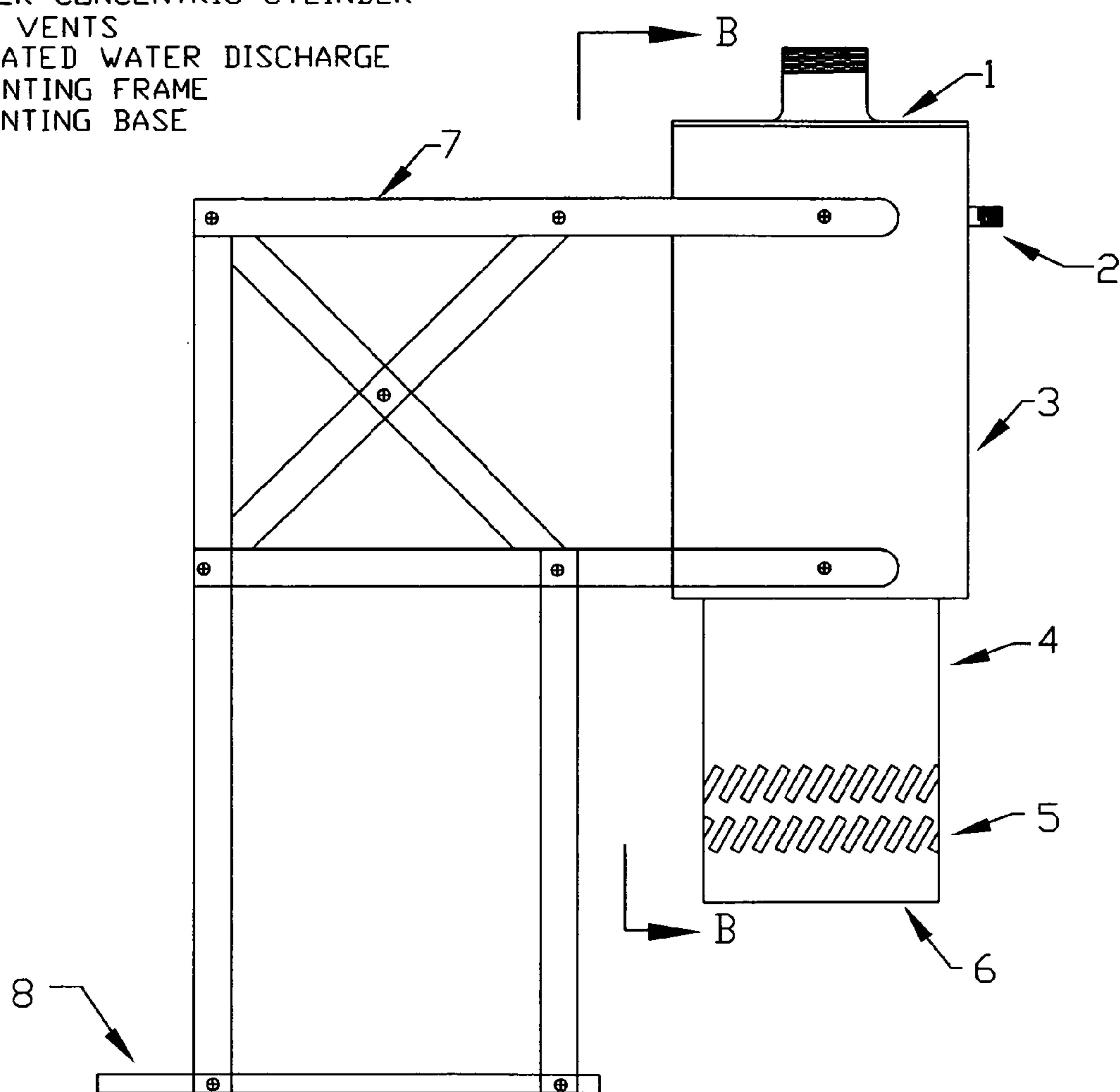
EXTERNAL VIEW ACID MINE WATER DEMINERALIZER FIG 1 AMENDED
