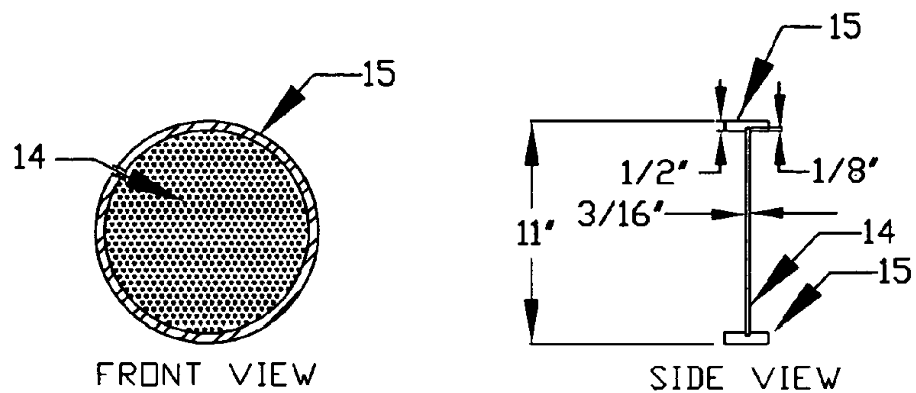
POROUS PLATE ASSEMBLY FIG 7 AMMENDED
