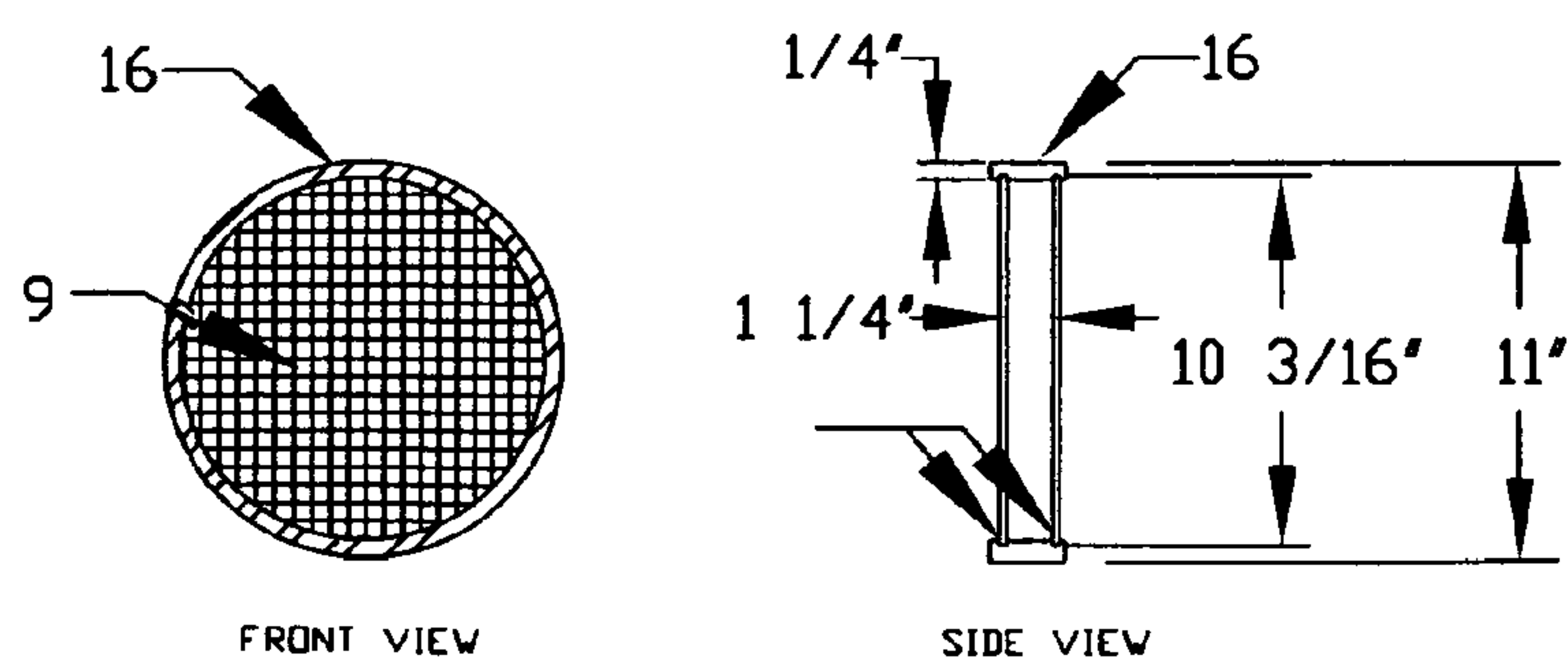
SCREEN AND HOLDER FIG 8 AMMENDED
